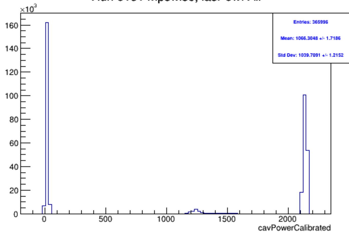
Run 6131 mpwise, lasPow: All
