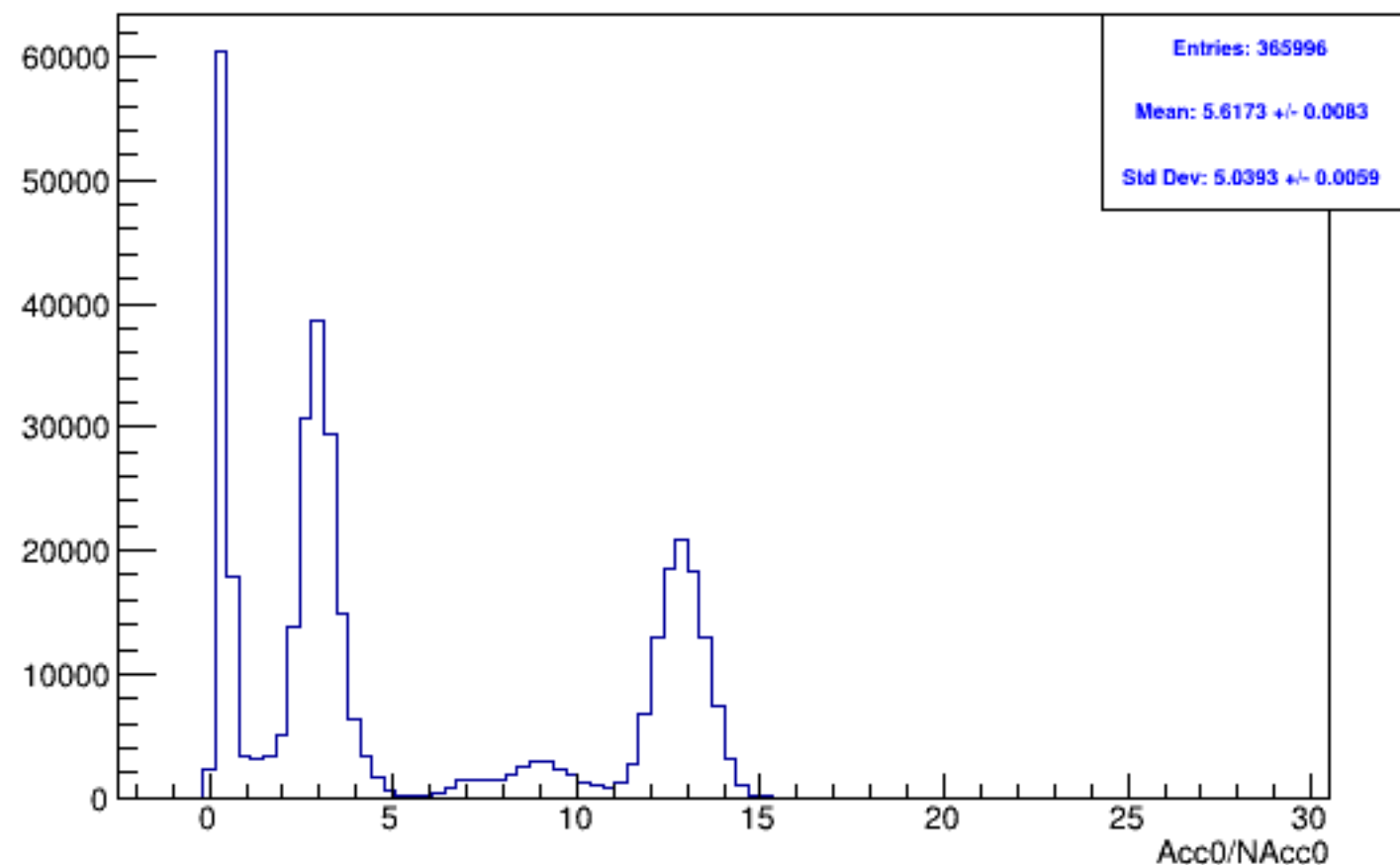
Run 6131 mpwise, acc0: All
