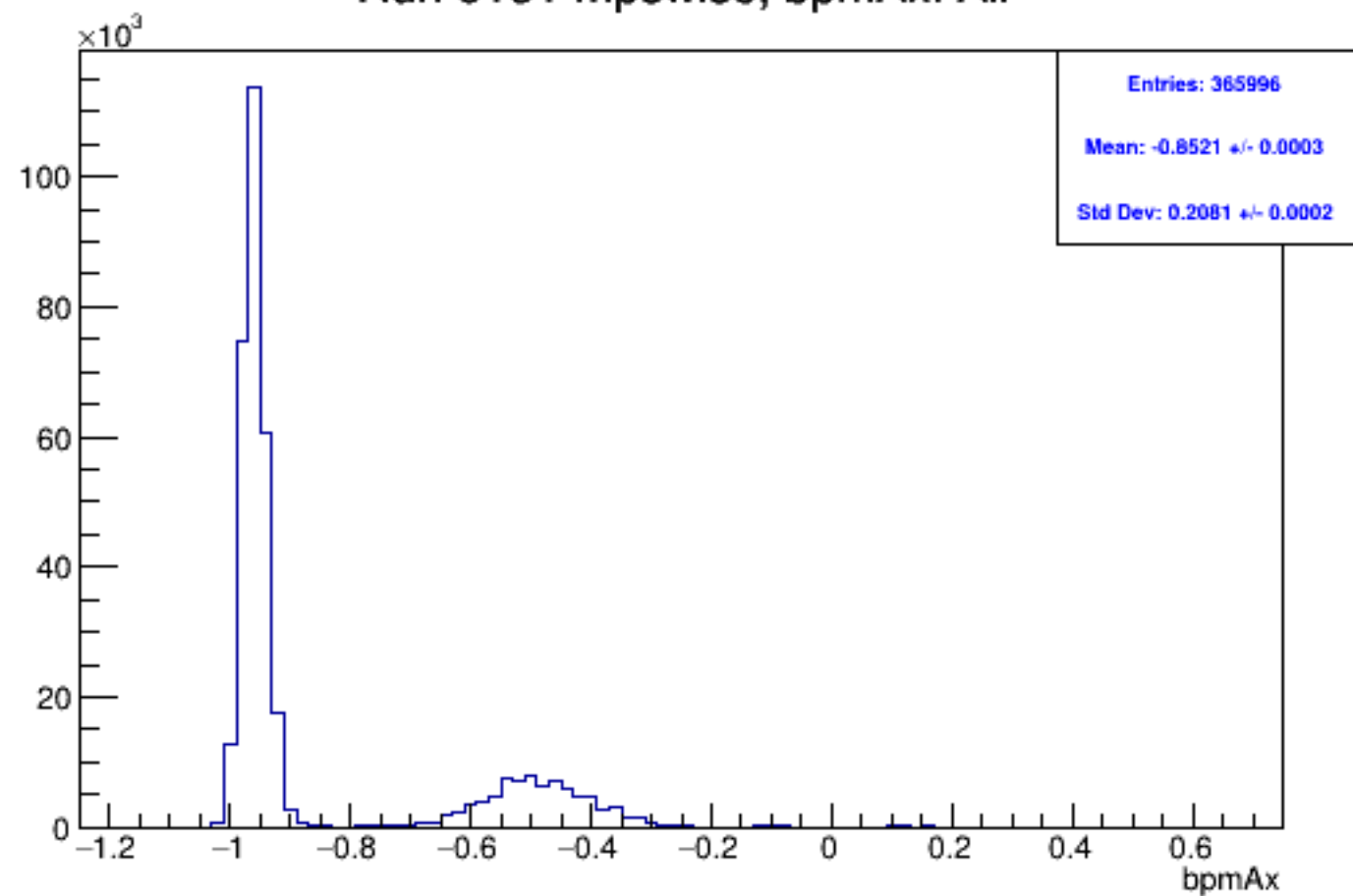
Run 6131 mpwise, bpmAx: All
