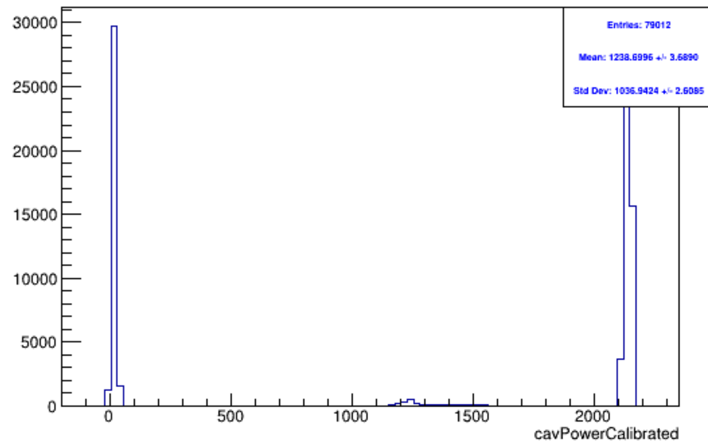
Run 6131 mpwise, lasPow: Beam OFF
