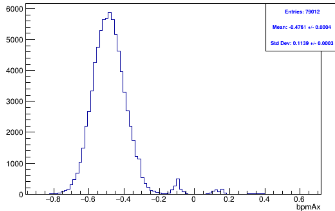
Run 6131 mpwise, bpmAx: Beam OFF
