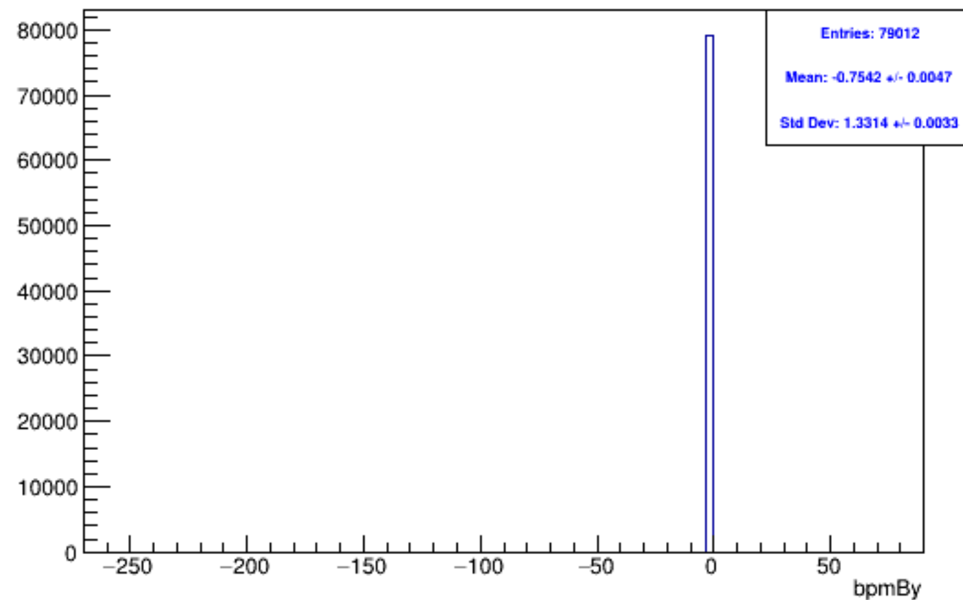
Run 6131 mpwise, bpmBy: Beam OFF
