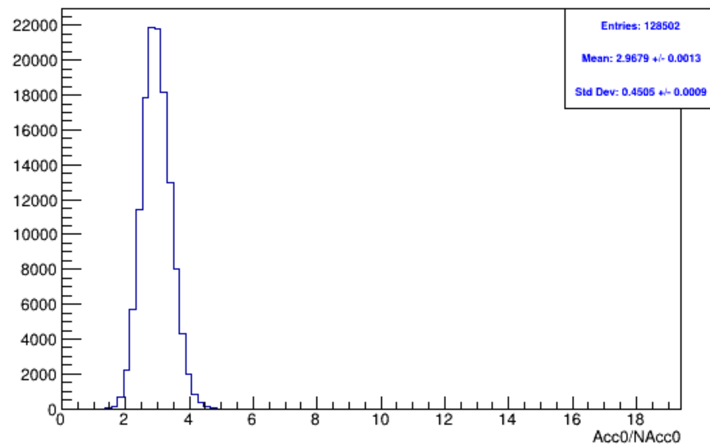
Run 6131, mpwise, acc0: Beam ON, Laser OFF
