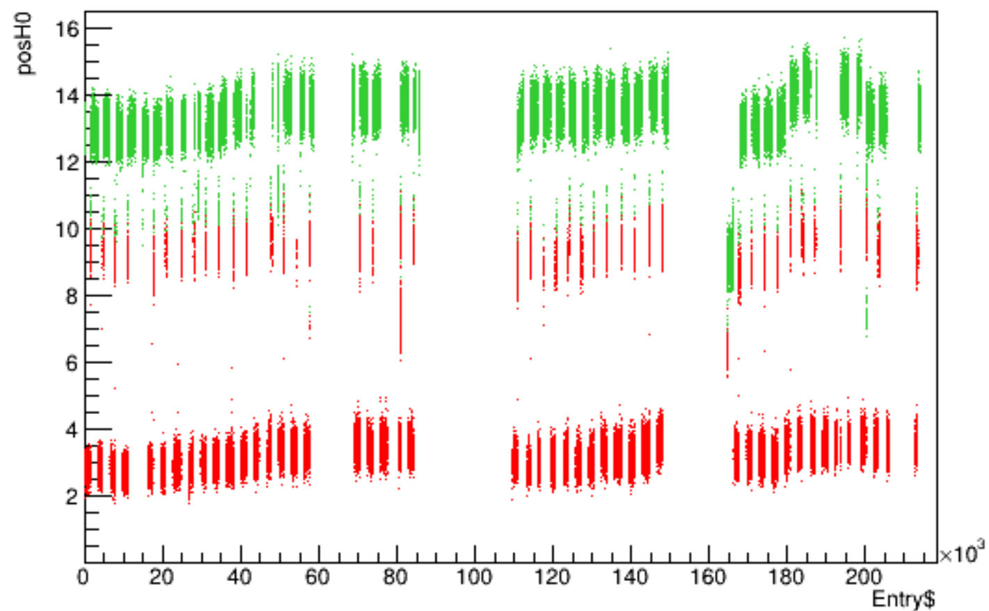
Run 6142 quartetwise, posH0 vs time
