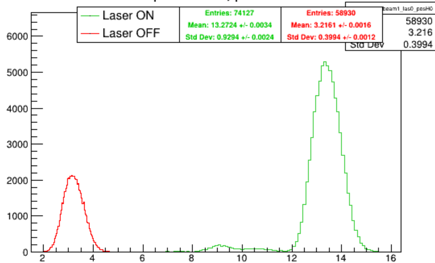
Run 6142 quartetwise, posH0: Beam ON
