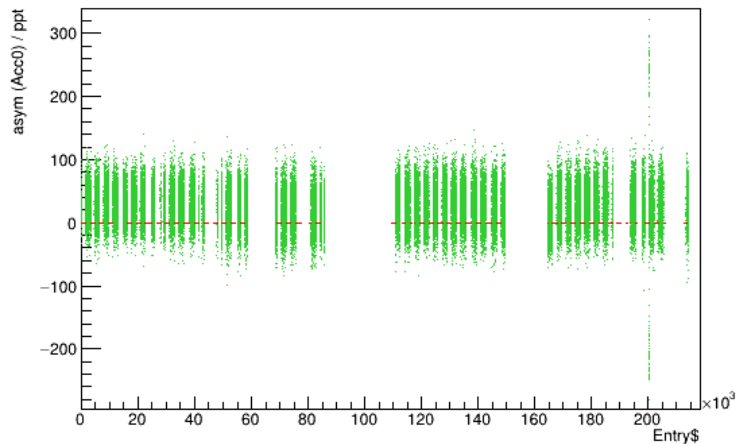
Run 6142 quartetwise, asym0sub vs time
