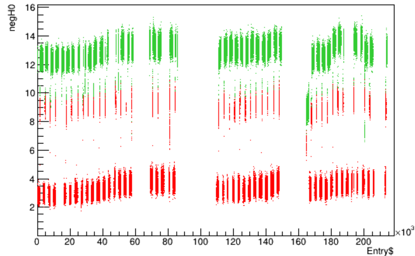
Run 6142 quartetwise, negH0 vs time
