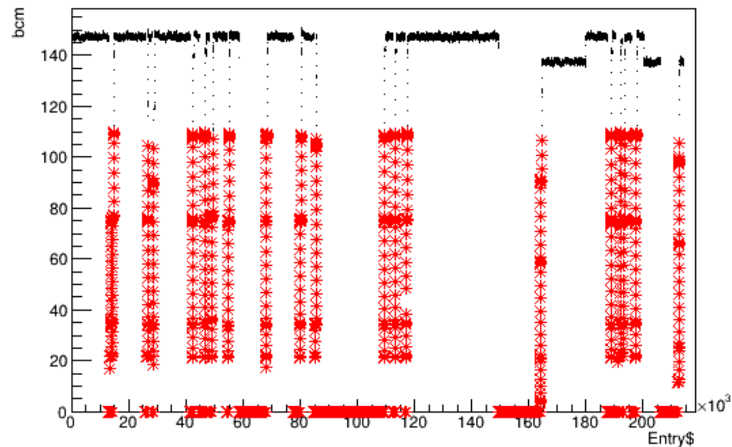
Run 6142 quartetwise, bcm vs time
