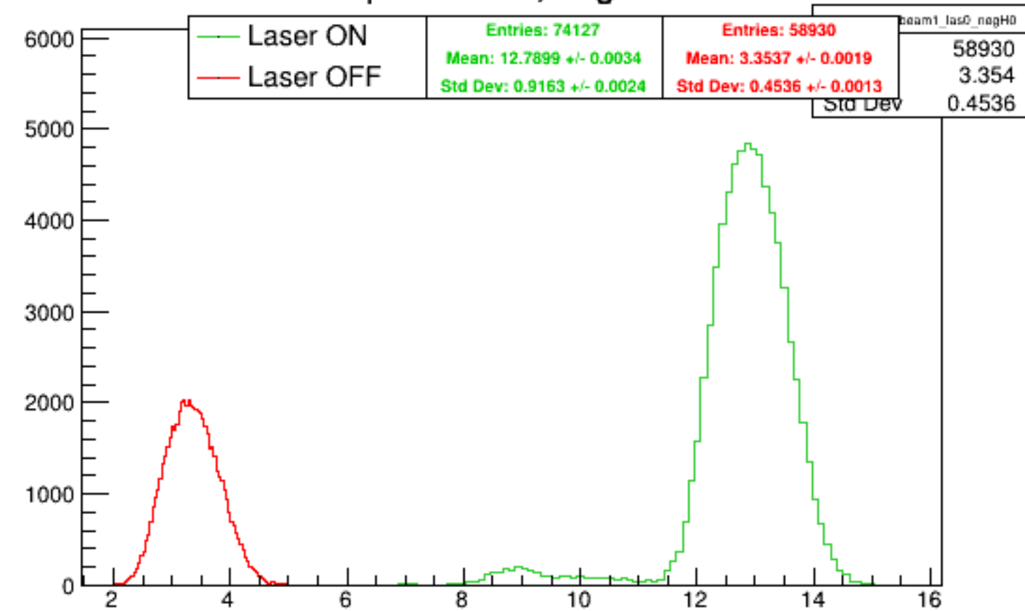
Run 6142 quartetwise, negH0: Beam ON
