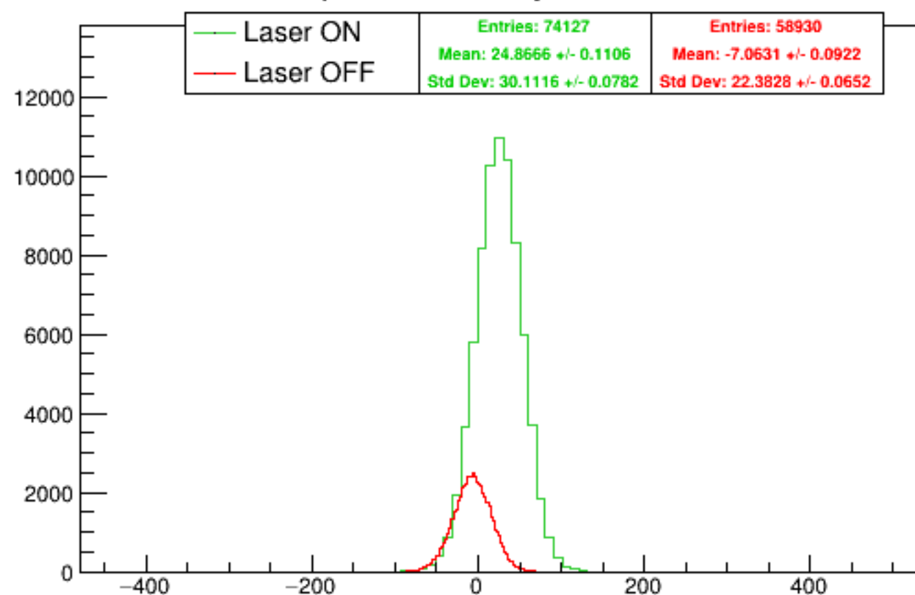
Run 6142 quartetwise, asym0sub: Beam ON
