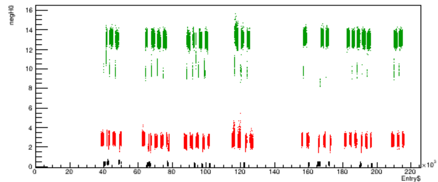
Run 6149 quartetwise, negH0 vs time
