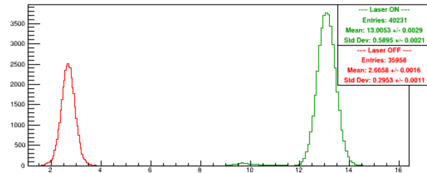
Run 6149 quartetwise, NegHelAcc0/NSamples0
