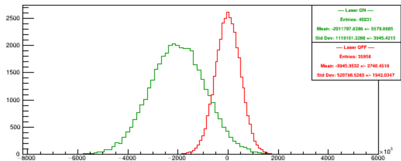
Run 6149 quartetwise, Diffs4
