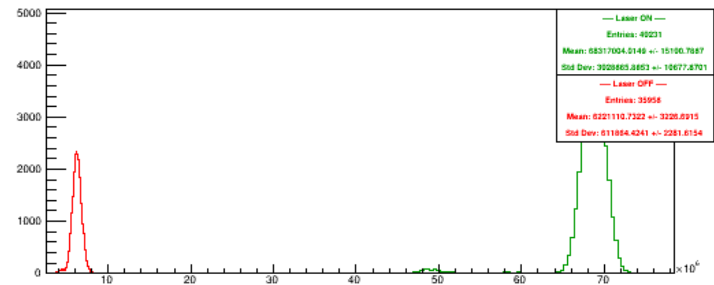
Run 6149 quartetwise, Sums4
