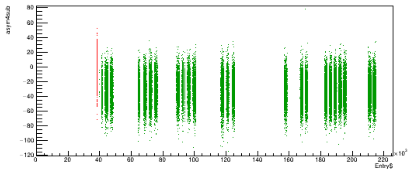
Run 6149 quartetwise, asym4sub vs time
