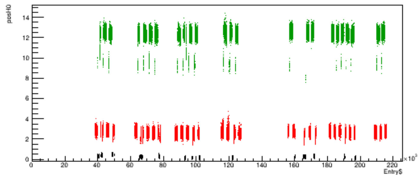
Run 6149 quartetwise, posH0 vs time
