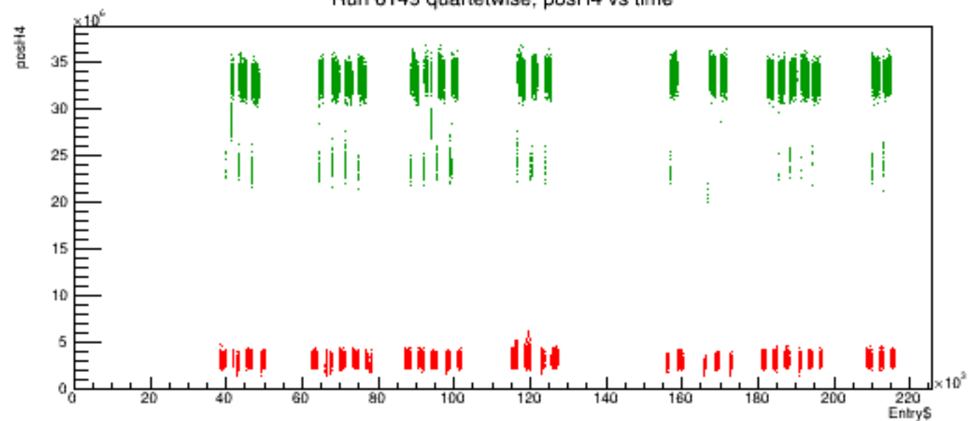
Run 6149 quartetwise, posH4 vs time
