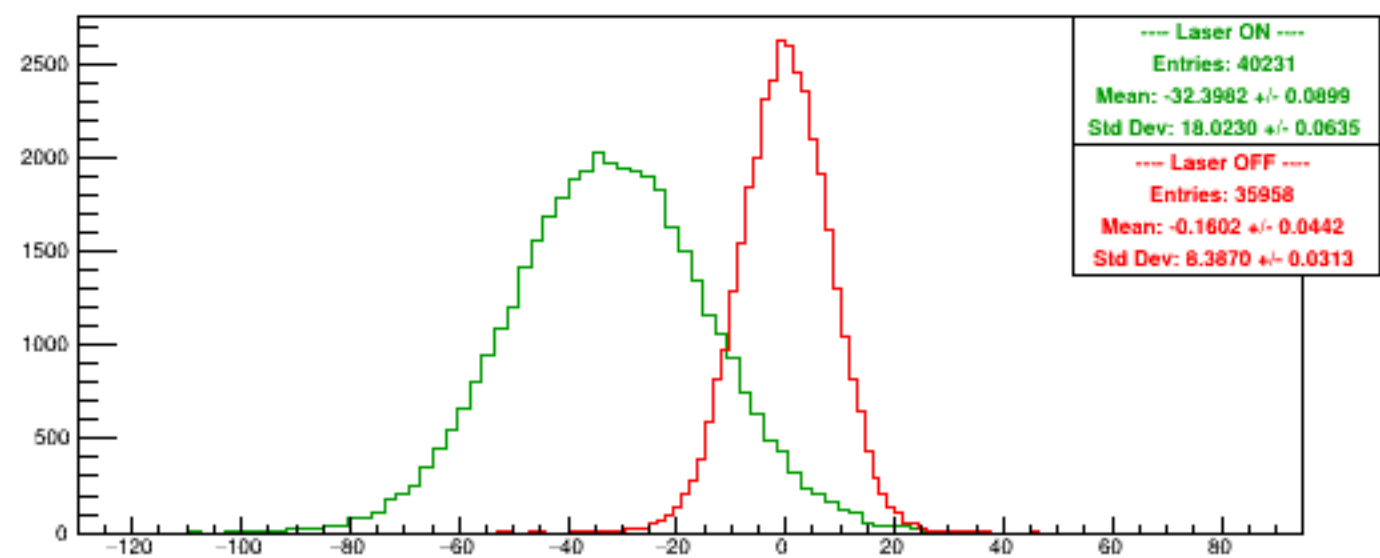
Run 6149 quartetwise, Asyms4
