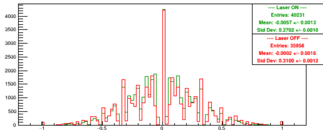
Run 6149 quartetwise, Asyms Horiz Finger
