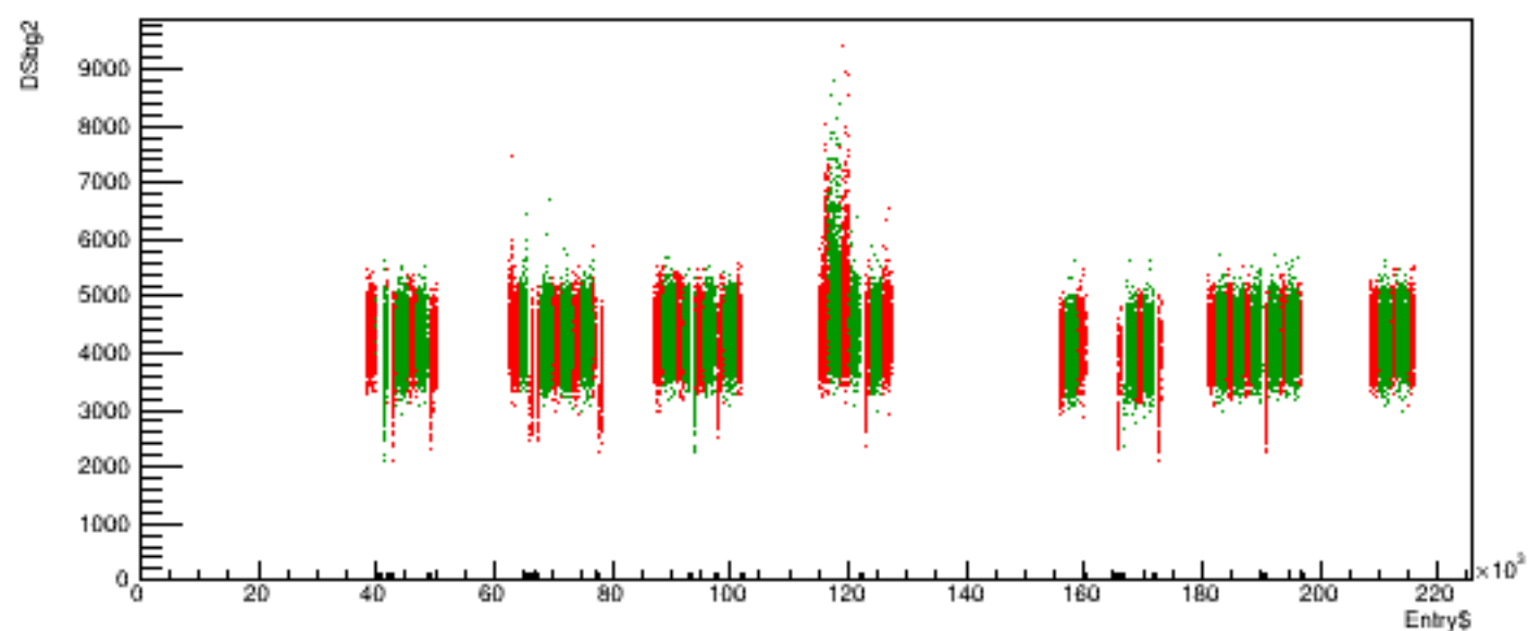
Run 6149 quartetwise, DSbg2 vs time
