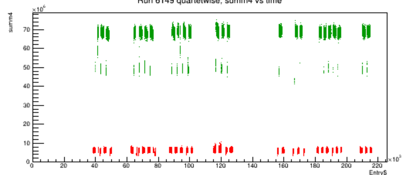
Run 6149 quartetwise, summ4 vs time
