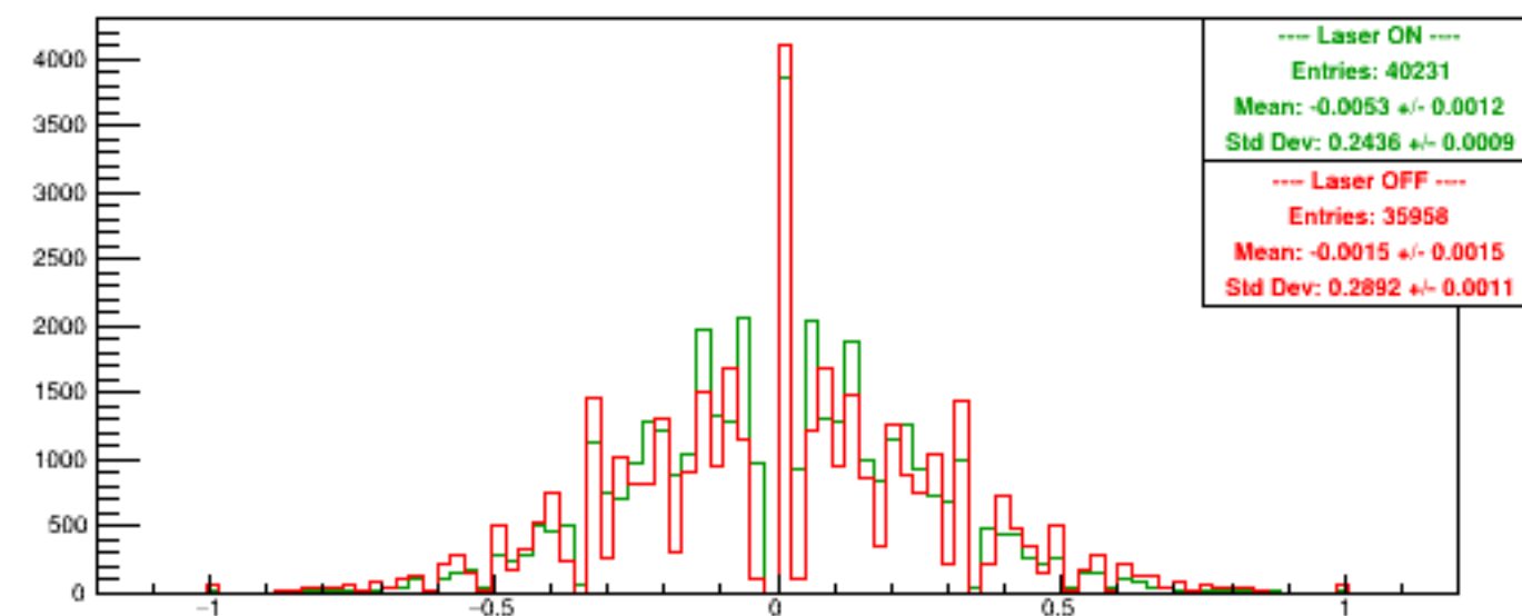
Run 6149 quartetwise, Asyms Vert Finger
