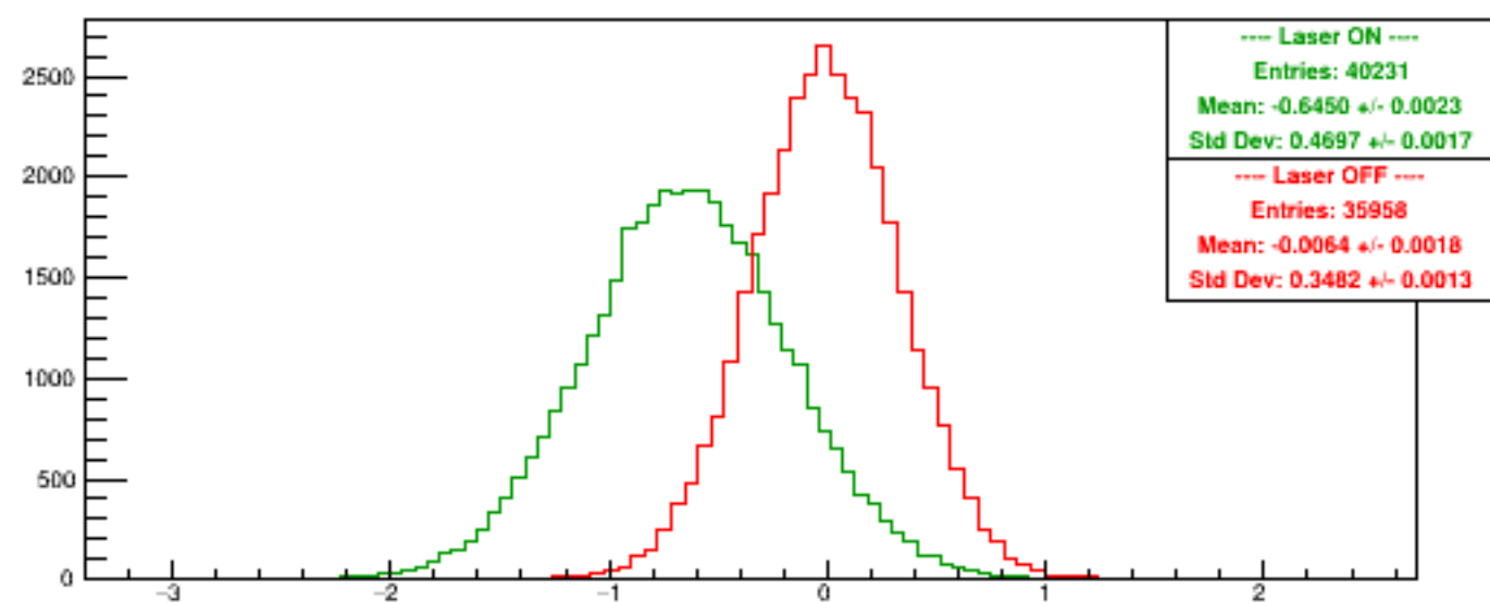
Run 6149 quartetwise, Diffs0
