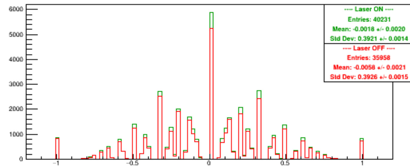
Run 6149 quartetwise, Asyms USbg2
