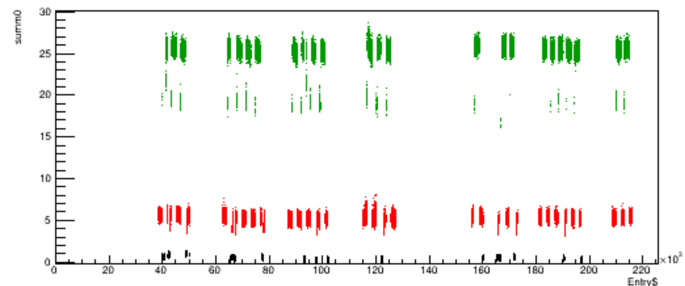
Run 6149 quartetwise, summ0 vs time
