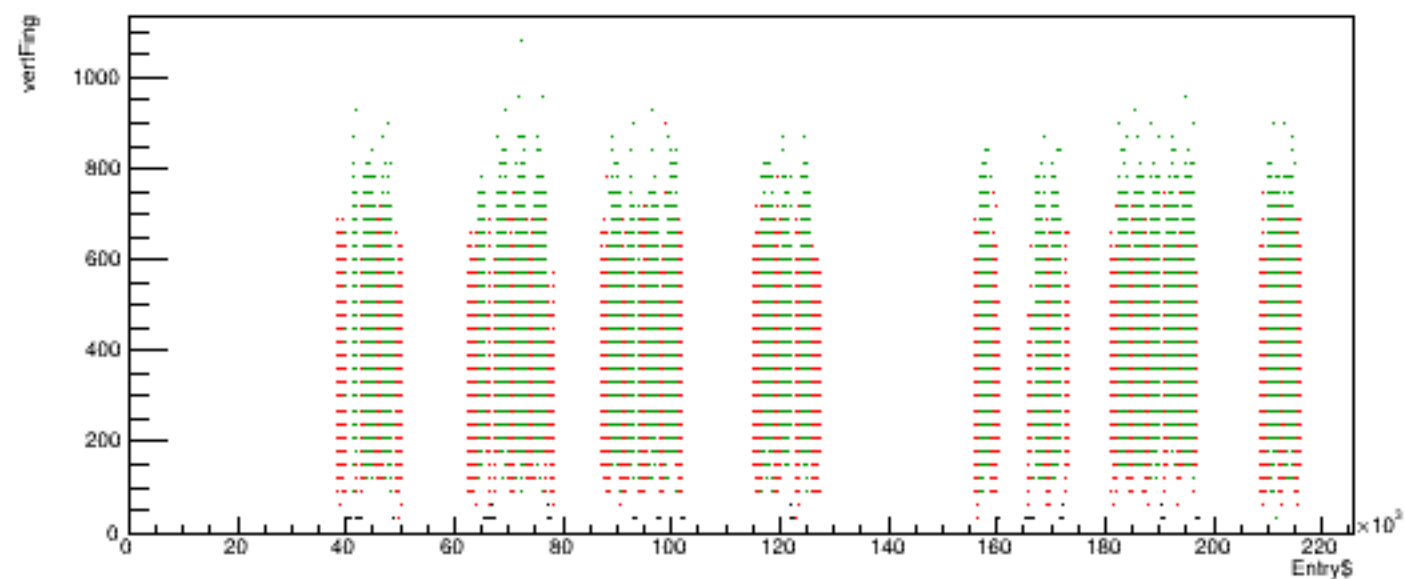
Run 6149 quartetwise, vertFing vs time
