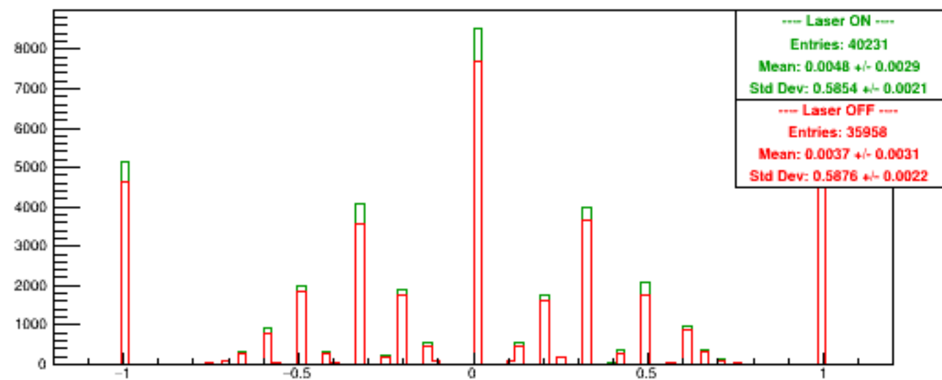
Run 6149 quartetwise, Asyms USbg1
