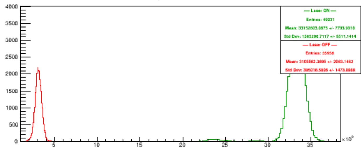
Run 6149 quartetwise, PosHelAcc4
