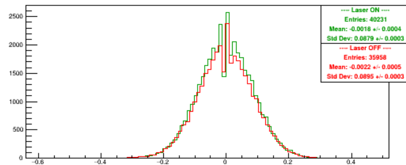
Run 6149 quartetwise, Asyms DSbg2
