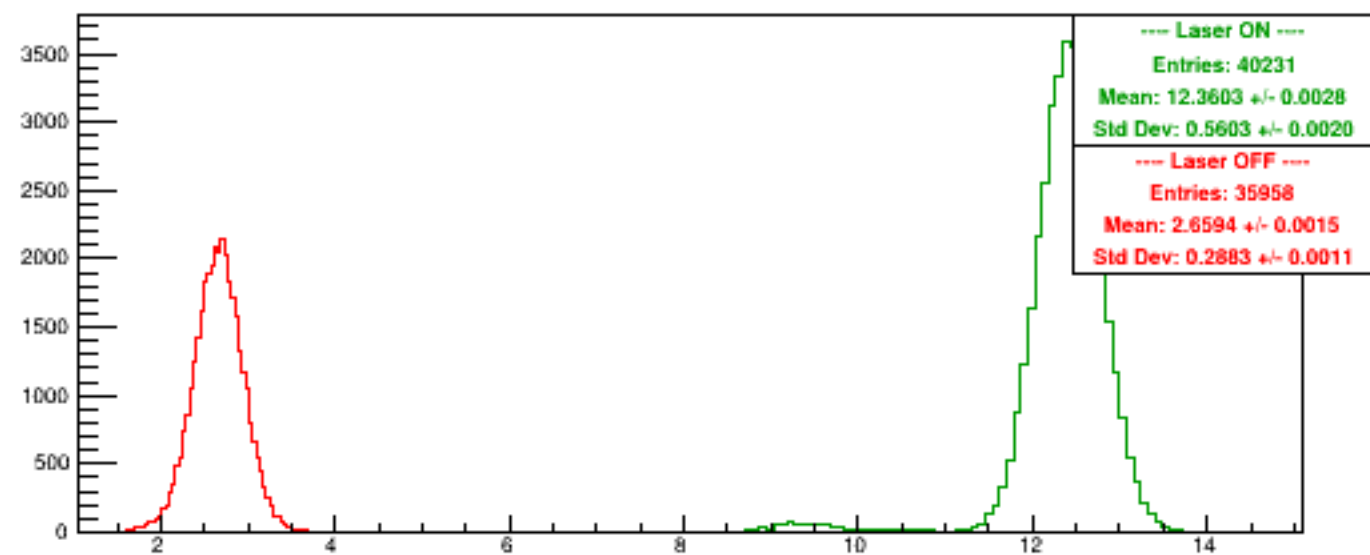
Run 6149 quartetwise, PosHelAcc0/NSamples0
