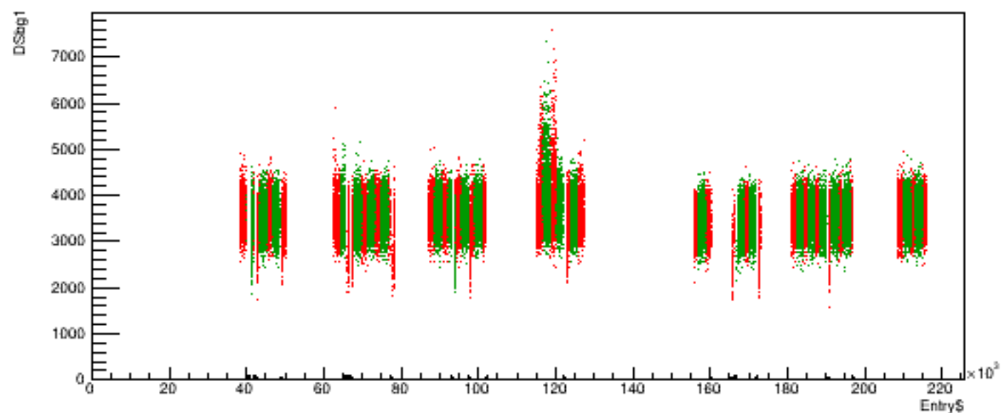
Run 6149 quartetwise, DSbg1 vs time
