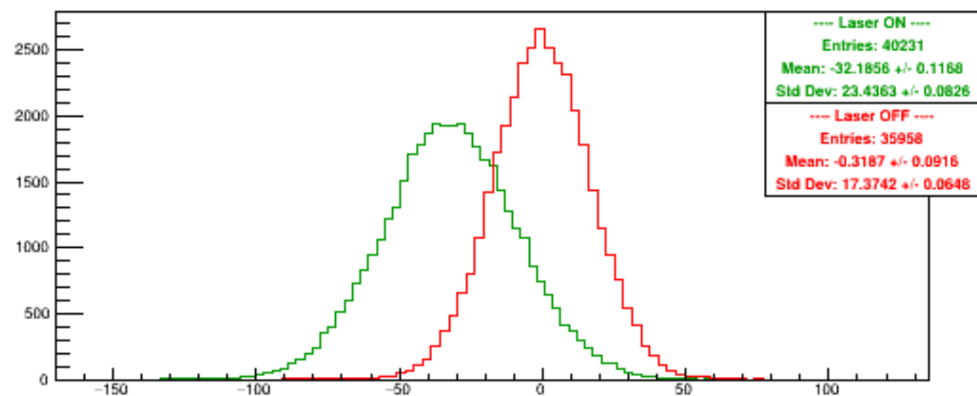
Run 6149 quartetwise, Asyms0
