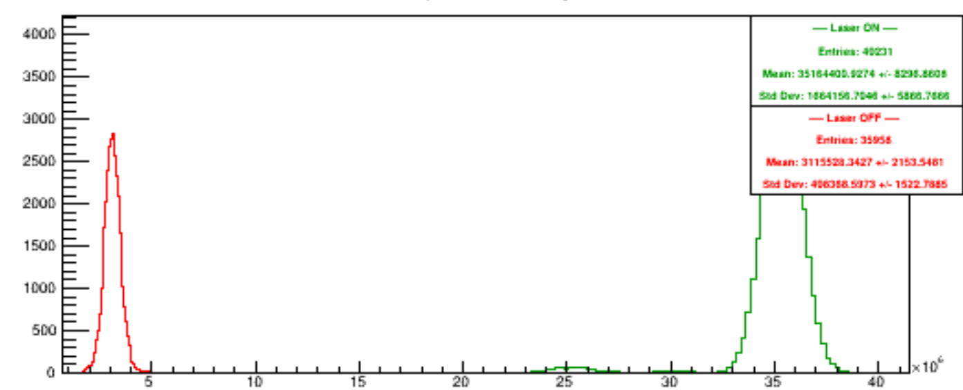
Run 6149 quartetwise, NegHelAcc4
