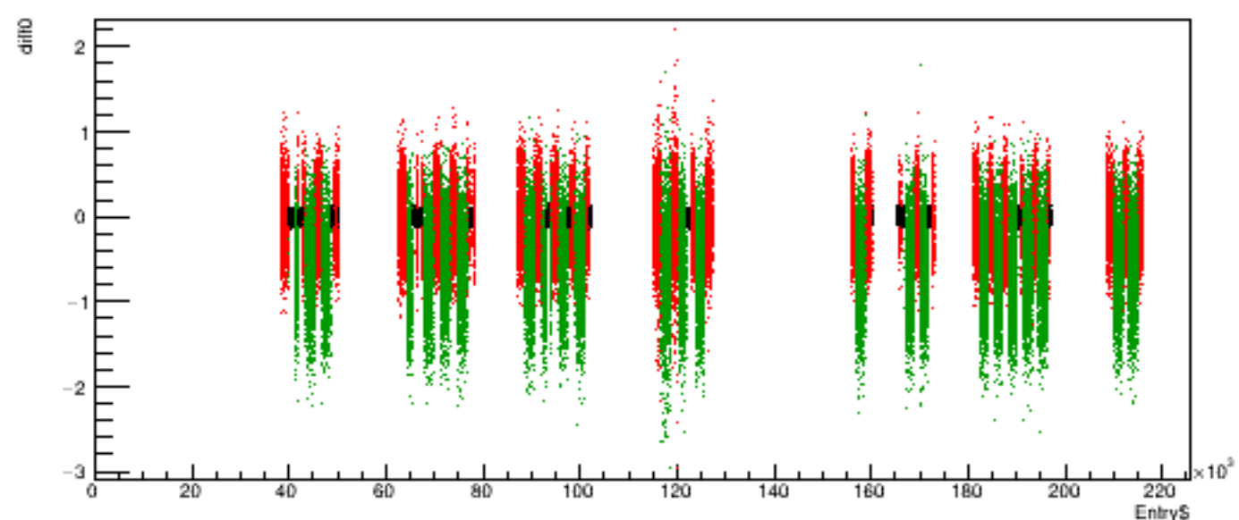
Run 6149 quartetwise, diff0 vs time
