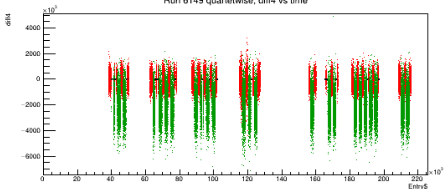
Run 6149 quartetwise, diff4 vs time
