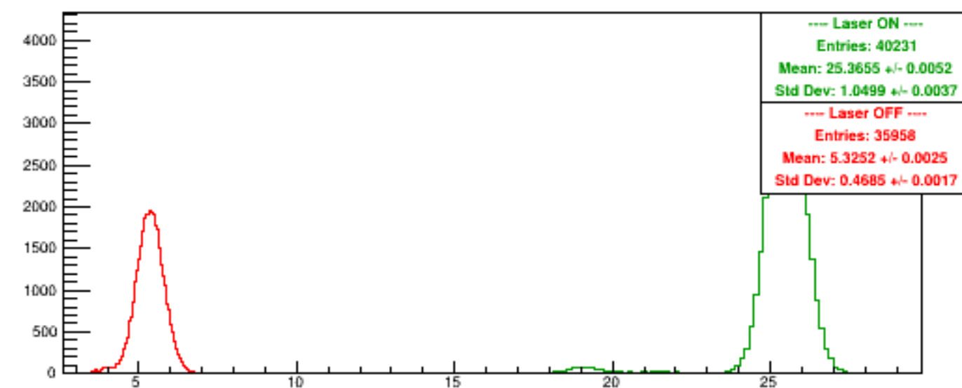
Run 6149 quartetwise, Sums0
