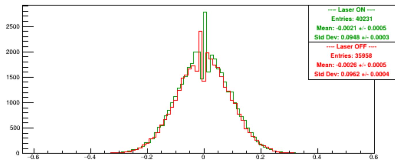
Run 6149 quartetwise, Asyms DSbg1
