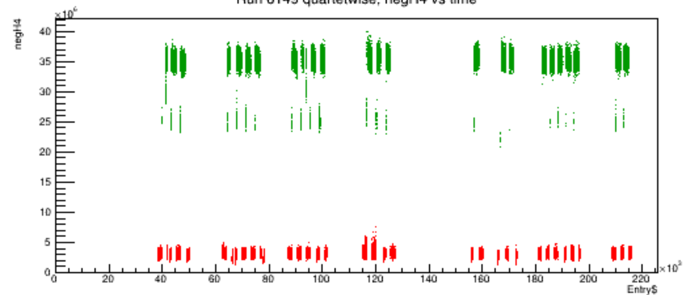
Run 6149 quartetwise, negH4 vs time
