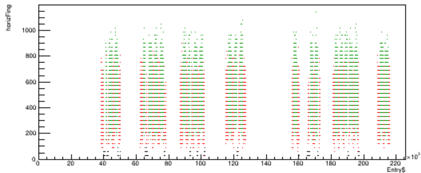
Run 6149 quartetwise, horizFing vs time
