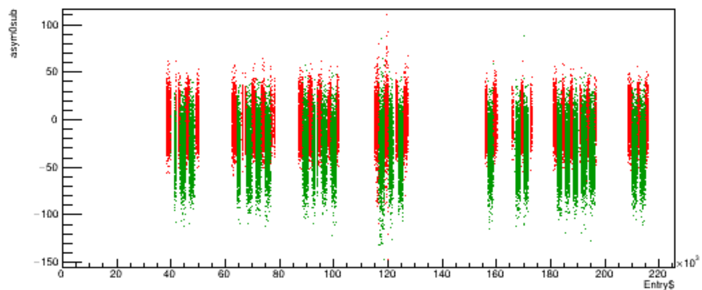
Run 6149 quartetwise, asym0sub vs time
