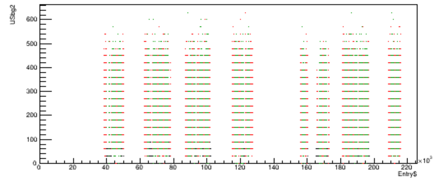
Run 6149 quartetwise, USbg2 vs time
