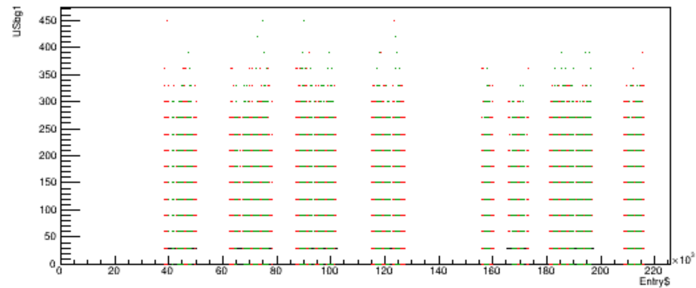
Run 6149 quartetwise, USbg1 vs time
