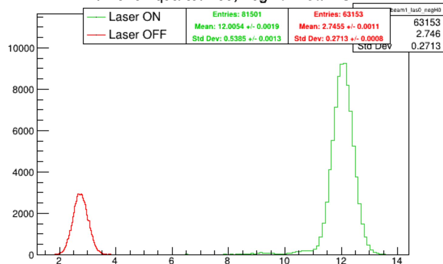
Run 6154 quartetwise, negH0: Beam ON
