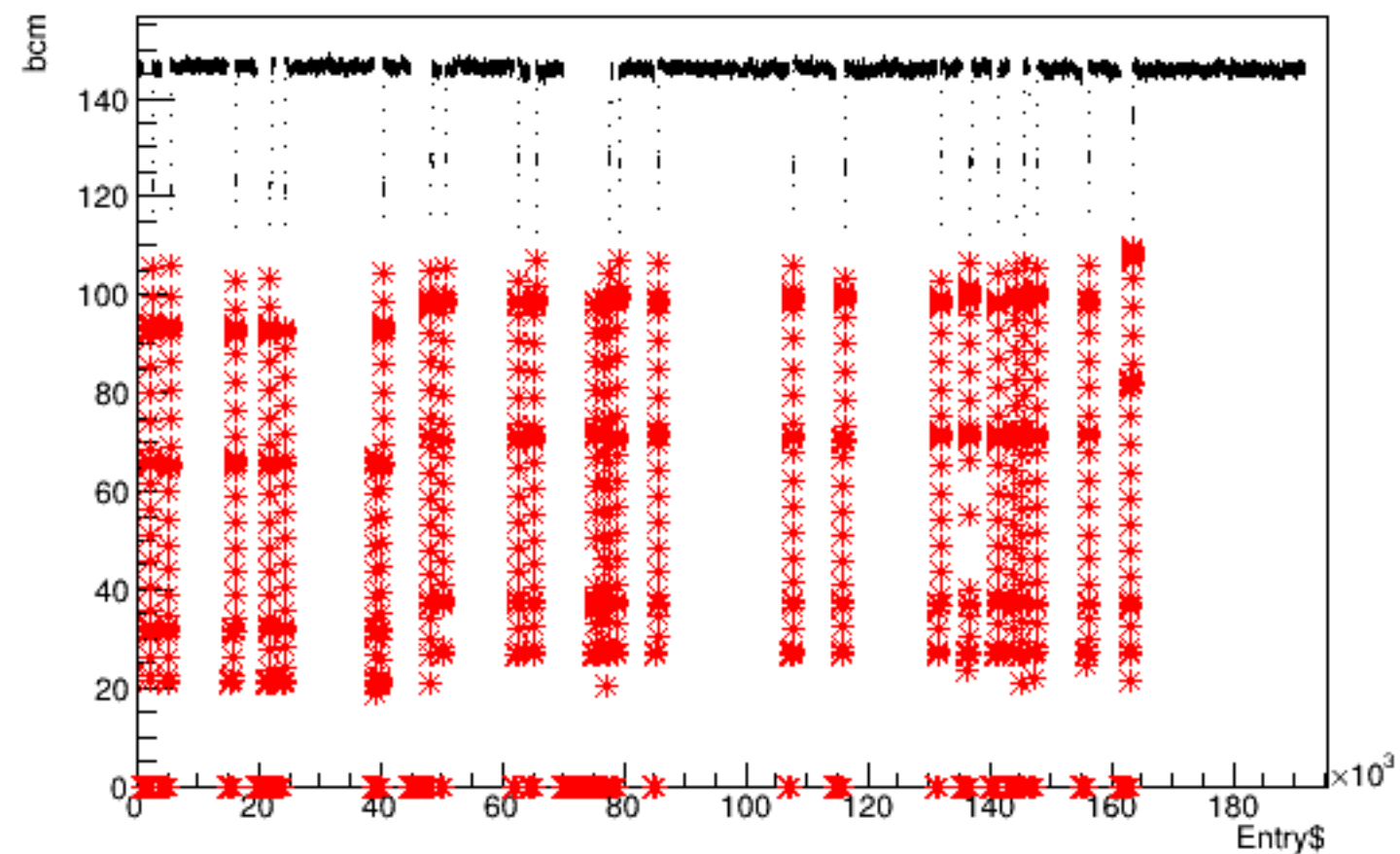
Run 6154 quartetwise, bcm vs time
