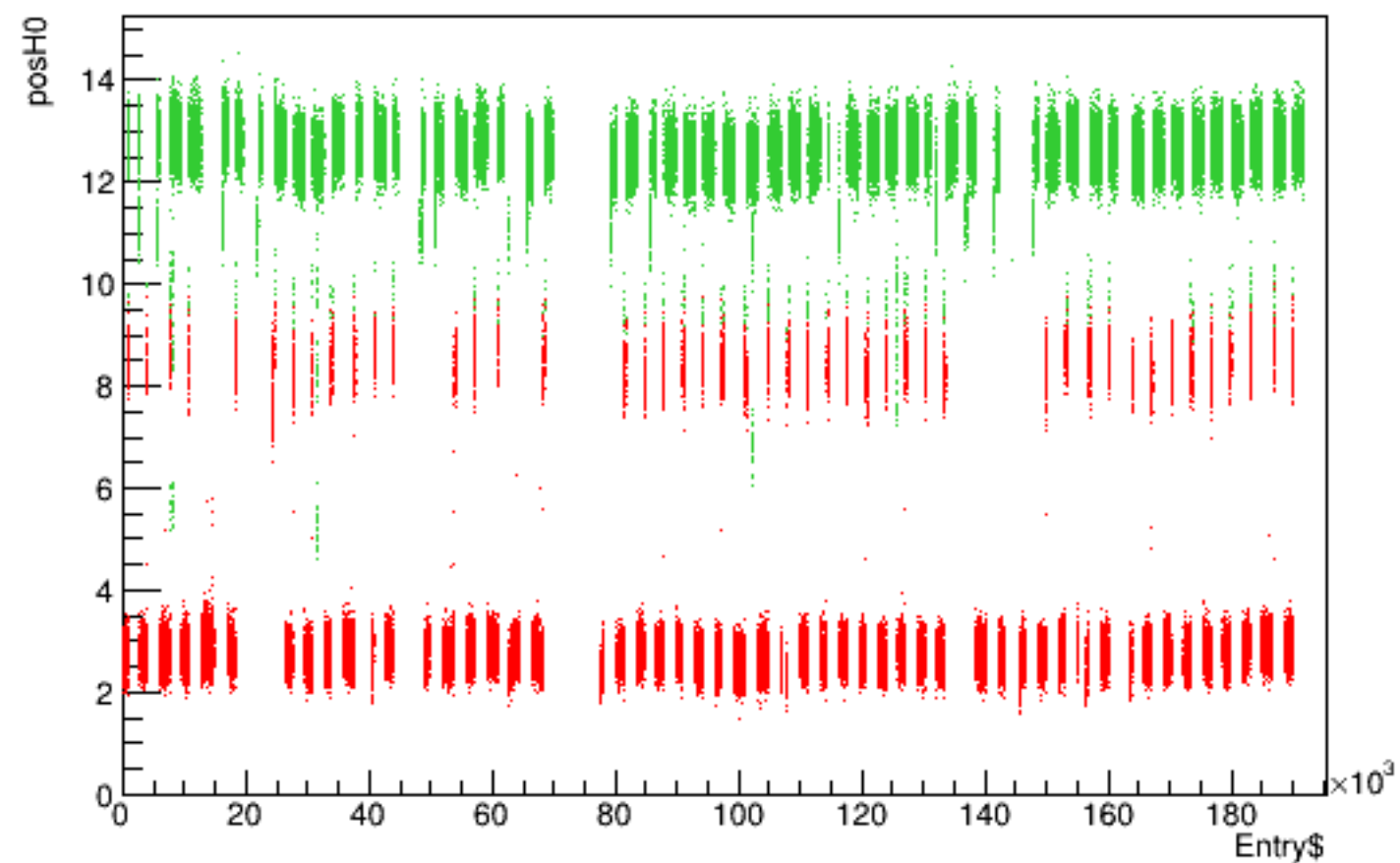
Run 6154 quartetwise, posH0 vs time
