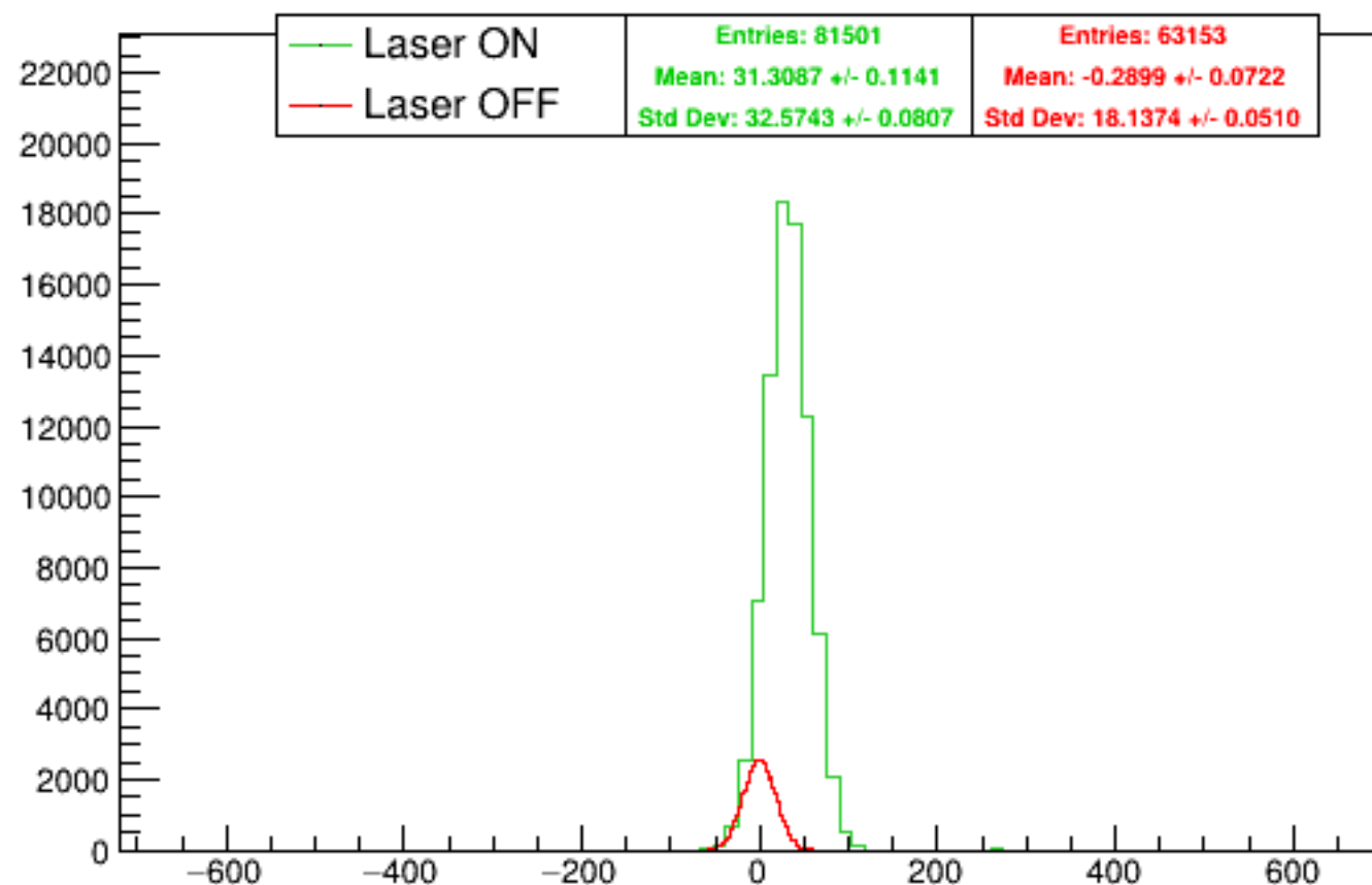
Run 6154 quartetwise, asym0sub: Beam ON
