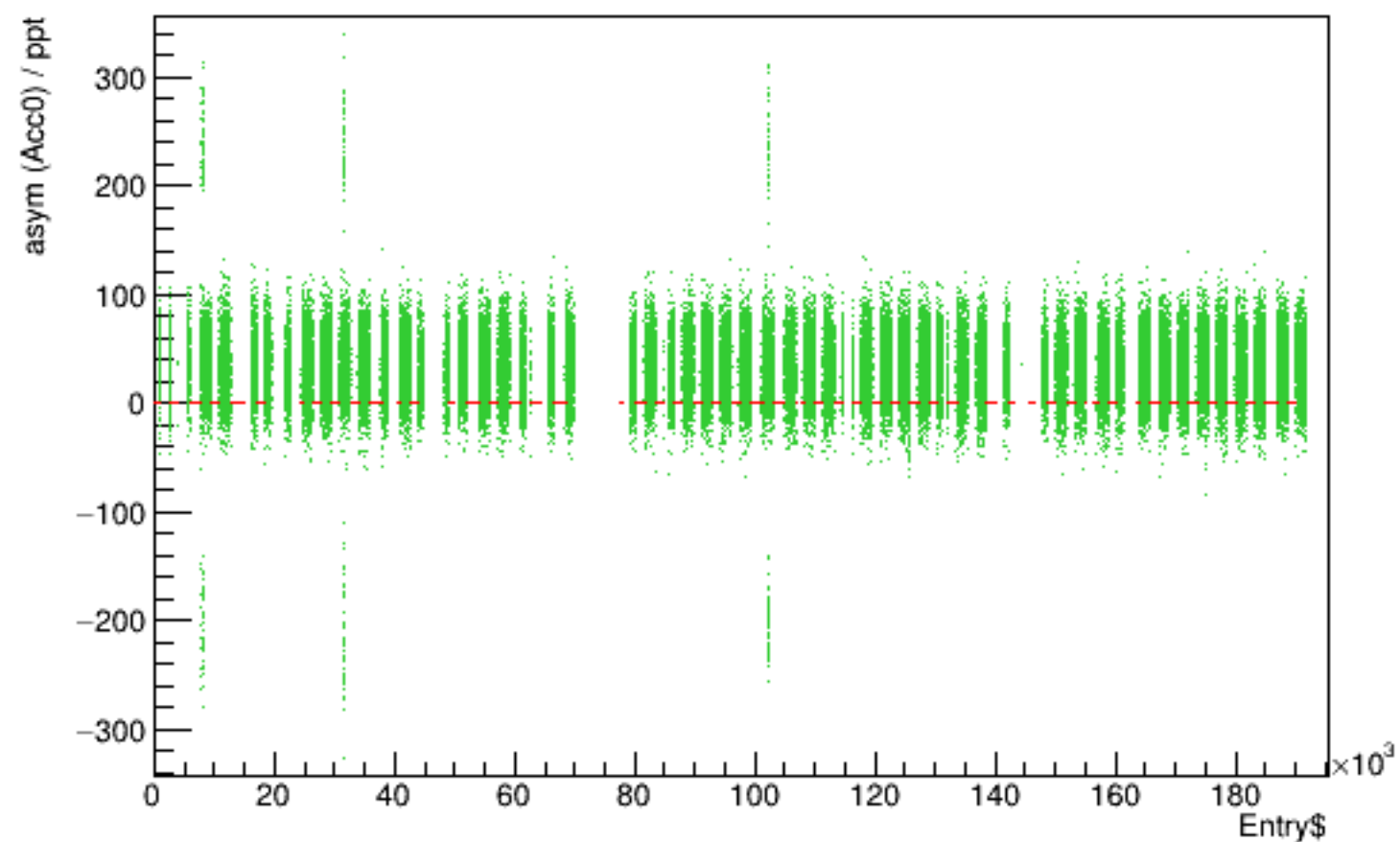
Run 6154 quartetwise, asym0sub vs time
