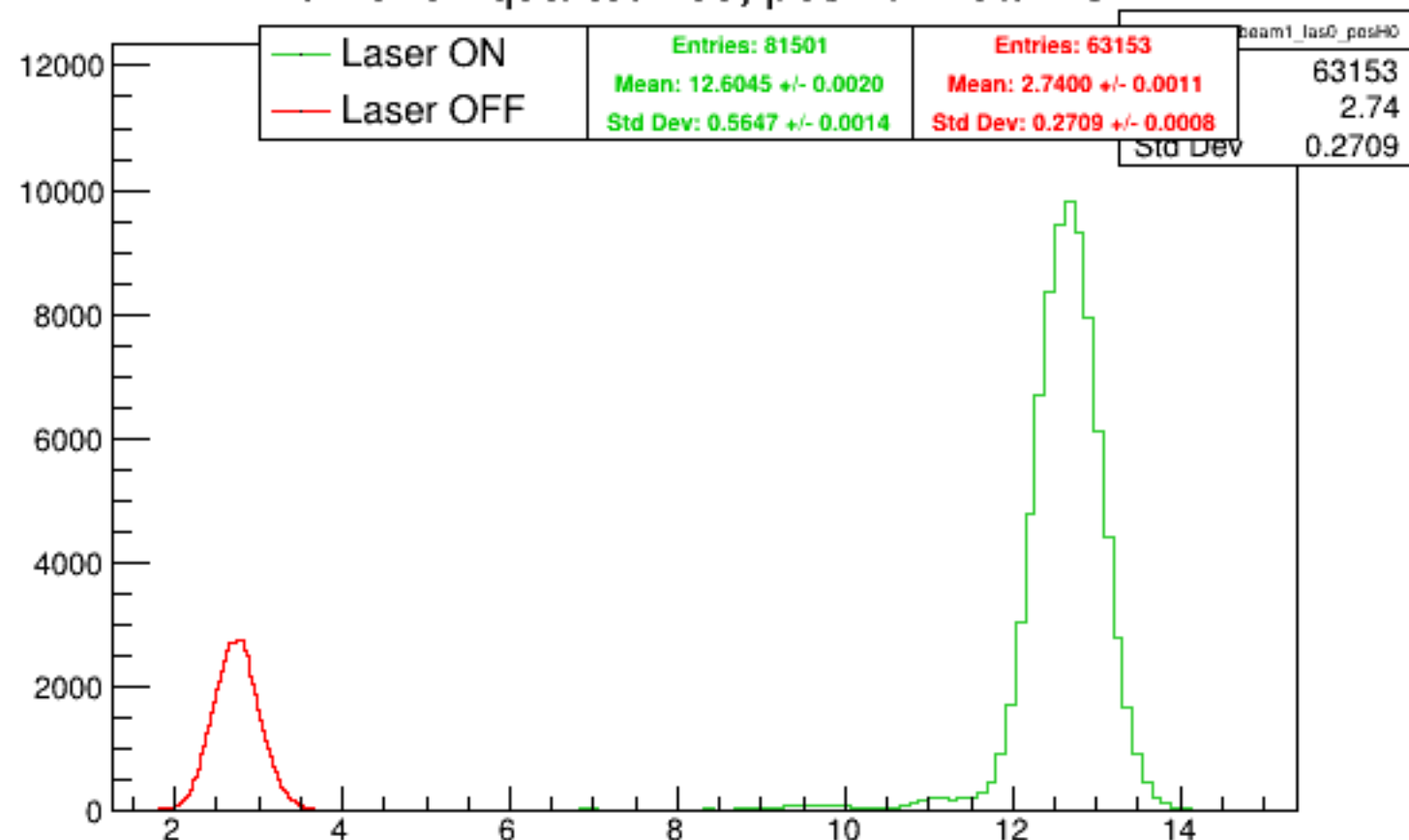
Run 6154 quartetwise, posH0: Beam ON
