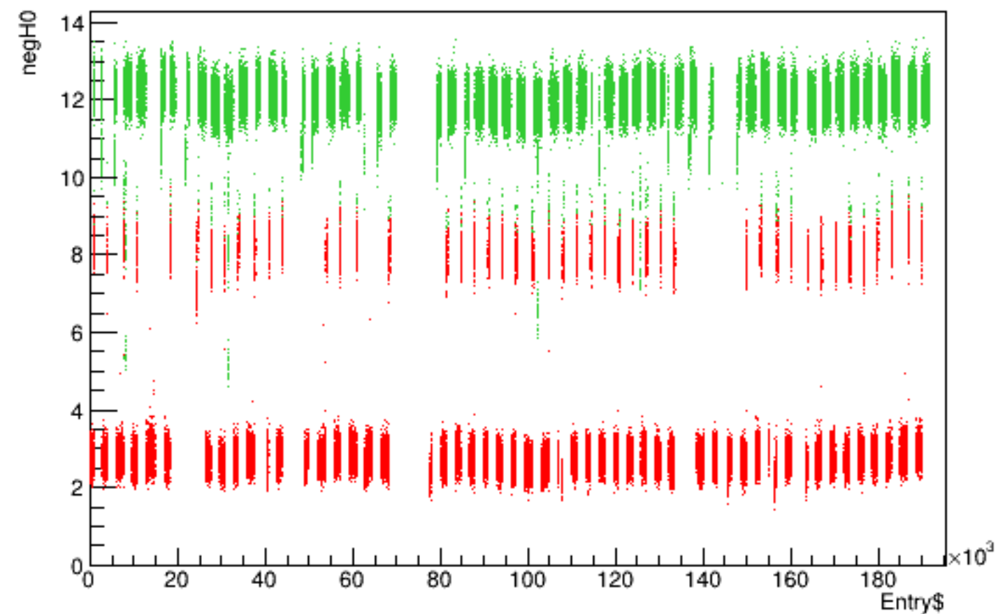
Run 6154 quartetwise, negH0 vs time
