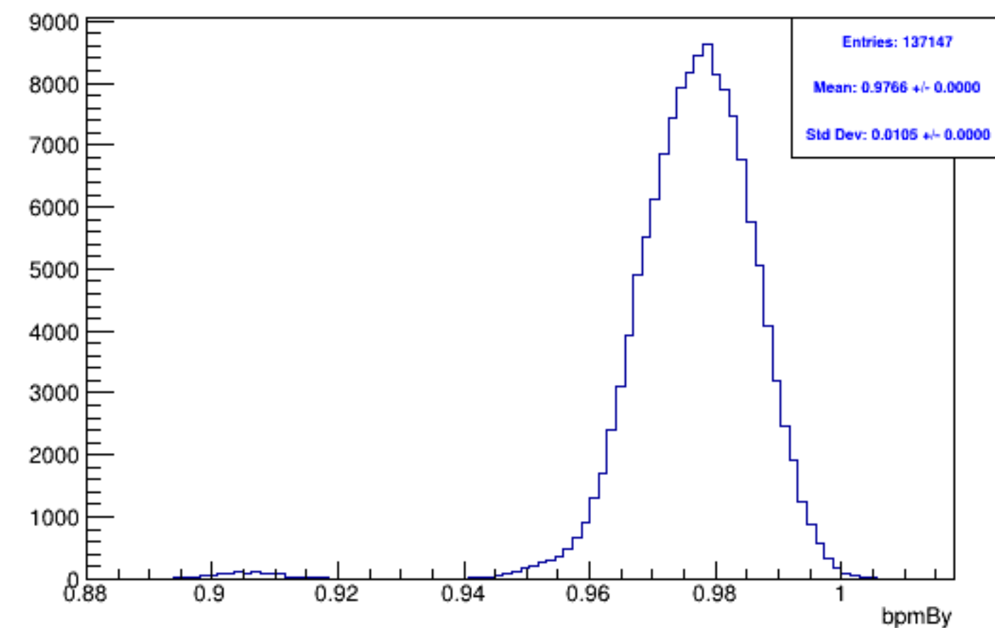
Run 6161, mpswise, bpmBy: Beam ON, Laser OFF
