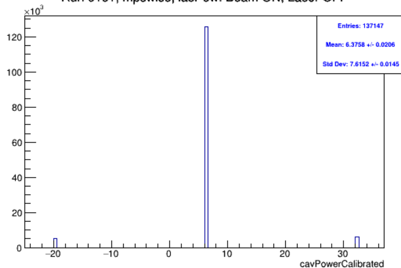
Run 6161, mpwise, lasPow: Beam ON, Laser OFF
