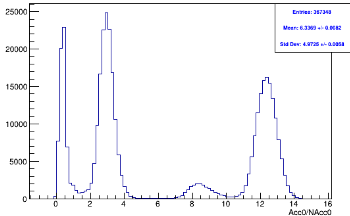
Run 6161 mpwise, acc0: All
