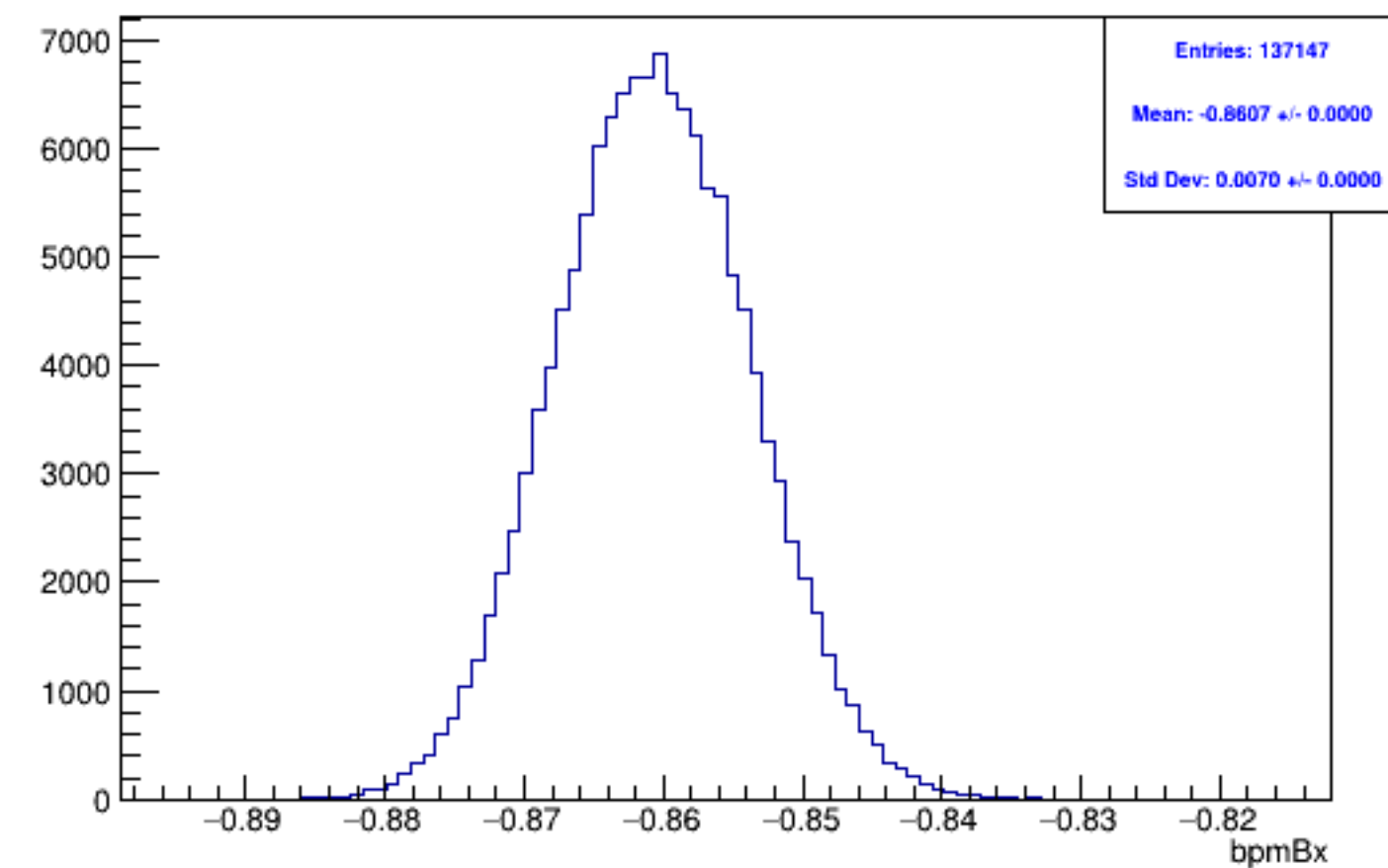
Run 6161, mpswise, bpmBx: Beam ON, Laser OFF
