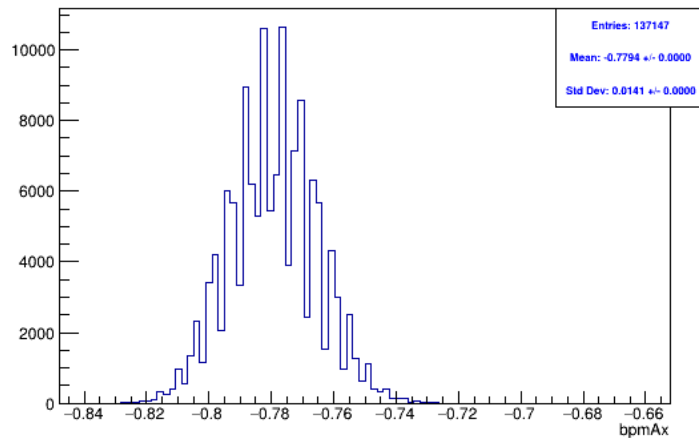
Run 6161, mpwise, bpmAx: Beam ON, Laser OFF
