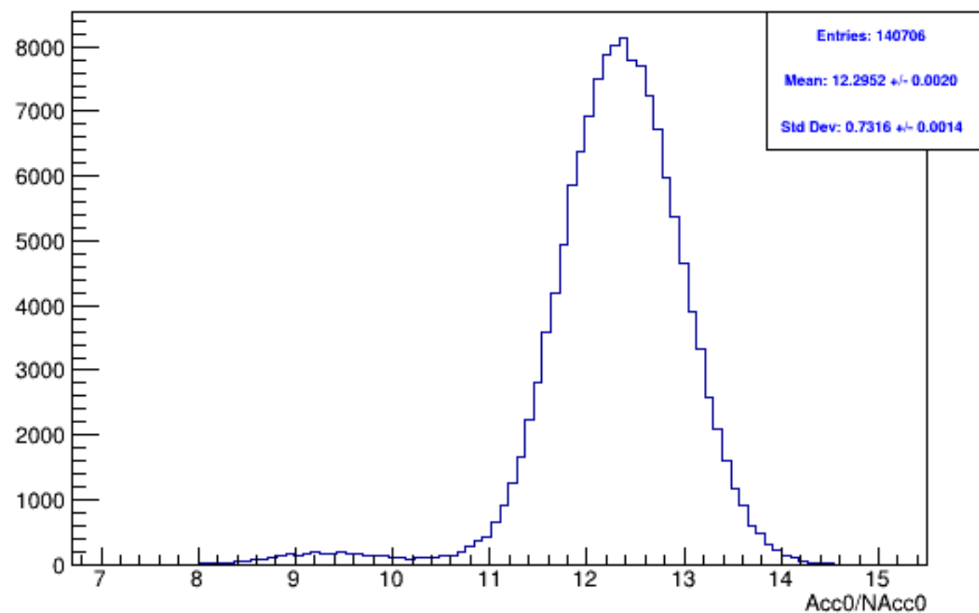
Run 6161, mpwise, acc0: Beam ON, Laser ON
