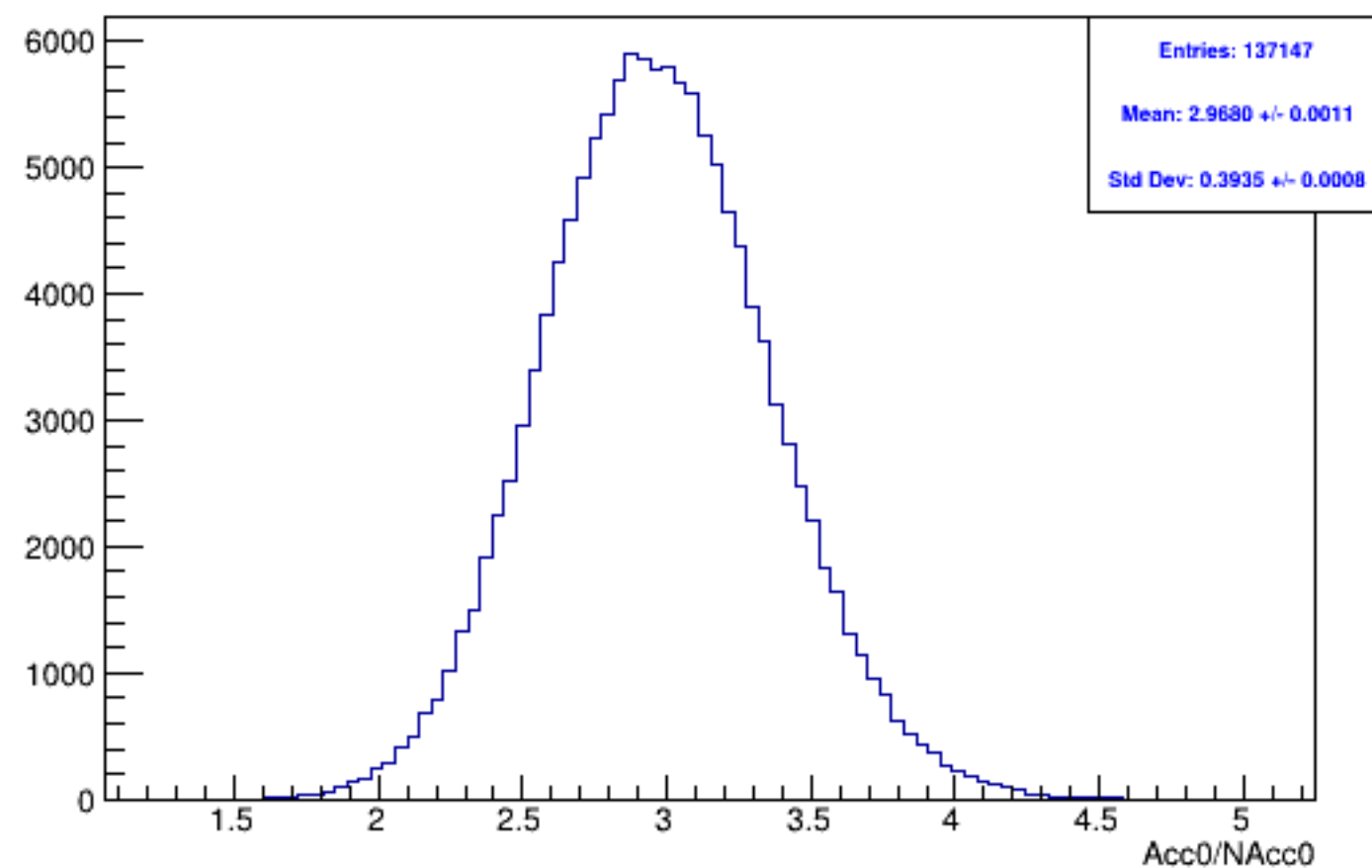
Run 6161, mpwise, acc0: Beam ON, Laser OFF
