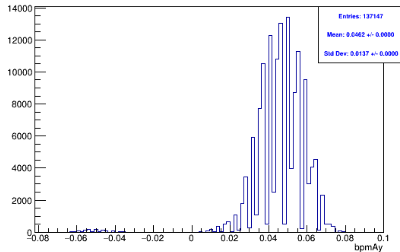
Run 6161, mpwise, bpmAy: Beam ON, Laser OFF
