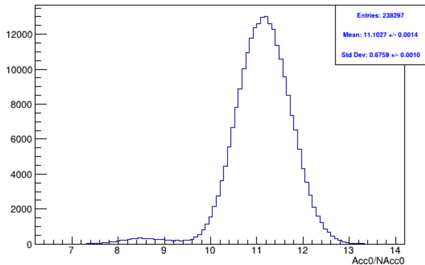
Run 6167, mpwise, acc0: Beam ON, Laser ON
