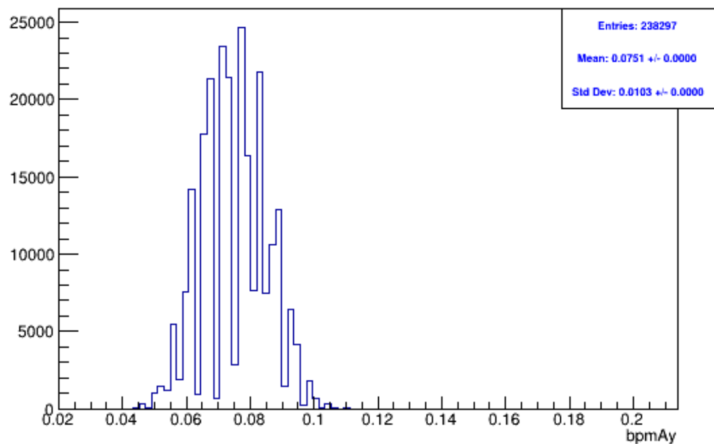
Run 6167, mpwise, bpmAy: Beam ON, Laser ON
