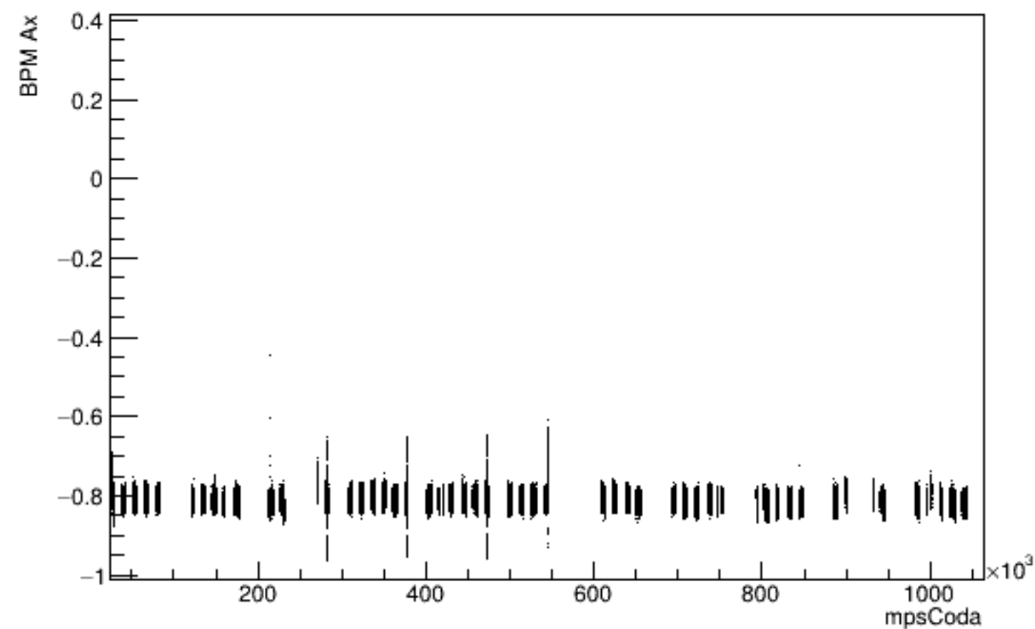
Run 6167 mpwise, beam ON, laser OFF
