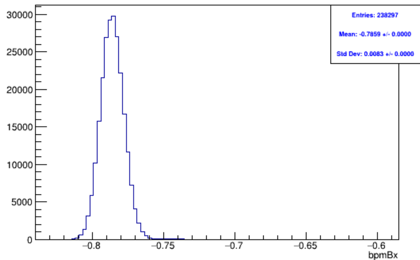
Run 6167, mpswise, bpmBx: Beam ON, Laser ON
