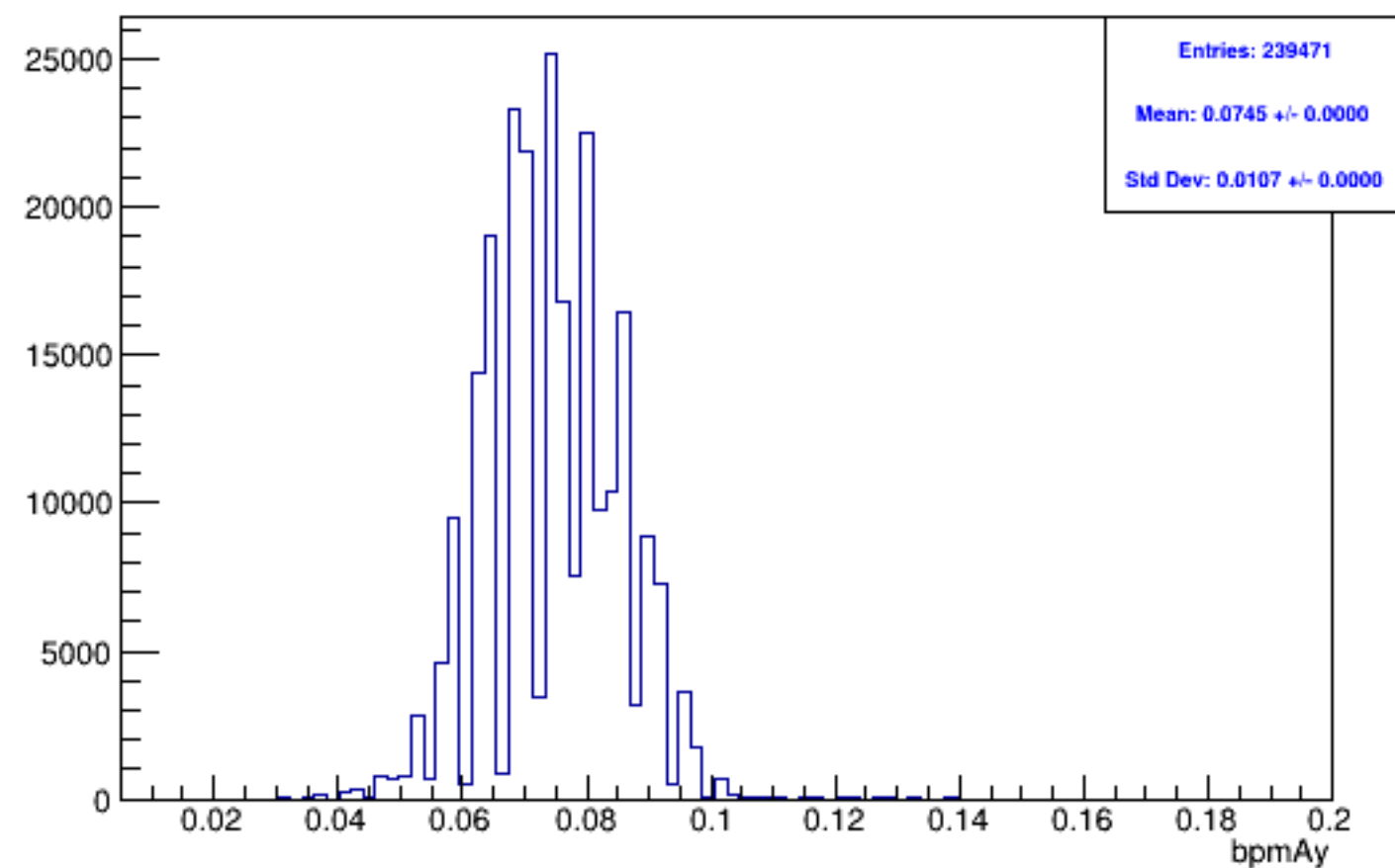
Run 6167, mpwise, bpmAy: Beam ON, Laser OFF
