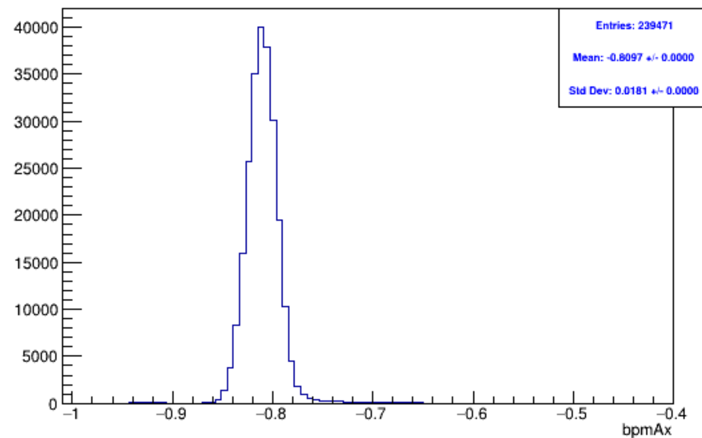
Run 6167, mpwise, bpmAx: Beam ON, Laser OFF
