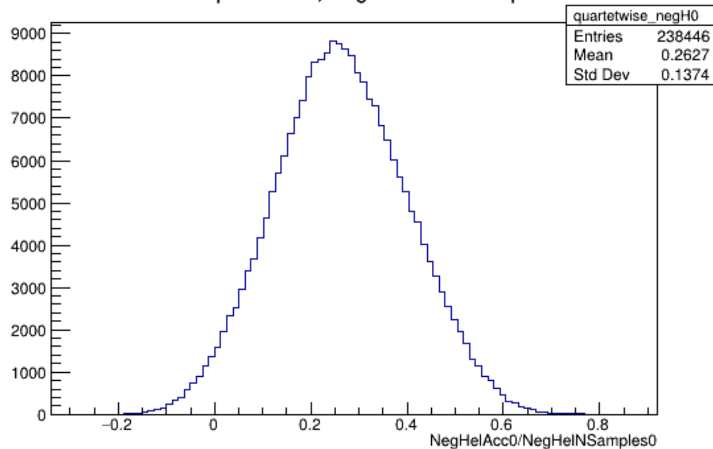
Run 6168 quartetwise, NegHelAcc0/NSamples0: All
