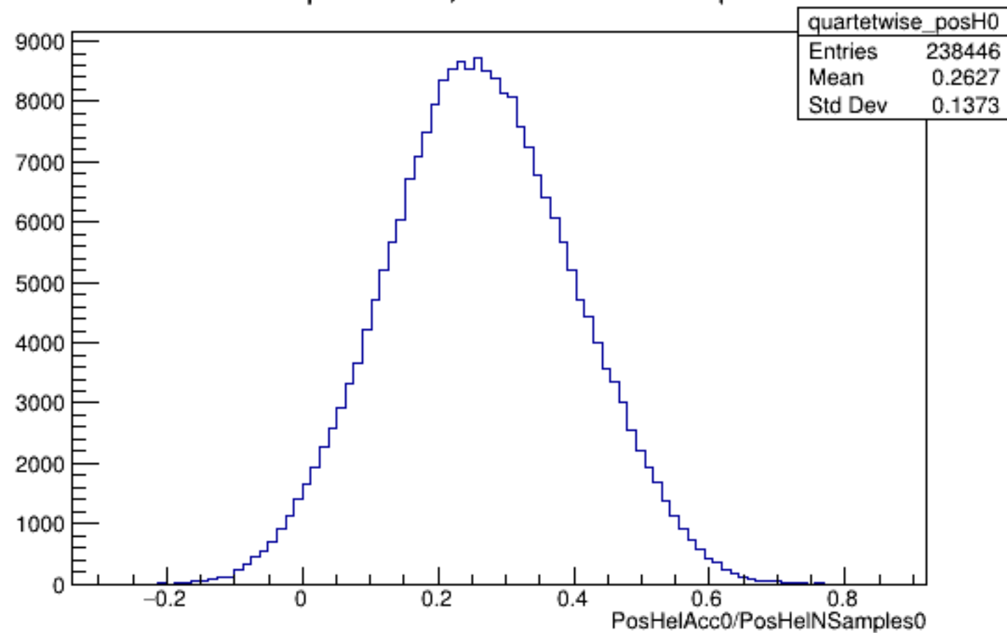
Run 6168 quartetwise, PosHelAcc0/NSamples0: All
