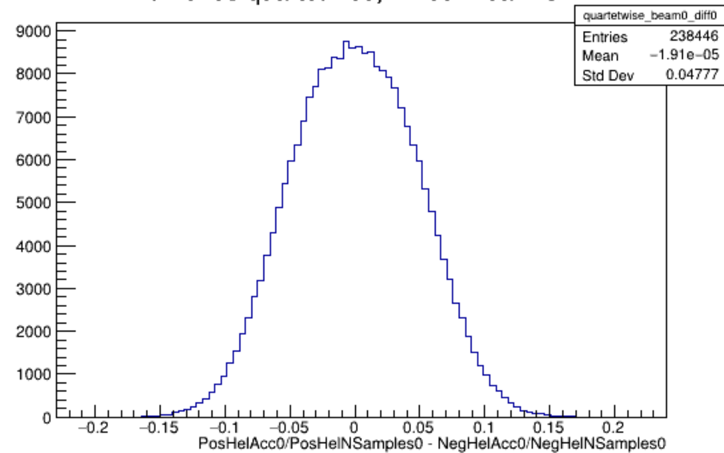
Run 6168 quartetwise, Diffs0: Beam OFF
