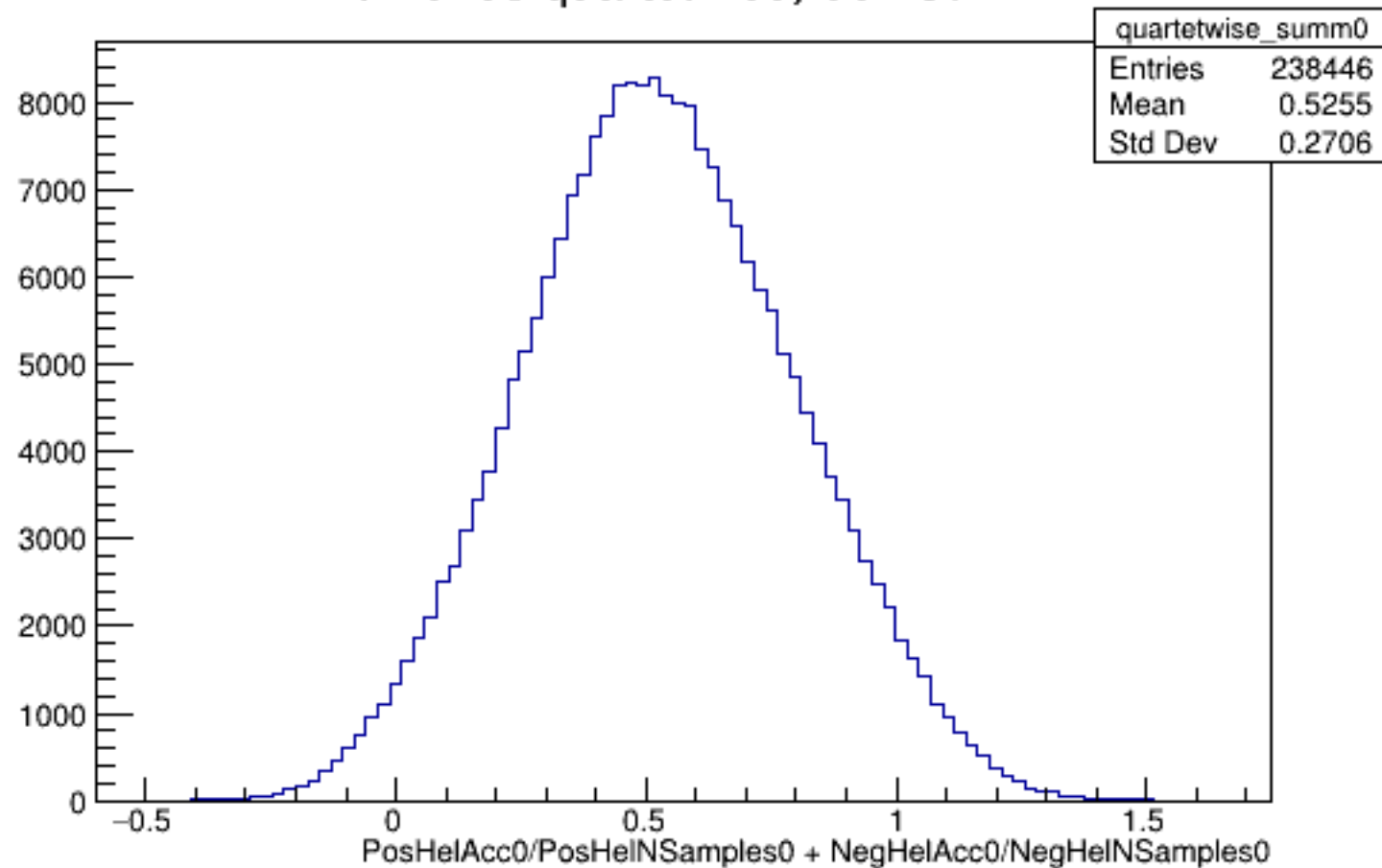
Run 6168 quartetwise, Sums0: All
