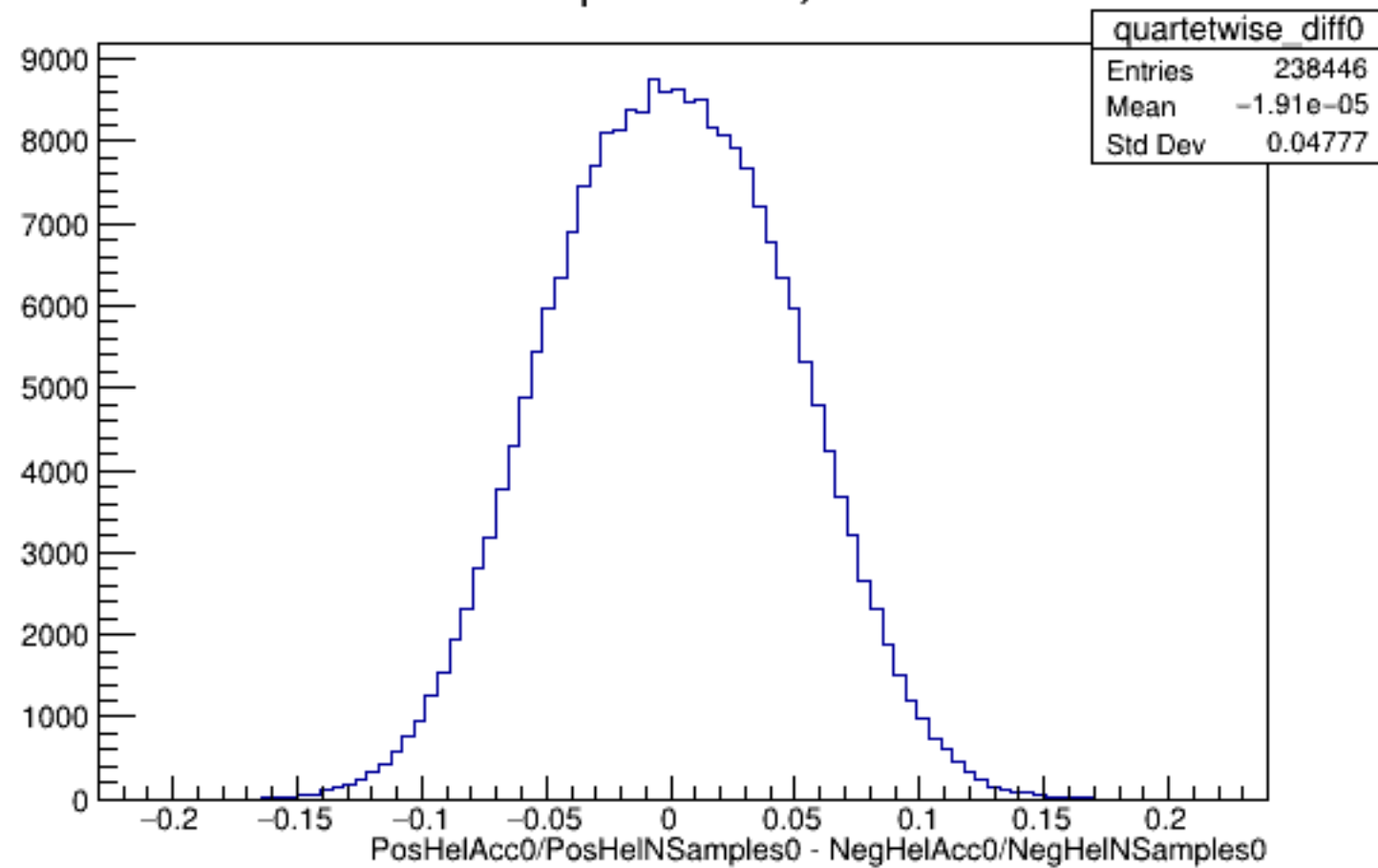
Run 6168 quartetwise, Diffs0: All
