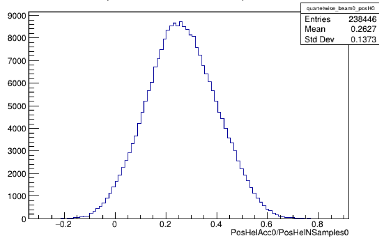
Run 6168 quartetwise, PosHelAcc0/NSamples0: Beam OFF
