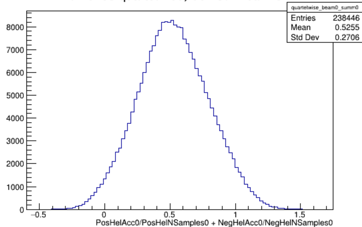
Run 6168 quartetwise, Sums0: Beam OFF
