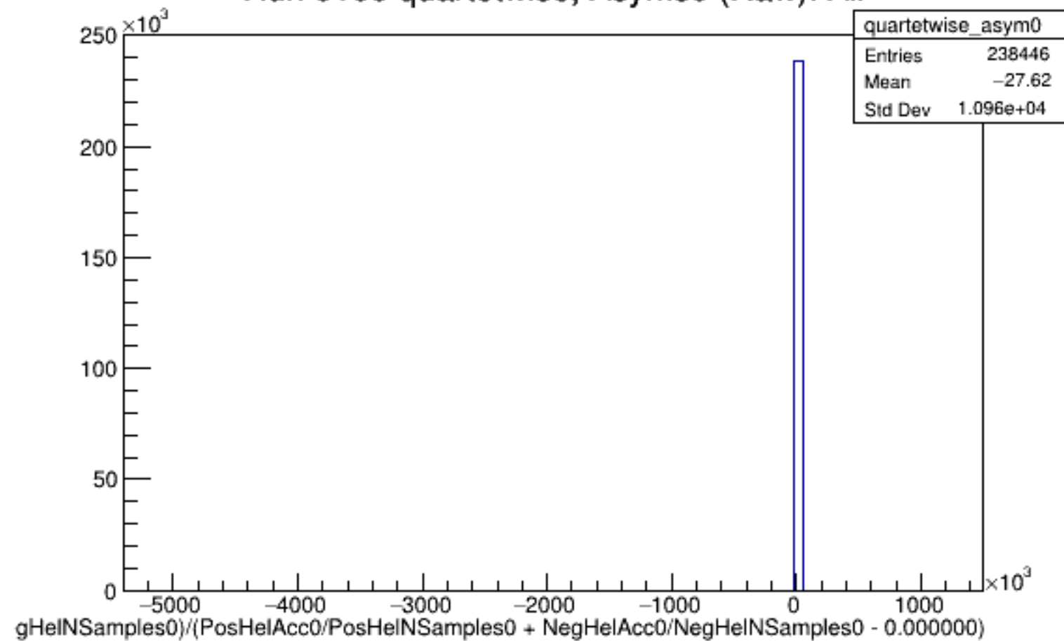
Run 6168 quartetwise, Asyms0 (Raw): All
