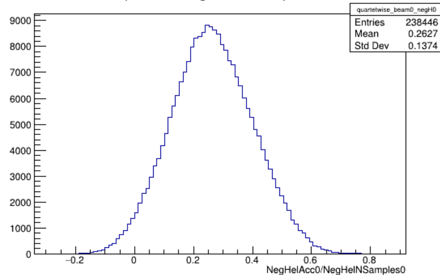
Run 6168 quartetwise, NegHelAcc0/NSamples0: Beam OFF
