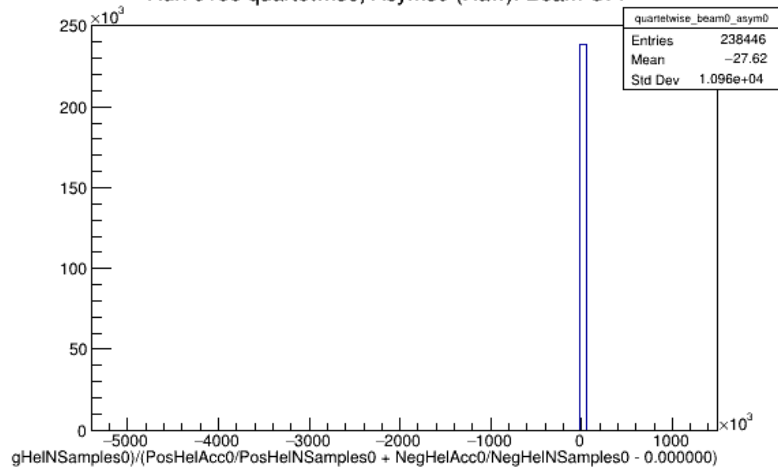
Run 6168 quartetwise, Asyms0 (Raw): Beam OFF
