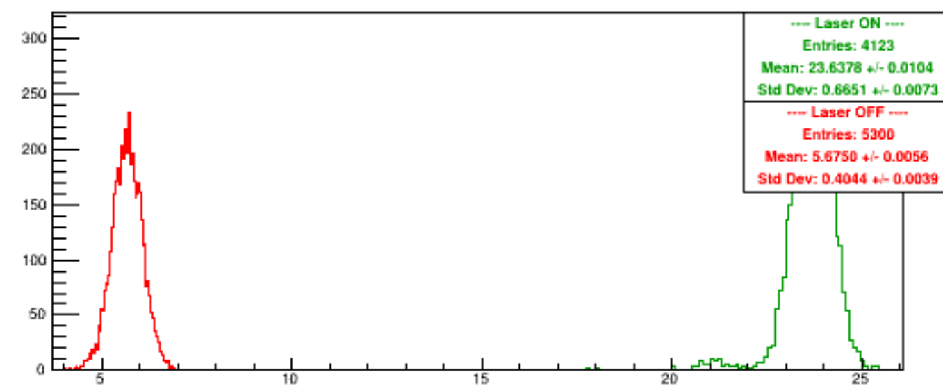
Run 6171 quartetwise, Sums0
