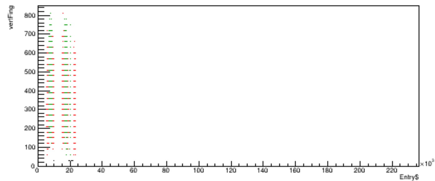
Run 6171 quartetwise, vertFing vs time
