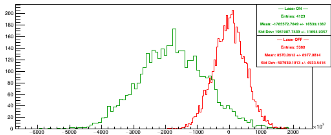
Run 6171 quartetwise, Diffs4
