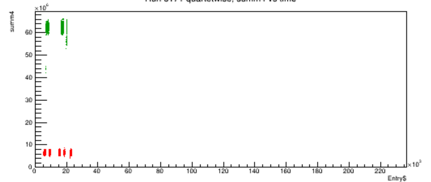
Run 6171 quartetwise, summ4 vs time
