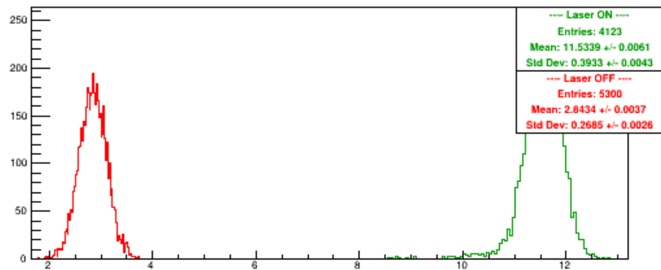
Run 6171 quartetwise, PosHelAcc0/NSamples0
