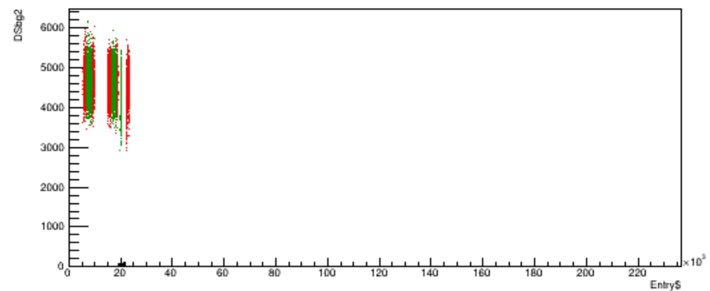
Run 6171 quartetwise, DSbg2 vs time
