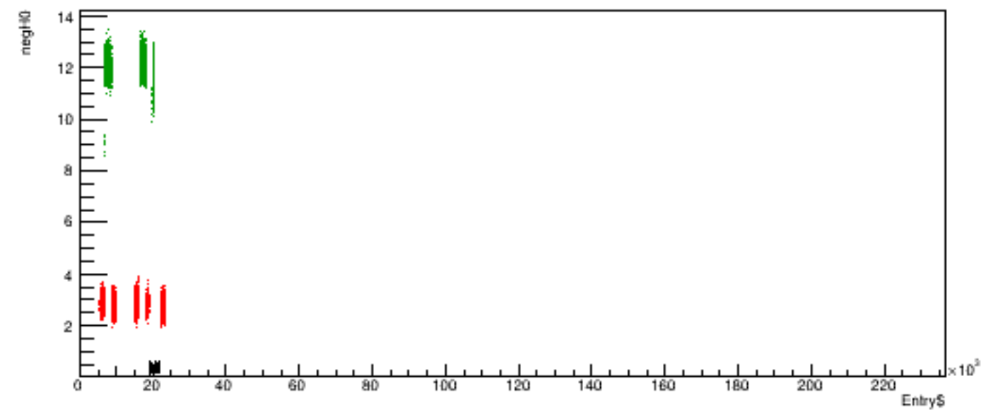
Run 6171 quartetwise, negH0 vs time
