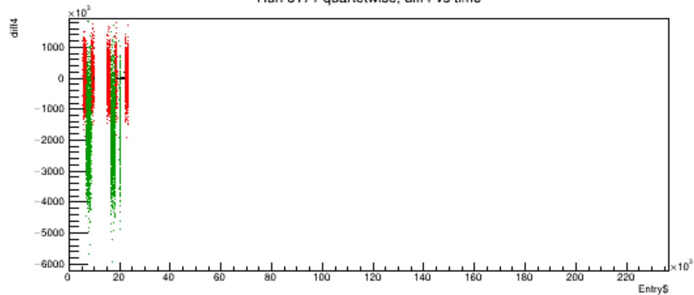
Run 6171 quartetwise, diff4 vs time
