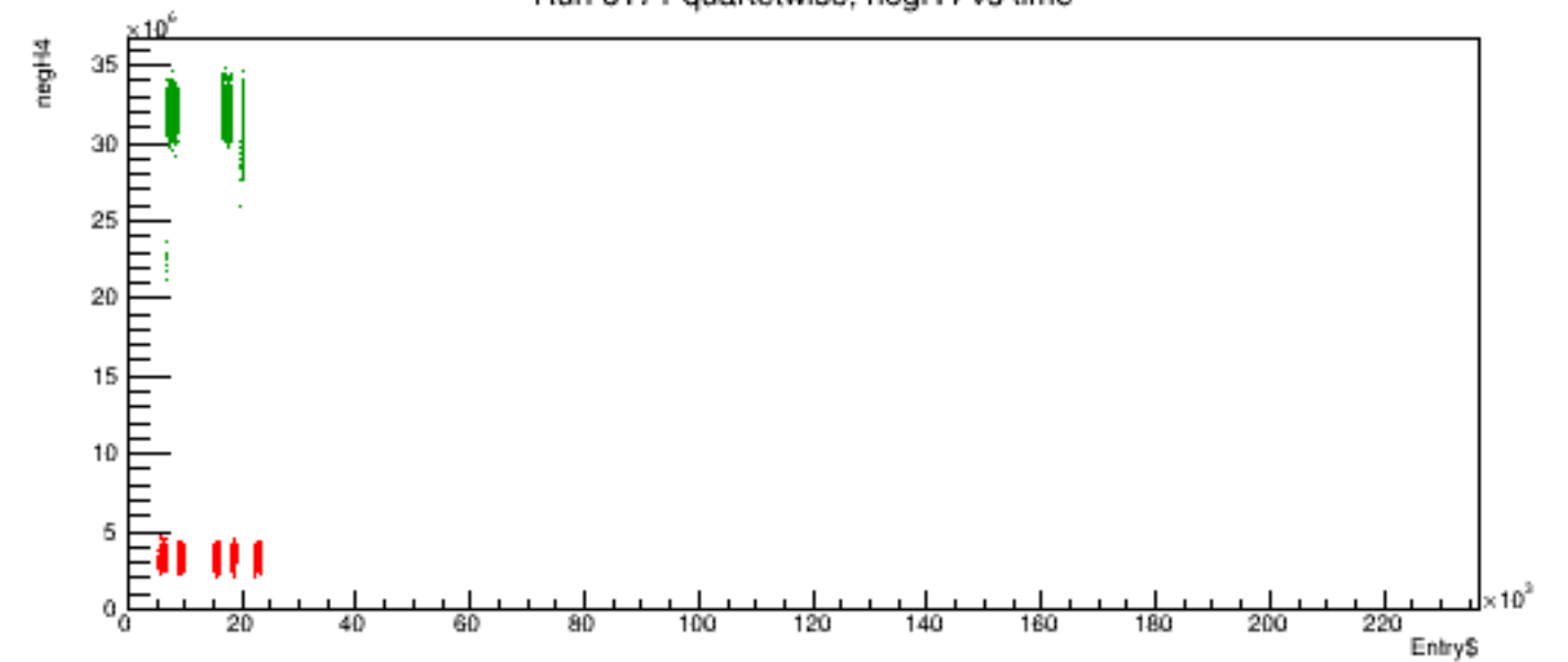
Run 6171 quartetwise, negH4 vs time
