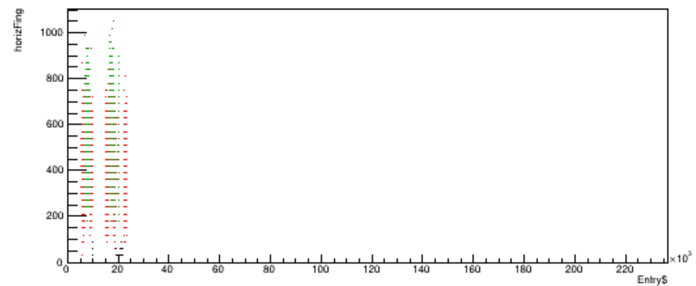
Run 6171 quartetwise, horizFing vs time
