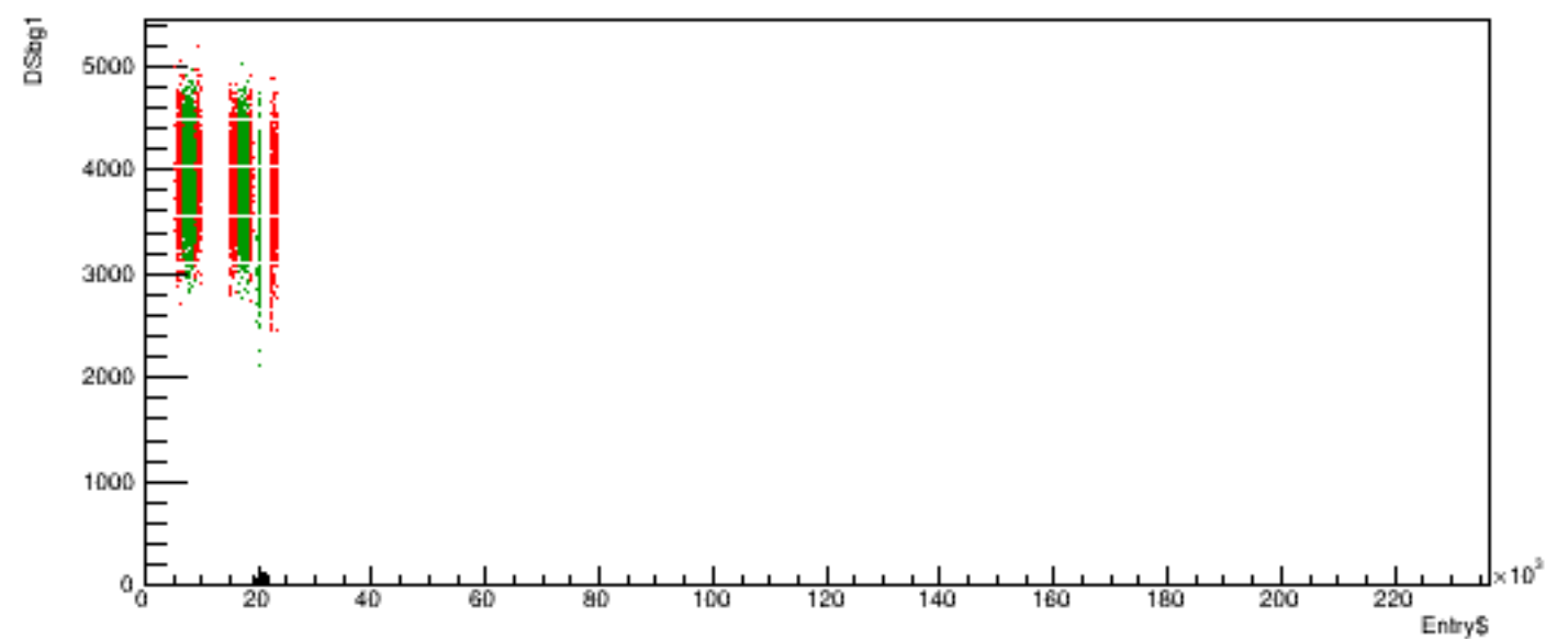
Run 6171 quartetwise, DSbg1 vs time
