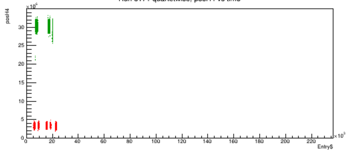
Run 6171 quartetwise, posH4 vs time
