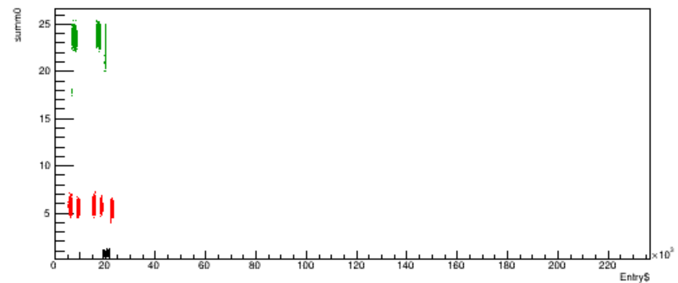
Run 6171 quartetwise, summ0 vs time
