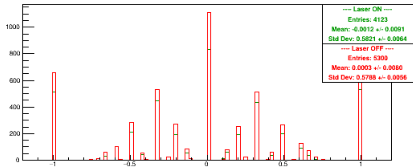
Run 6171 quartetwise, Asyms USbg1
