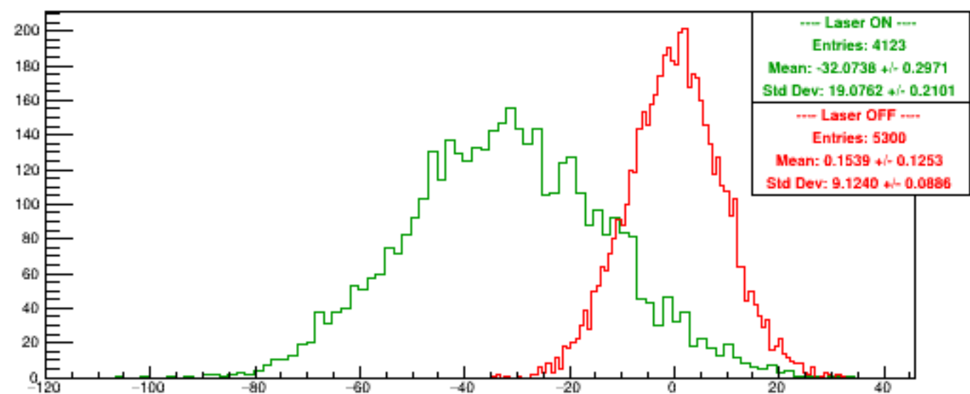
Run 6171 quartetwise, Asyms4
