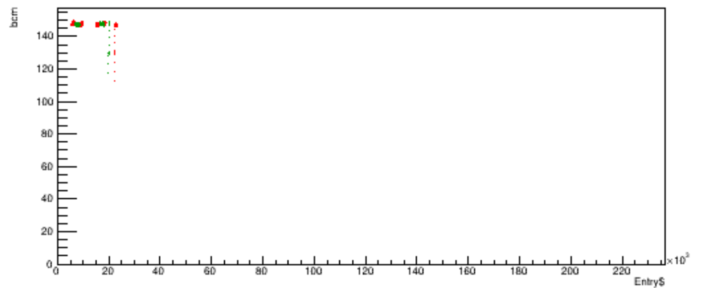
Run 6171 quartetwise, posH4 vs time
