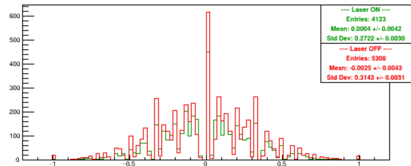
Run 6171 quartetwise, Asyms Horiz Finger
