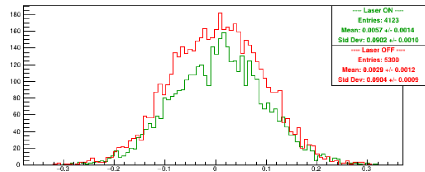
Run 6171 quartetwise, Asyms DSbg1
