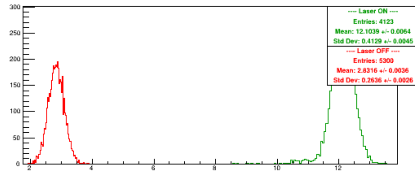
Run 6171 quartetwise, NegHelAcc0/NSamples0
