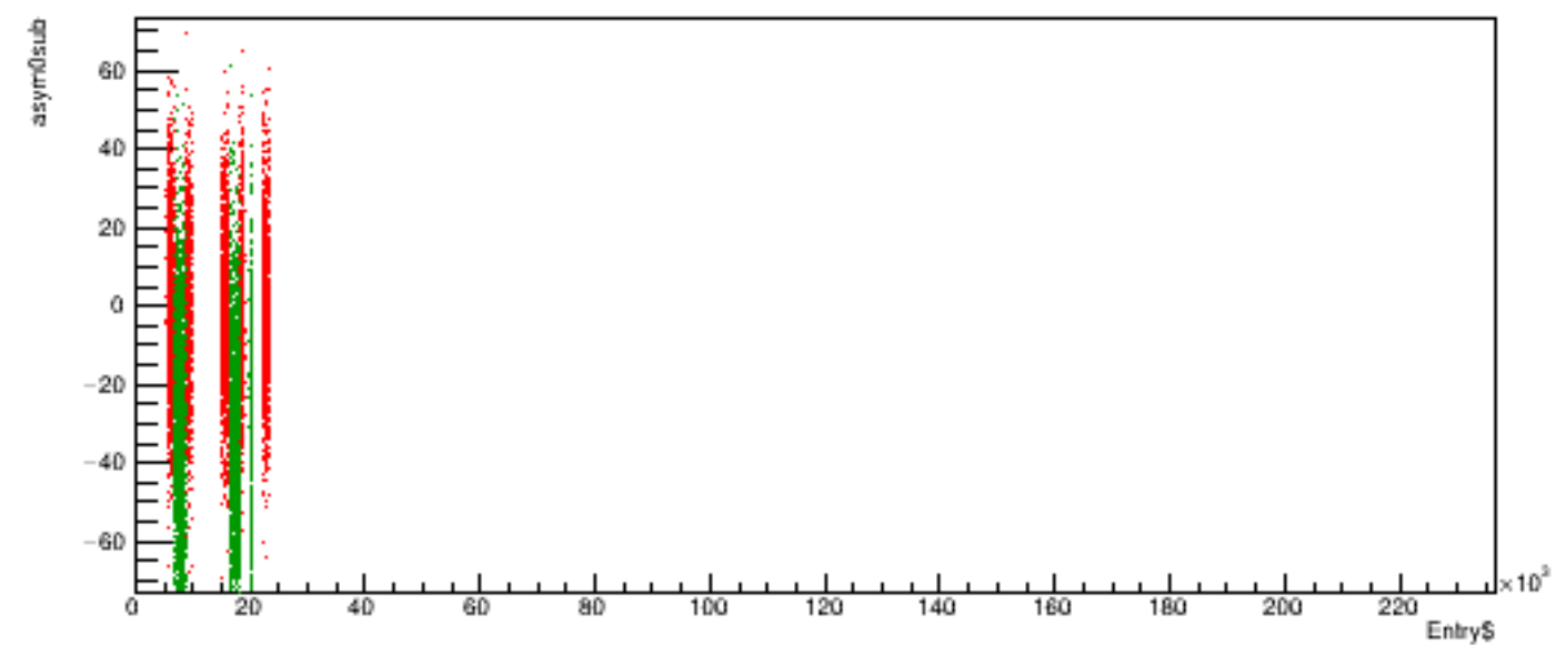
Run 6171 quartetwise, asym0sub vs time
