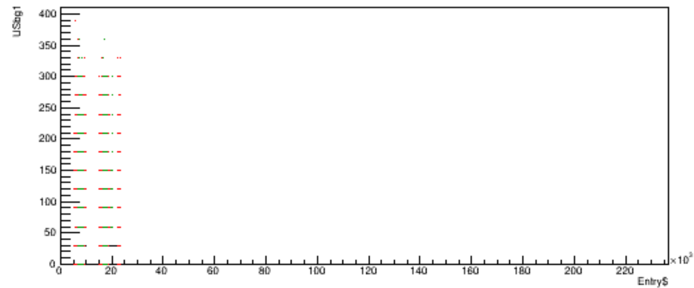
Run 6171 quartetwise, USbg1 vs time
