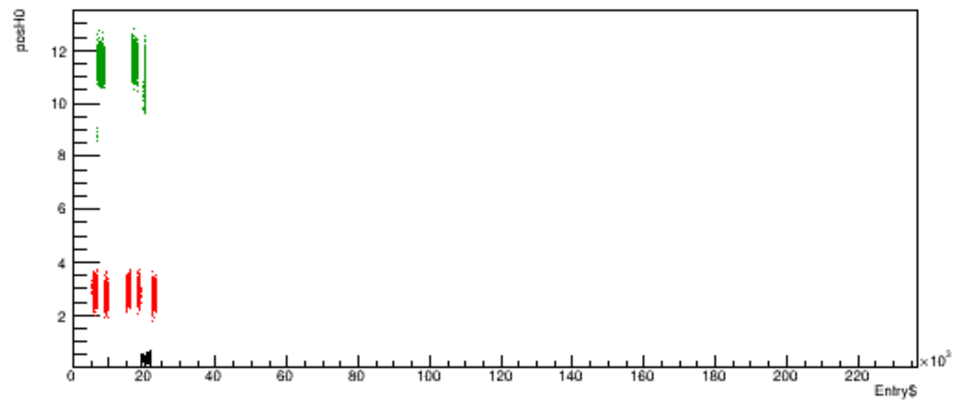
Run 6171 quartetwise, posH0 vs time
