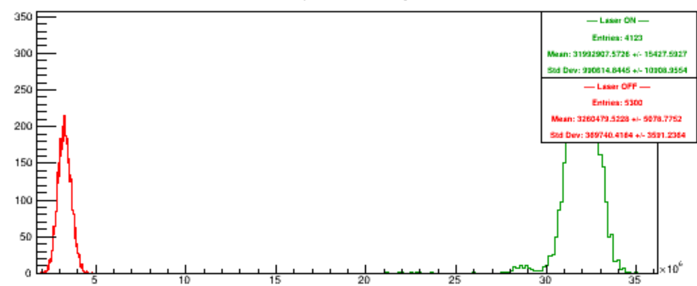
Run 6171 quartetwise, NegHelAcc4
