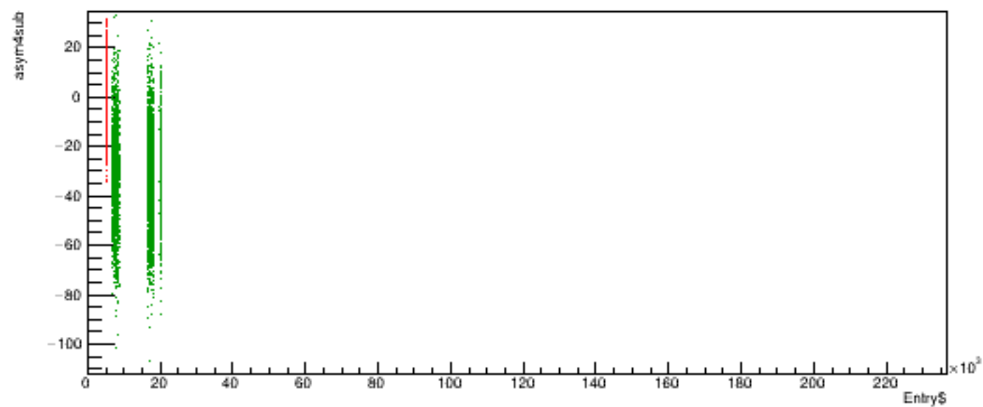
Run 6171 quartetwise, asym4sub vs time
