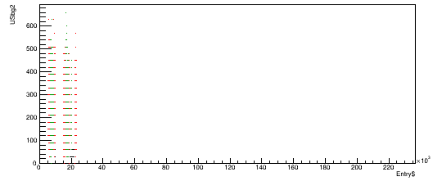
Run 6171 quartetwise, USbg2 vs time
