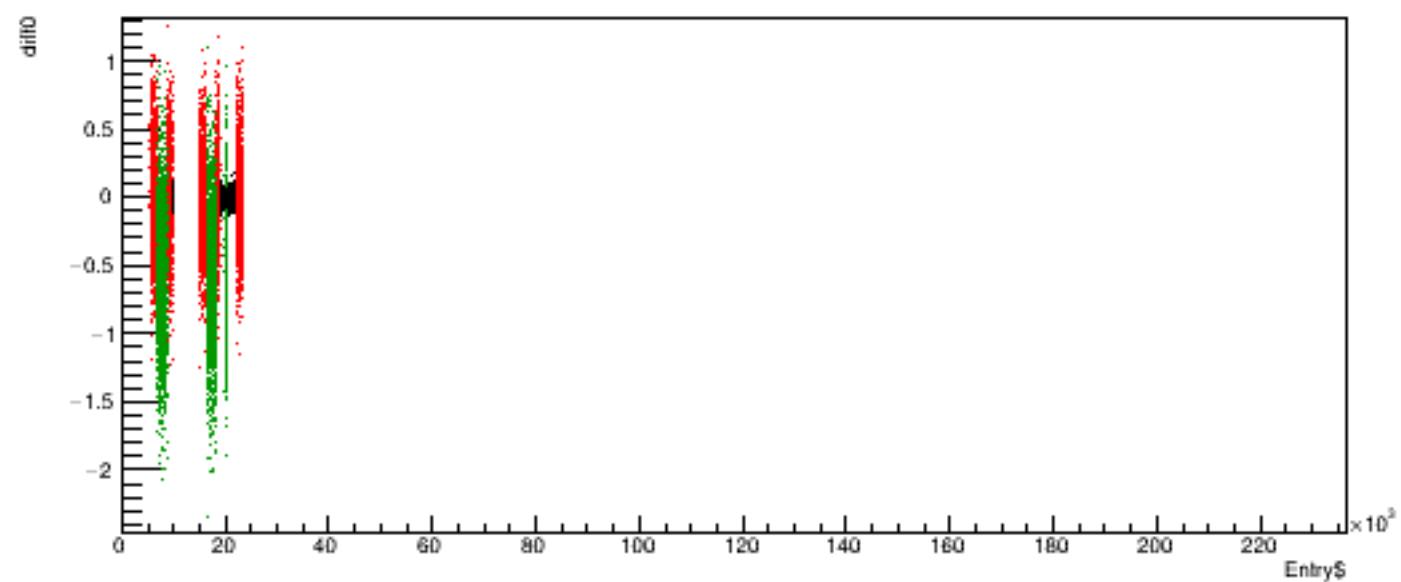
Run 6171 quartetwise, diff0 vs time
