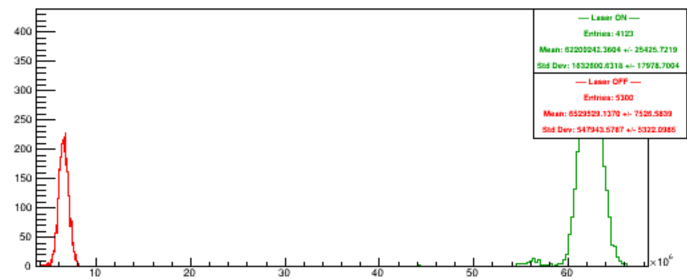
Run 6171 quartetwise, Sums4
