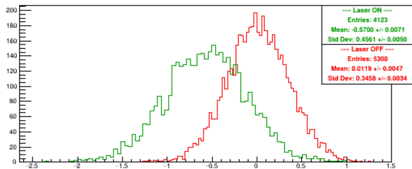
Run 6171 quartetwise, Diffs0
