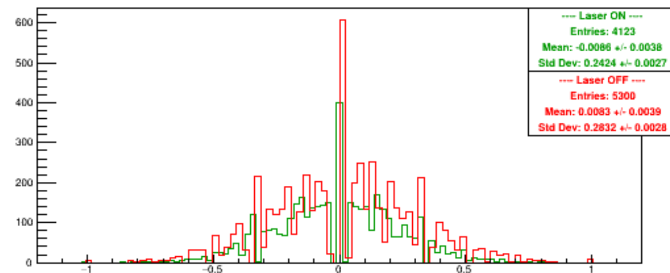
Run 6171 quartetwise, Asyms Vert Finger
