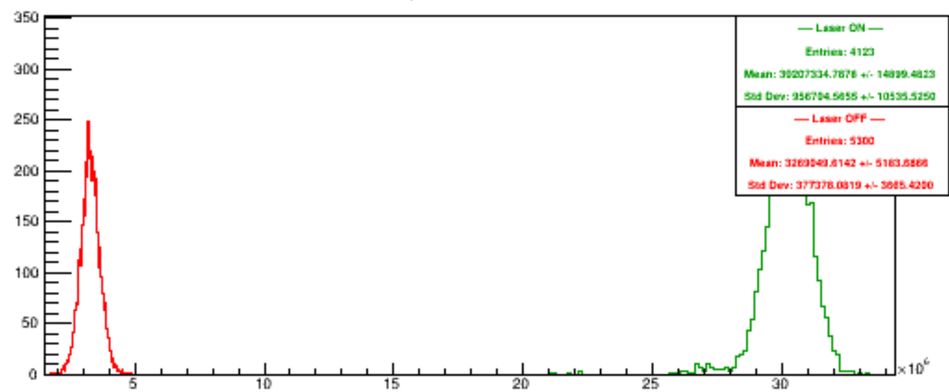
Run 6171 quartetwise, PosHelAcc4
