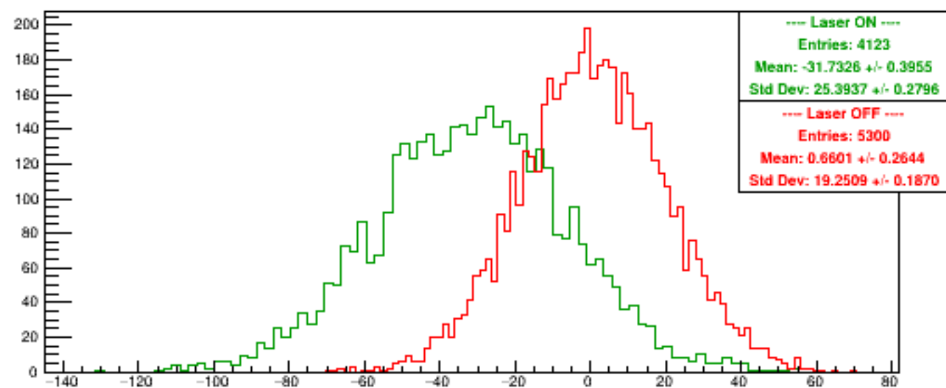
Run 6171 quartetwise, Asyms0
