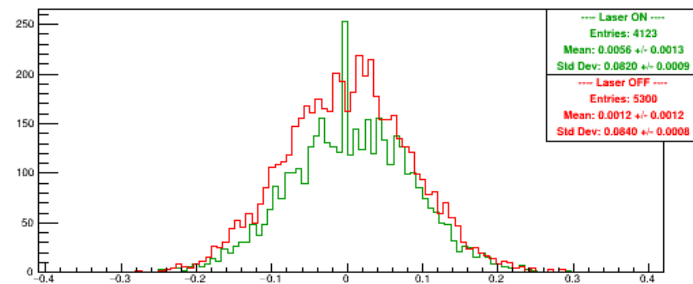
Run 6171 quartetwise, Asyms DSbg2
