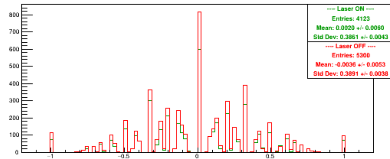
Run 6171 quartetwise, Asyms USbg2
