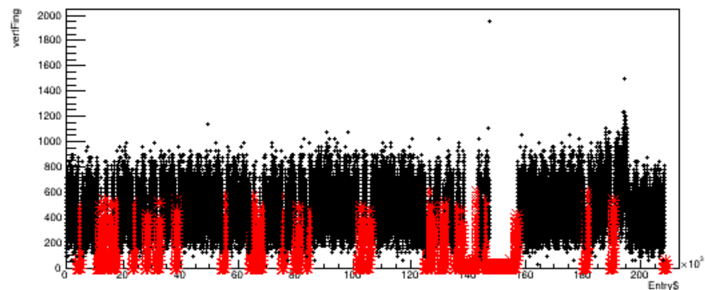
Run 6173, quartetwise: vertFing vs time
