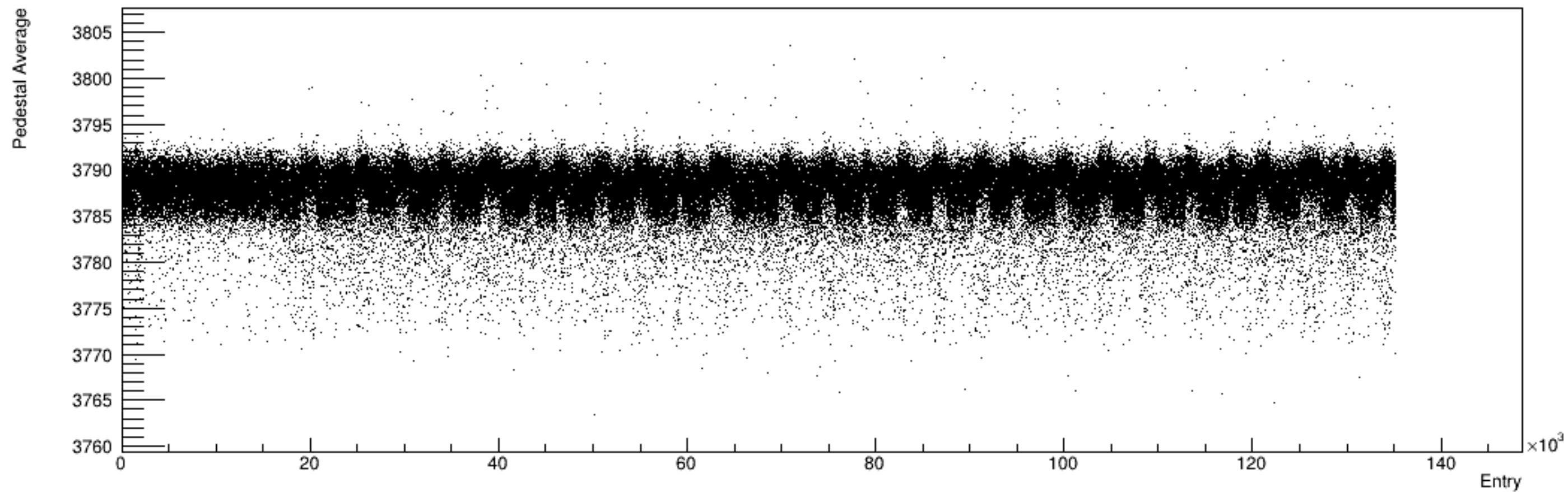
Run 6176, snapshots: Pedestal vs. Time
