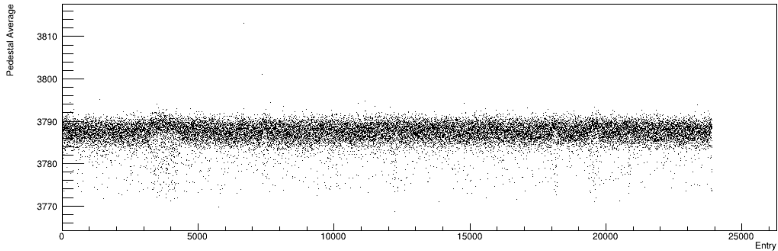
Run 6183, snapshots: Pedestal vs. Time
