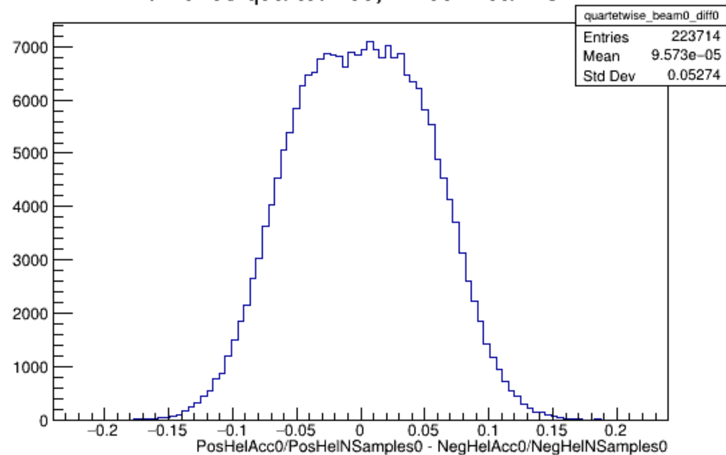
Run 6203 quartetwise, Diffs0: Beam OFF
