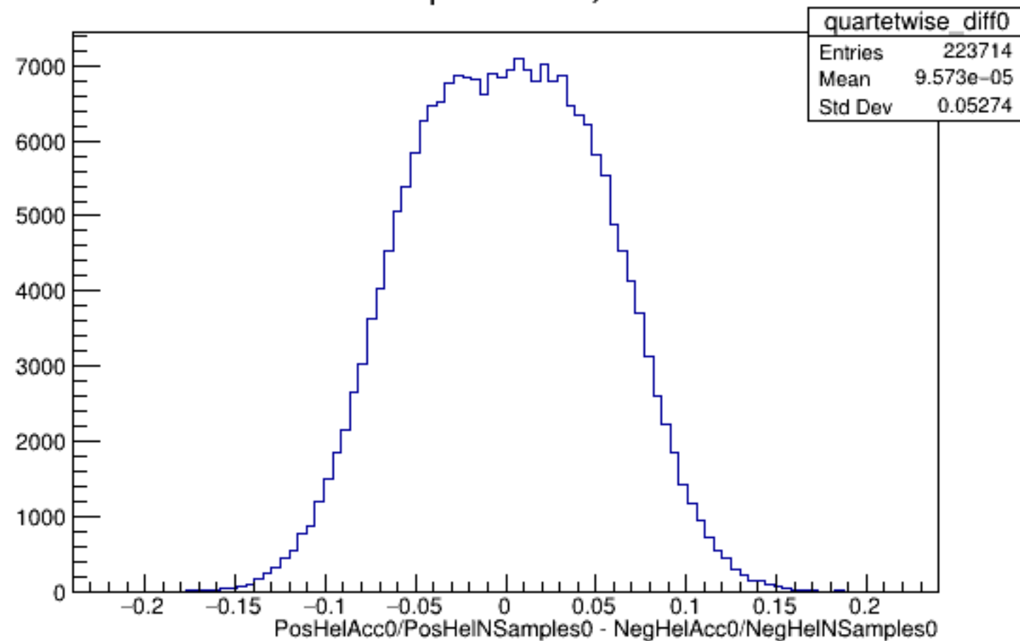
Run 6203 quartetwise, Diffs0: All
