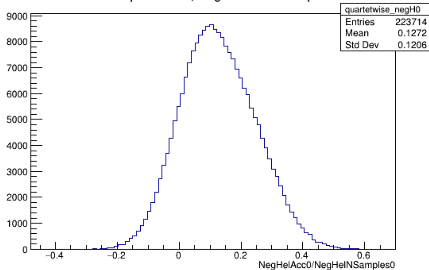
Run 6203 quartetwise, NegHelAcc0/NSamples0: All
