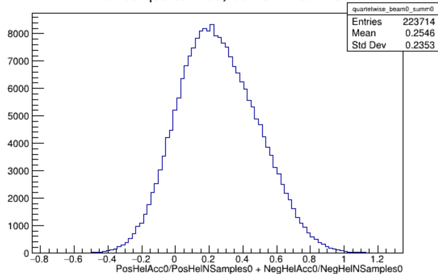
Run 6203 quartetwise, Sums0: Beam OFF
