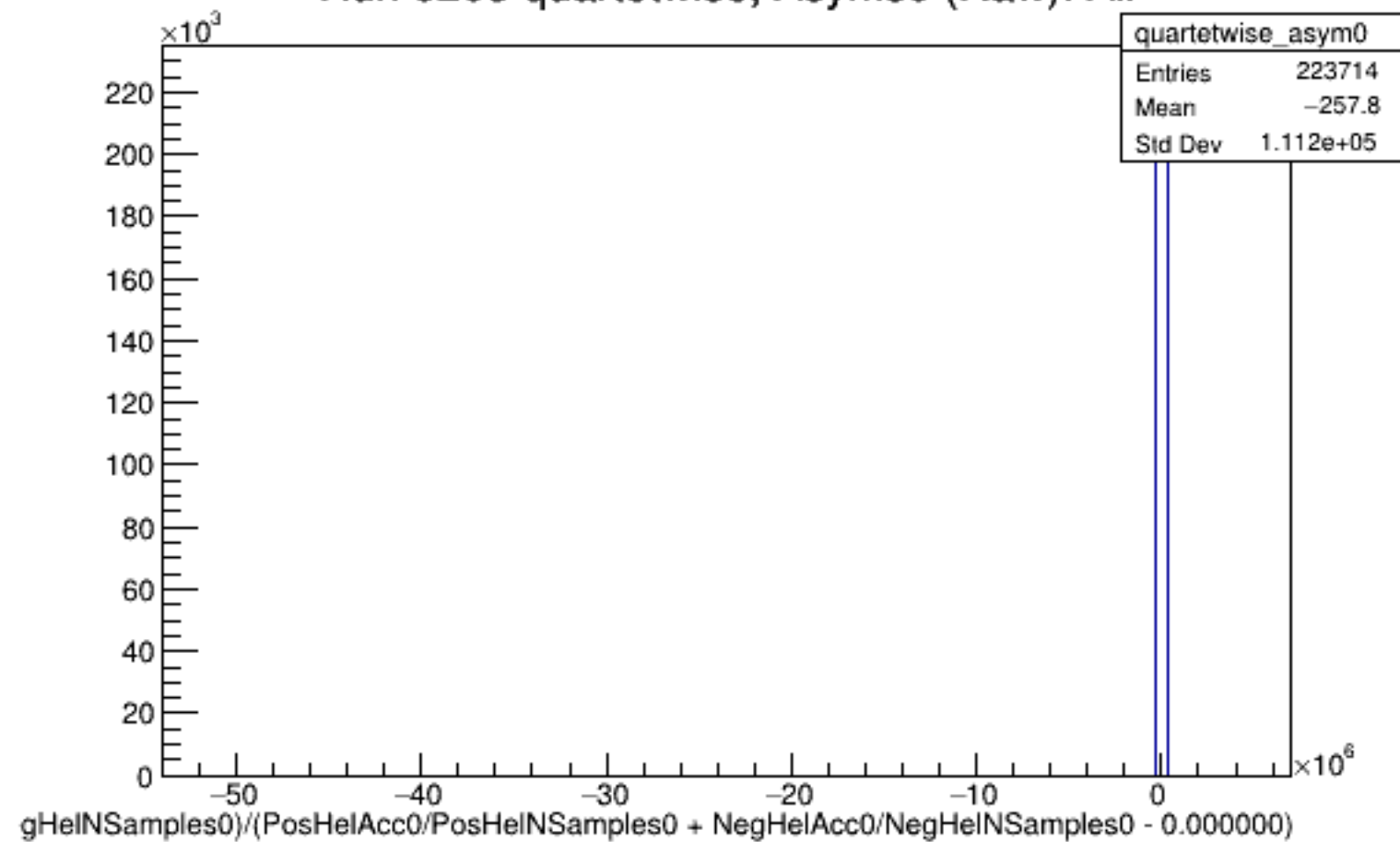
Run 6203 quartetwise, Asyms0 (Raw): All
