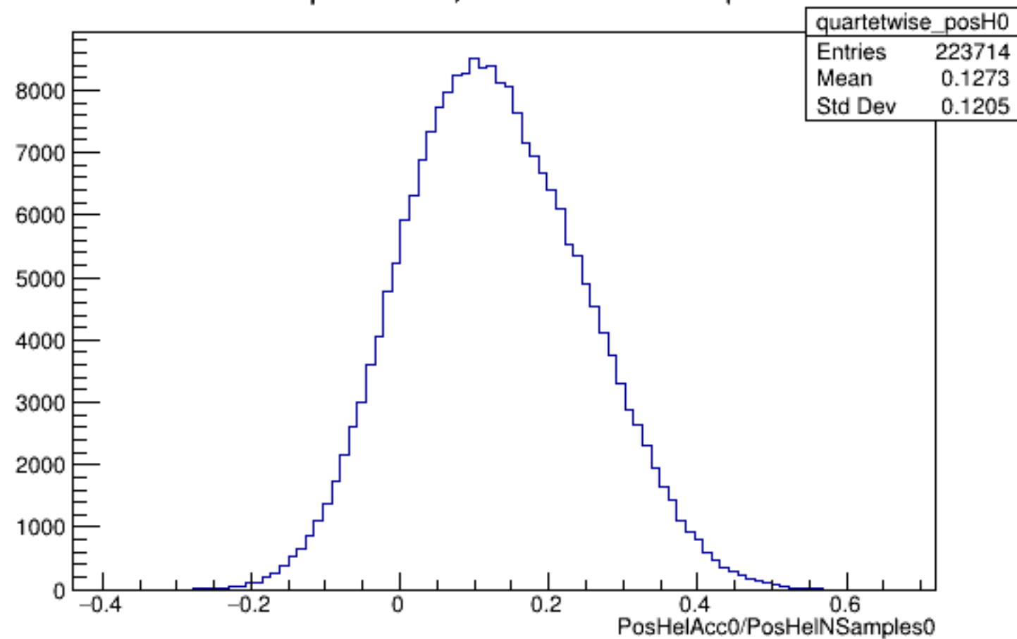
Run 6203 quartetwise, PosHelAcc0/NSamples0: All
