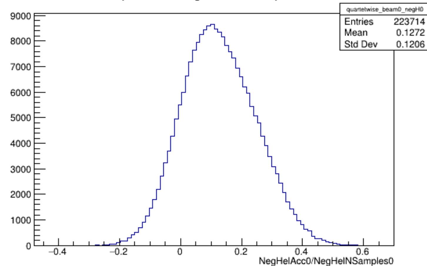
Run 6203 quartetwise, NegHelAcc0/NSamples0: Beam OFF
