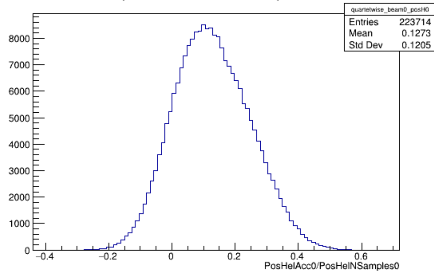
Run 6203 quartetwise, PosHelAcc0/NSamples0: Beam OFF
