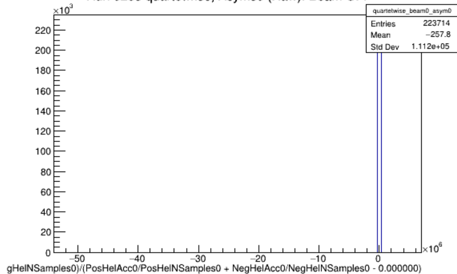
Run 6203 quartetwise, Asyms0 (Raw): Beam OFF
