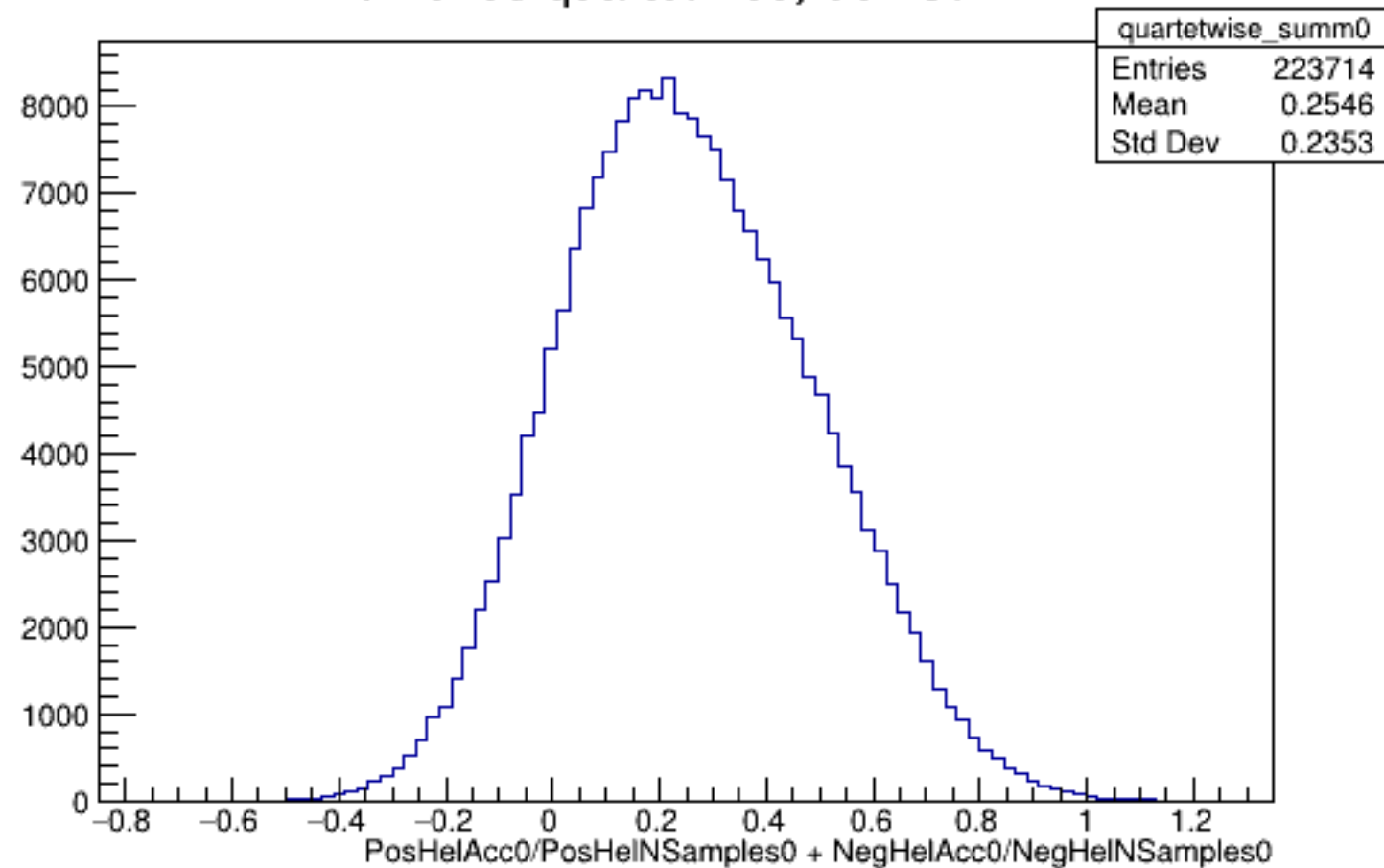
Run 6203 quartetwise, Sums0: All
