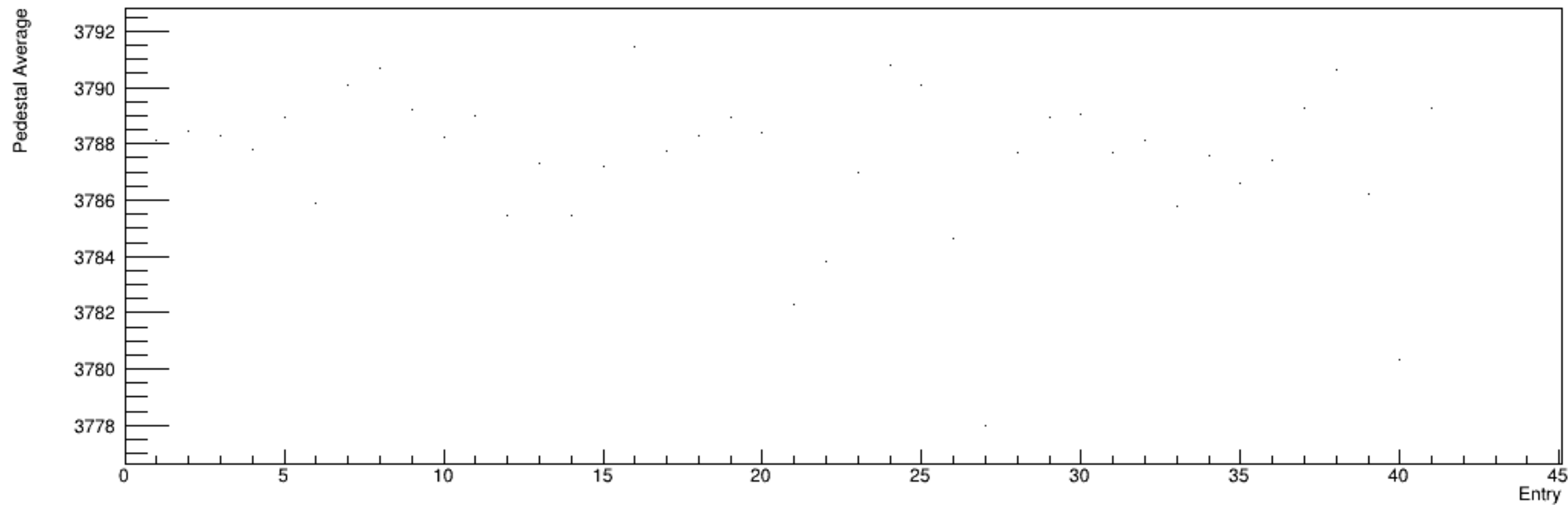
Run 6203, snapshots: Pedestal vs. Time
