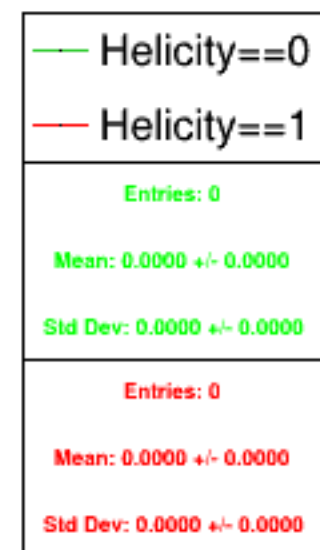
Run 6203 triggerwise, sums: Beam ON, Laser OFF
