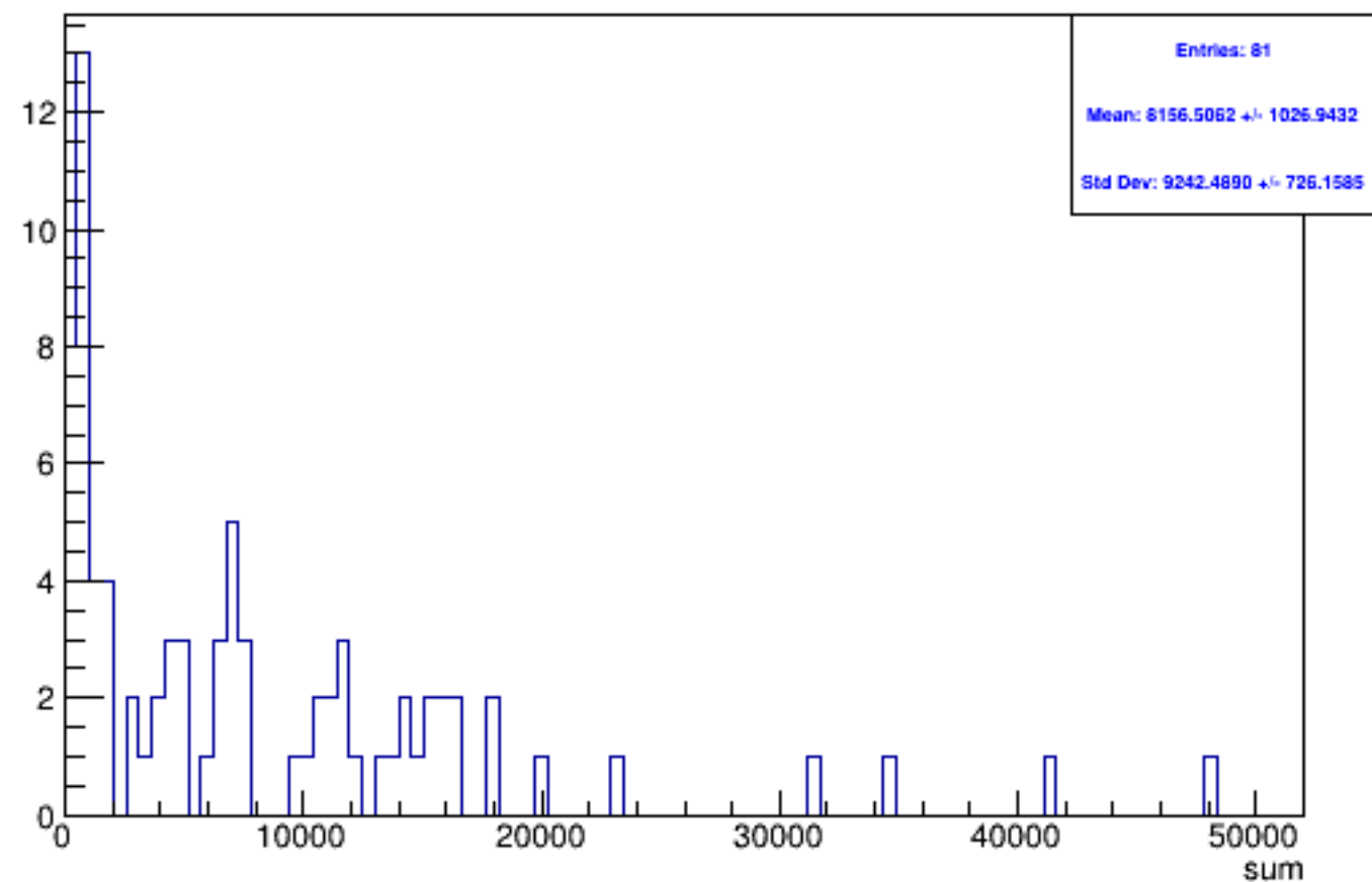
Run 6203 triggerwise, sums: Beam OFF
