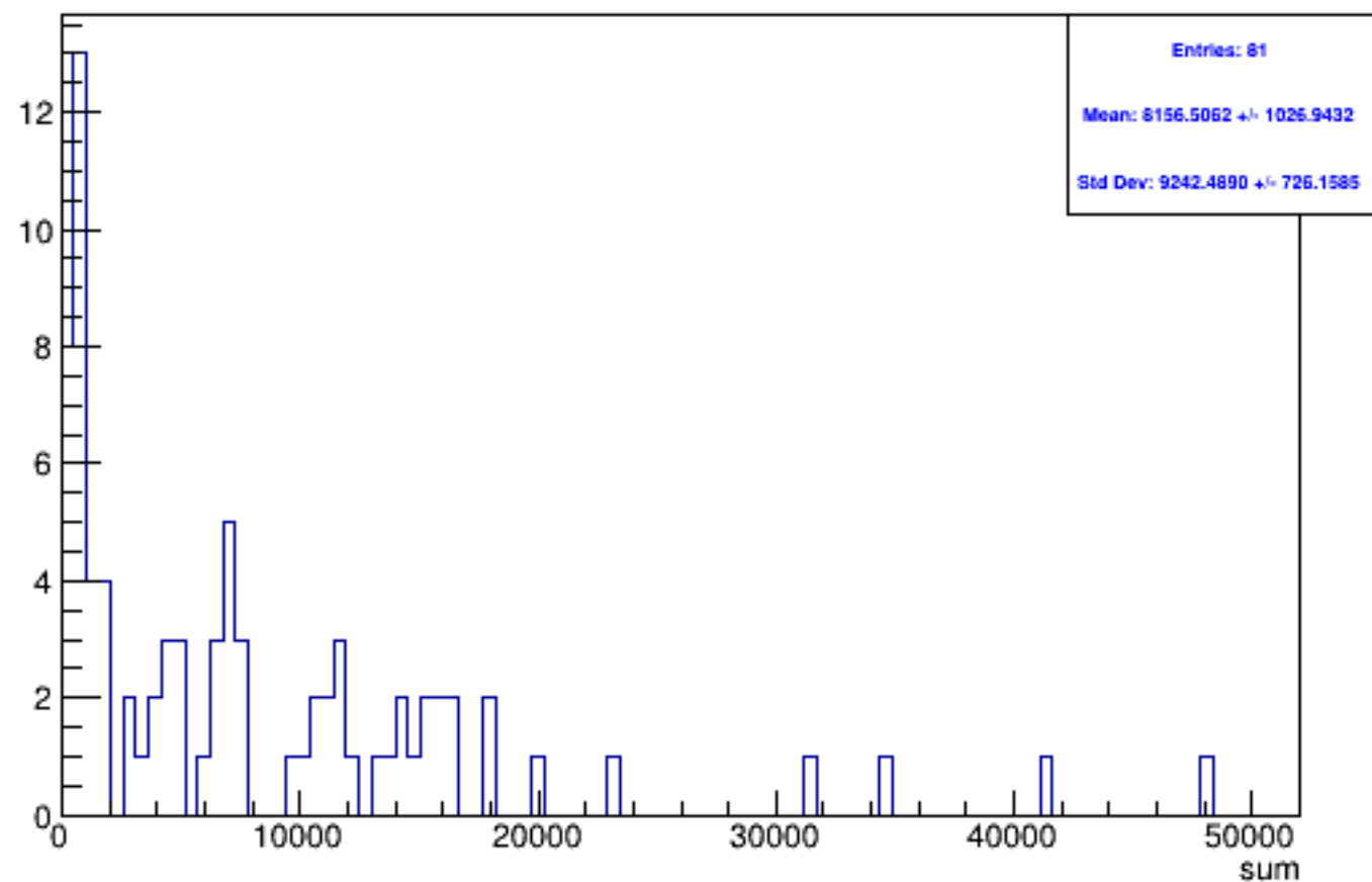
Run 6203 triggerwise, sums: All
