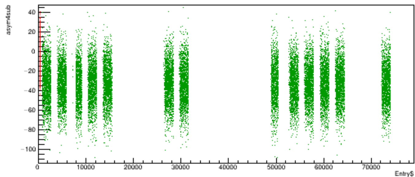
Run 6226 quartetwise, asym4sub vs time
