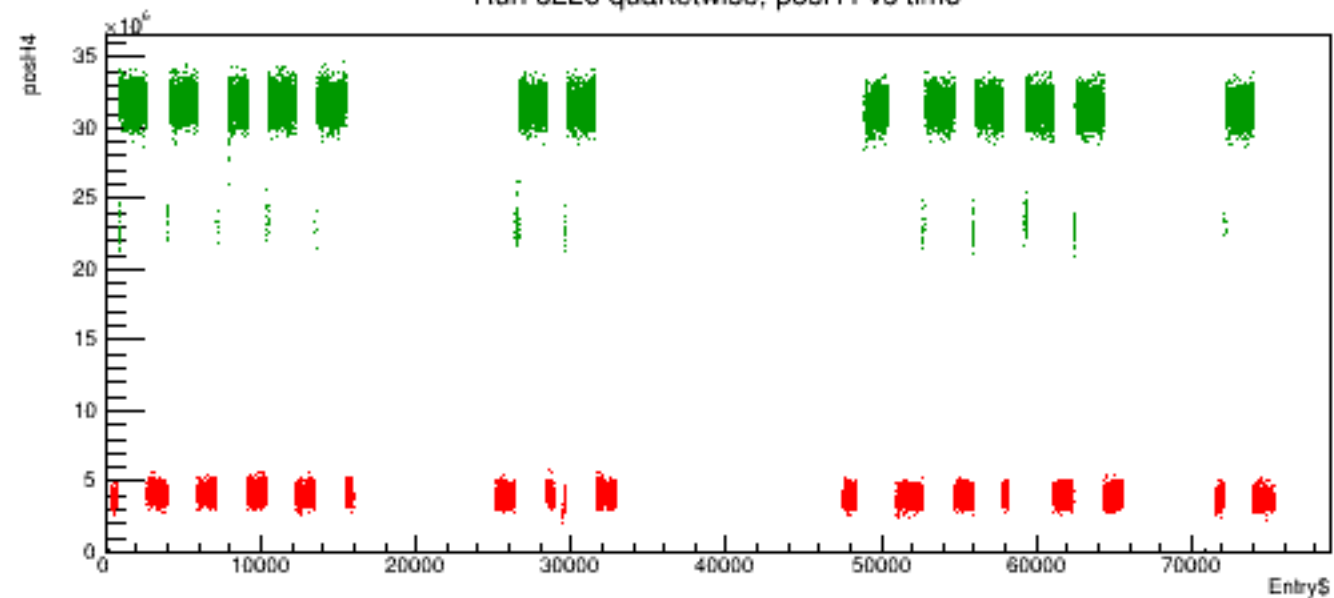
Run 6226 quartetwise, posH4 vs time
