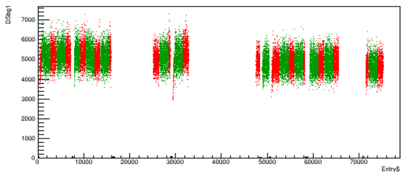
Run 6226 quartetwise, DSbg1 vs time
