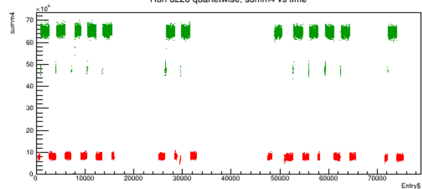
Run 6226 quartetwise, summ4 vs time
