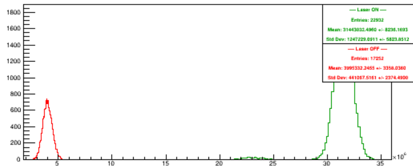
Run 6226 quartetwise, PosHelAcc4
