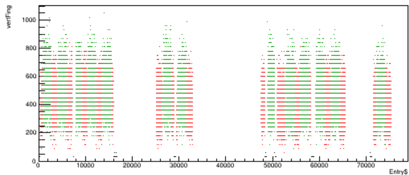
Run 6226 quartetwise, vertFing vs time
