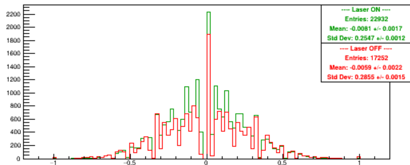
Run 6226 quartetwise, Asyms Horiz Finger
