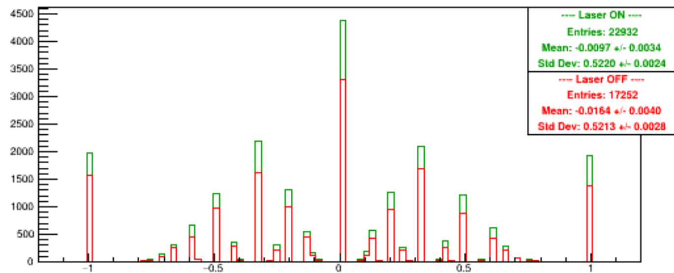
Run 6226 quartetwise, Asyms USbg1
