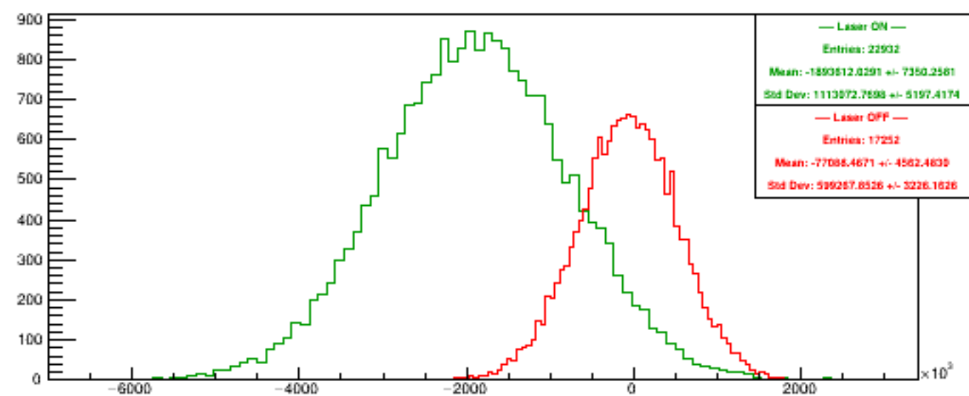
Run 6226 quartetwise, Diffs4
