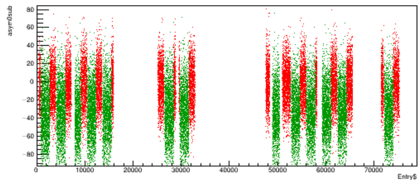
Run 6226 quartetwise, asym0sub vs time
