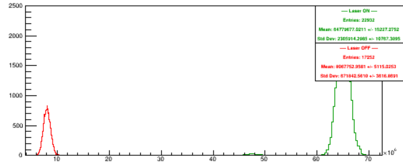
Run 6226 quartetwise, Sums4
