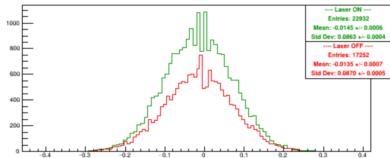
Run 6226 quartetwise, Asyms DSbg1
