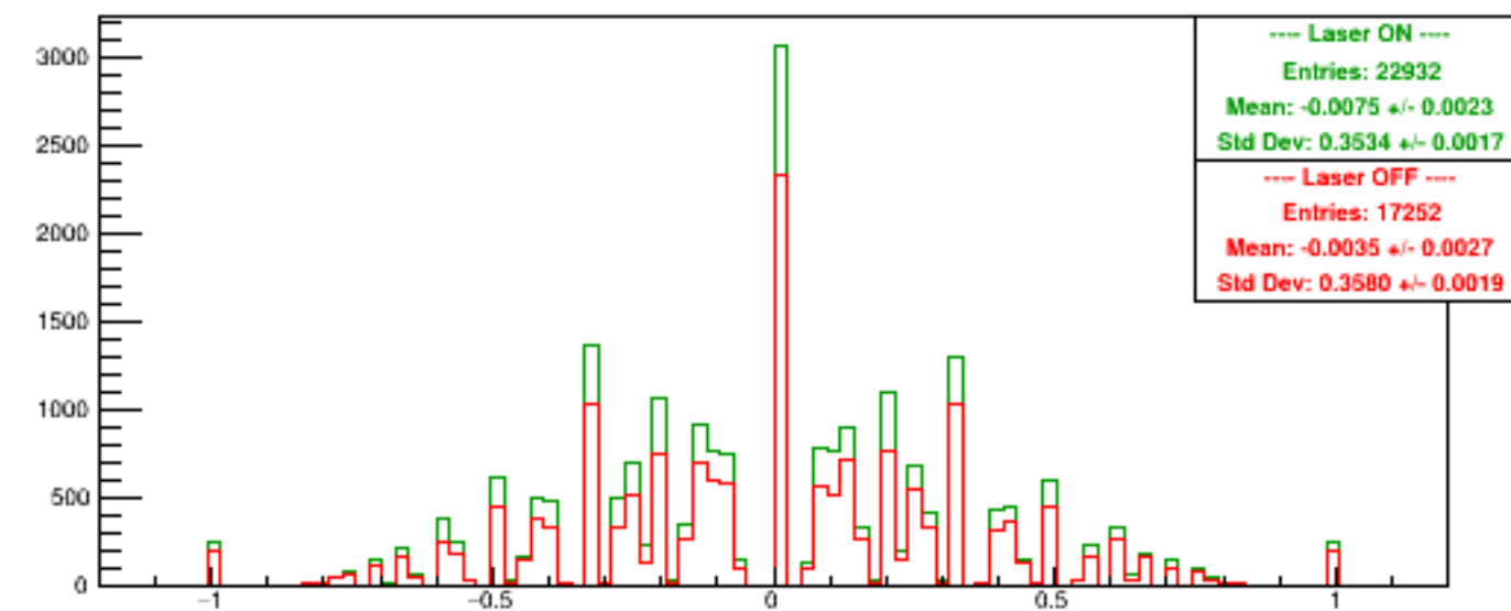
Run 6226 quartetwise, Asyms USbg2
