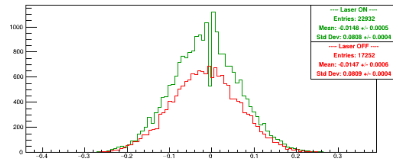
Run 6226 quartetwise, Asyms DSbg2
