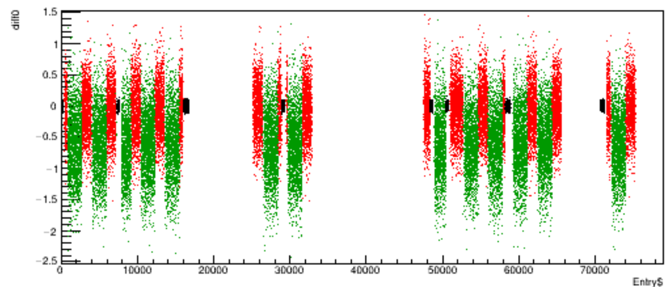
Run 6226 quartetwise, diff0 vs time
