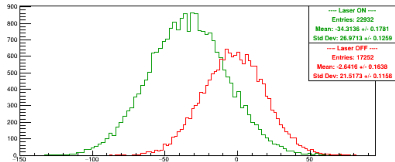
Run 6226 quartetwise, Asyms0
