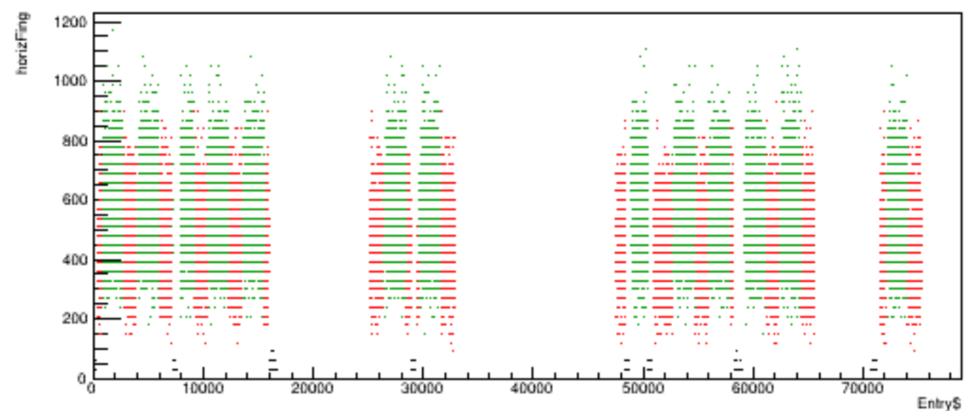
Run 6226 quartetwise, horizFing vs time
