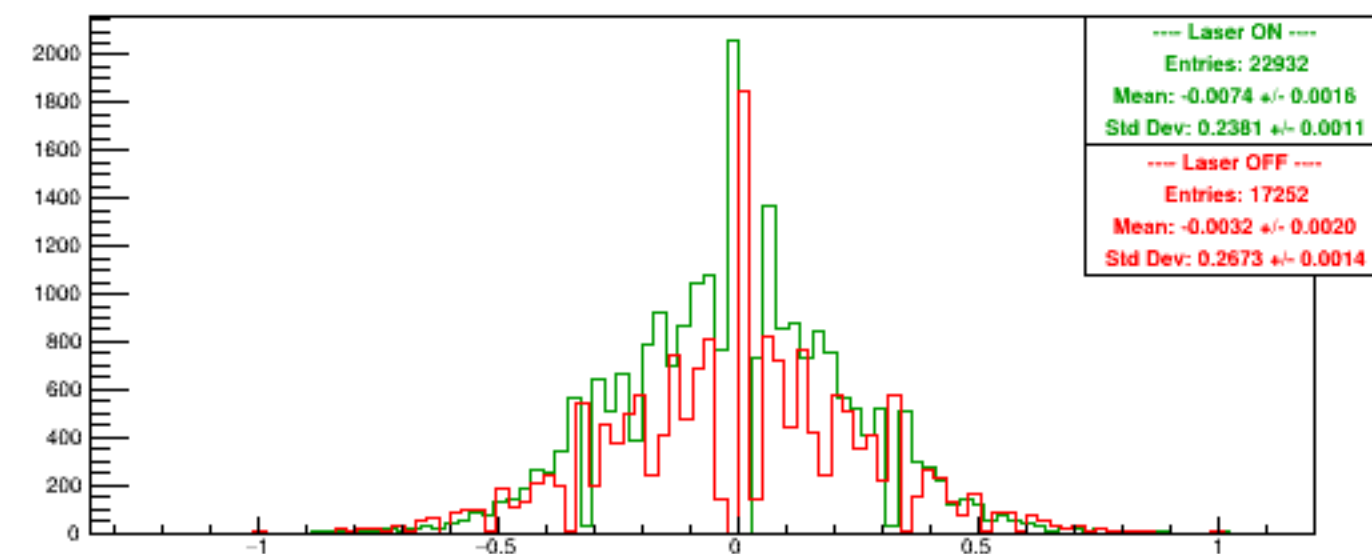
Run 6226 quartetwise, Asyms Vert Finger
