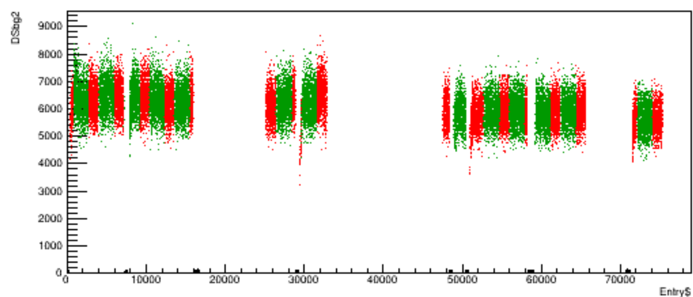
Run 6226 quartetwise, DSbg2 vs time
