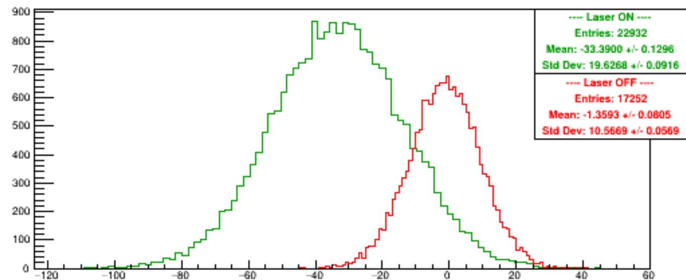
Run 6226 quartetwise, Asyms4
