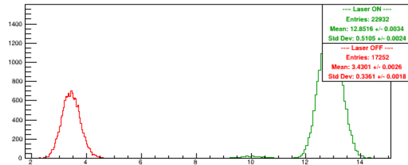
Run 6226 quartetwise, NegHelAcc0/NSamples0
