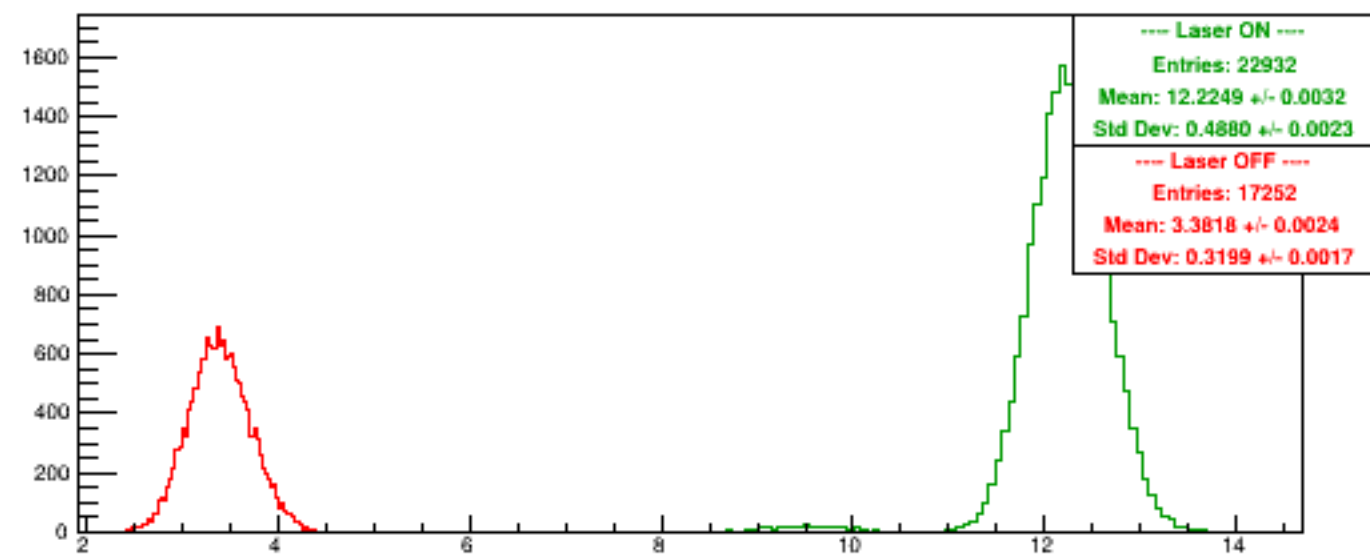
Run 6226 quartetwise, PosHelAcc0/NSamples0
