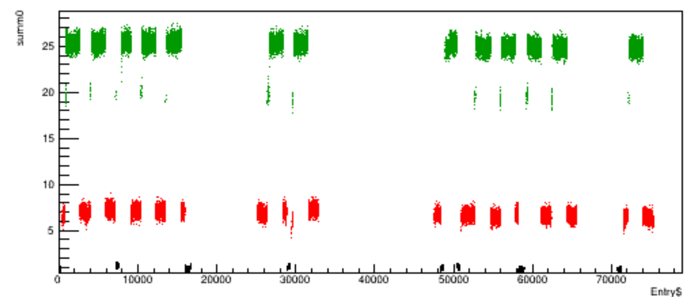
Run 6226 quartetwise, summ0 vs time
