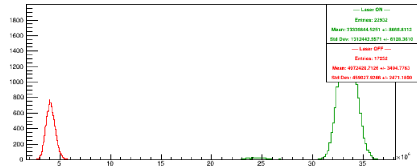
Run 6226 quartetwise, NegHelAcc4
