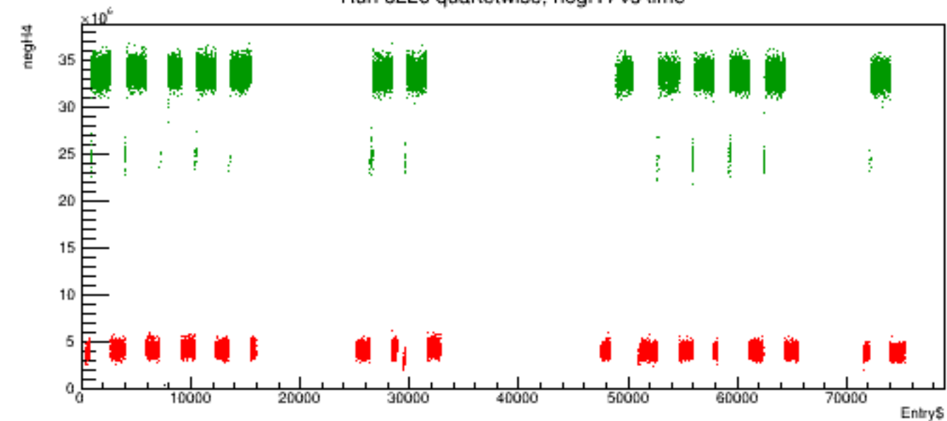
Run 6226 quartetwise, negH4 vs time
