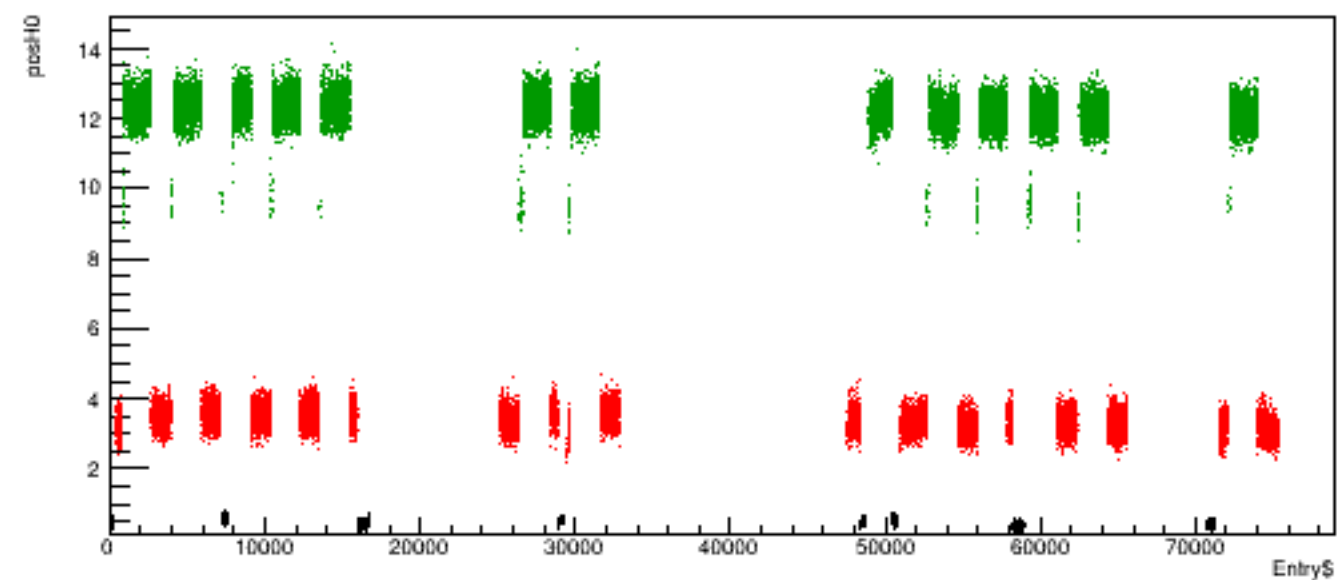
Run 6226 quartetwise, posH0 vs time
