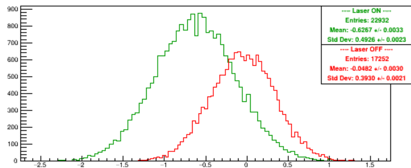
Run 6226 quartetwise, Diffs0
