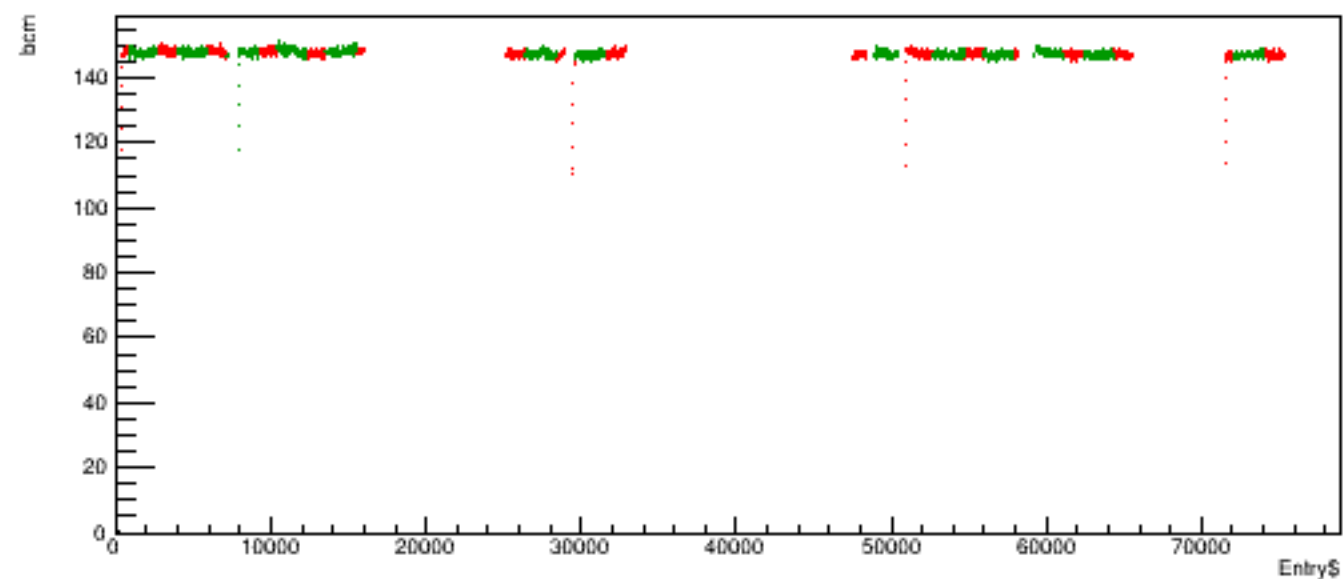
Run 6226 quartetwise, posH4 vs time
