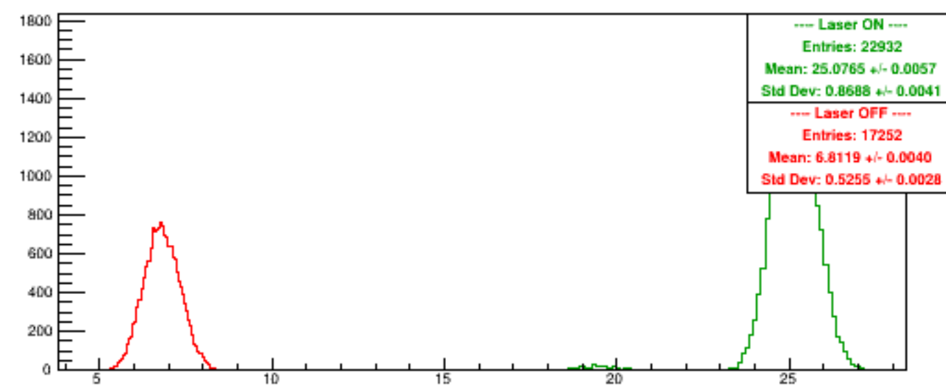
Run 6226 quartetwise, Sums0
