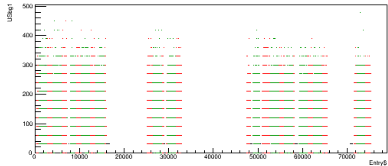
Run 6226 quartetwise, USbg1 vs time
