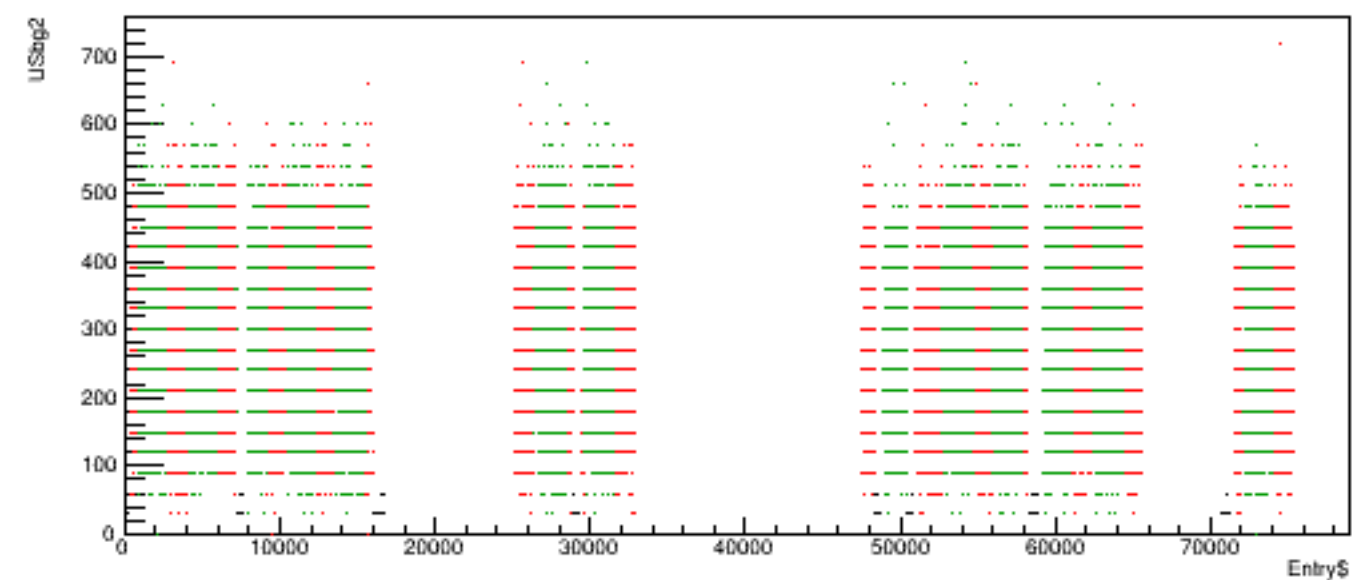
Run 6226 quartetwise, USbg2 vs time
