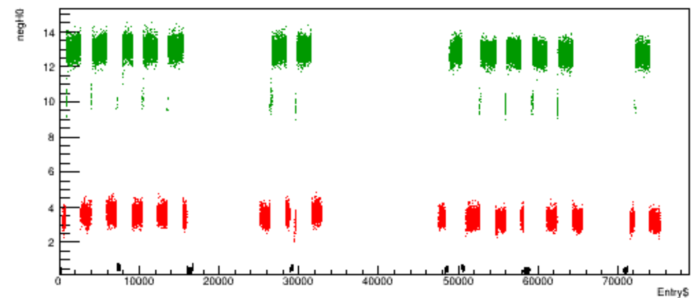
Run 6226 quartetwise, negH0 vs time
