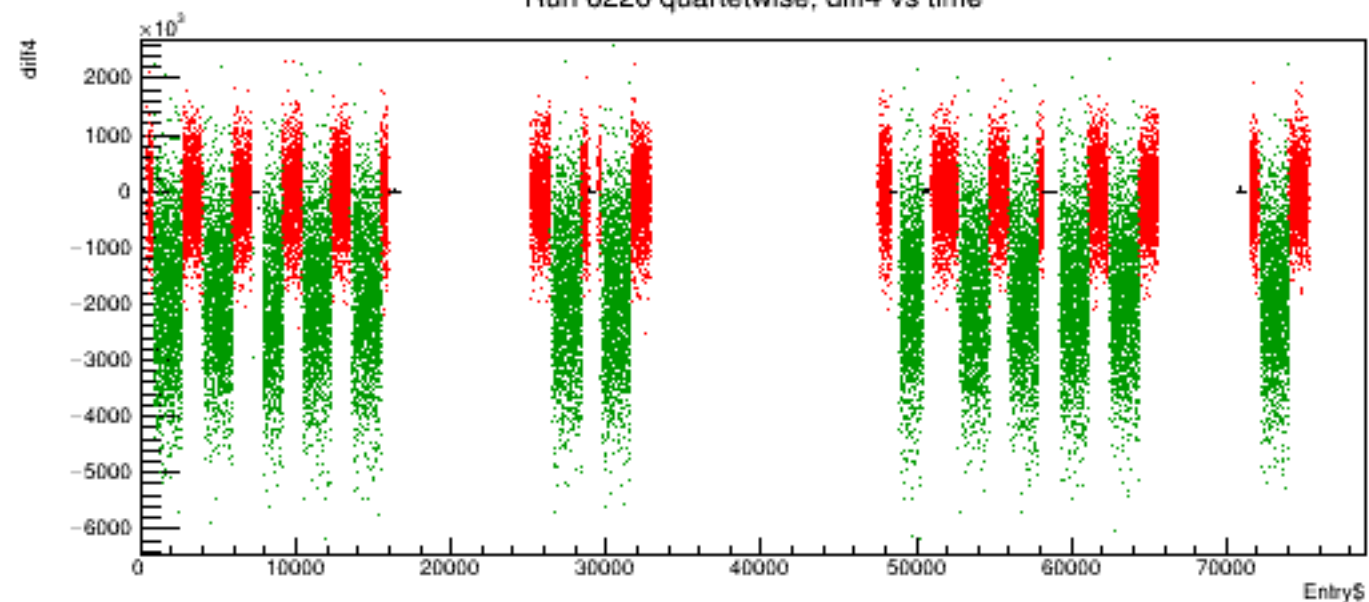
Run 6226 quartetwise, diff4 vs time
