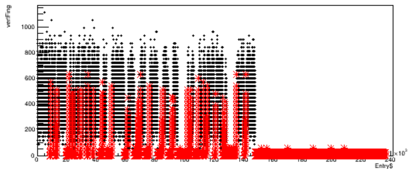
Run 6227, quartetwise: vertFing vs time
