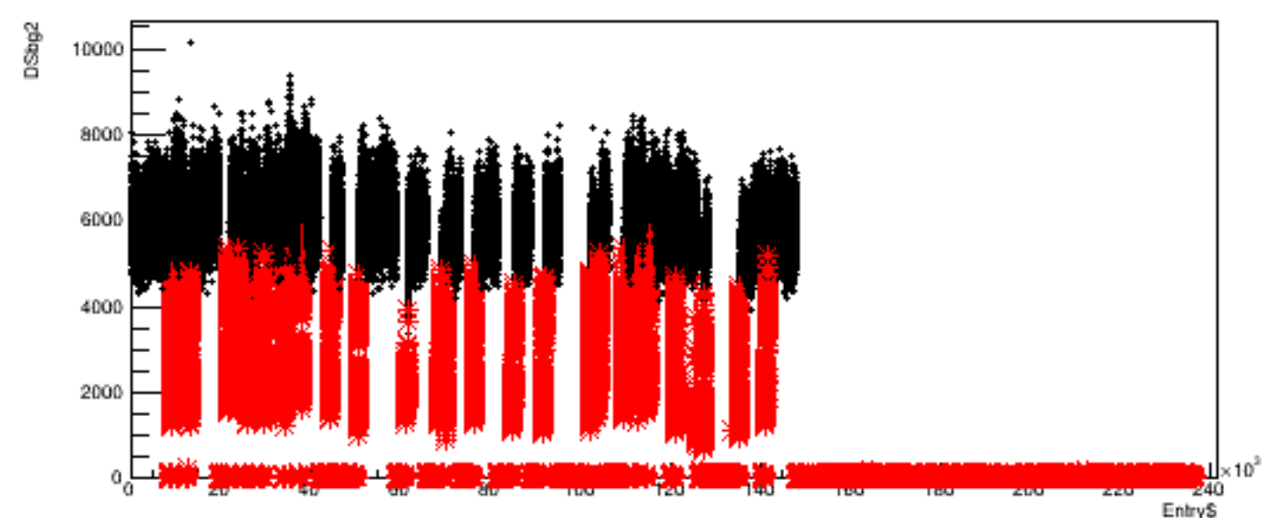
Run 6227, quartetwise: DSbg2 vs time
