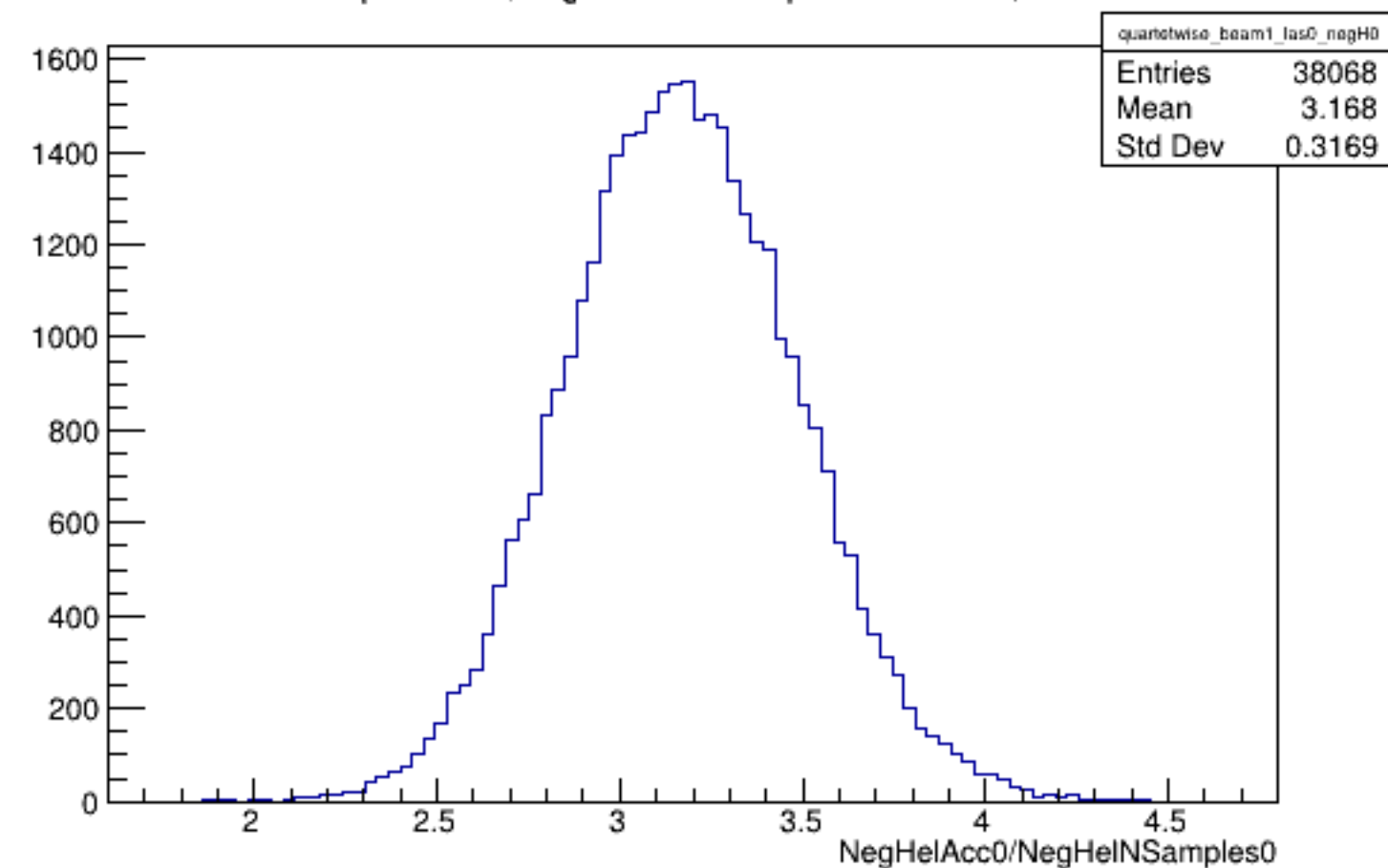
Run 6227 quartetwise, NegHelAcc0/NSamples0: Beam ON, Laser OFF
