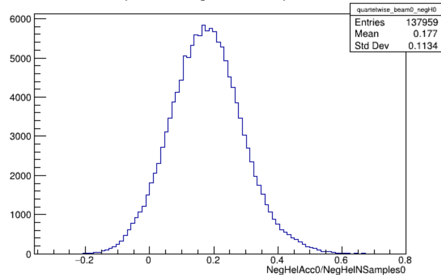
Run 6227 quartetwise, NegHelAcc0/NSamples0: Beam OFF
