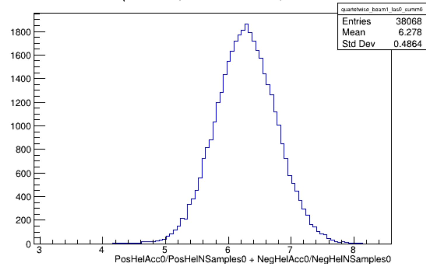
Run 6227 quartetwise, Sums0: Beam ON, Laser OFF
