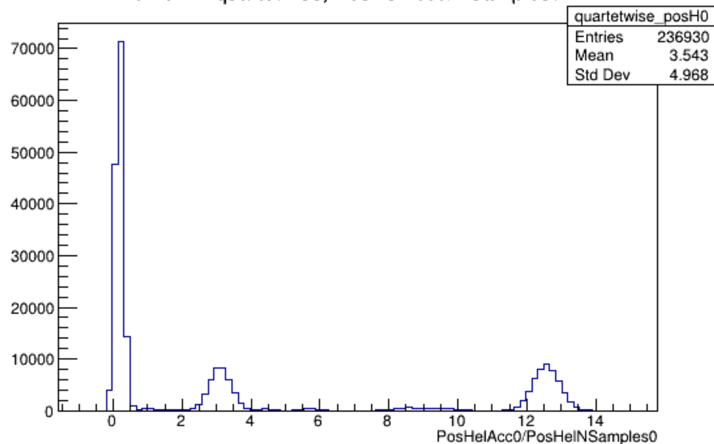
Run 6227 quartetwise, PosHelAcc0/NSamples0: All
