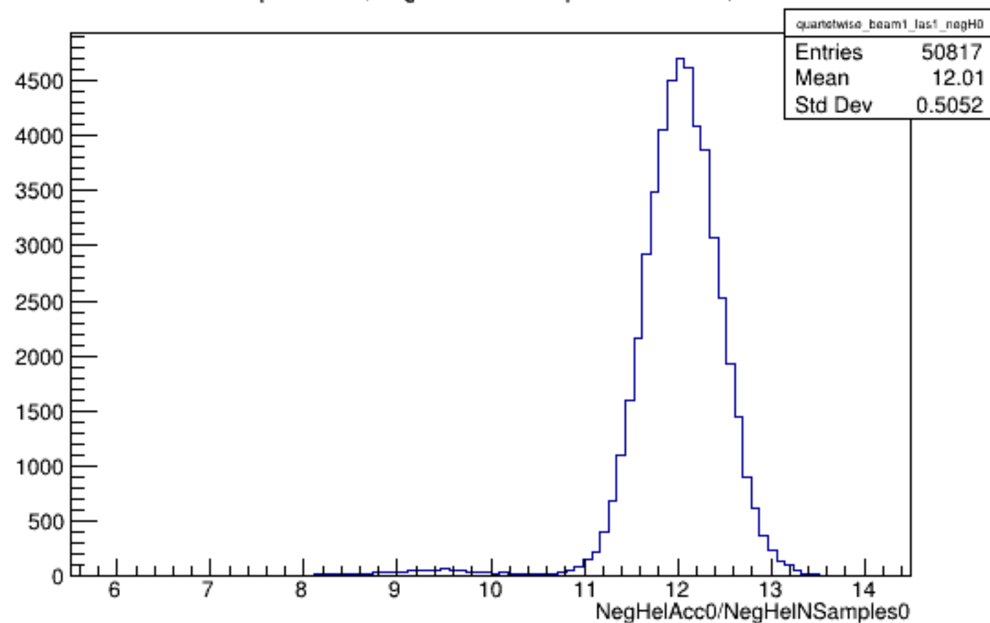
Run 6227 quartetwise, NegHelAcc0/NSamples0: Beam ON, Laser ON
