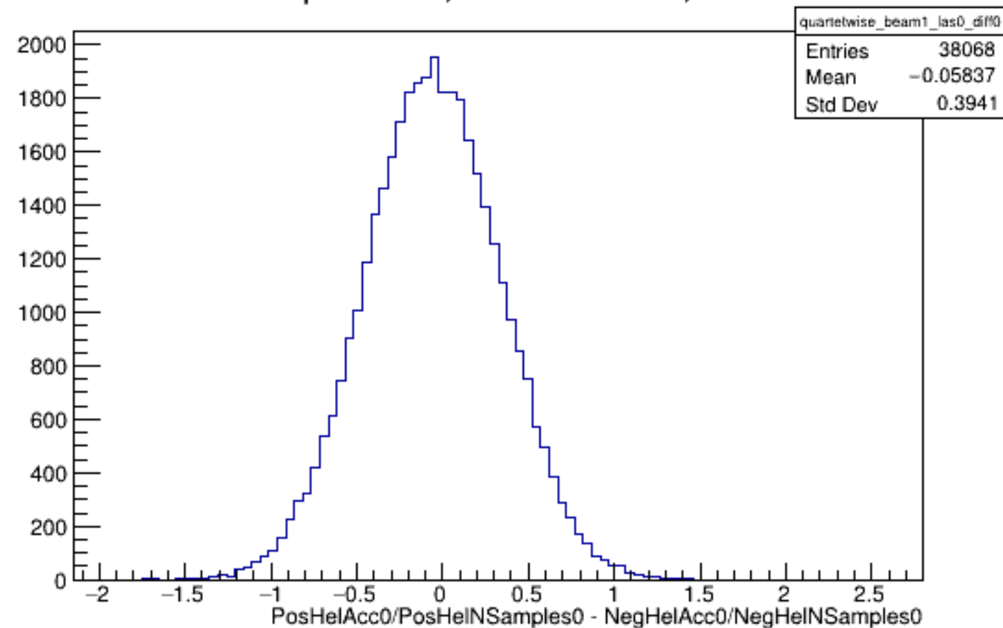
Run 6227 quartetwise, Diffs0: Beam ON, Laser OFF
