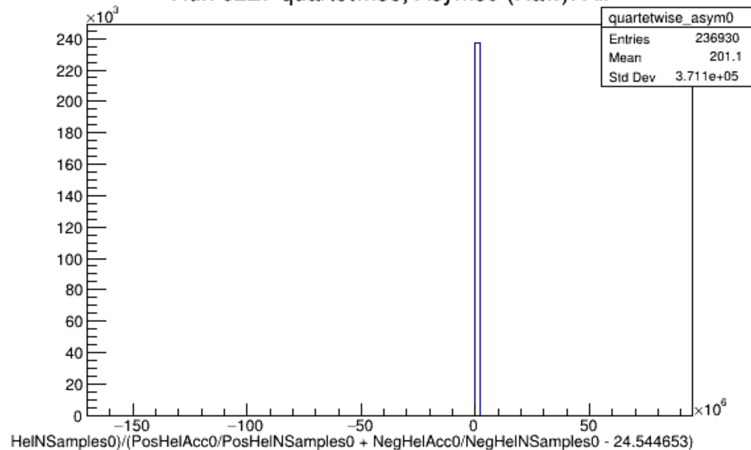
Run 6227 quartetwise, Asyms0 (Raw): All
