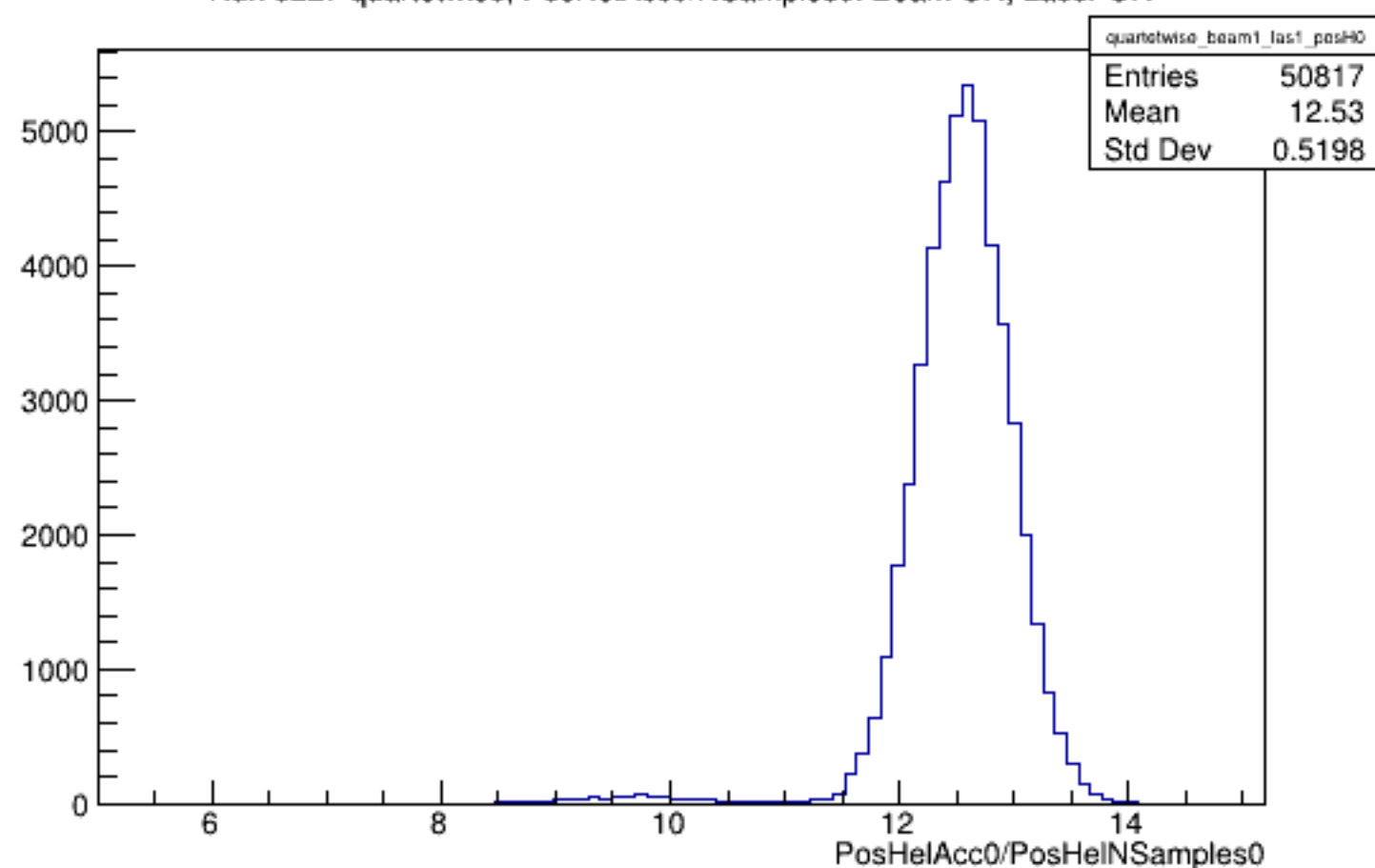
Run 6227 quartetwise, PosHelAcc0/NSamples0: Beam ON, Laser ON
