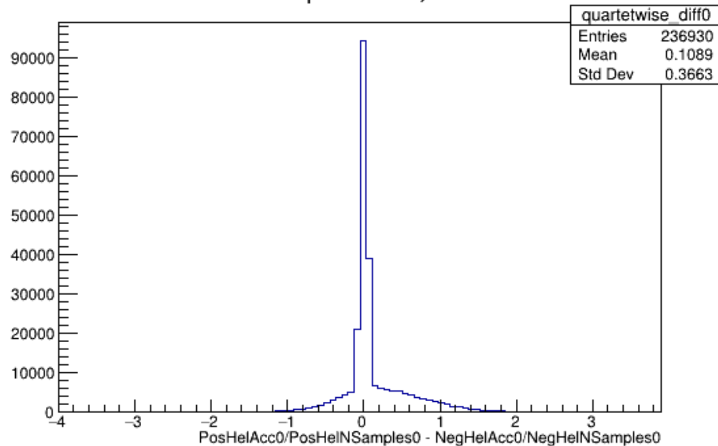
Run 6227 quartetwise, Diffs0: All
