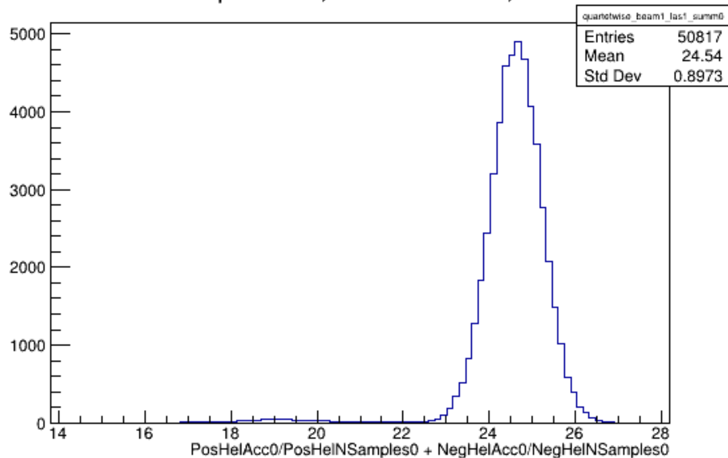
Run 6227 quartetwise, Sums0: Beam ON, Laser ON
