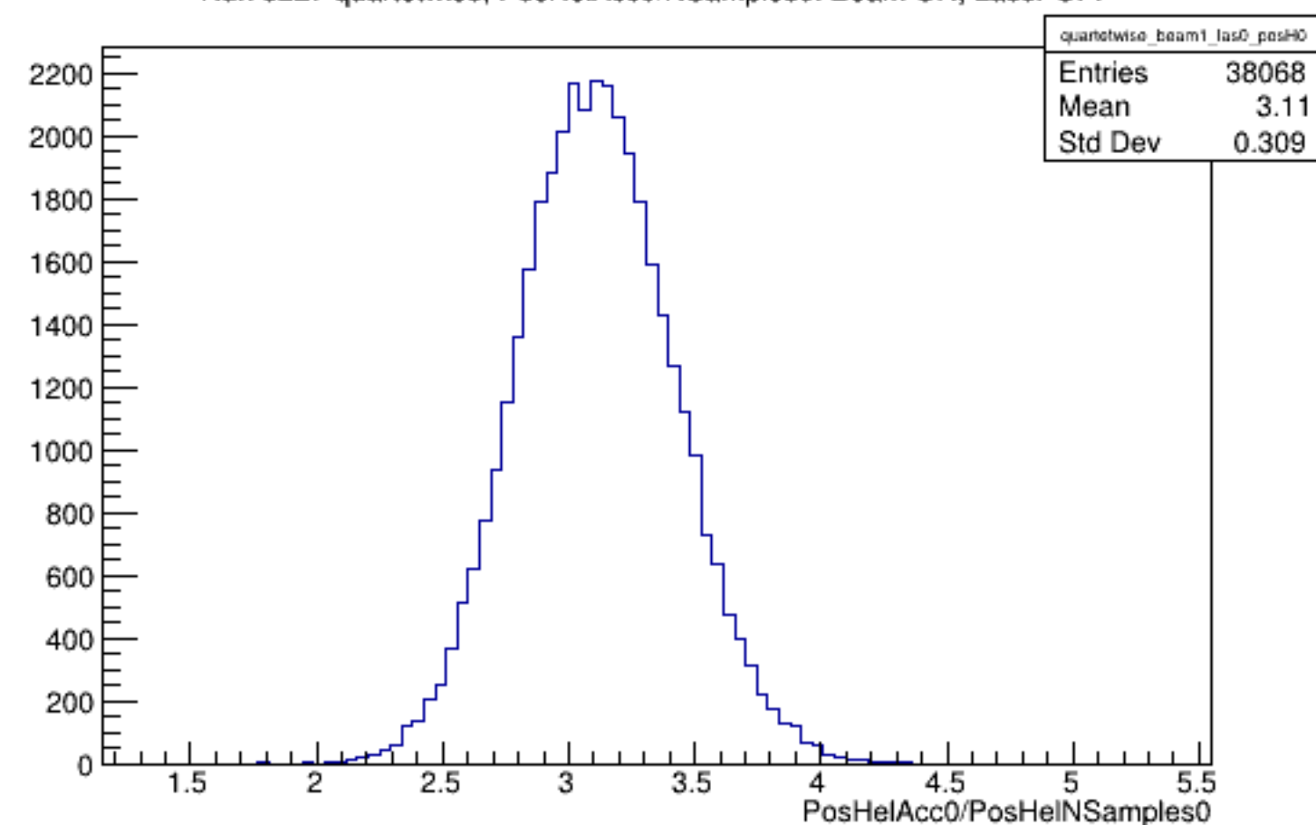
Run 6227 quartetwise, PosHelAcc0/NSamples0: Beam ON, Laser OFF
