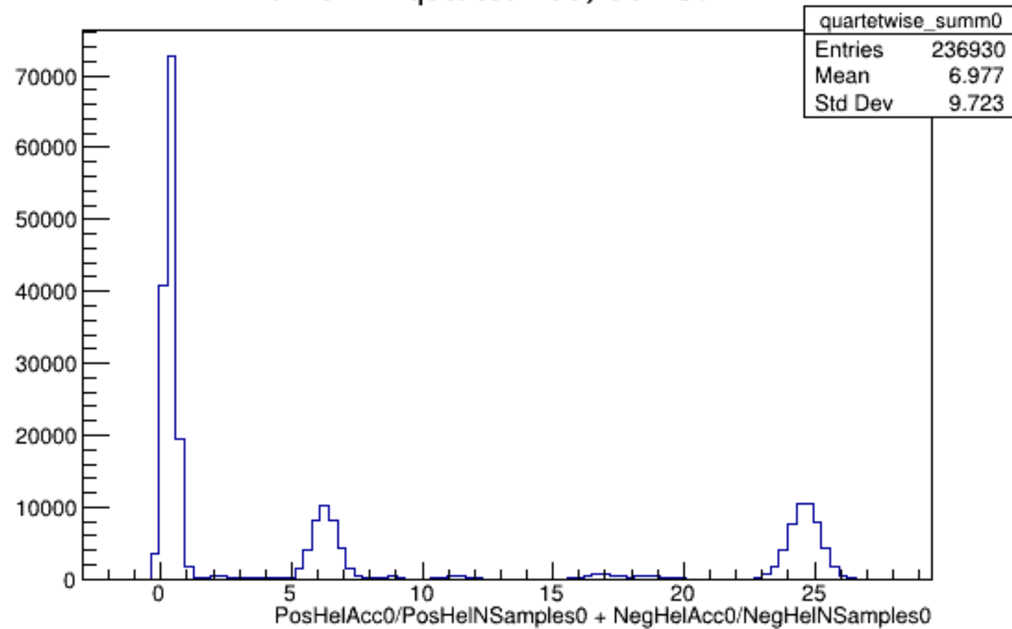
Run 6227 quartetwise, Sums0: All
