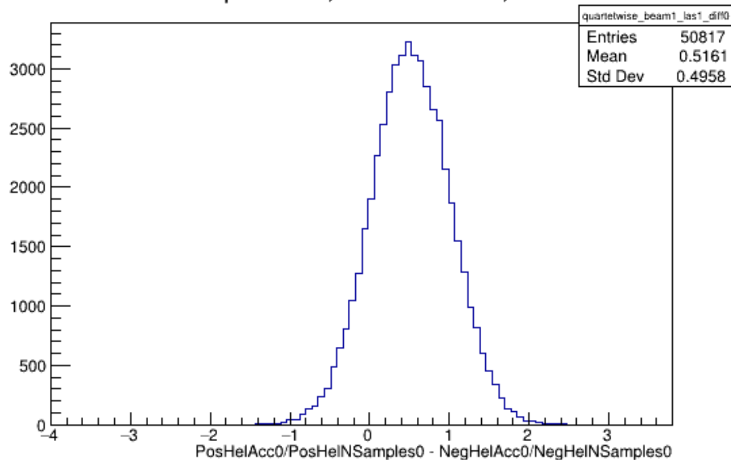
Run 6227 quartetwise, Diffs0: Beam ON, Laser ON
