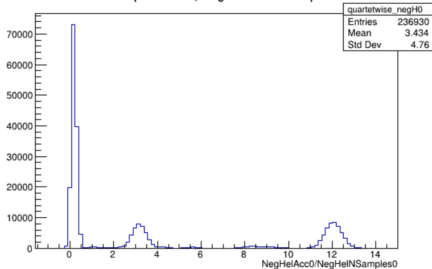
Run 6227 quartetwise, NegHelAcc0/NSamples0: All
