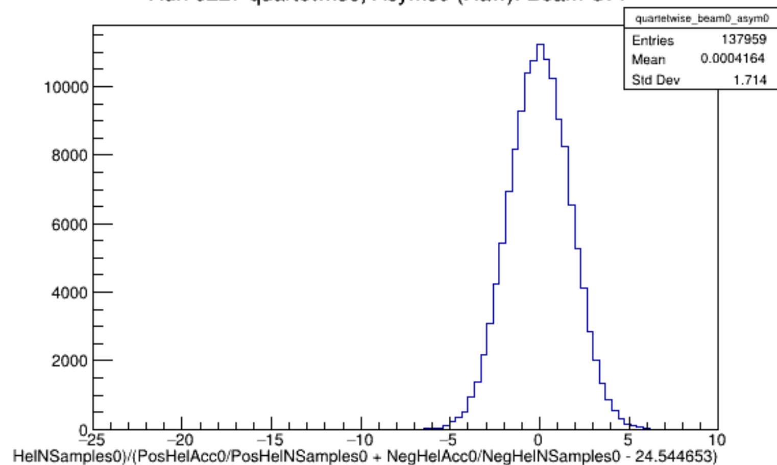
Run 6227 quartetwise, Asyms0 (Raw): Beam OFF
