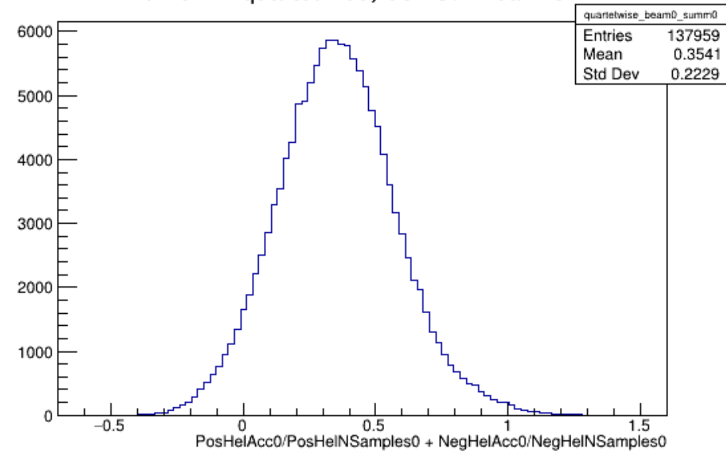
Run 6227 quartetwise, Sums0: Beam OFF
