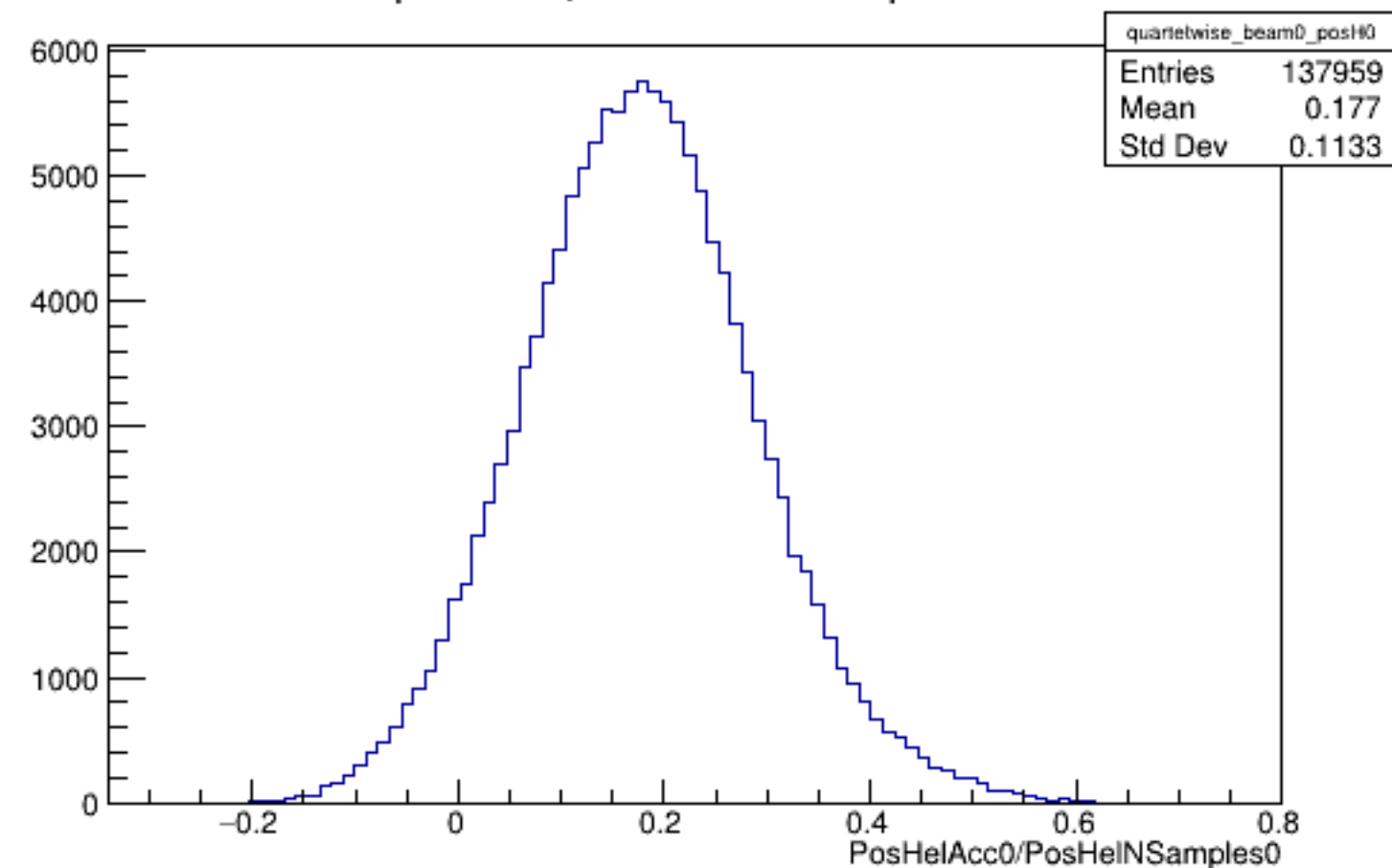
Run 6227 quartetwise, PosHelAcc0/NSamples0: Beam OFF
