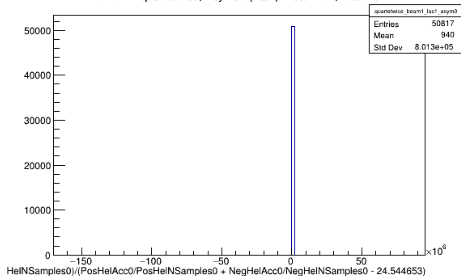
Run 6227 quartetwise, Asyms0 (Raw): Beam ON, Laser ON
