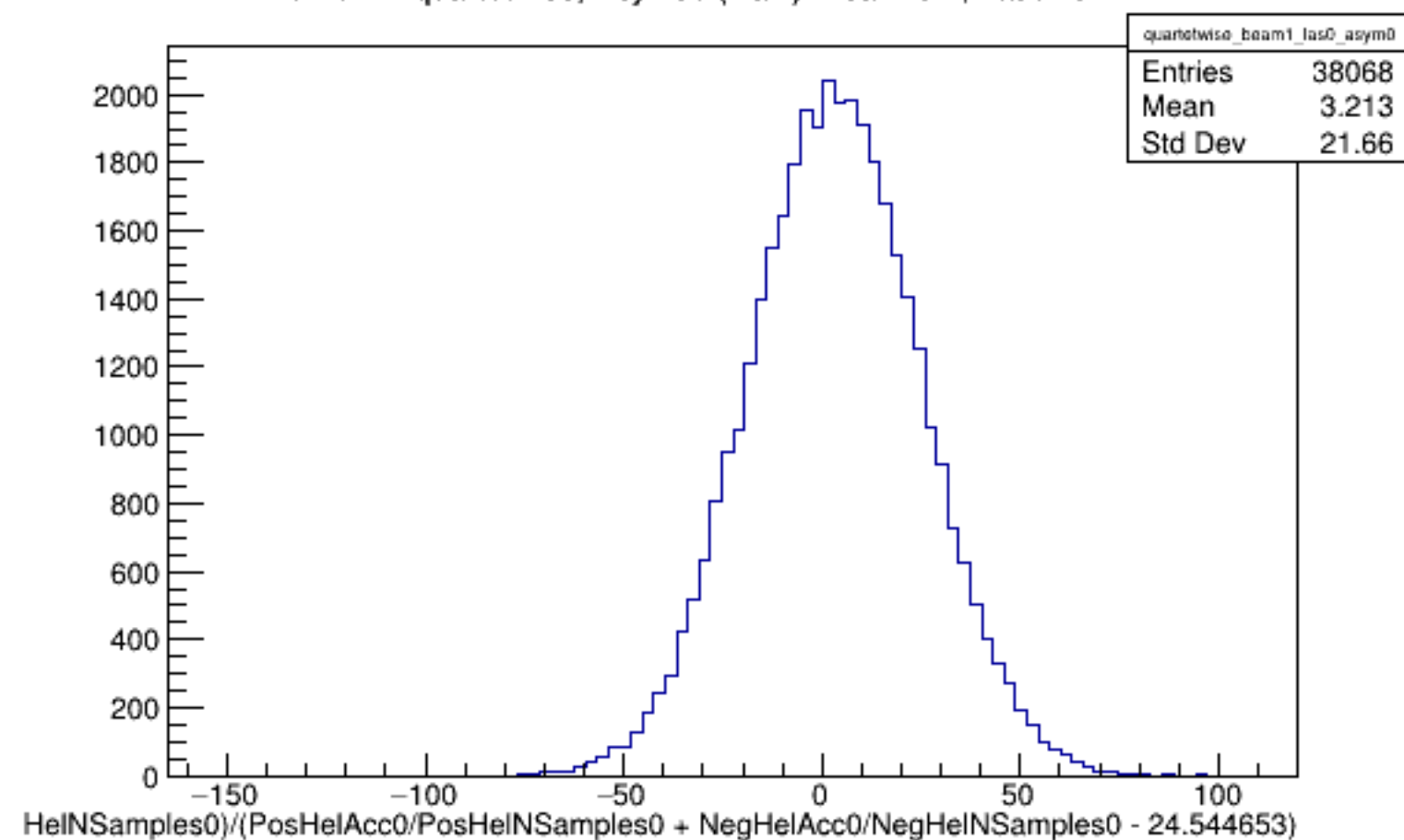
Run 6227 quartetwise, Asyms0 (Raw): Beam ON, Laser OFF
