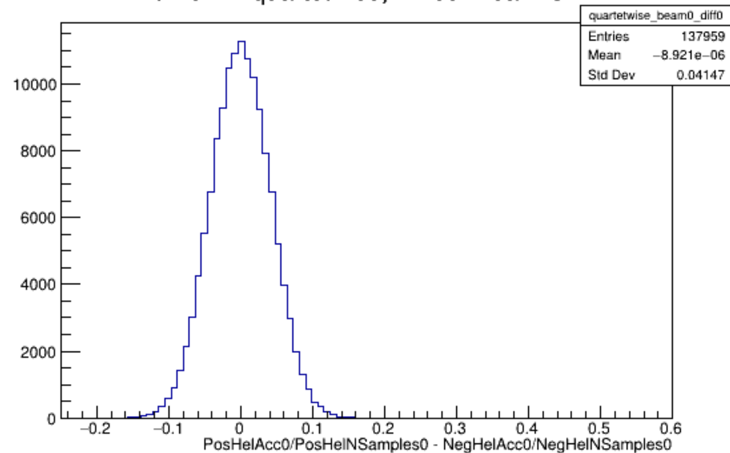
Run 6227 quartetwise, Diffs0: Beam OFF
