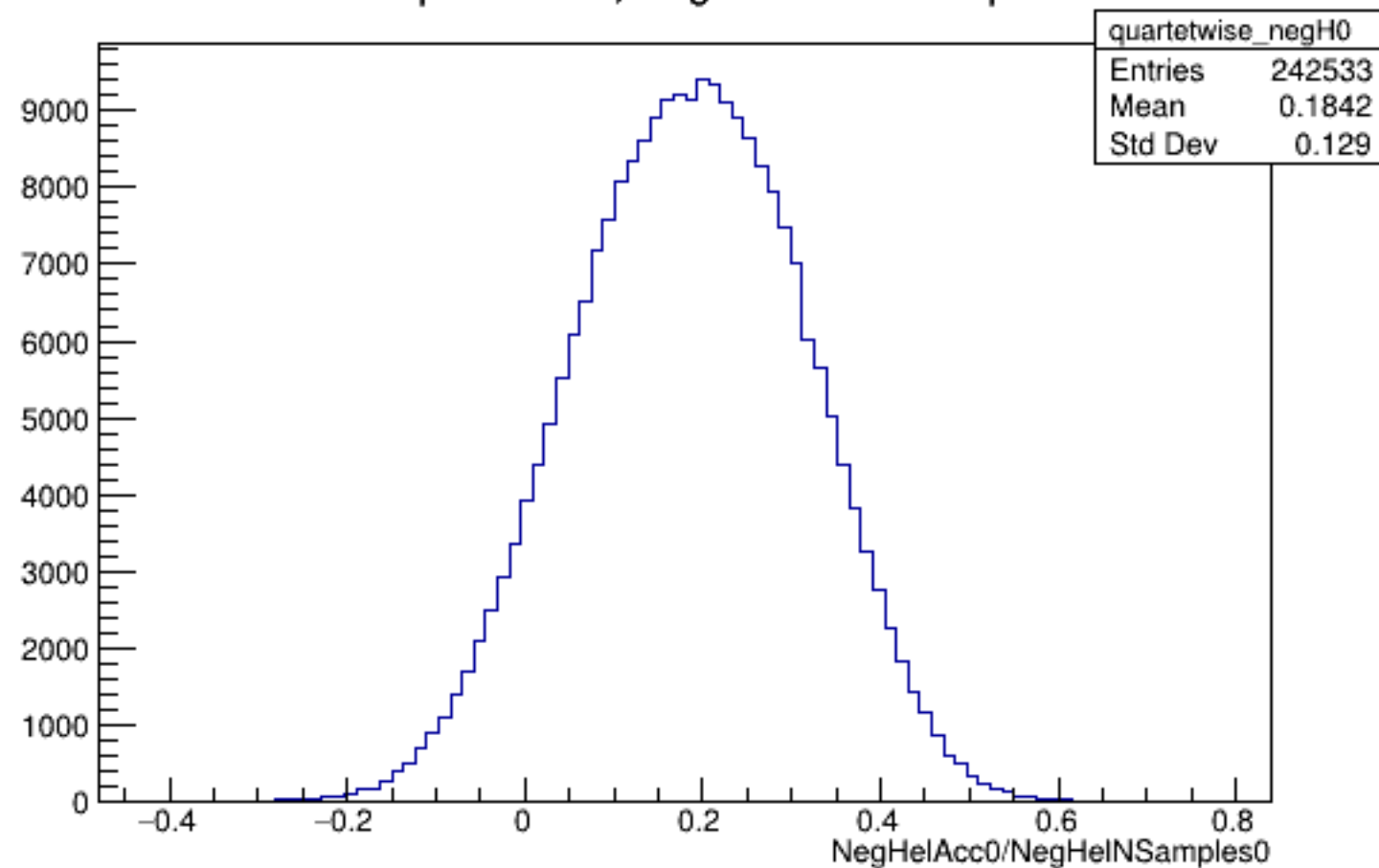
Run 6228 quartetwise, NegHelAcc0/NSamples0: All
