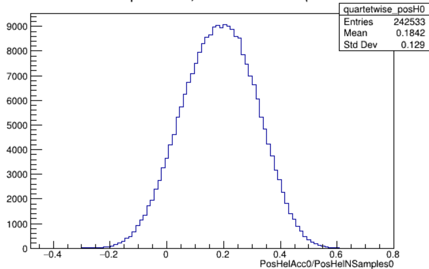
Run 6228 quartetwise, PosHelAcc0/NSamples0: All
