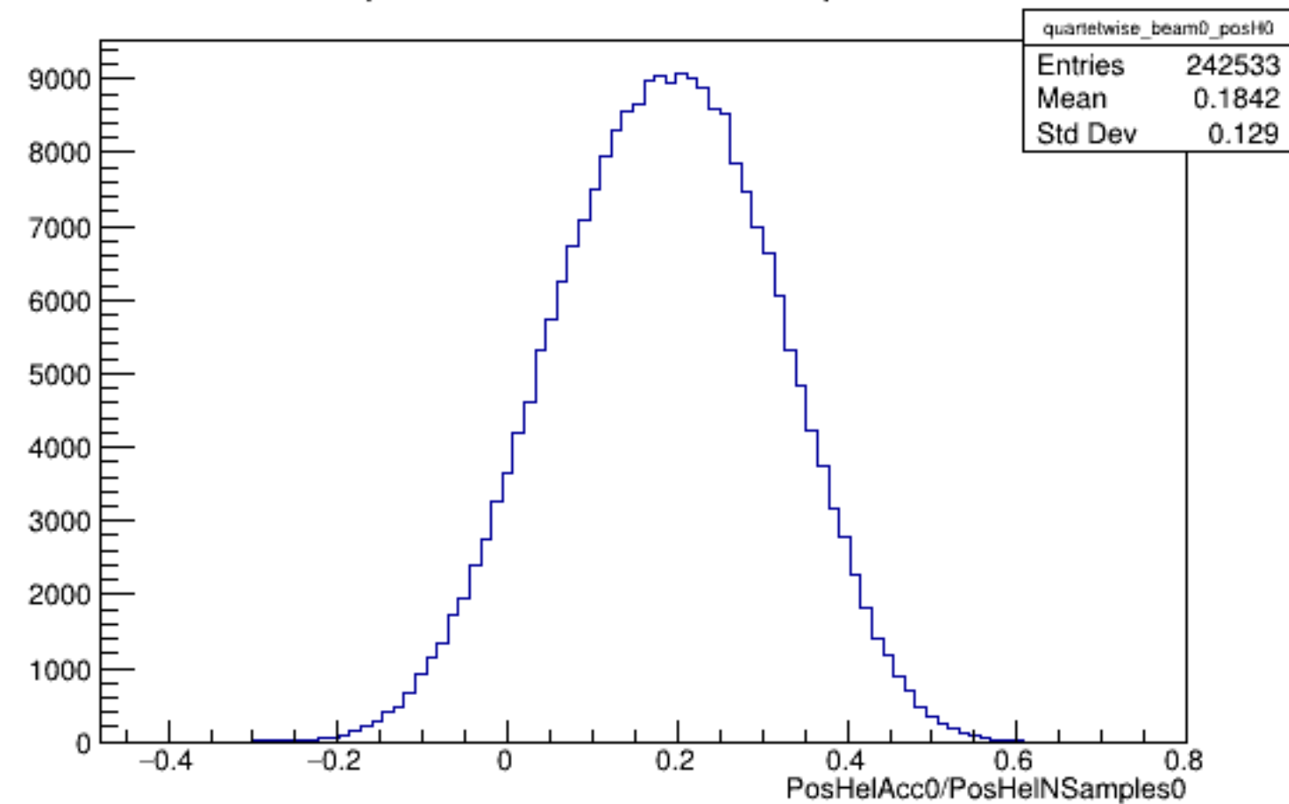
Run 6228 quartetwise, PosHelAcc0/NSamples0: Beam OFF
