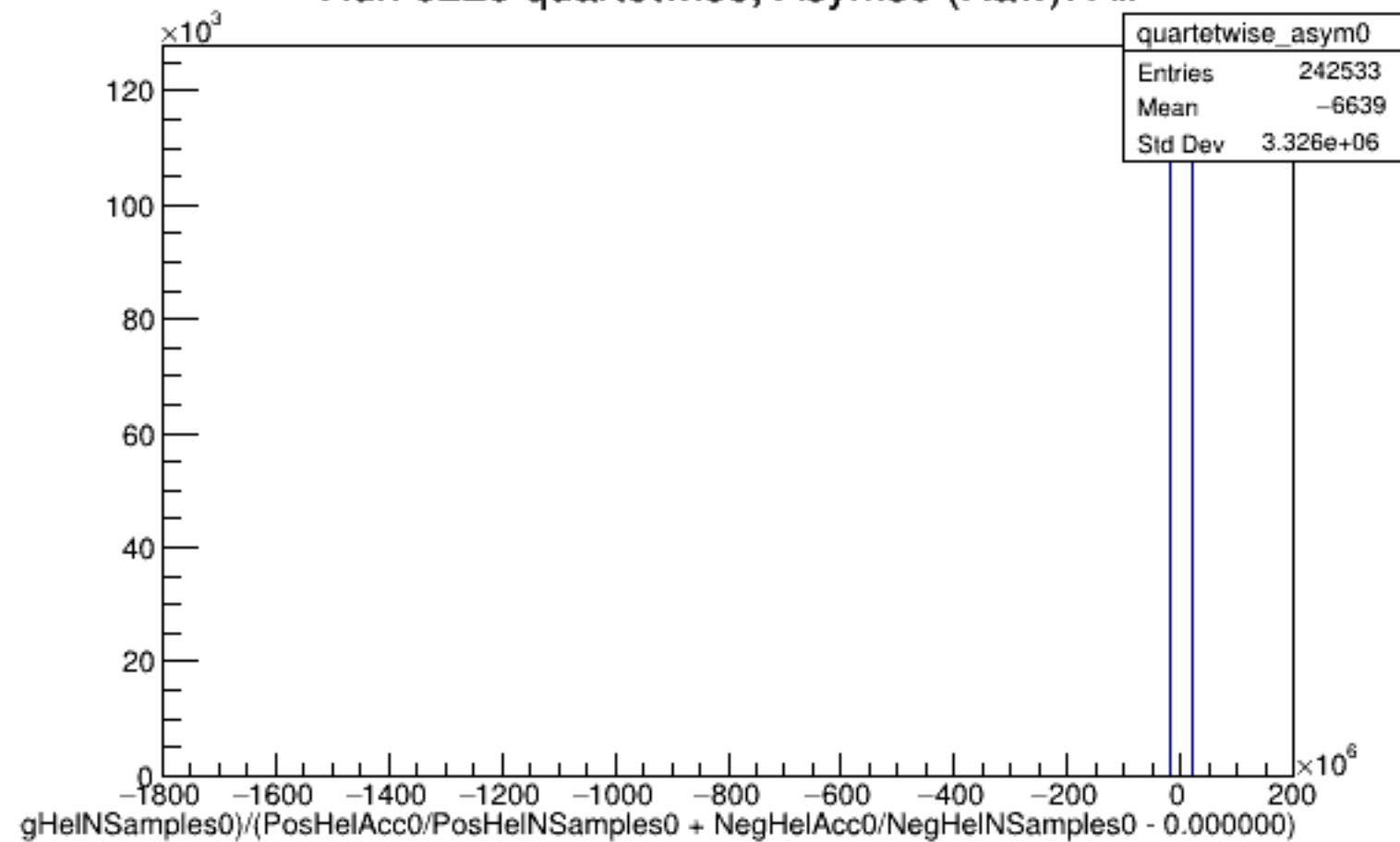
Run 6228 quartetwise, Asyms0 (Raw): All
