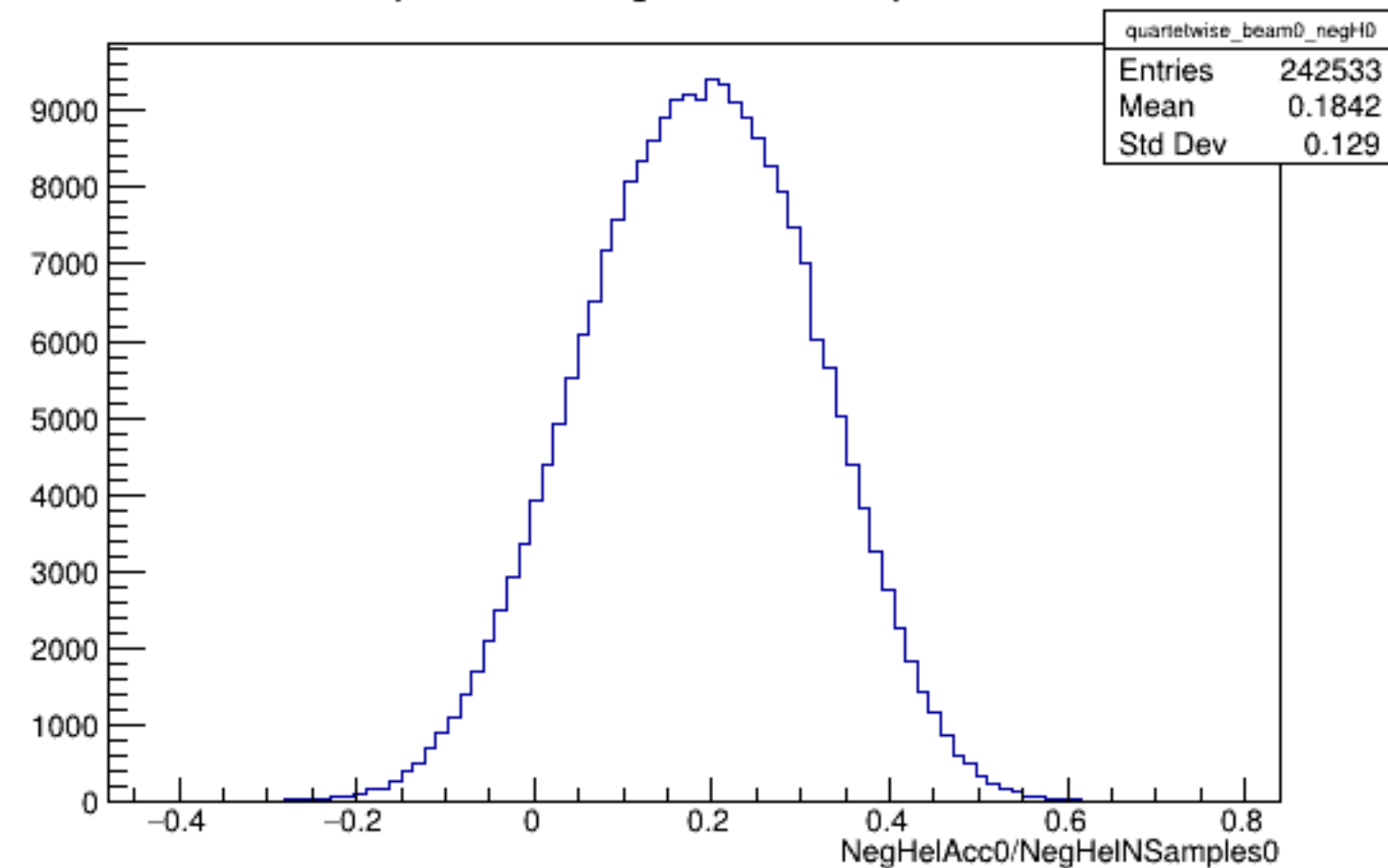
Run 6228 quartetwise, NegHelAcc0/NSamples0: Beam OFF
