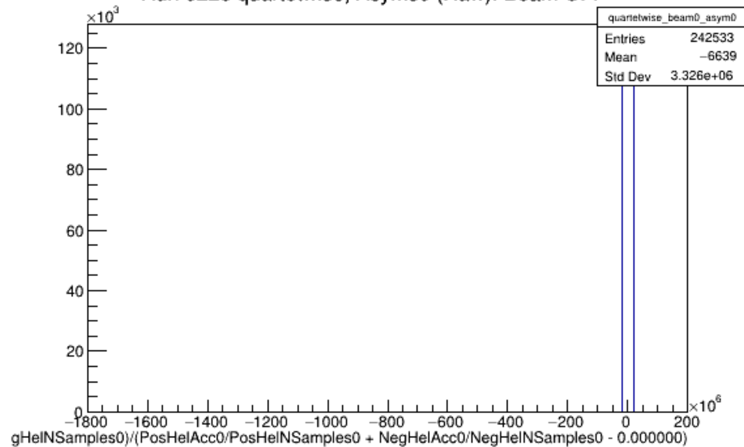
Run 6228 quartetwise, Asyms0 (Raw): Beam OFF
