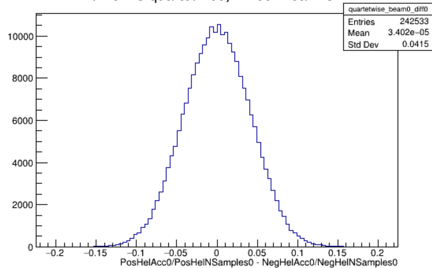
Run 6228 quartetwise, Diffs0: Beam OFF
