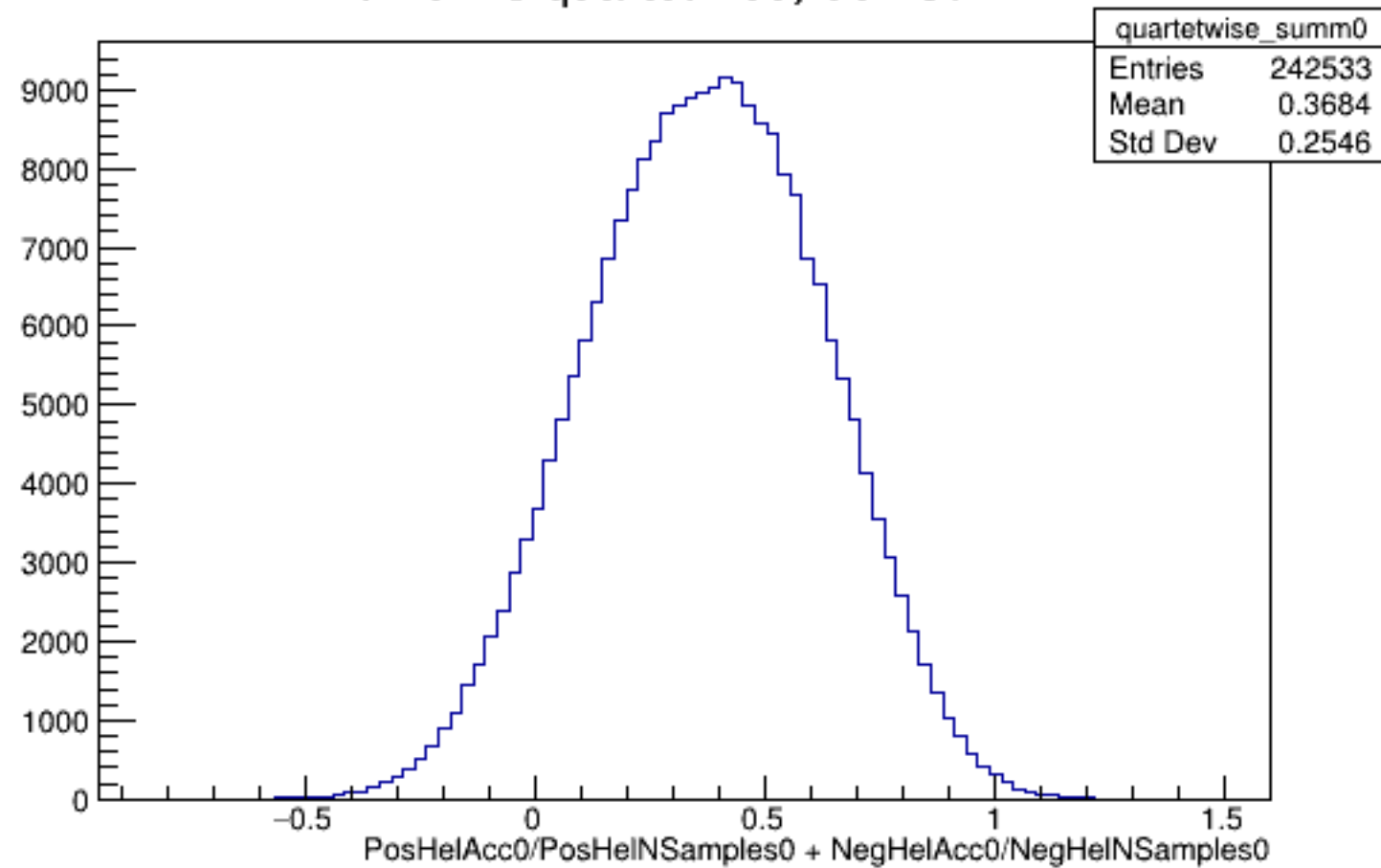
Run 6228 quartetwise, Sums0: All
