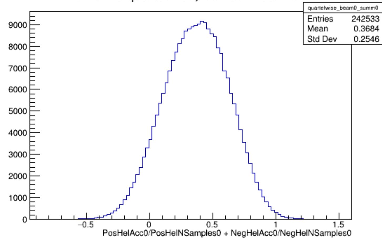
Run 6228 quartetwise, Sums0: Beam OFF
