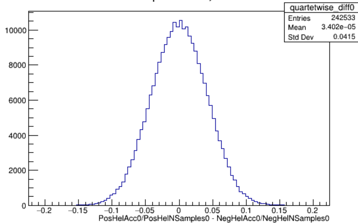
Run 6228 quartetwise, Diffs0: All
