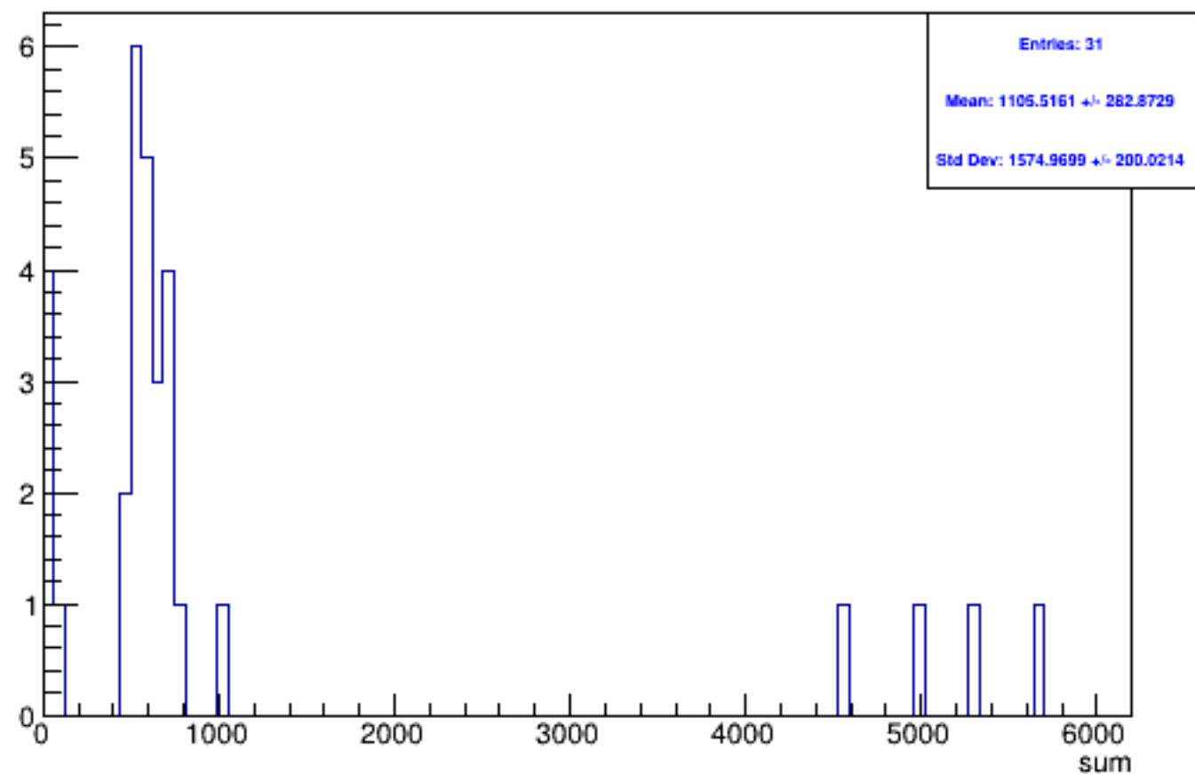
Run 6228 triggerwise, sums: All
