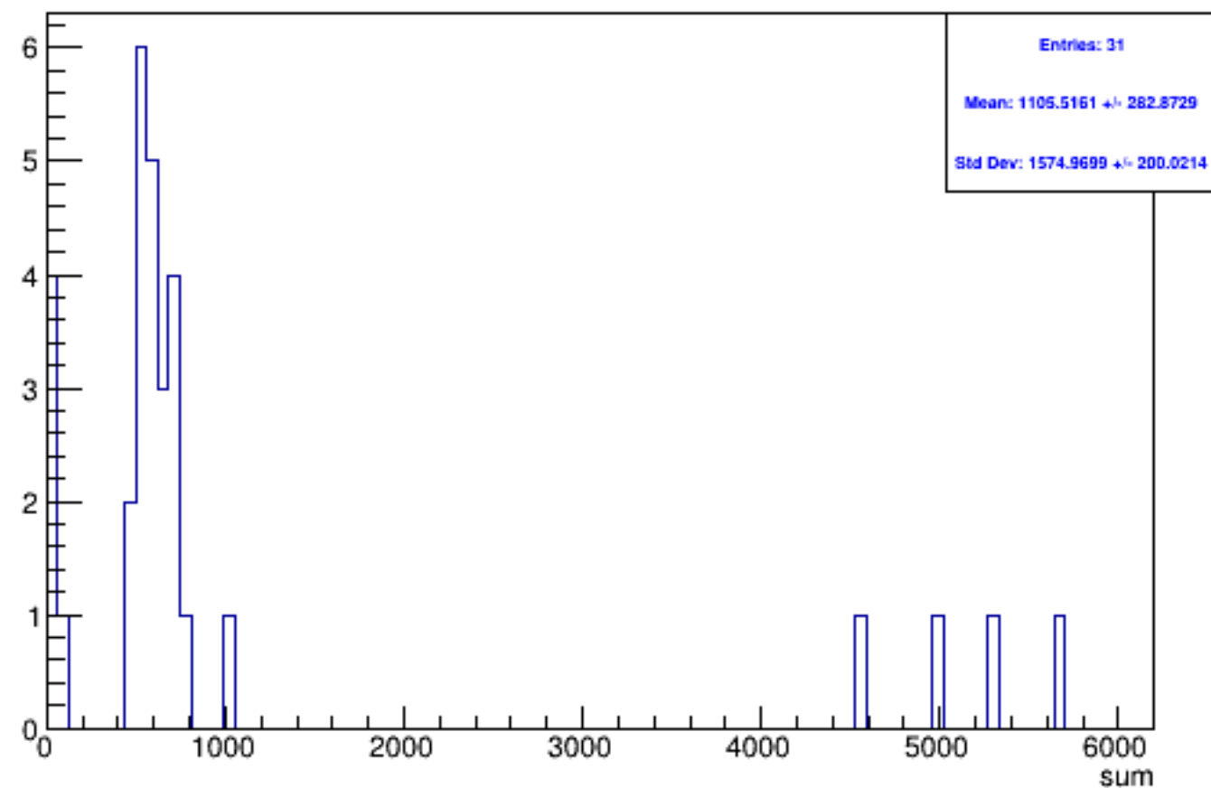
Run 6228 triggerwise, sums: Beam OFF
