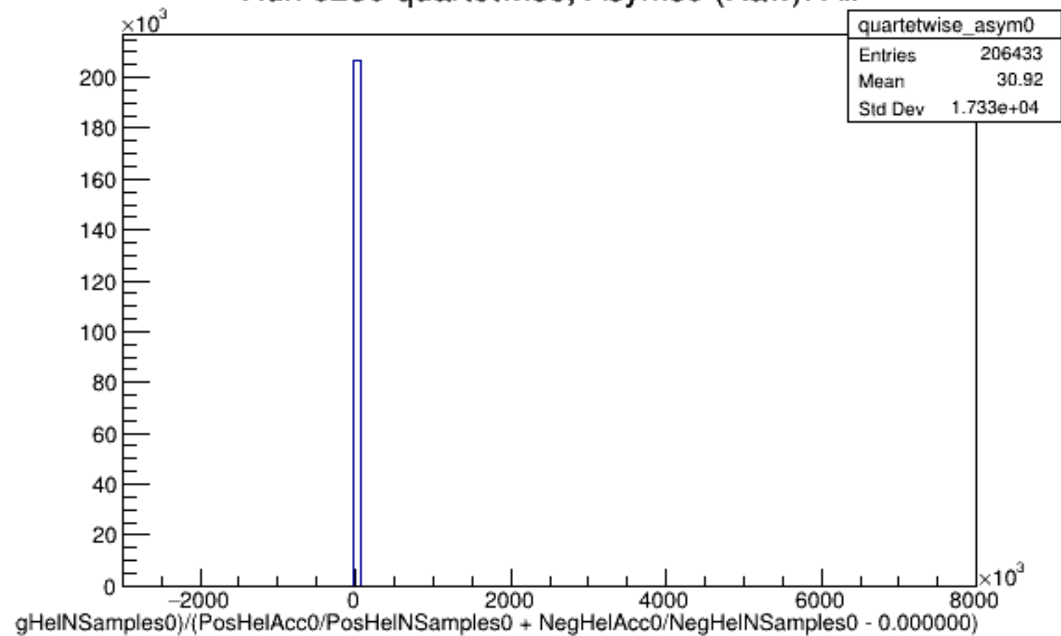
Run 6230 quartetwise, Asyms0 (Raw): All
