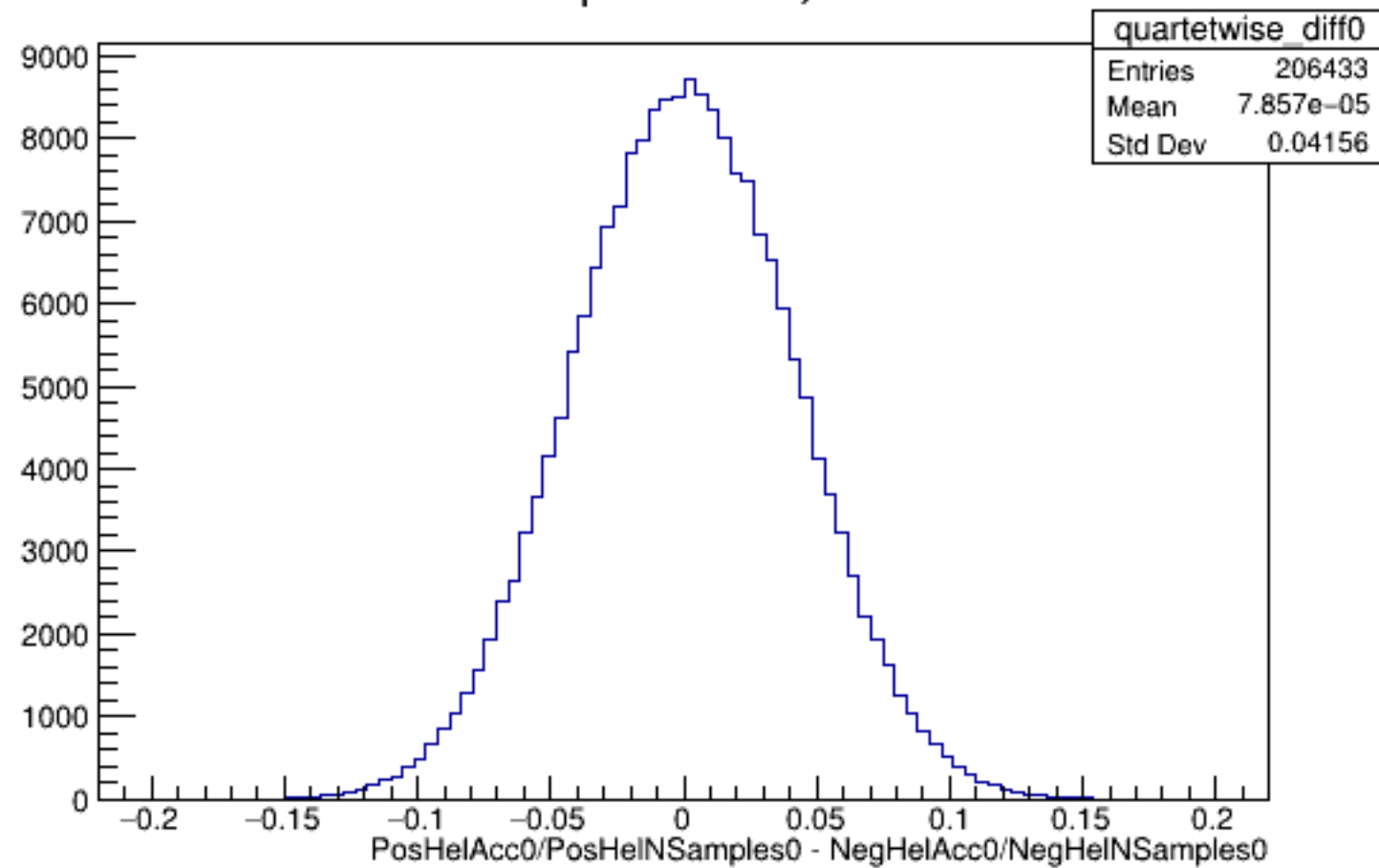
Run 6230 quartetwise, Diffs0: All
