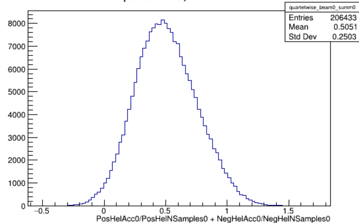
Run 6230 quartetwise, Sums0: Beam OFF
