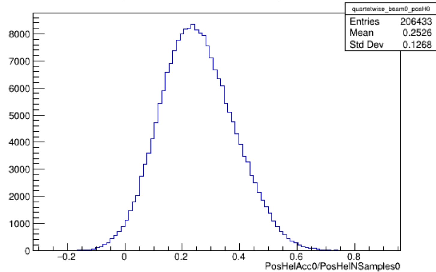
Run 6230 quartetwise, PosHelAcc0/NSamples0: Beam OFF
