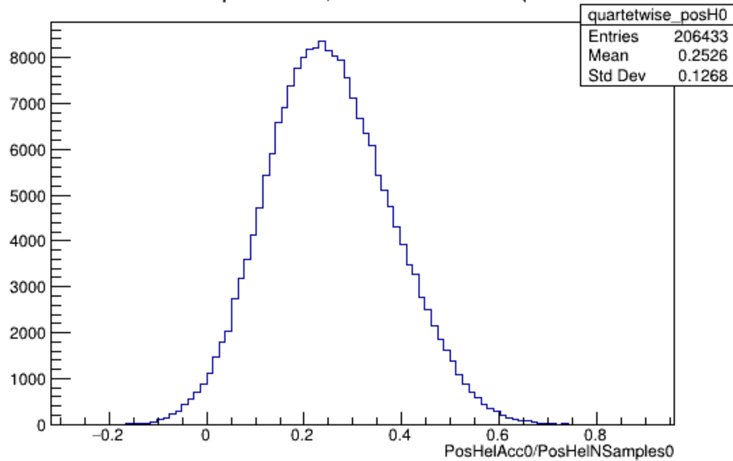
Run 6230 quartetwise, PosHelAcc0/NSamples0: All
