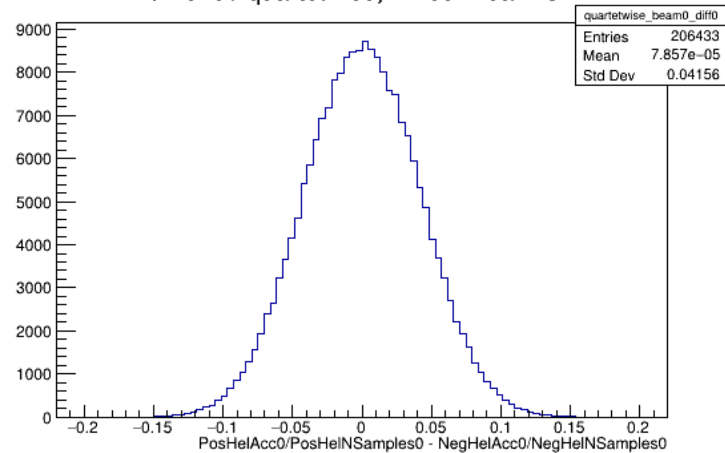
Run 6230 quartetwise, Diffs0: Beam OFF
