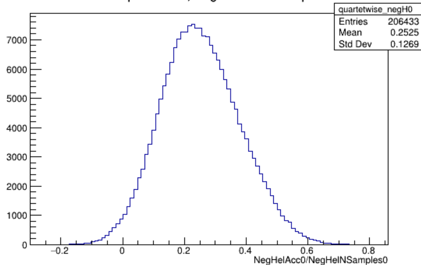
Run 6230 quartetwise, NegHelAcc0/NSamples0: All
