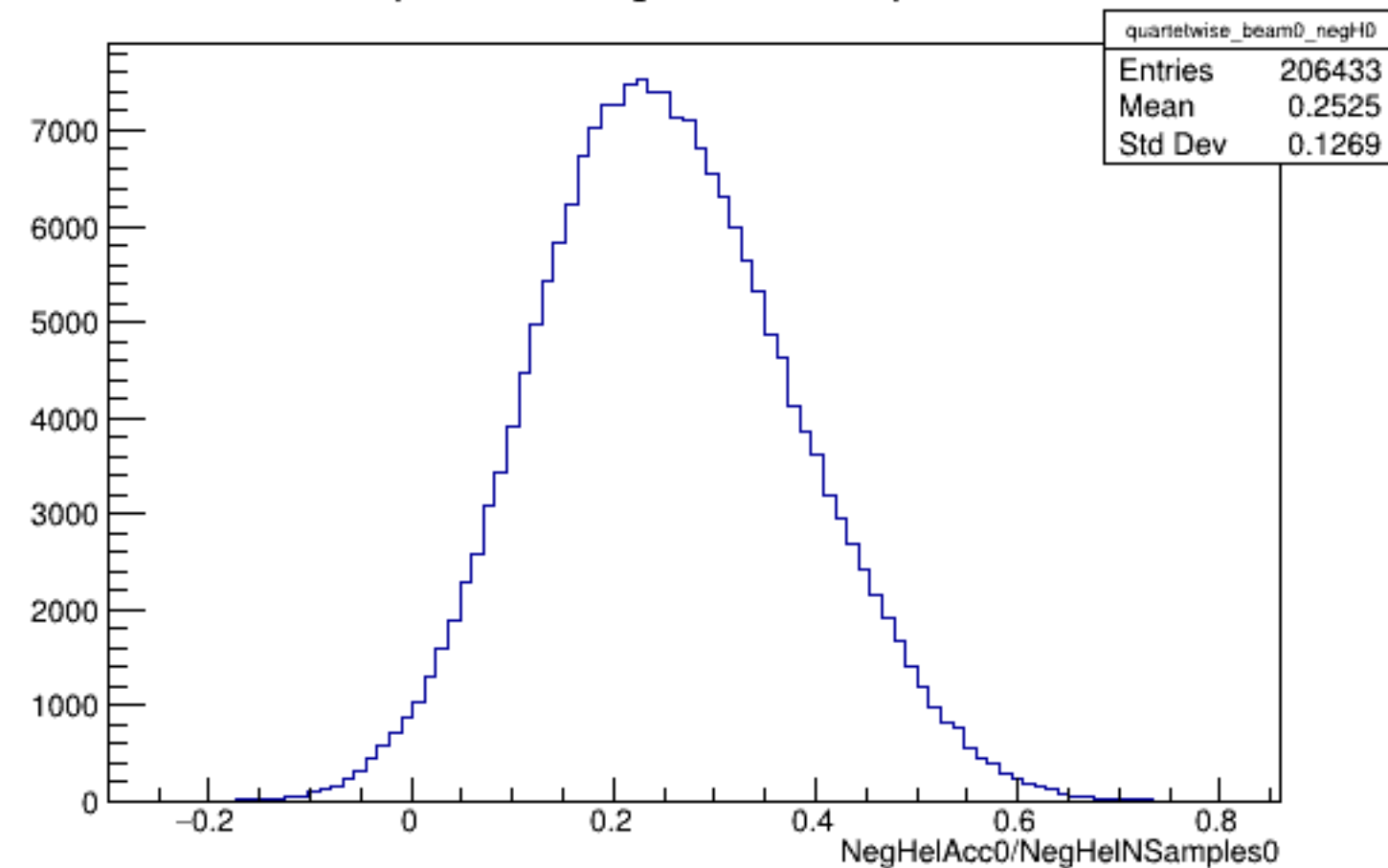
Run 6230 quartetwise, NegHelAcc0/NSamples0: Beam OFF
