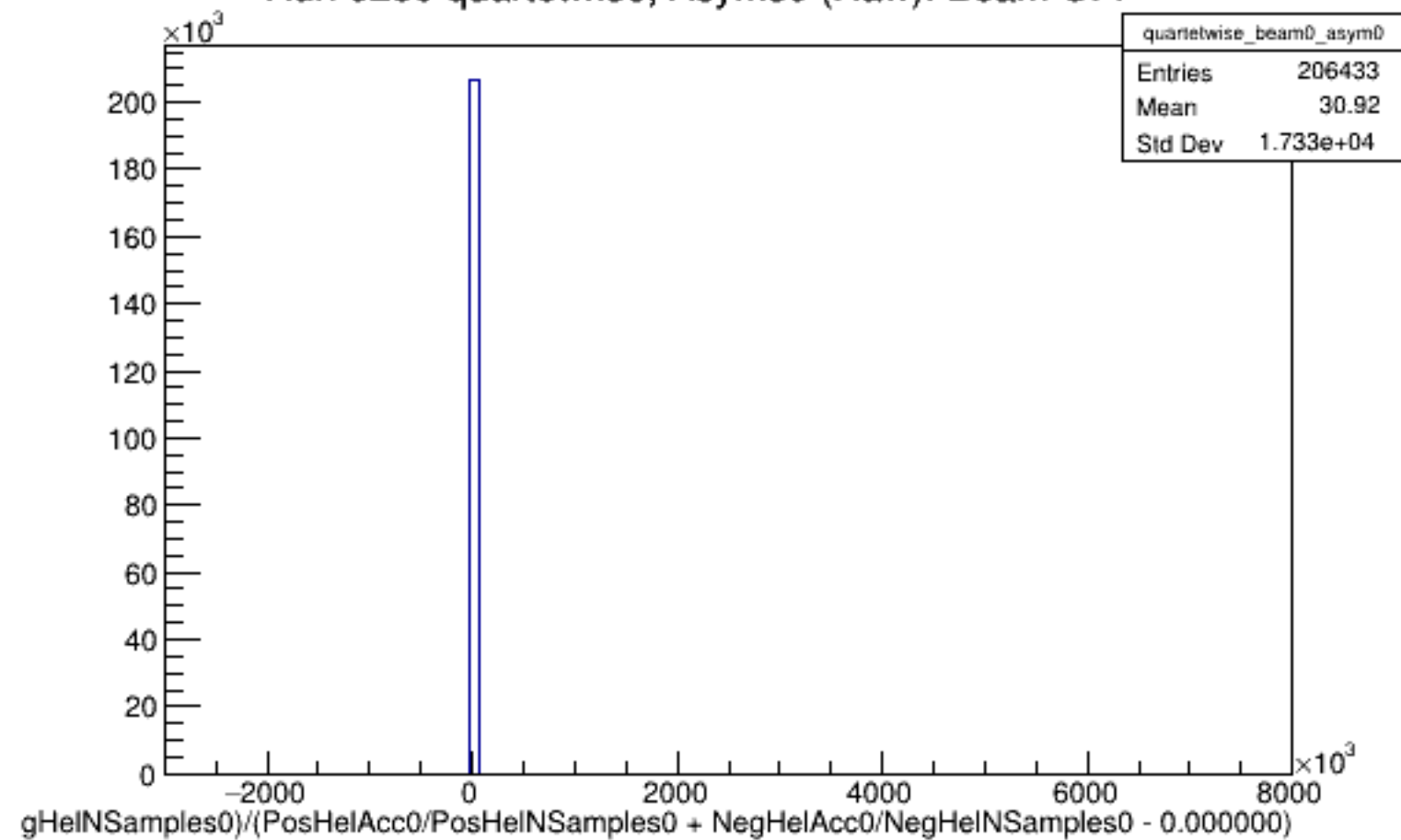
Run 6230 quartetwise, Asyms0 (Raw): Beam OFF
