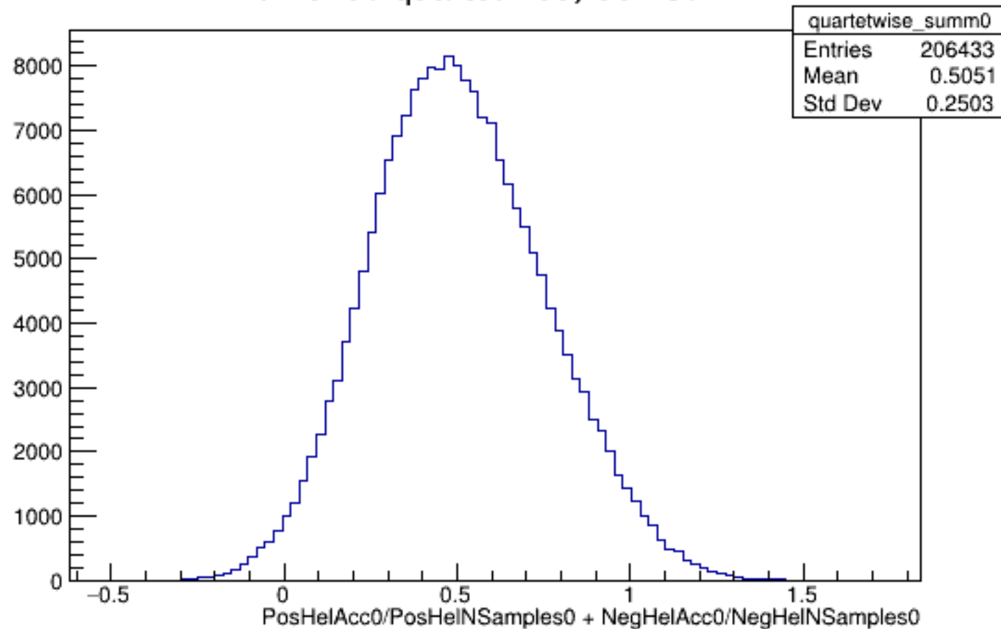
Run 6230 quartetwise, Sums0: All
