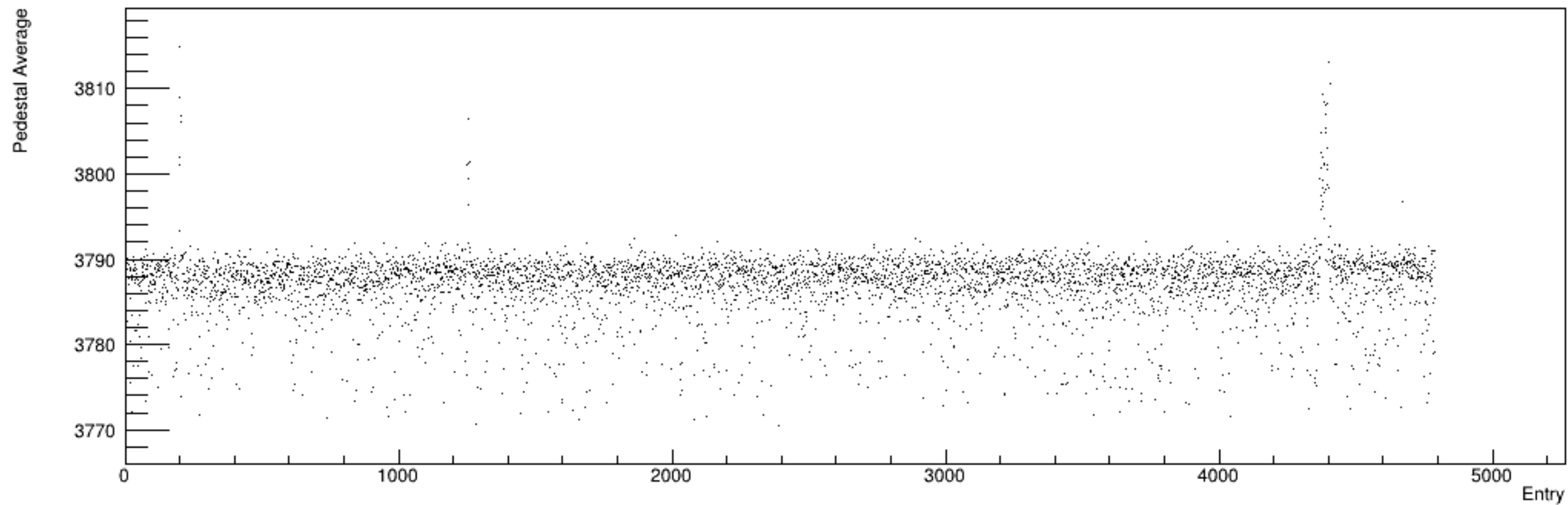
Run 6232, snapshots: Pedestal vs. Time
