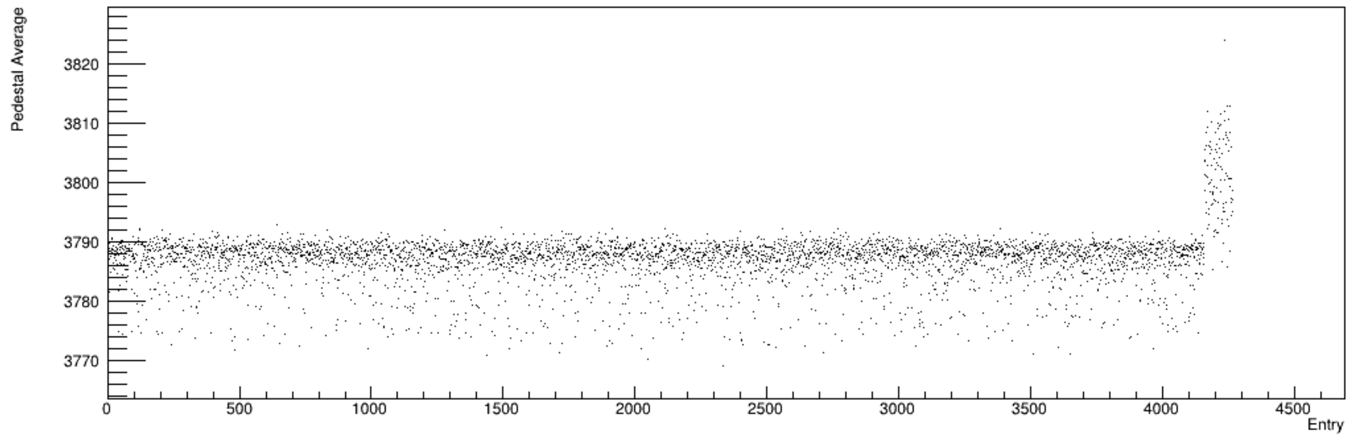
Run 6233, snapshots: Pedestal vs. Time
