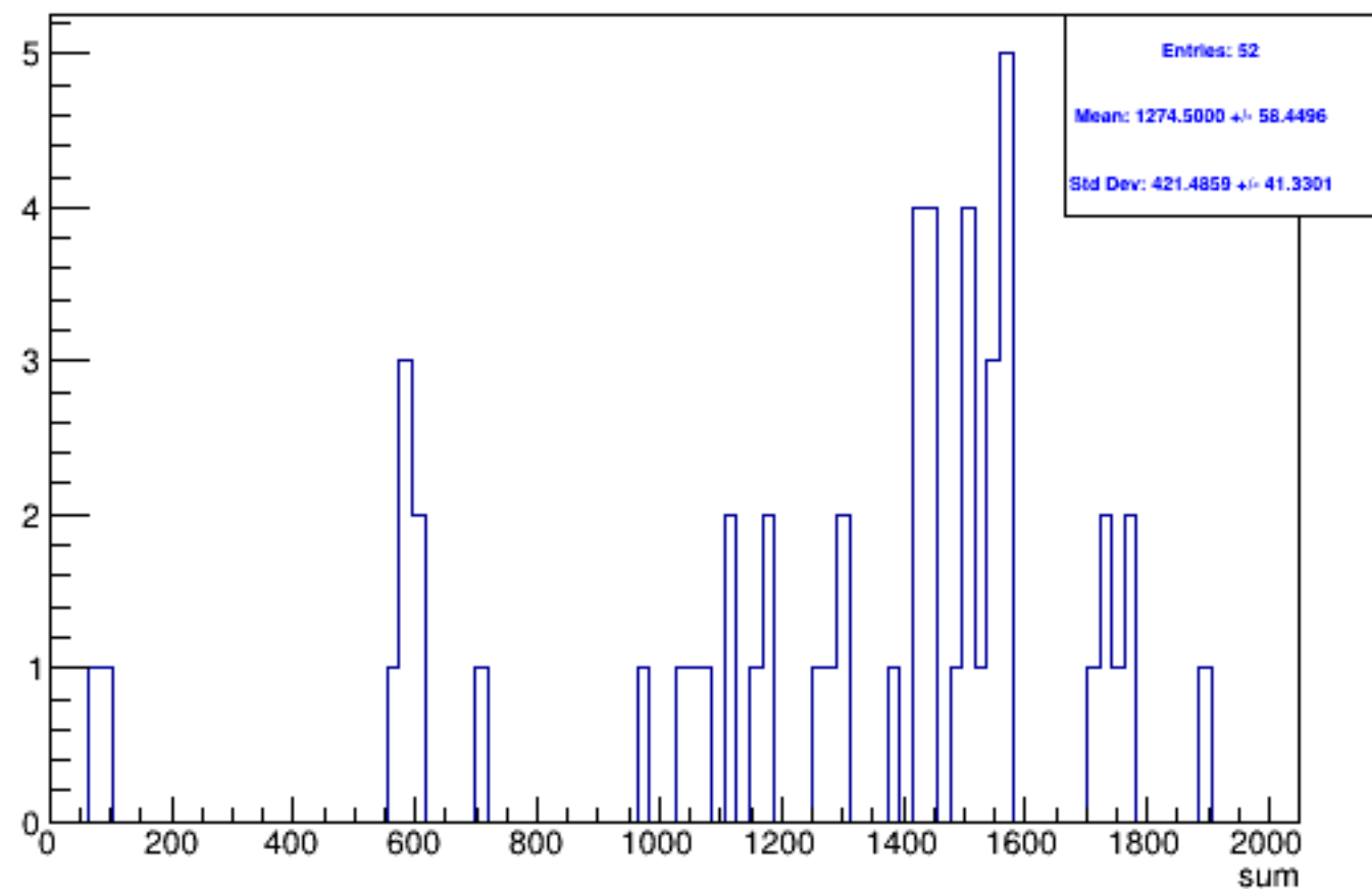
Run 6236 triggerwise, sums: All
