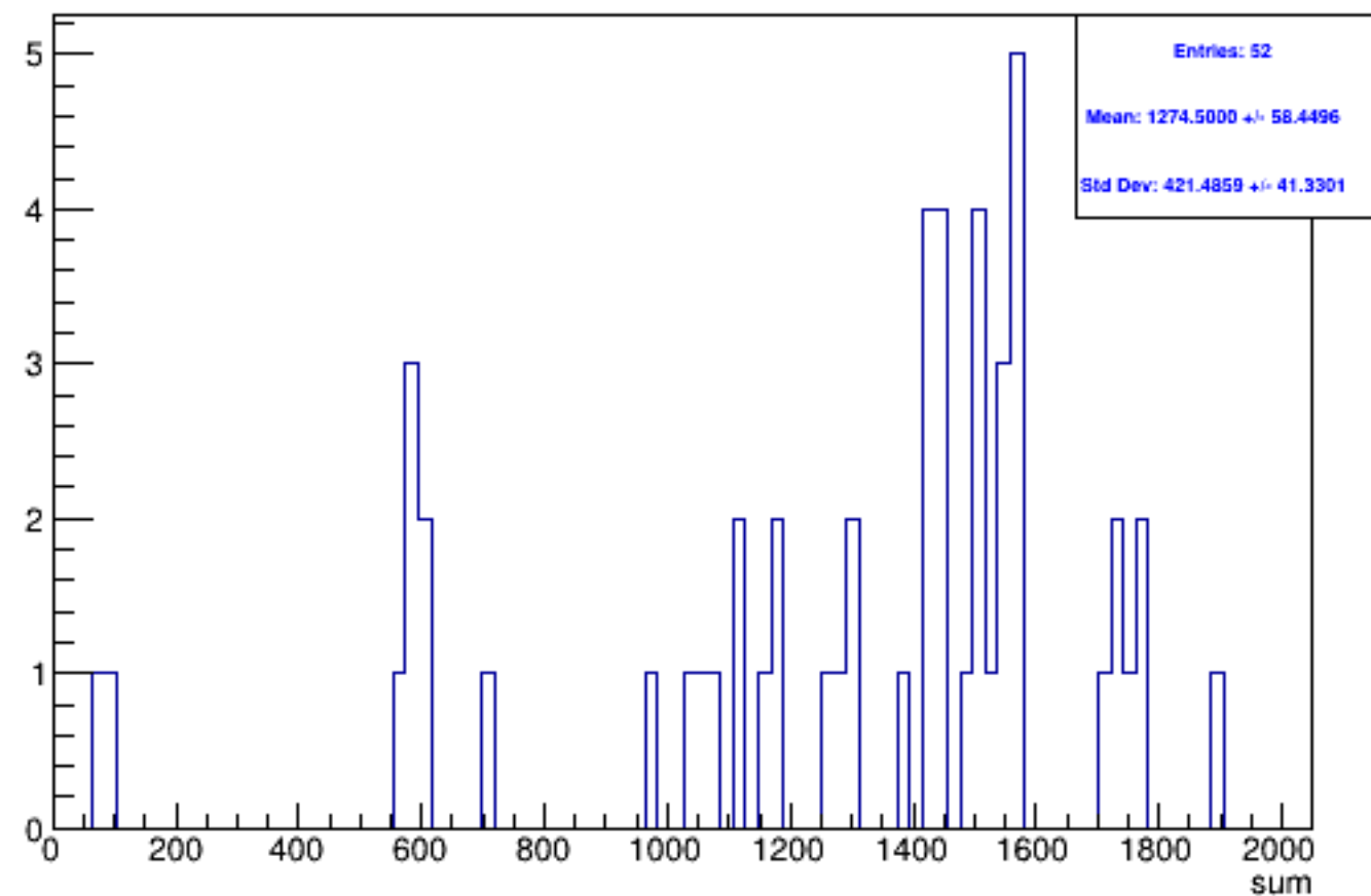
Run 6236 triggerwise, sums: Beam OFF
