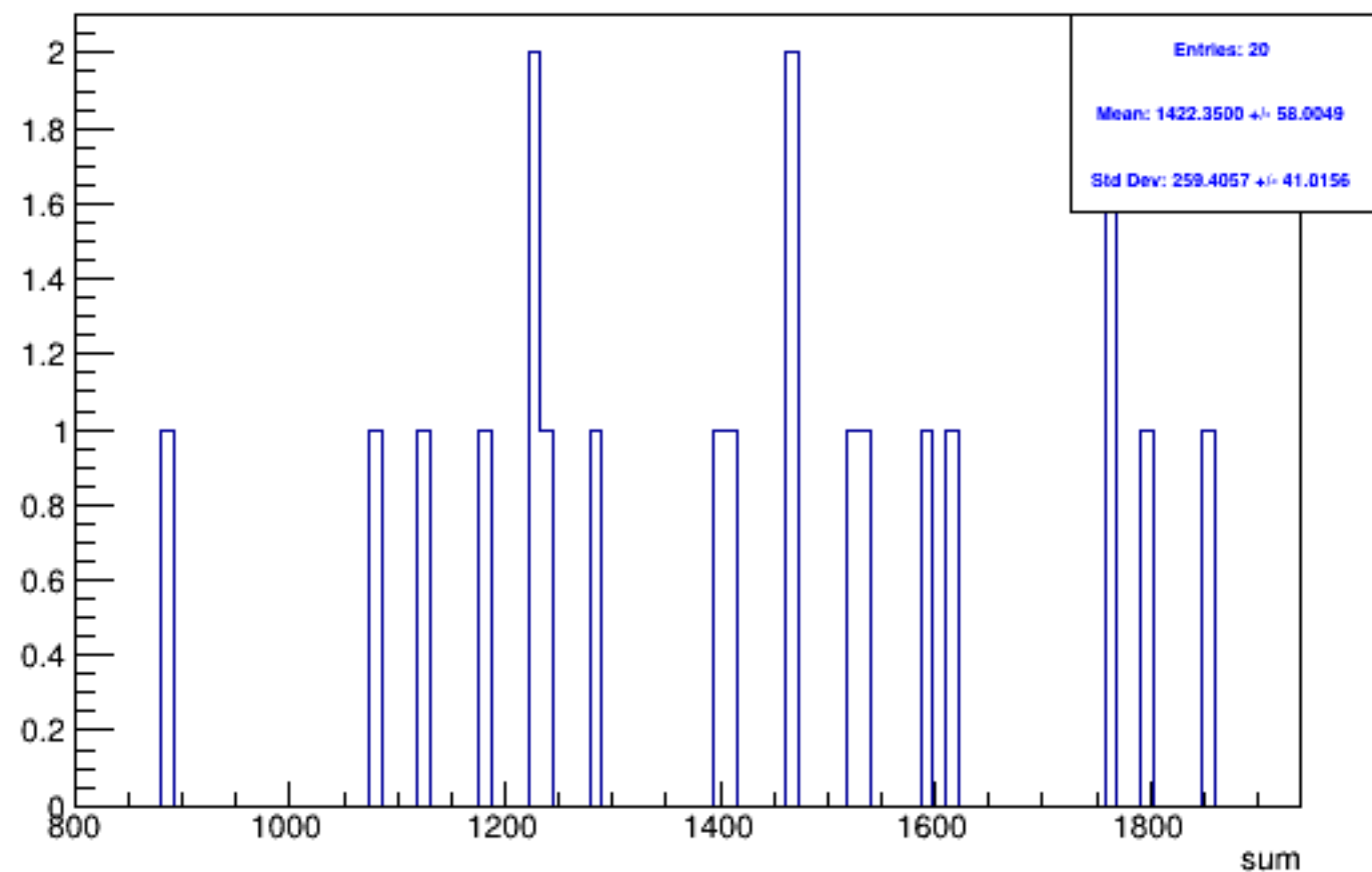
Run 6237 triggerwise, sums: All
