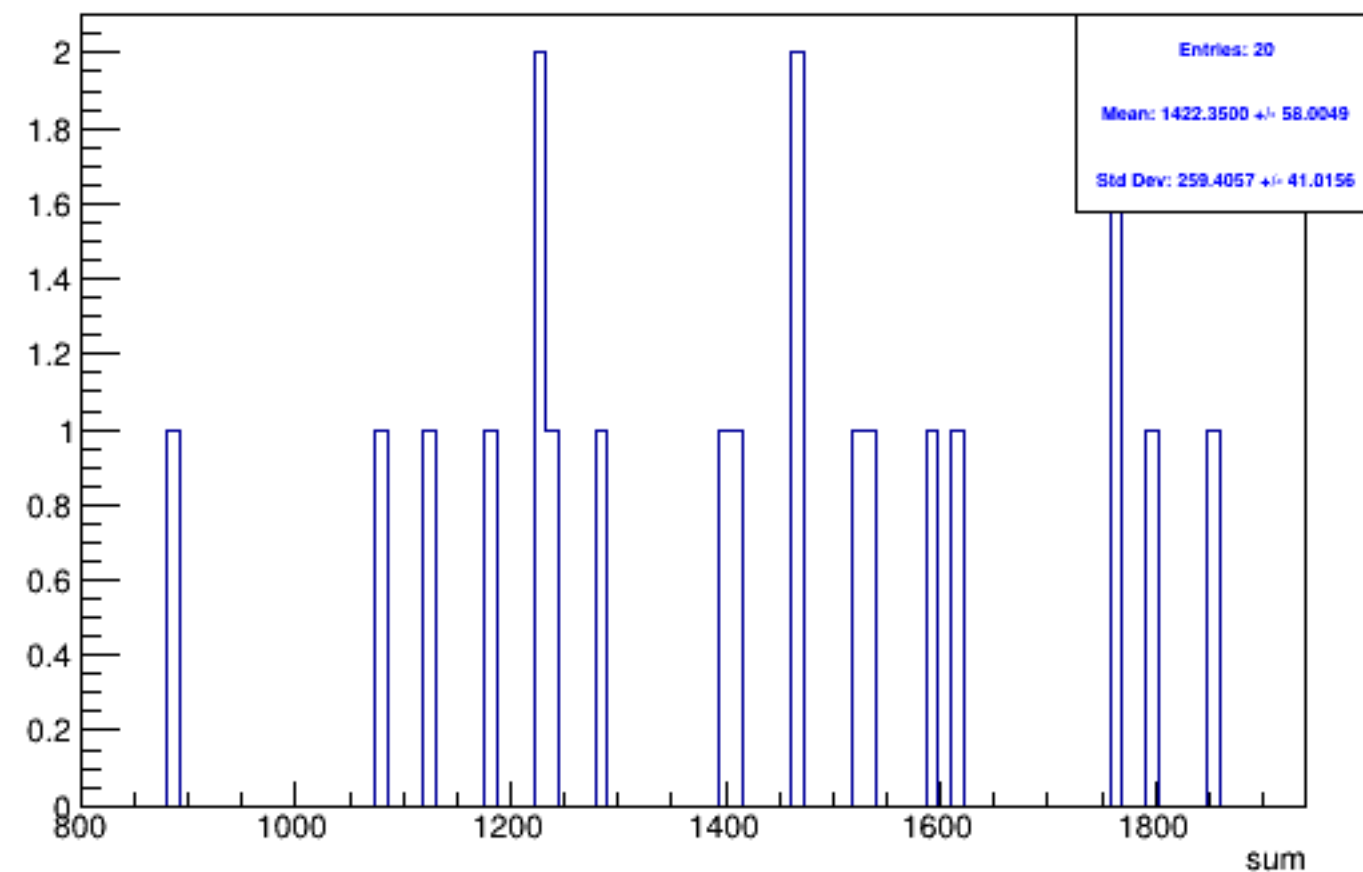
Run 6237 triggerwise, sums: Beam OFF
