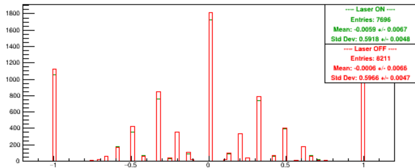
Run 6241 quartetwise, Asyms USbg1
