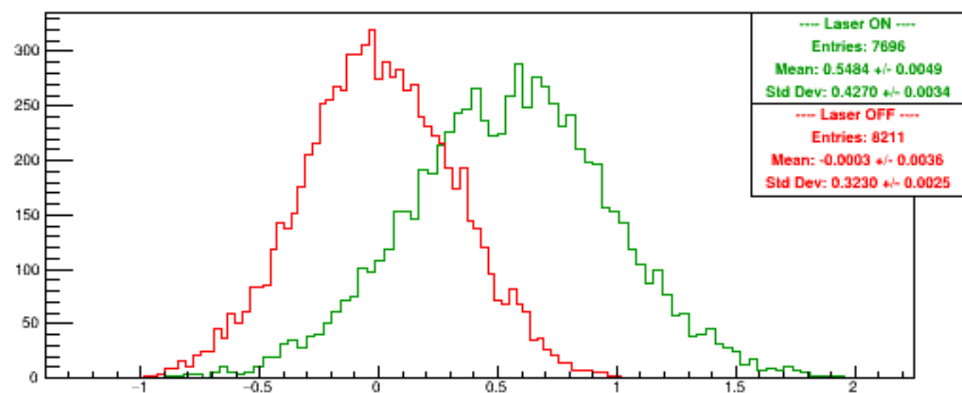
Run 6241 quartetwise, Diffs0
