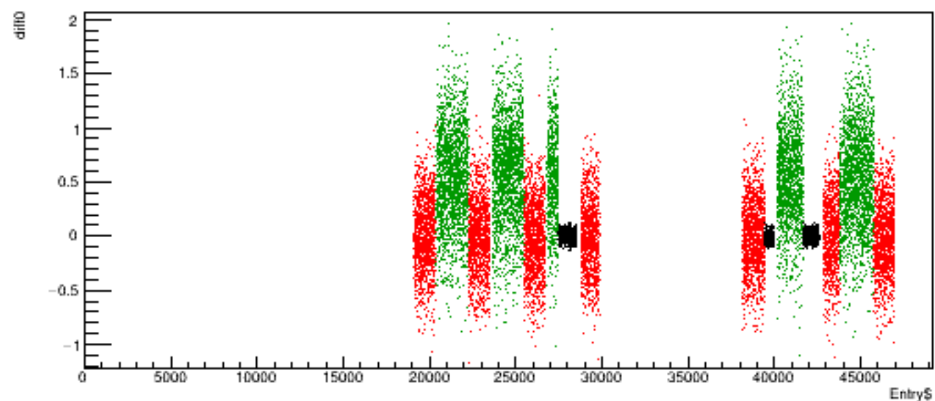
Run 6241 quartetwise, diff0 vs time
