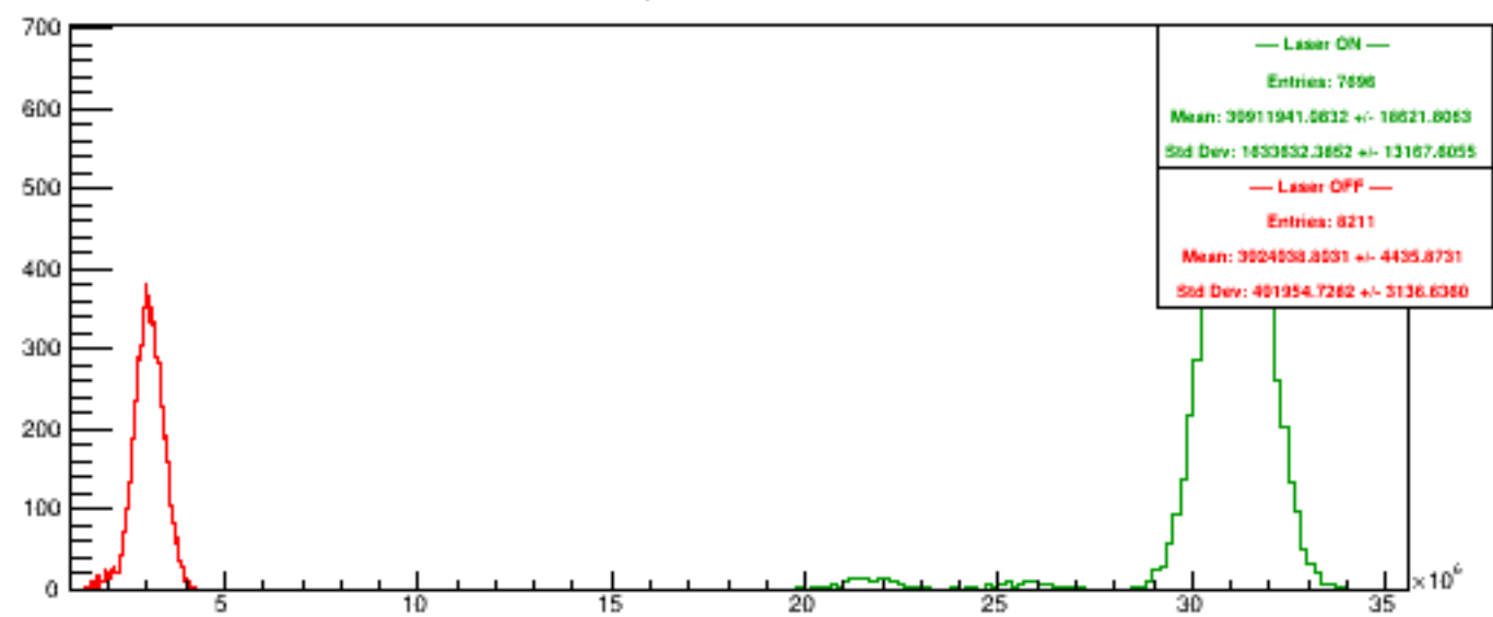
Run 6241 quartetwise, PosHelAcc4
