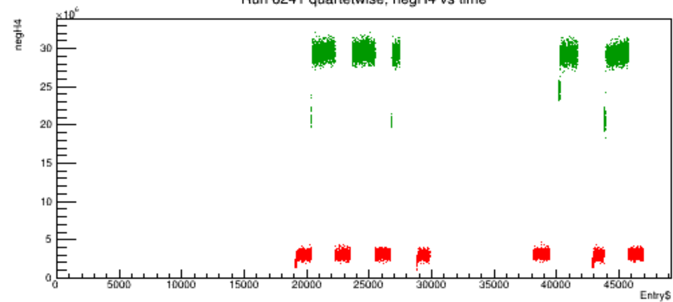
Run 6241 quartetwise, negH4 vs time
