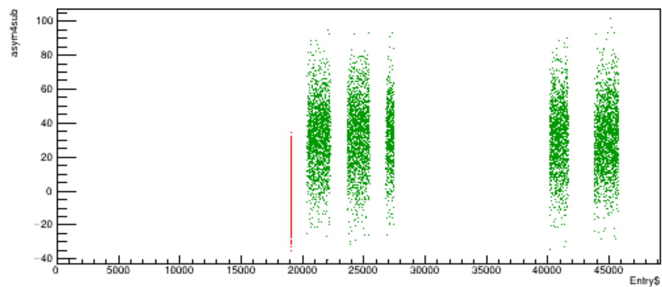
Run 6241 quartetwise, asym4sub vs time
