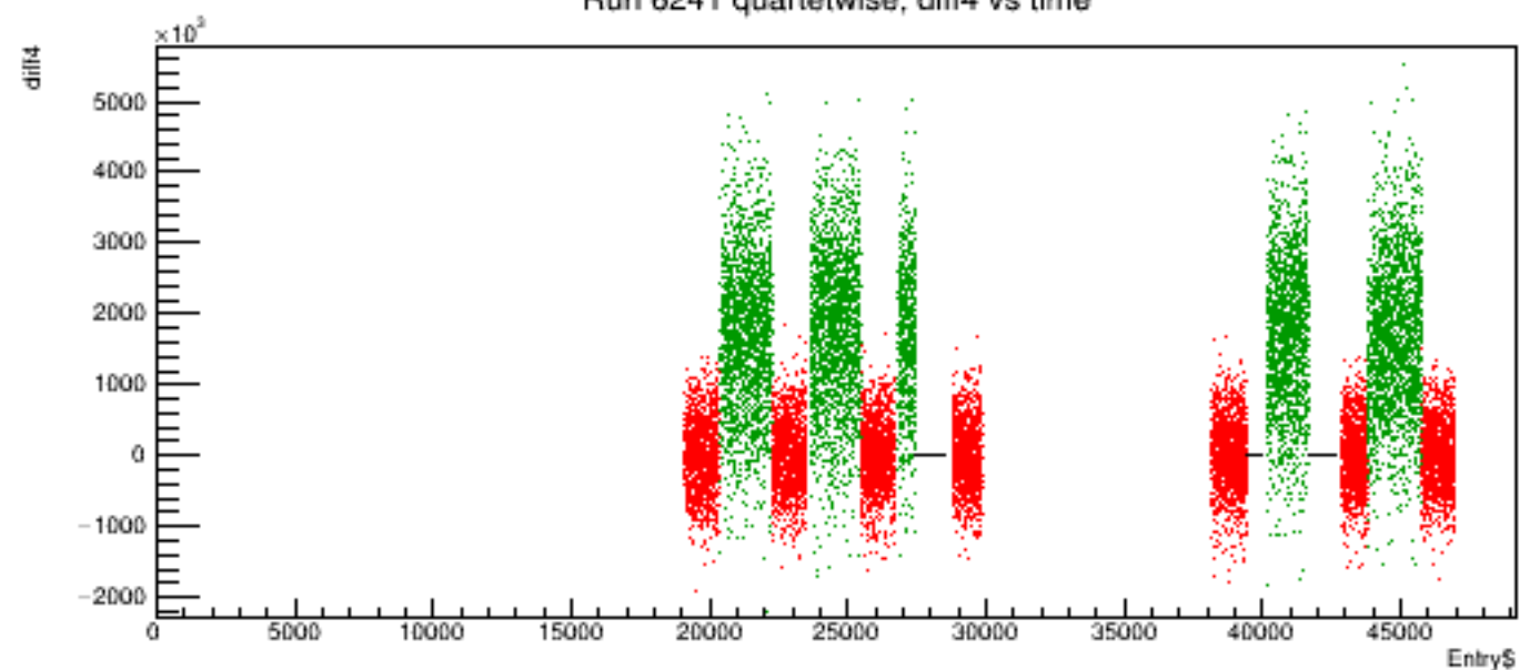
Run 6241 quartetwise, diff4 vs time
