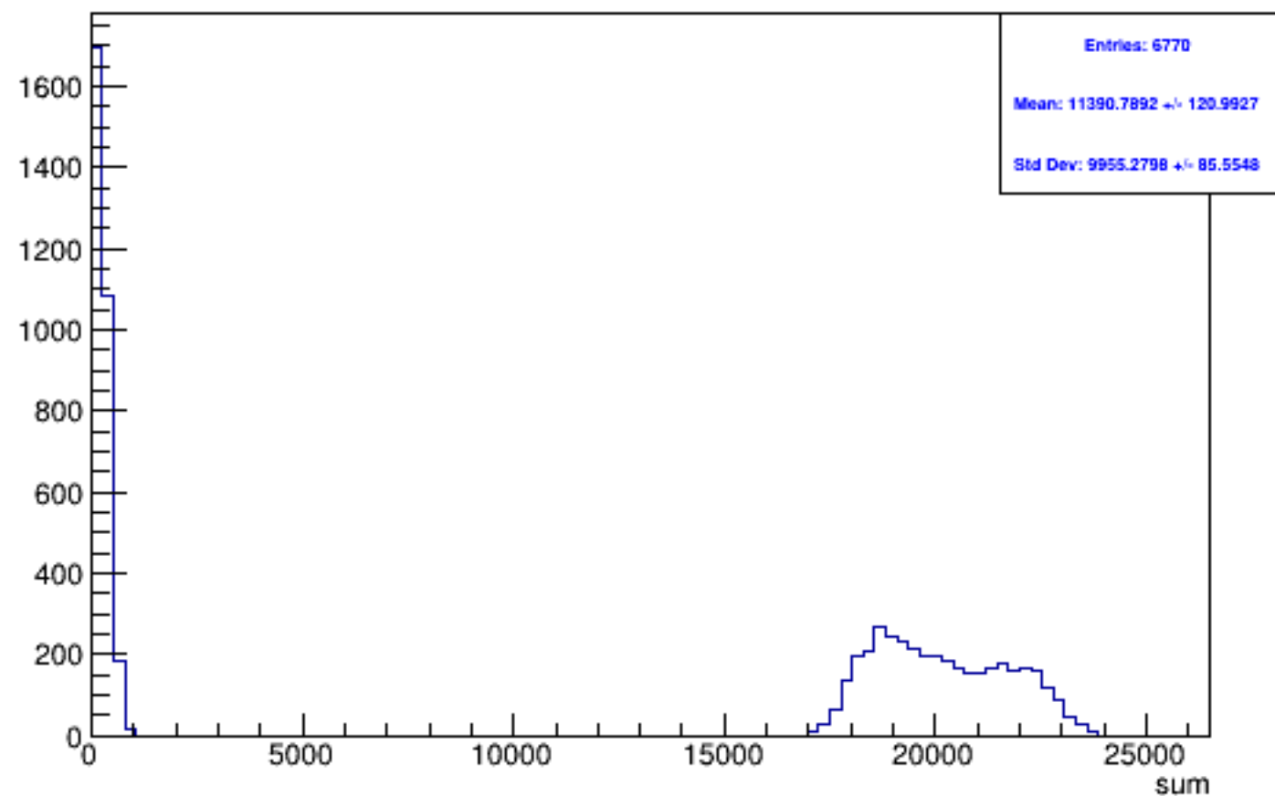
Run 6259 triggerwise, sums: All
