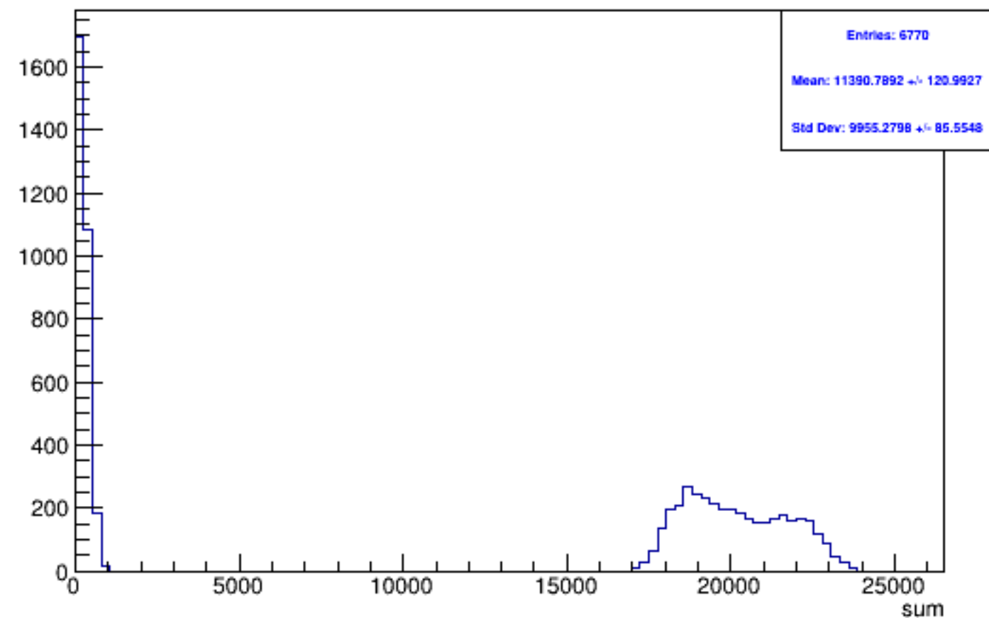
Run 6259 triggerwise, sums: Beam OFF
