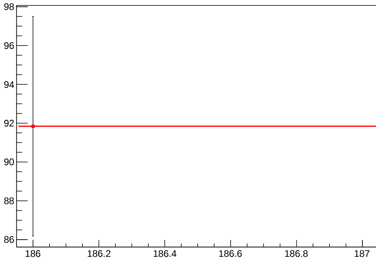
reg_asym_sam_3748_avg_diff_bpm4eY_slope vs Slug
