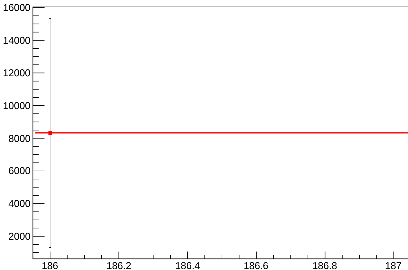
asym_sam_2468_avg_correction_mean vs Slug
