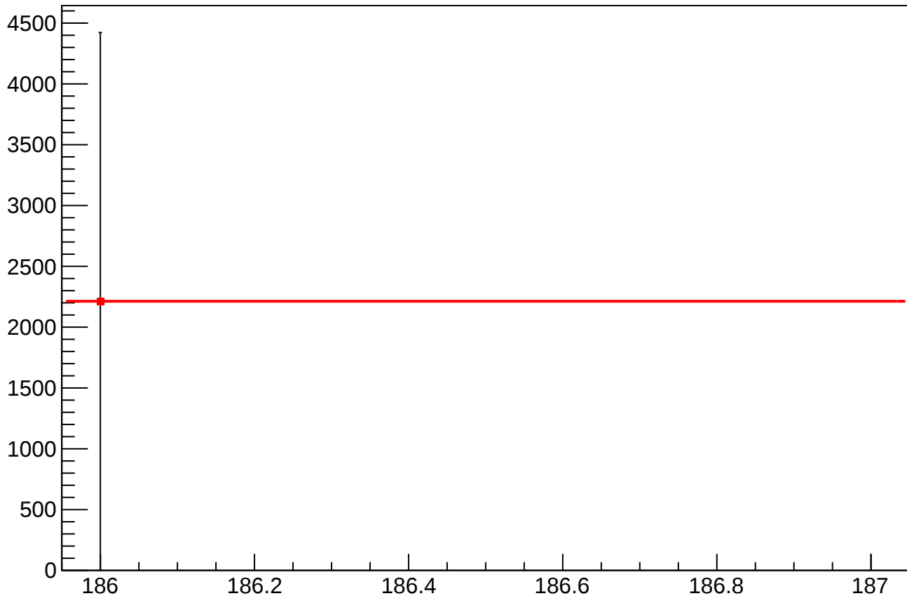
asym_sam_1526_avg_correction_mean vs Slug
