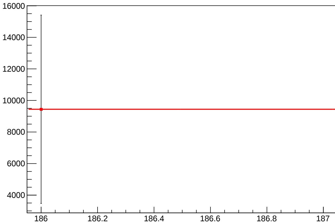
asym_sam_37_48_dd_mean vs Slug
