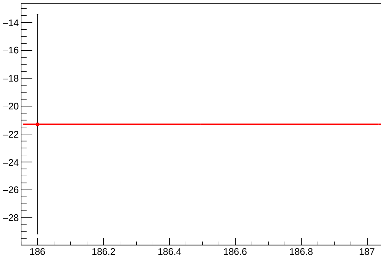
reg_asym_sam_26_dd_diff_bpm4aY_slope vs Slug
