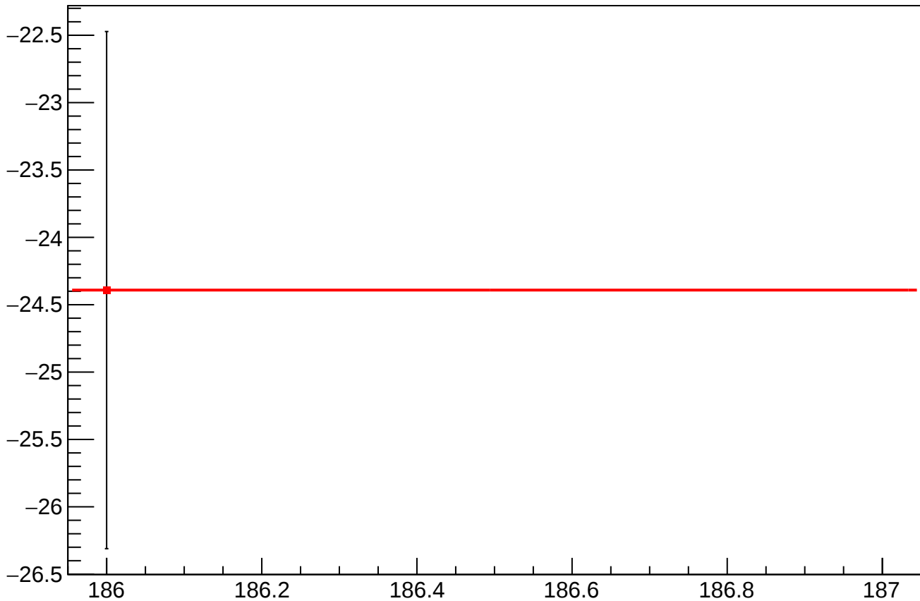
reg_asym_sam_37_48_dd_diff_bpm1X_slope vs Slug
