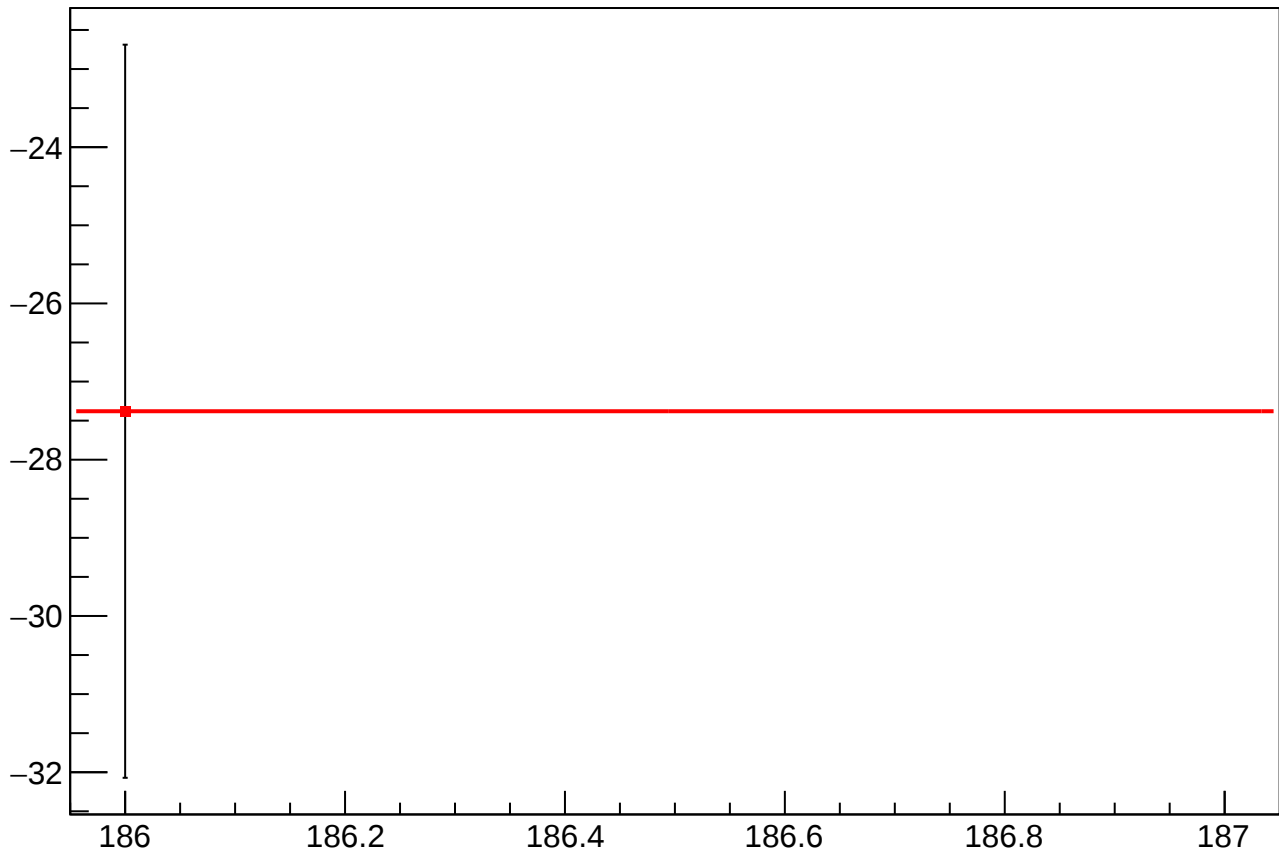
reg_asym_sam_15_dd_diff_bpm1X_slope vs Slug
