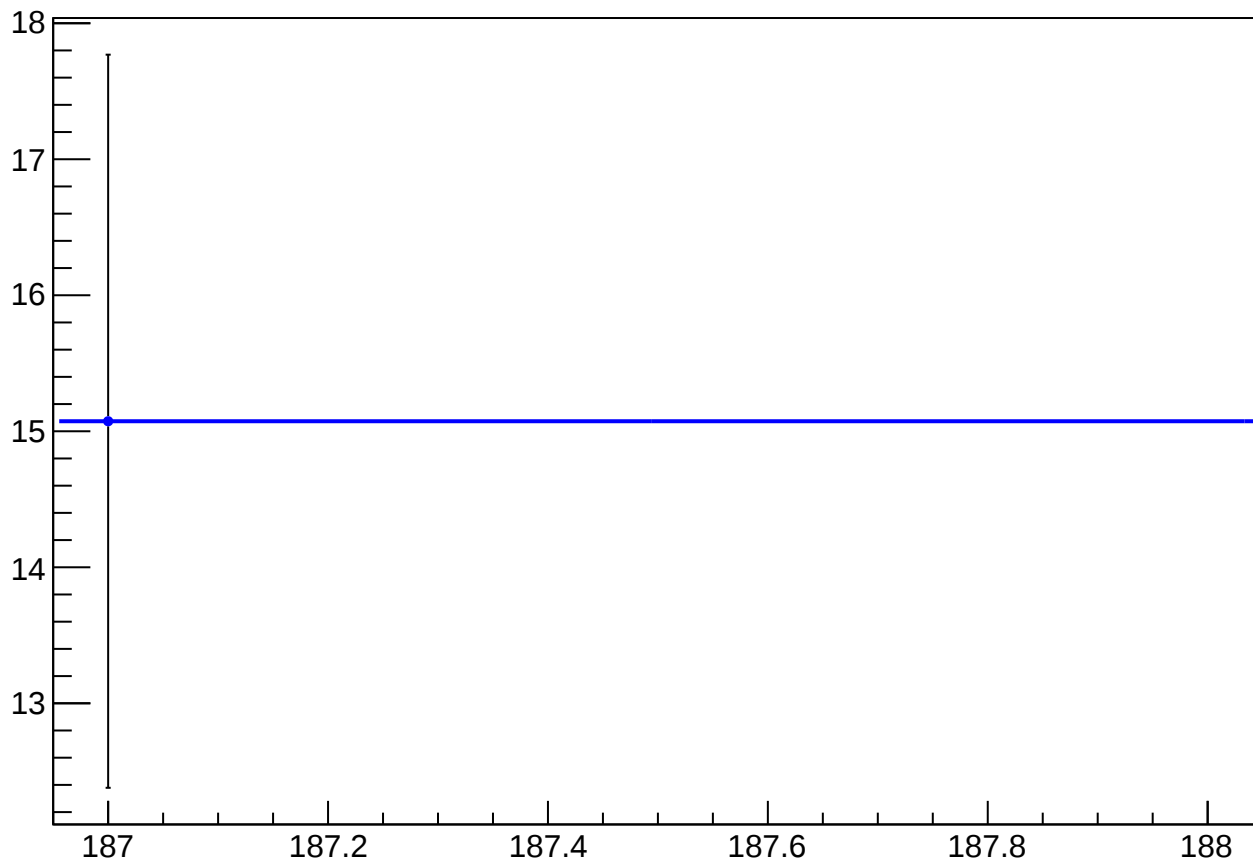
reg_asym_sam_1357_avg_diff_bpm4eY_slope vs Slug
