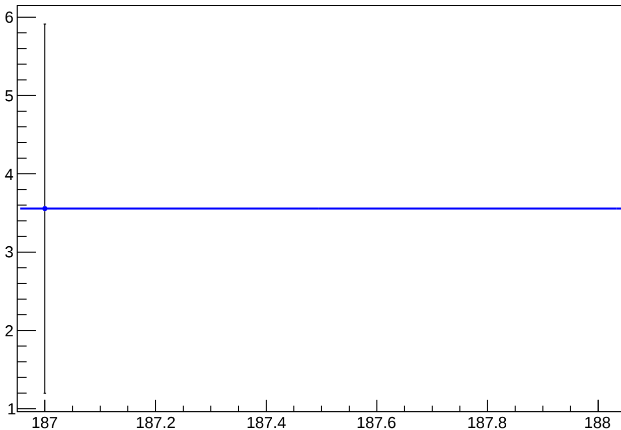
reg_asym_sam_15_48_dd_diff_bpm4aY_slope vs Slug
