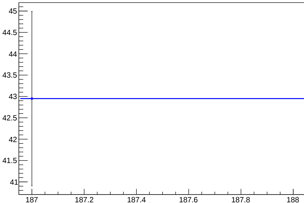
reg_asym_sam8_diff_bpm4eY_slope vs Slug
