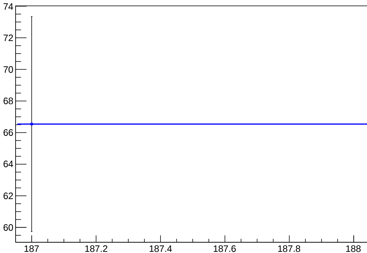
reg_asym_sam_48_dd_diff_bpm4eY_slope vs Slug
