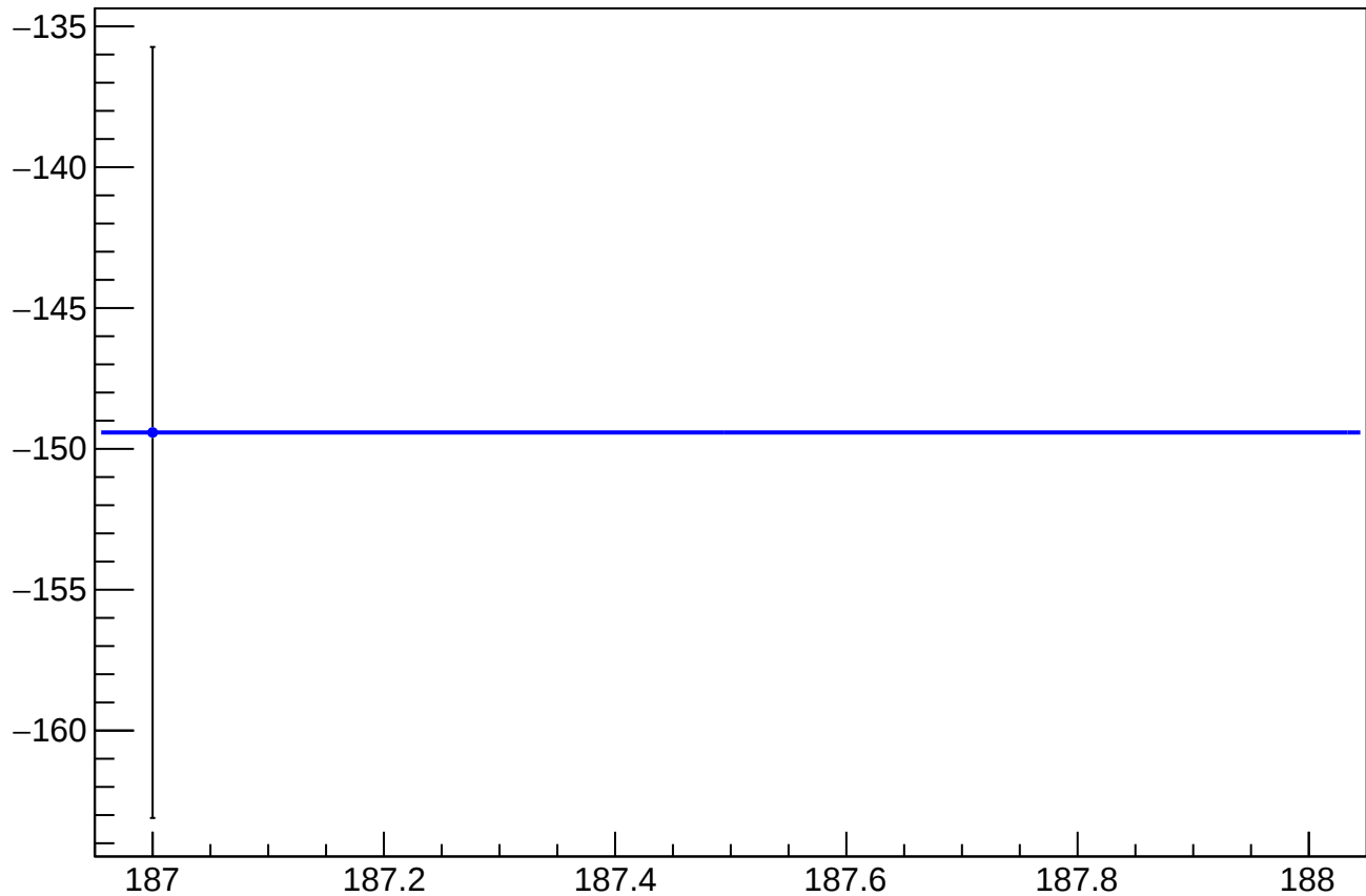
reg_asym_sam2_diff_bpm4eY_slope vs Slug
