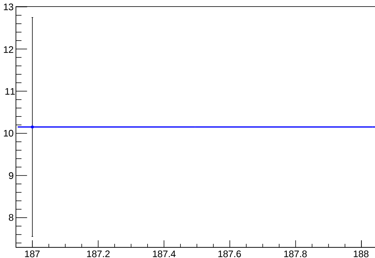
reg_asym_sam_3748_avg_diff_bpm1X_slope vs Slug
