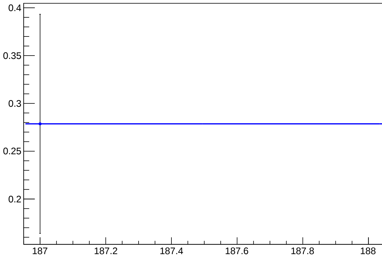
reg_asym_sam8_diff_bpm12X_slope vs Slug
