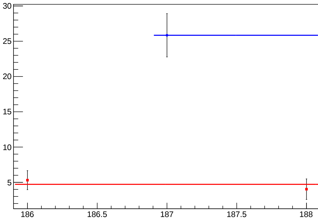
reg_asym_at1_avg_diff_bpm4aY_slope vs Slug
