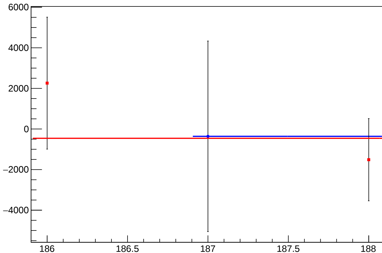
dit_asym_at1_dd_mean vs Slug
