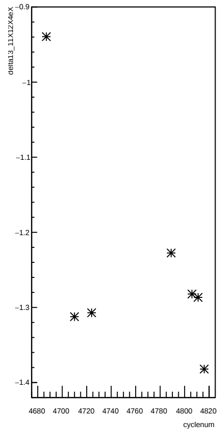
delta13_11X12X4eX:cyclenum
