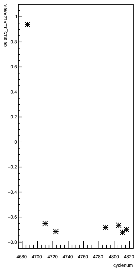
delta15_11X12X4eX:cyclenum
