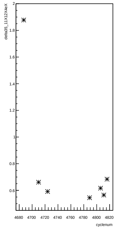
delta35_11X12X4eX:cyclenum
