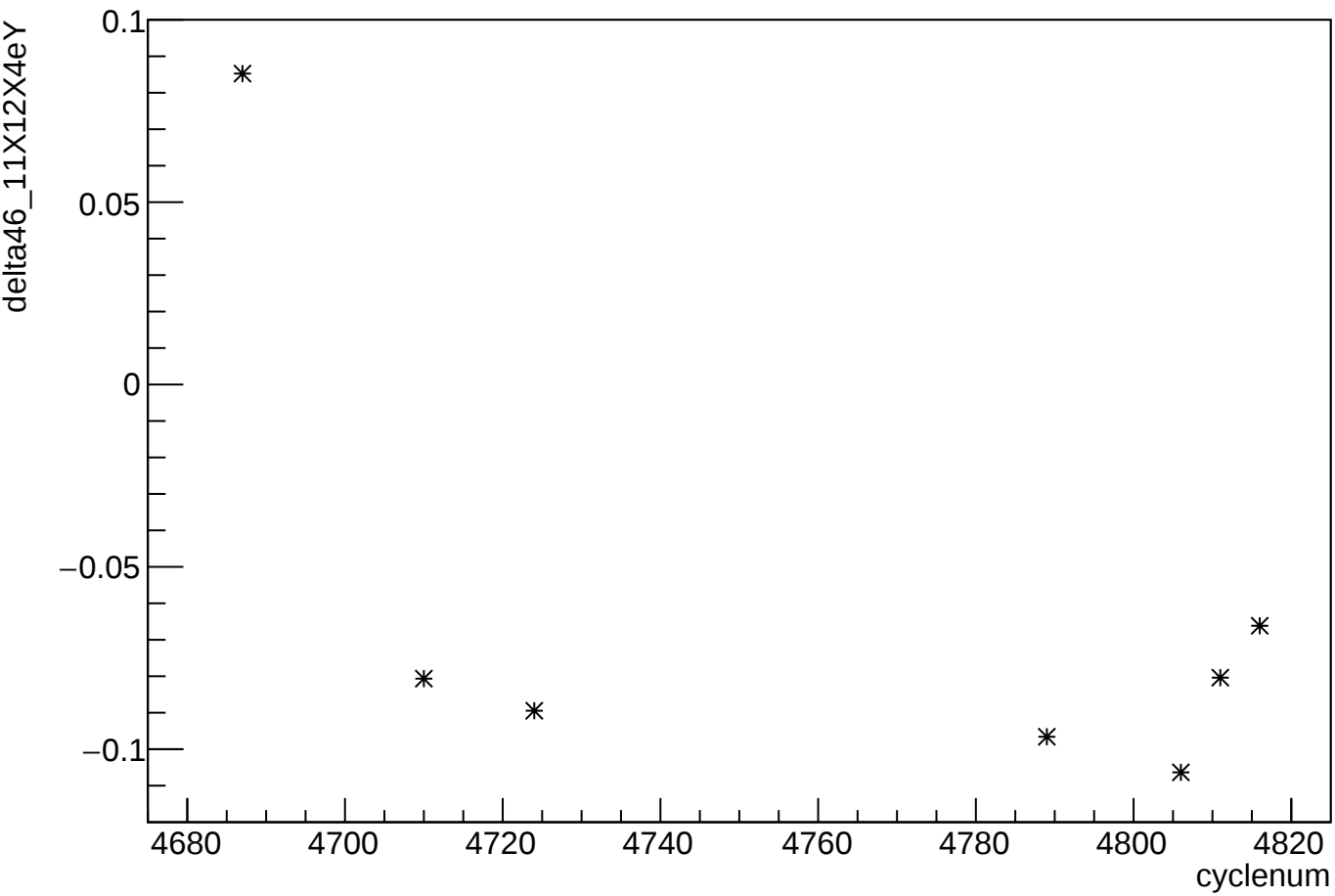
delta46_11X12X4eY:cyclenum
