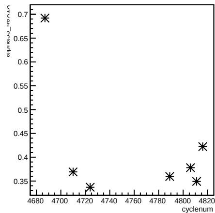
alpha53_4eX1X:cyclenum
