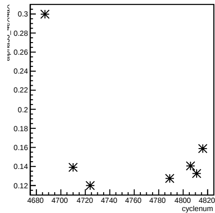
alpha53_4eX4aX:cyclenum
