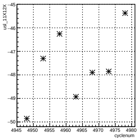
usl_11X12:cyclenum
