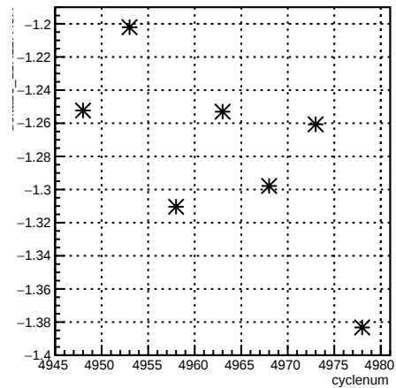
delta13_11X12X4eX:cyclenum
