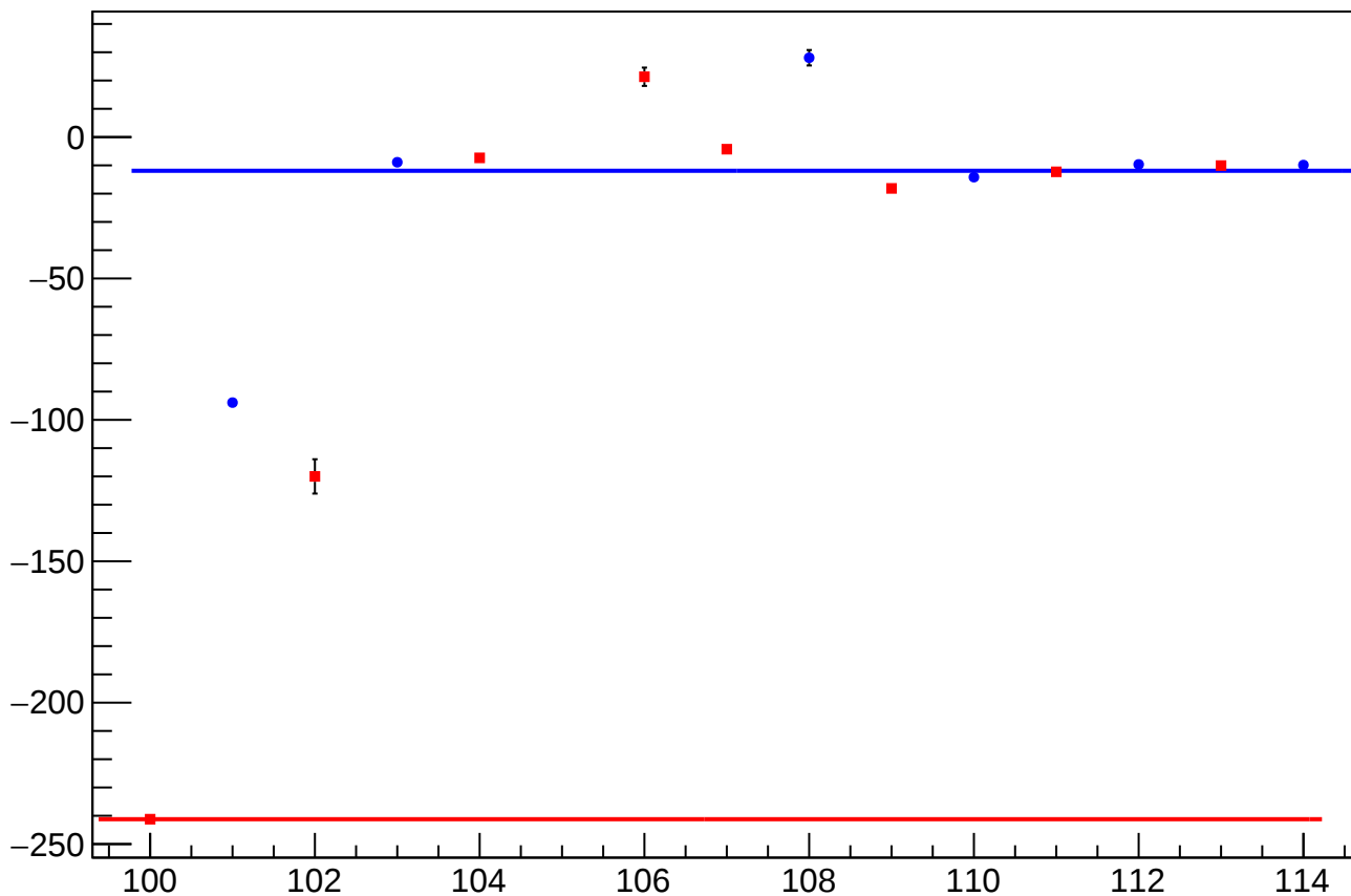
dit_atr1_11X12X_slope vs Slug
