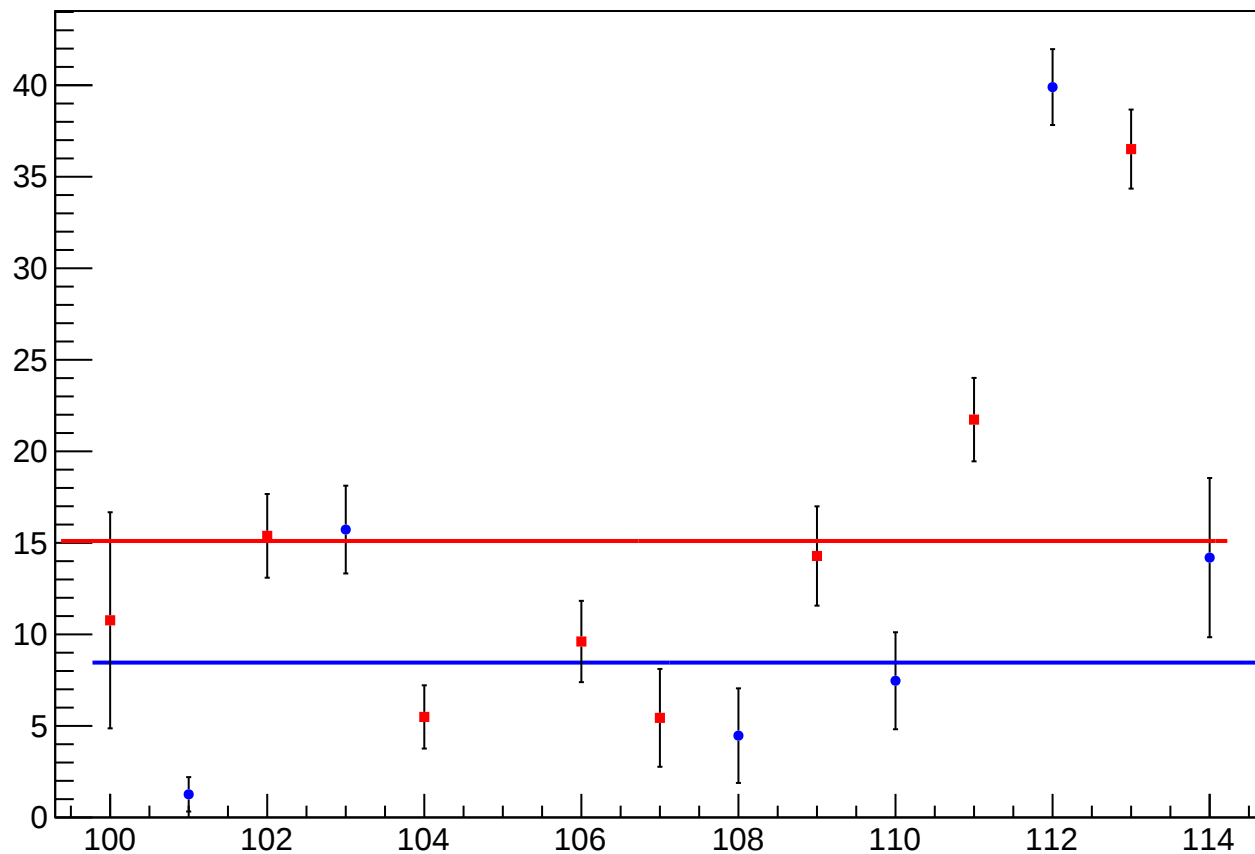
reg_asym_us_avg_diff_bpm4aY_slope vs Slug
