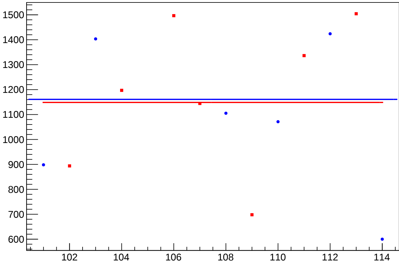
dit_sam4_coil4_Ndata_mean vs Slug
