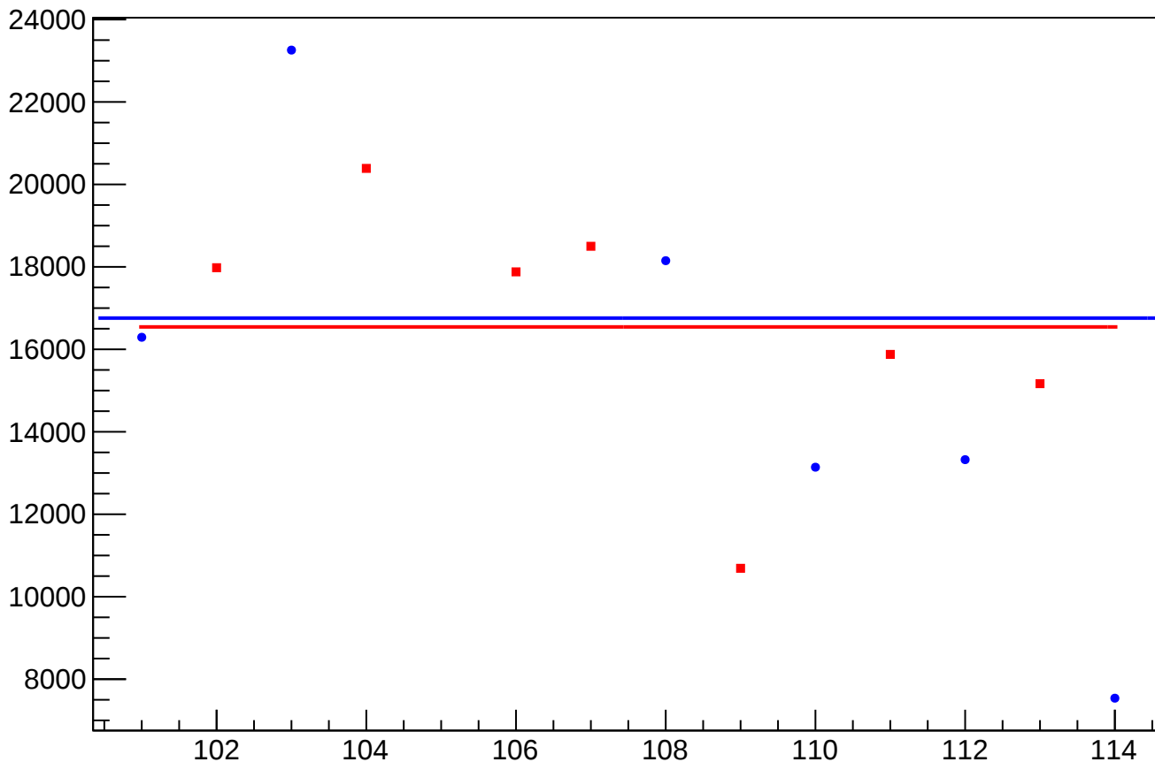
dit_sam5_coil4_mean vs Slug
