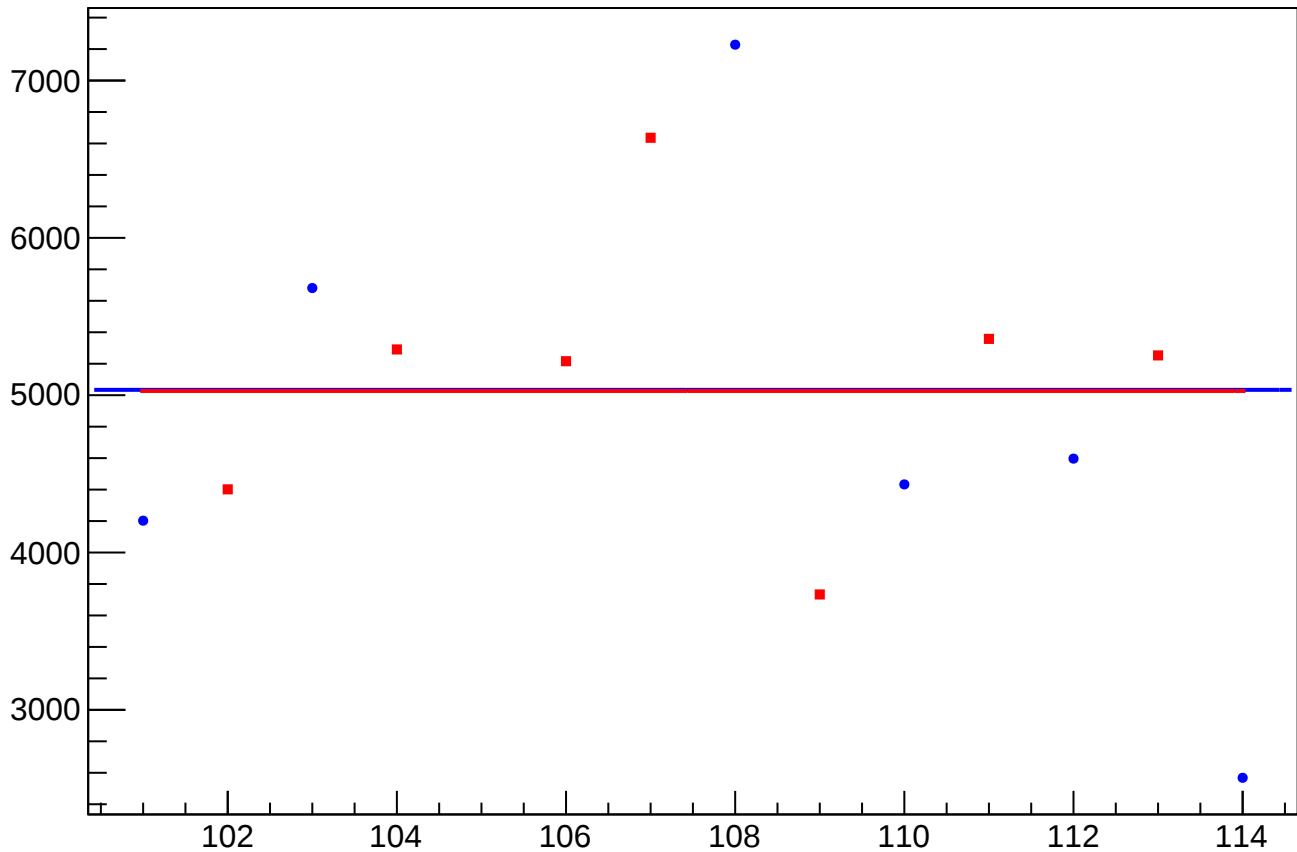
dit_sam4_coil3_mean vs Slug
