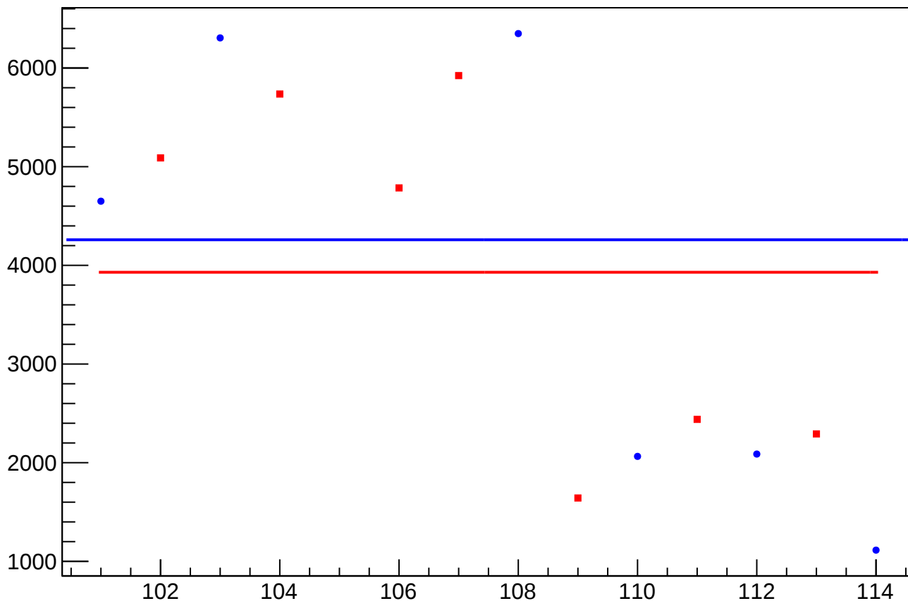
dit_sam8_coil1_mean vs Slug
