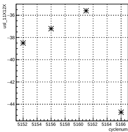
usl_11X12X:cyclenum
