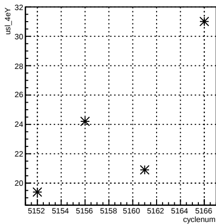
usl_4eY:cyclenum
