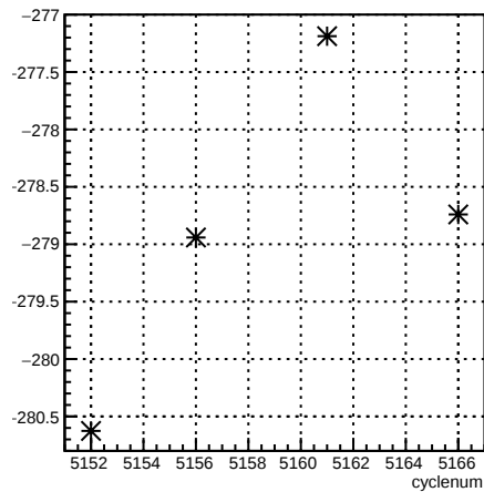
4aX_coil1:cyclenum
