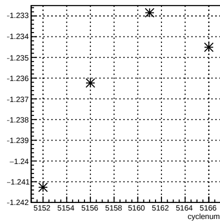
delta13_11X12X4eX:cyclenum
