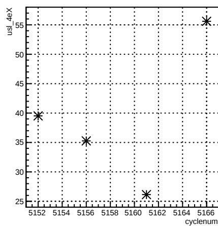
usl_4eX:cyclenum
