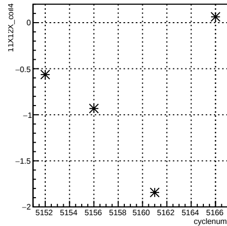
11X12X_coil4:cyclenum
