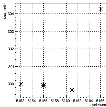
4aX_coil7:cyclenum
