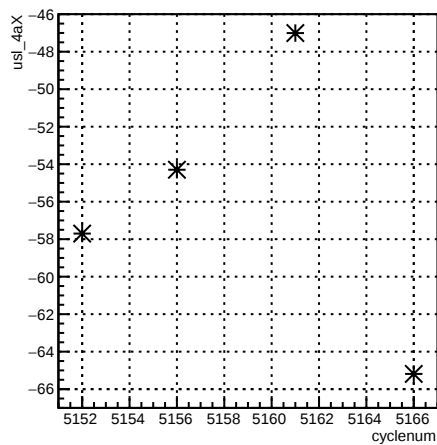
usl_4aX:cyclenum
