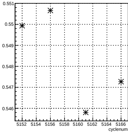
alpha13_4eX4aX:cyclenum
