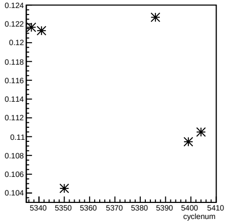
alpha53_4eX4aX:cyclenum
