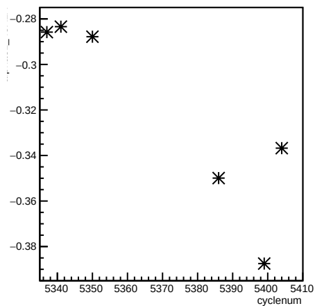
alpha51_4eX1X:cyclenum
