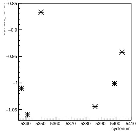
alpha31_4eX1X:cyclenum
