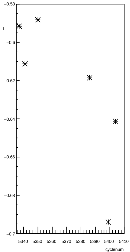
delta15_11X12X4eX:cyclenum
