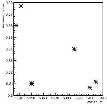
alpha53_4eX1X:cyclenum
