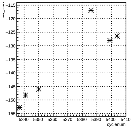
usr_4aX:cyclenum
