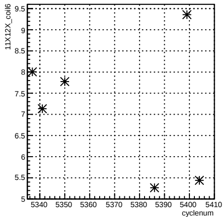
11X12X_coil6:cyclenum
