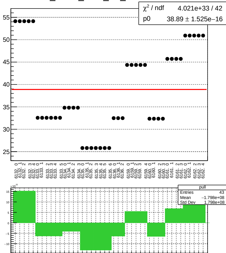
dit_sam1_coil3_err_mean vs run
