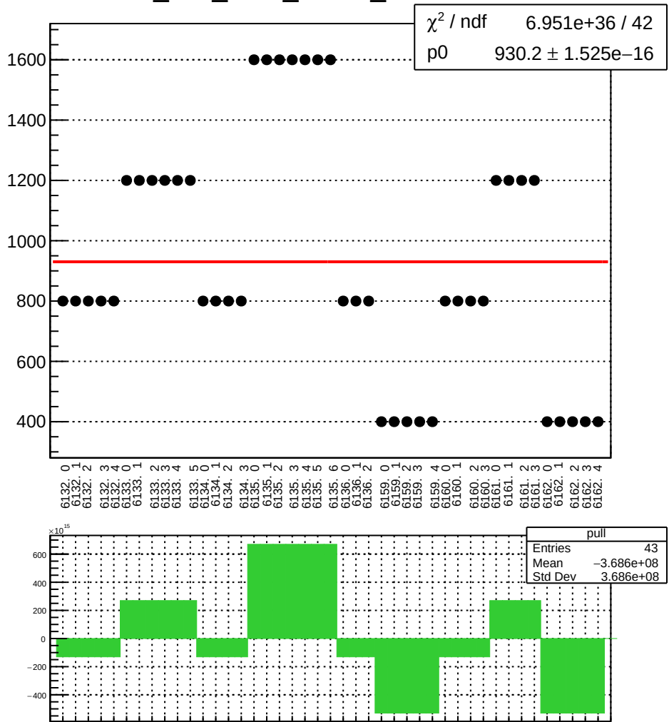
dit_atl2_coil4_Ndata_mean vs run
