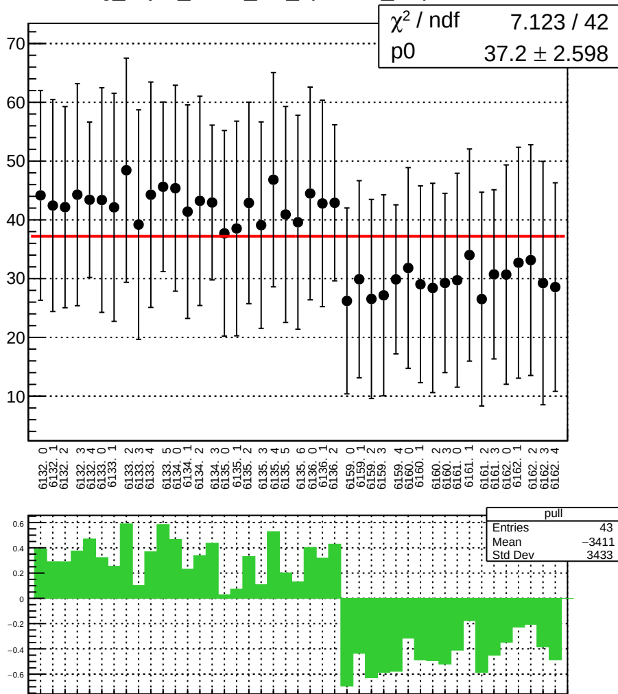
reg_asym_sam6_diff_bpm4aX_slope vs run
