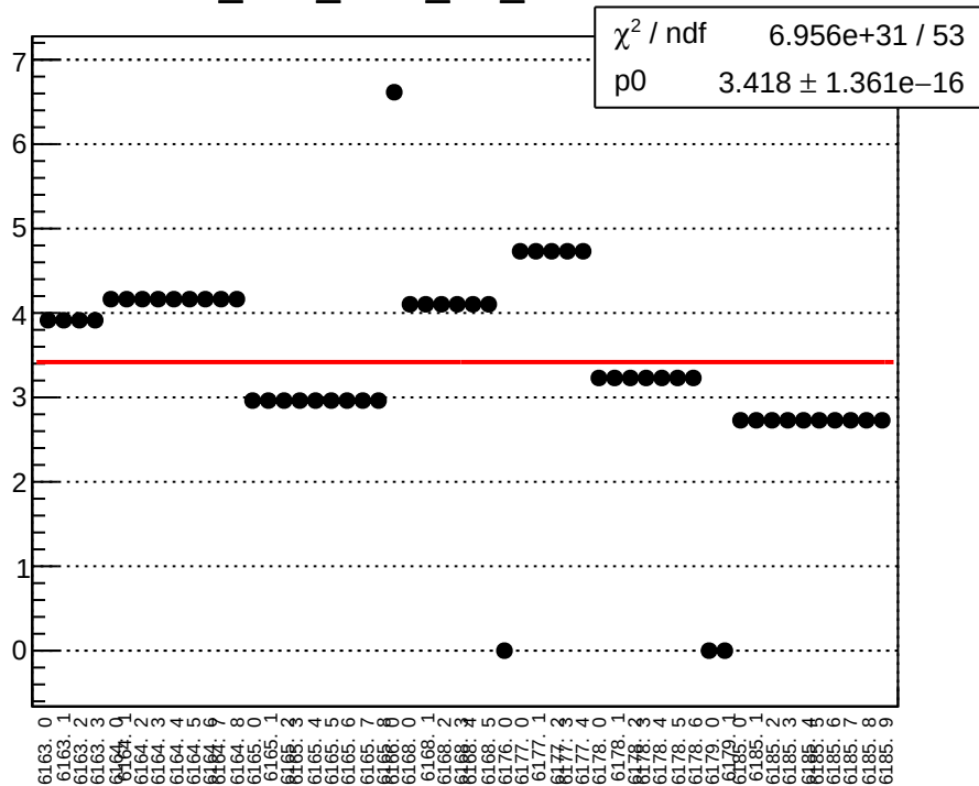
dit_4eX_coil1_err_mean vs run
