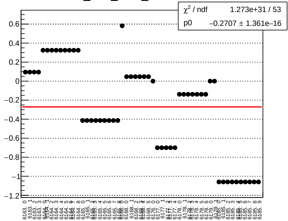
dit_4aX_coil6_mean vs run
