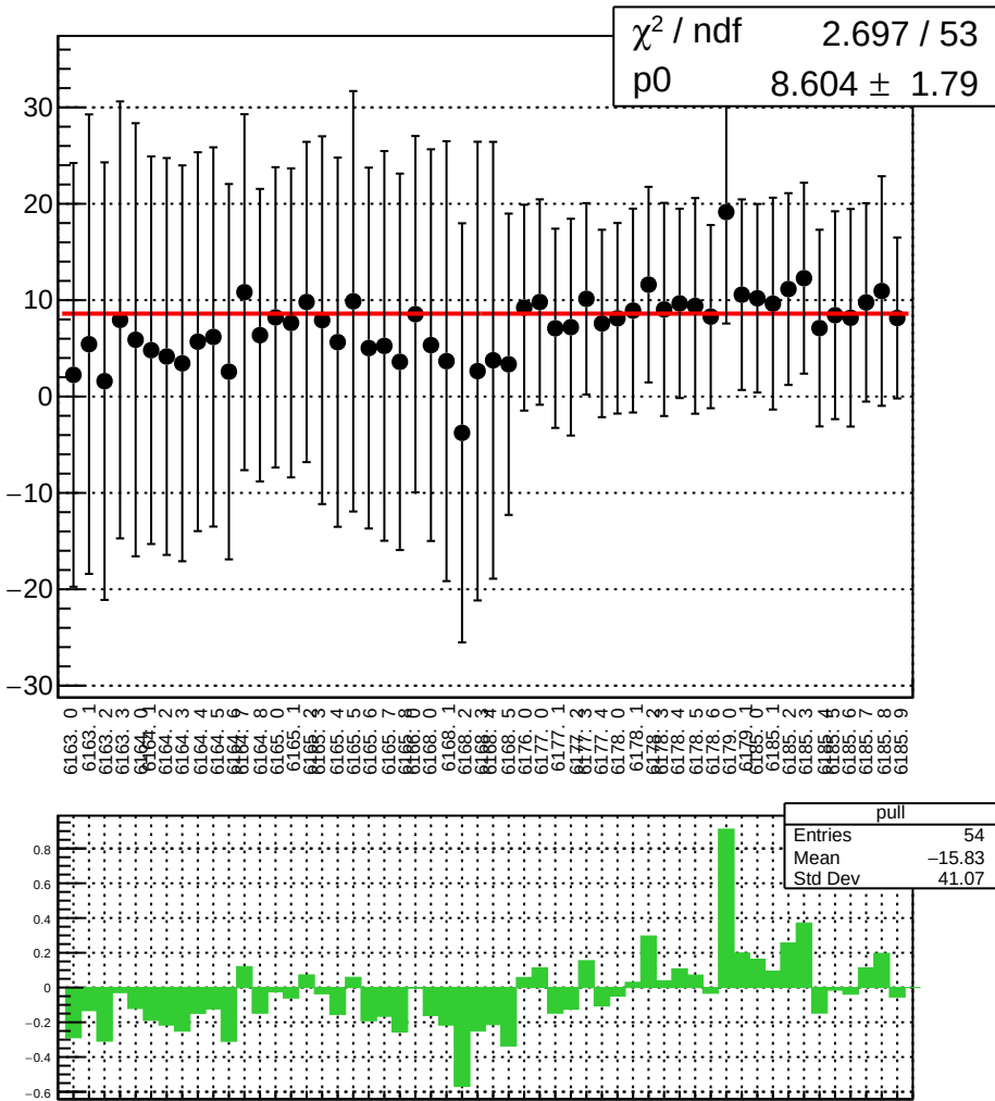
reg_asym_sam_37_dd_diff_bpm4eX_slope vs run
