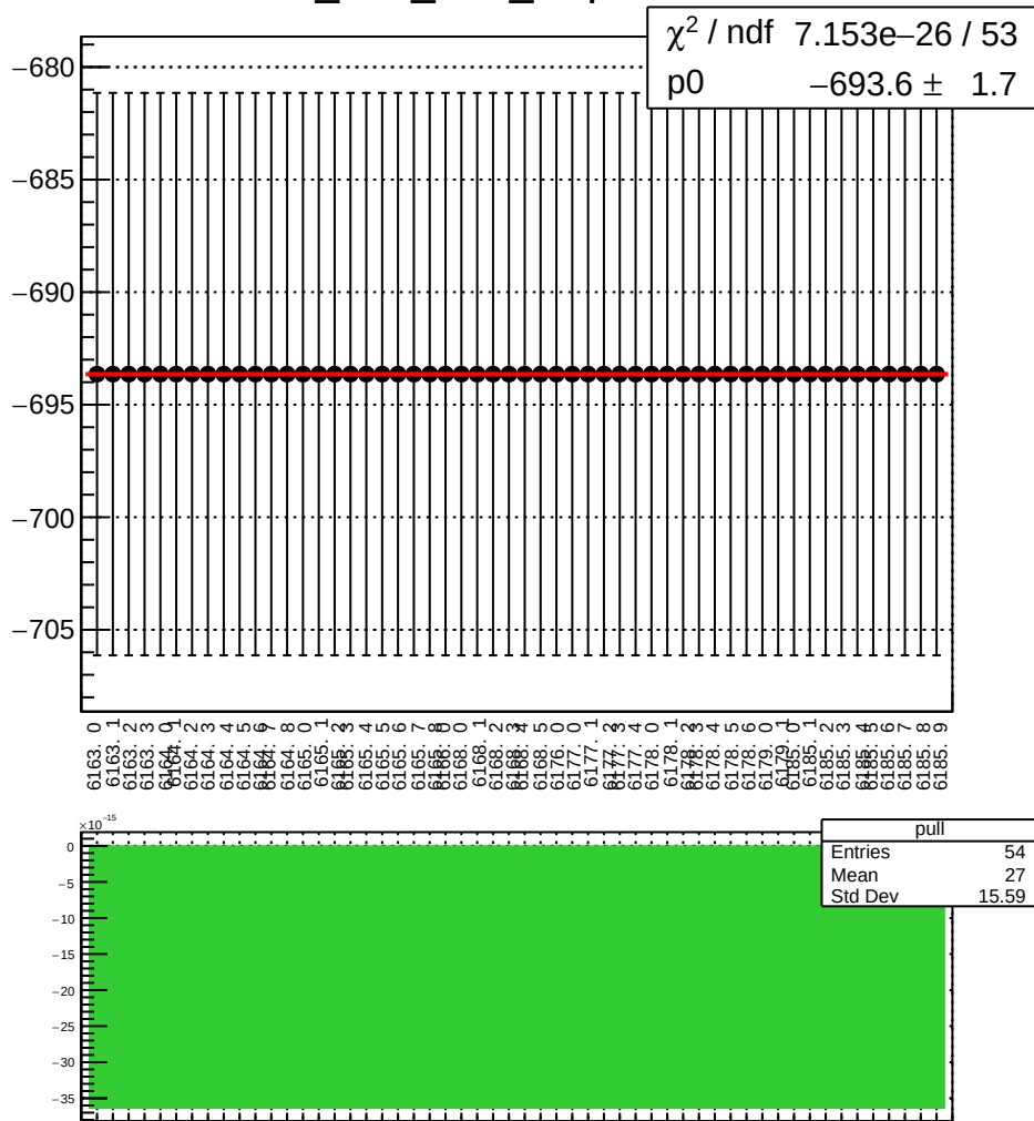
dit_atr2_4aX_slope vs run
