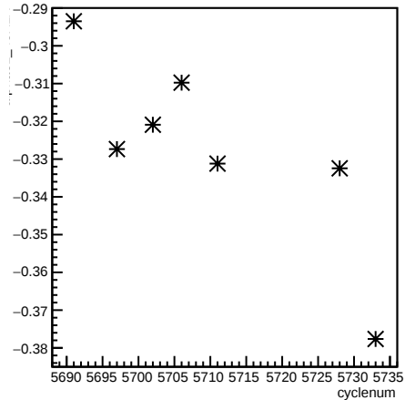
alpha51_4eX1X:cyclenum
