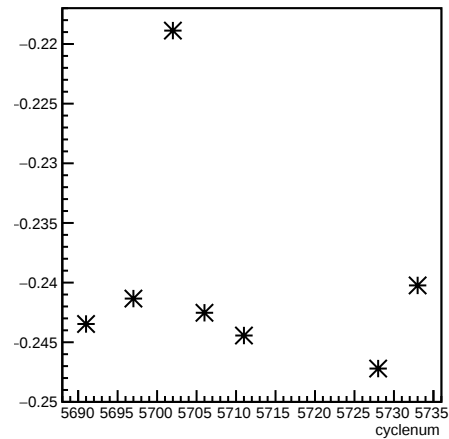
alpha31_4eX4aX:cyclenum
