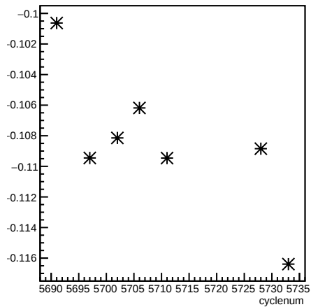
alpha51_4eX4aX:cyclenum
