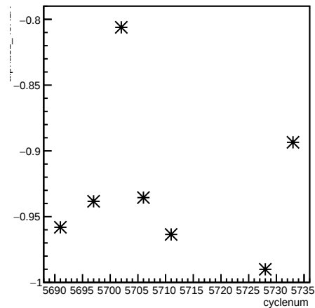
alpha31_4eX1X:cyclenum
