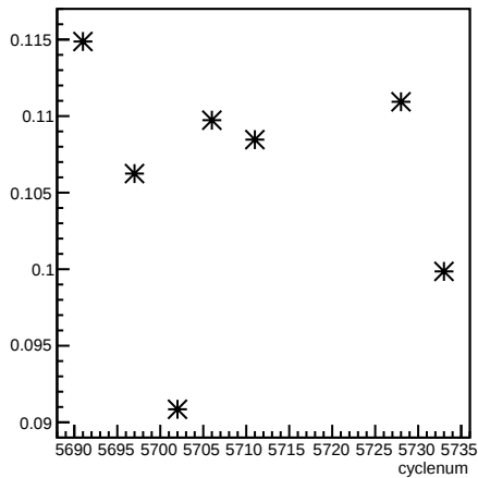
alpha53_4eX4aX:cyclenum
