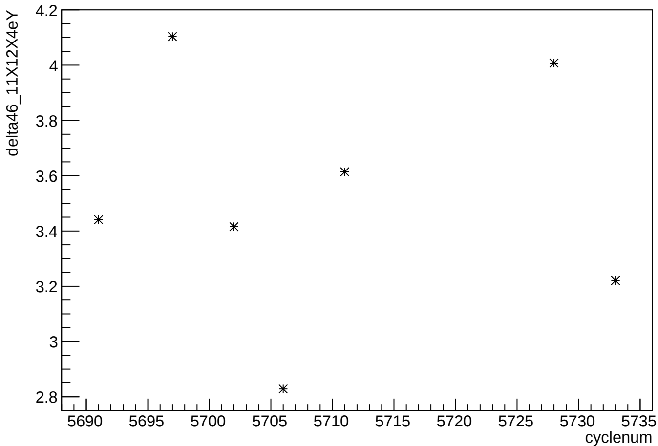
delta46_11X12X4eY:cyclenum
