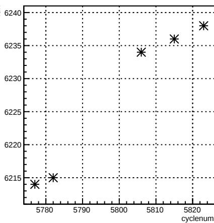
run:cyclenum
