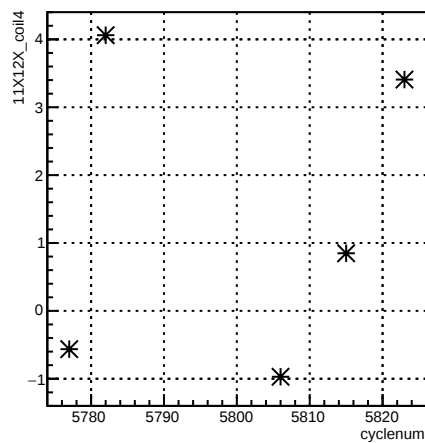
11X12X_coil4:cyclenum
