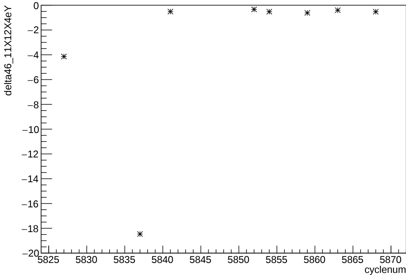
delta46_11X12X4eY:cyclenum
