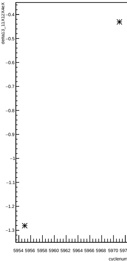
delta13_11X12X4eX:cyclenum
