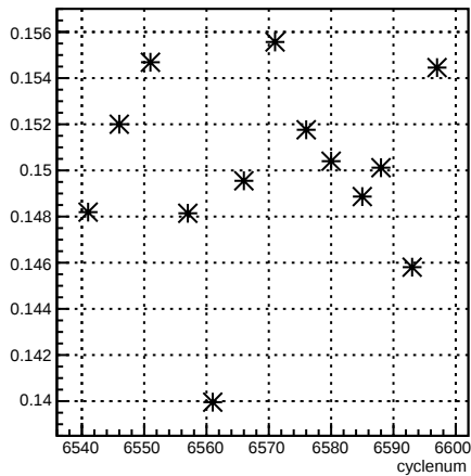
alpha13_4eX4aX:cyclenum
