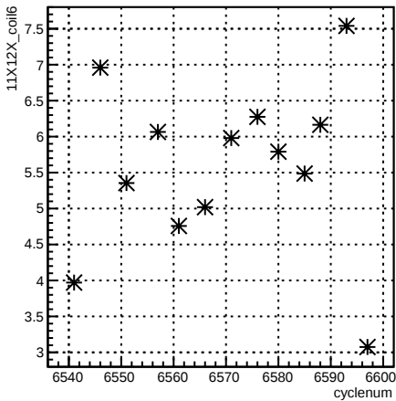
11X12X_coil6:cyclenum
