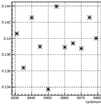
alpha13_4eX4aX:cyclenum
