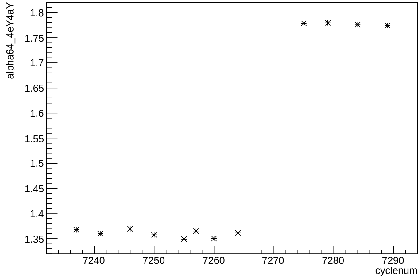
alpha64_4eY4aY:cyclenum
