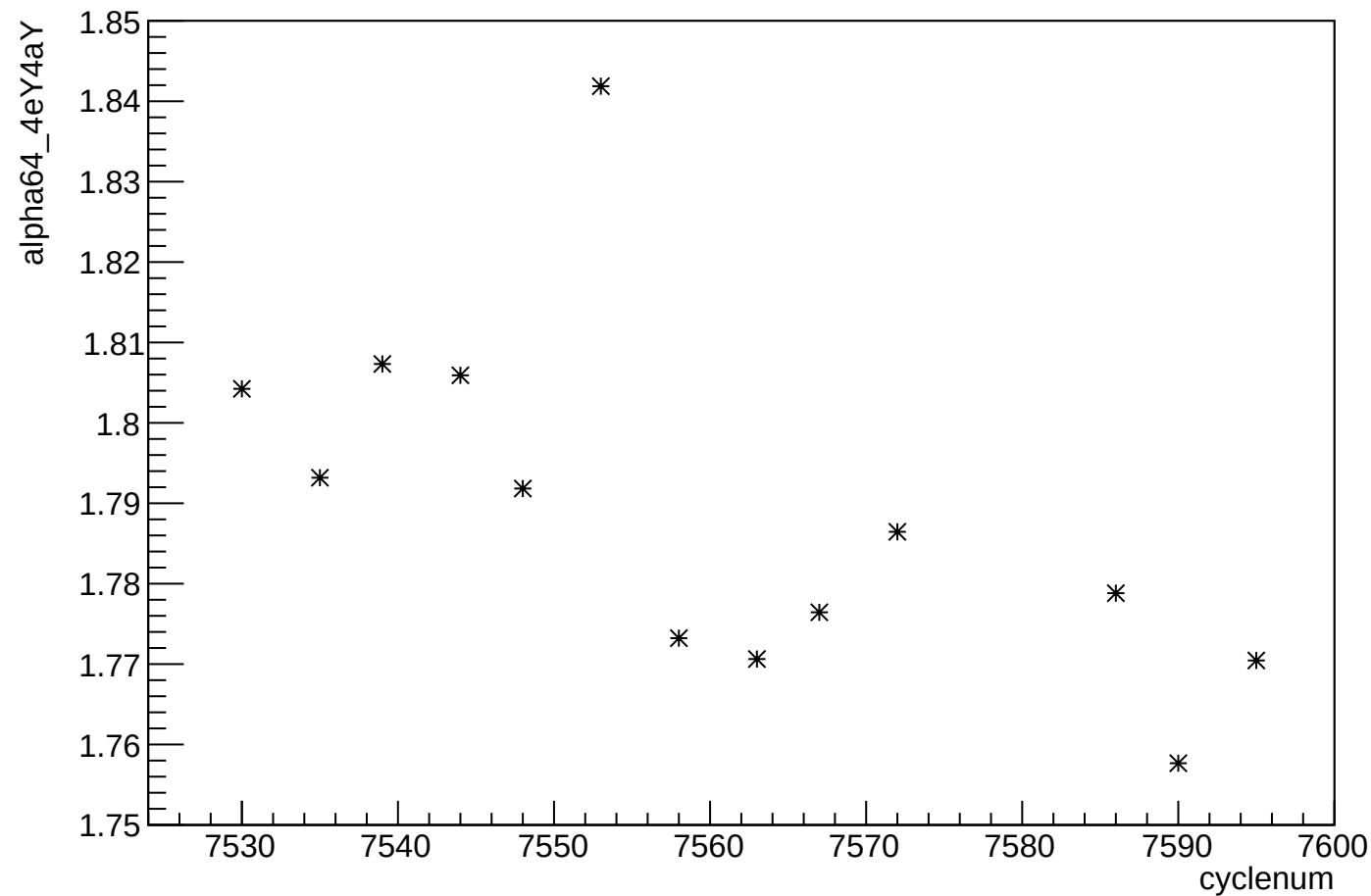
alpha64_4eY4aY:cyclenum
