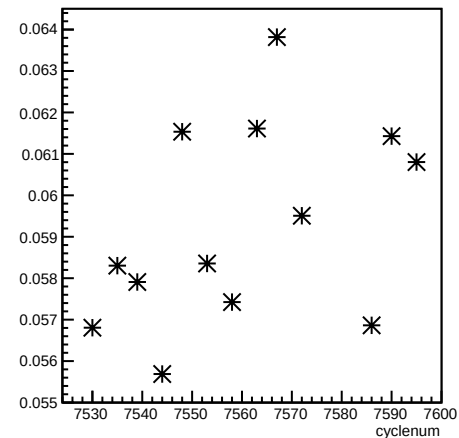
alpha53_4eX1X:cyclenum
