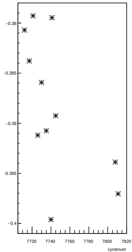
delta13_11X12X4eX:cyclenum
