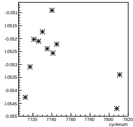
alpha31_4eX4aX:cyclenum
