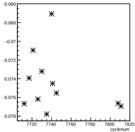
alpha51_4eX1X:cyclenum
