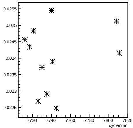
alpha53_4eX4aX:cyclenum
