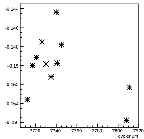
alpha31_4eX1X:cyclenum
