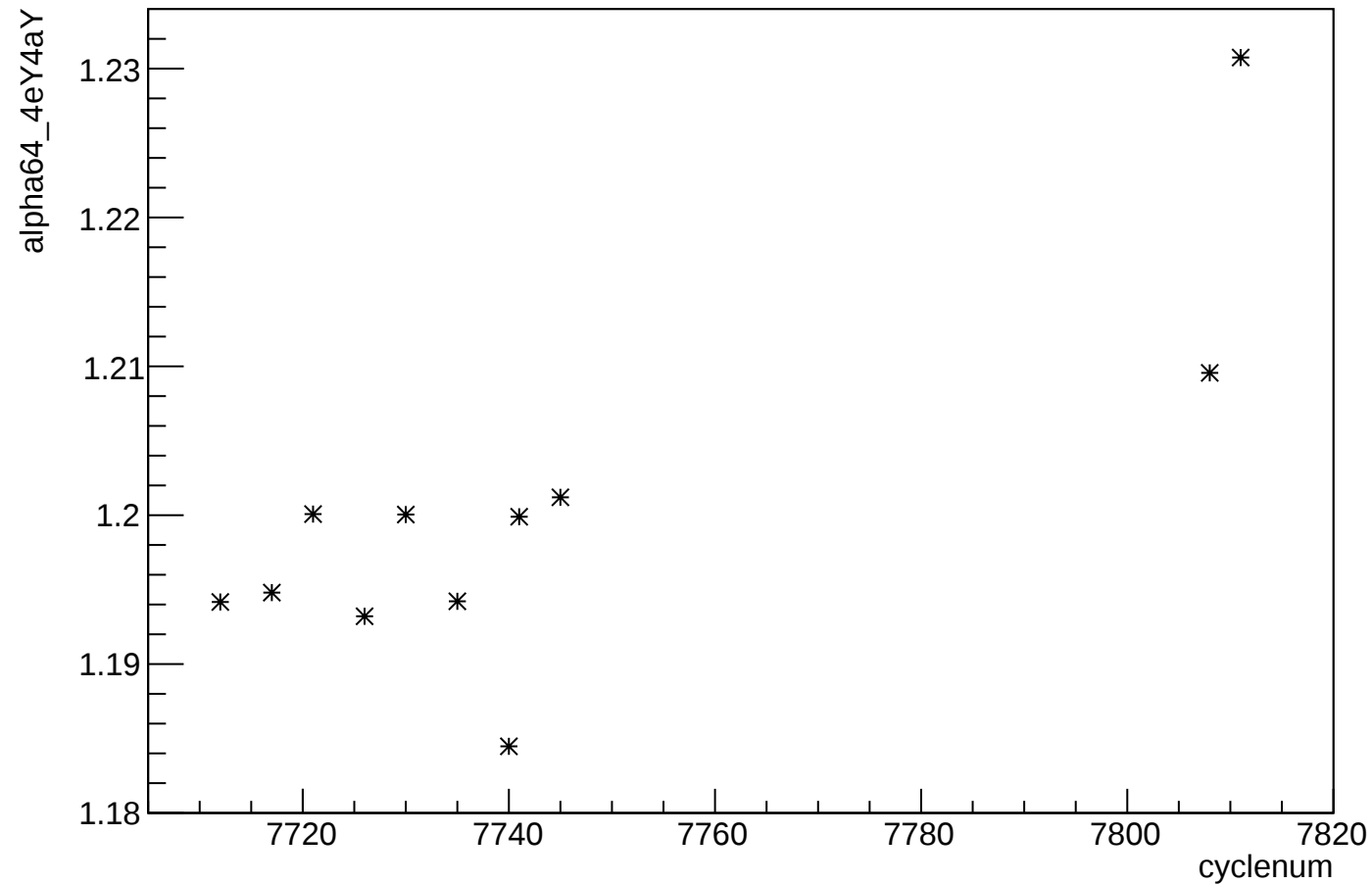
alpha64_4eY4aY:cyclenum
