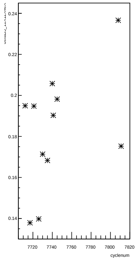
delta35_11X12X4eX:cyclenum
