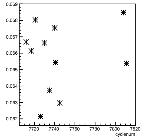
alpha53_4eX1X:cyclenum
