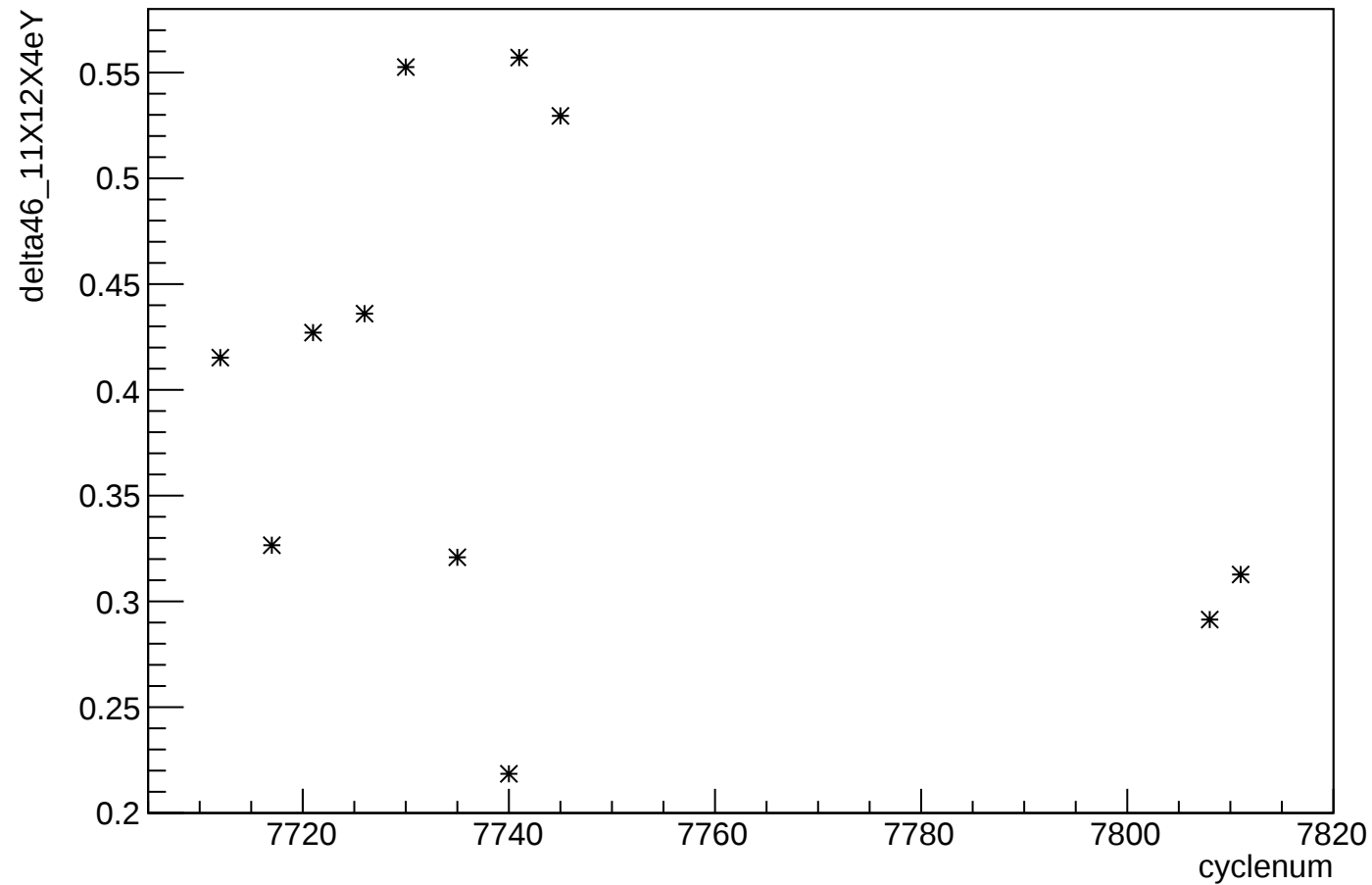
delta46_11X12X4eY:cyclenum
