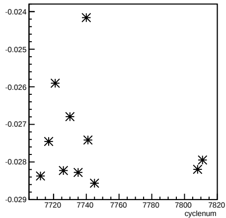
alpha51_4eX4aX:cyclenum
