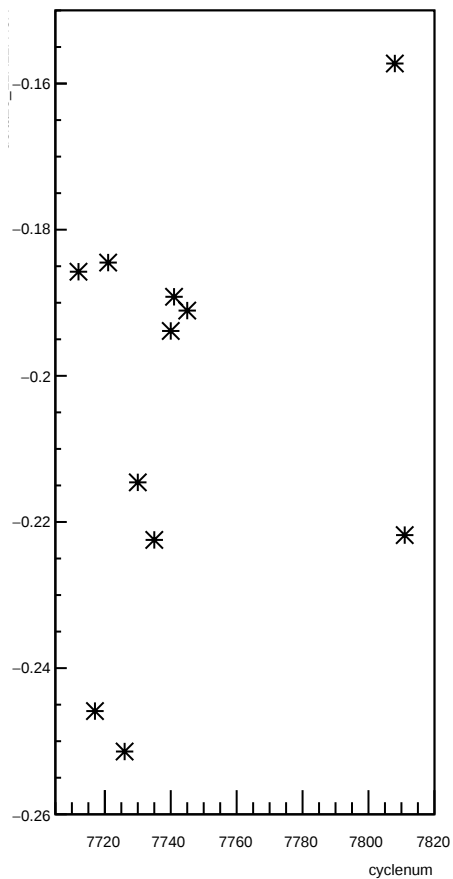
delta15_11X12X4eX:cyclenum
