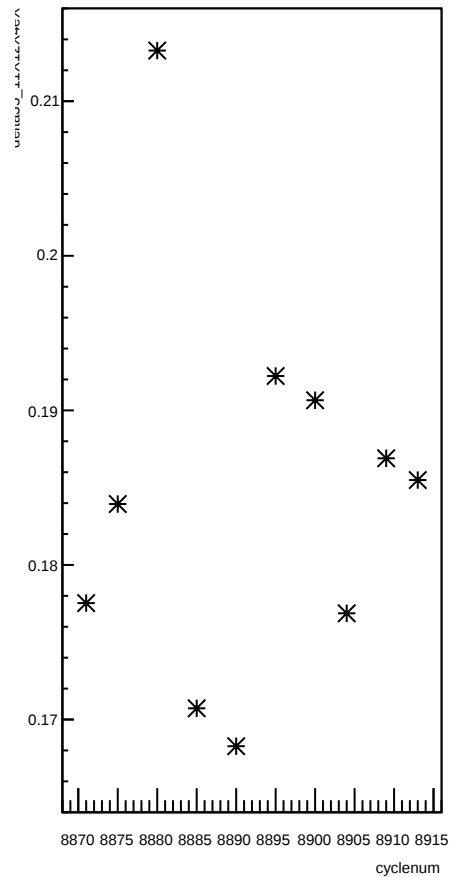
delta35_11X12X4eX:cyclenum
