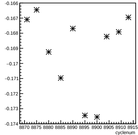
alpha31_4eX1X:cyclenum
