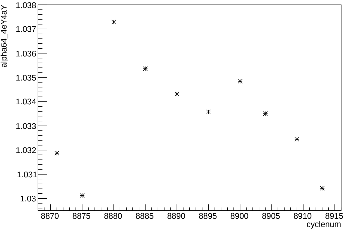
alpha64_4eY4aY:cyclenum
