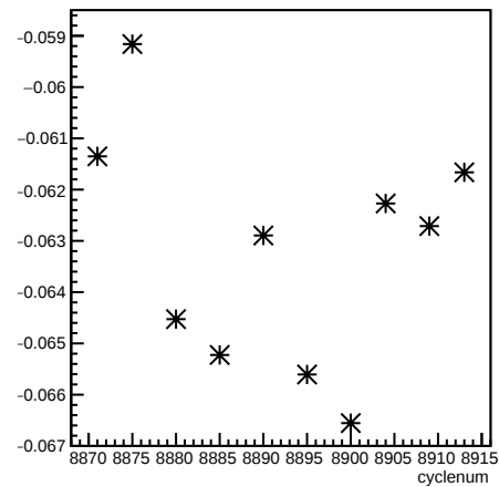
alpha31_4eX4aX:cyclenum
