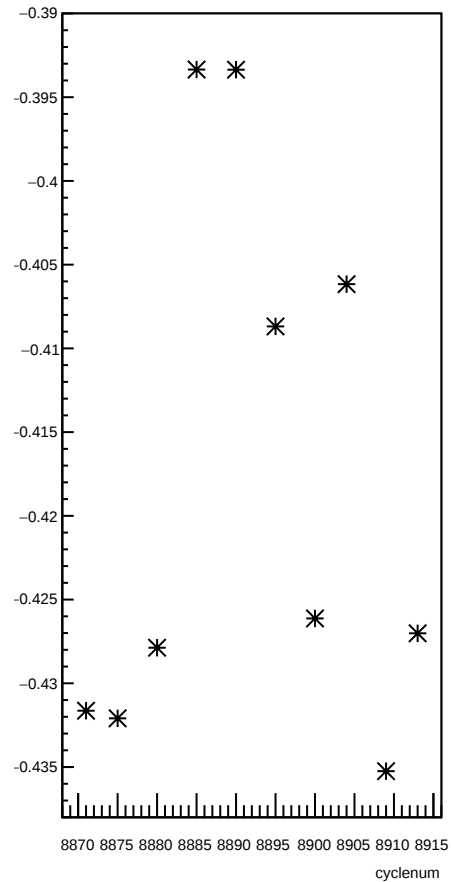
delta13_11X12X4eX:cyclenum
