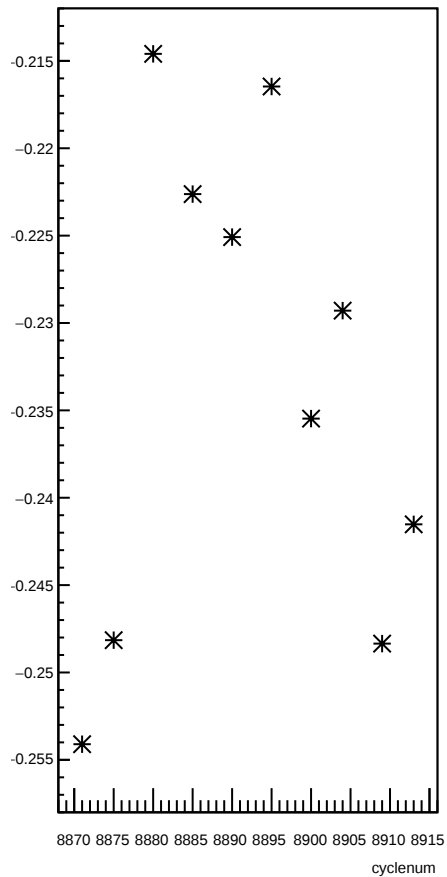
delta15_11X12X4eX:cyclenum
