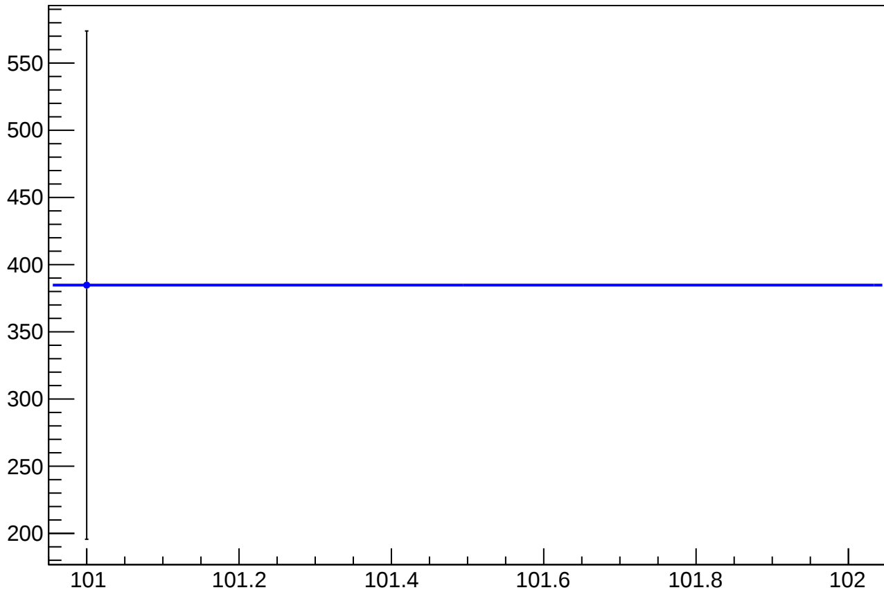
dit_asym_sam1_mean vs Slug
