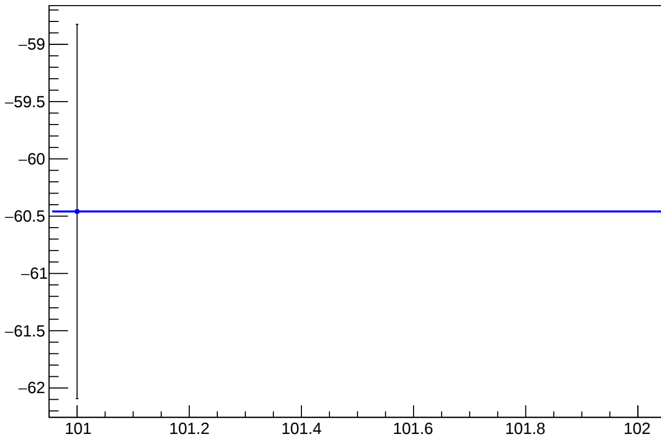
reg_asym_sam_48_dd_diff_bpm4aX_slope vs Slug
