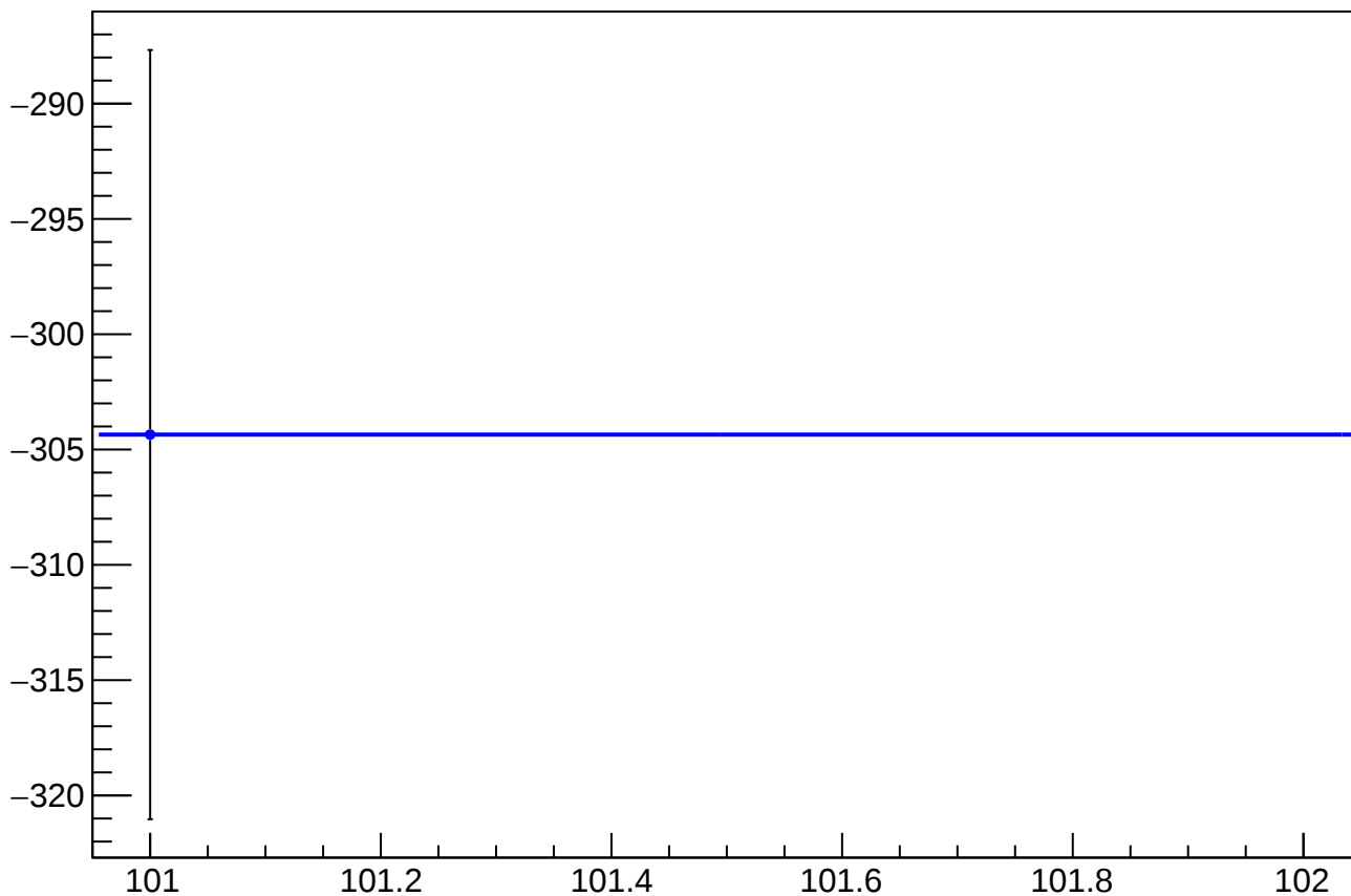
reg_asym_at2_avg_diff_bpm4aX_slope vs Slug
