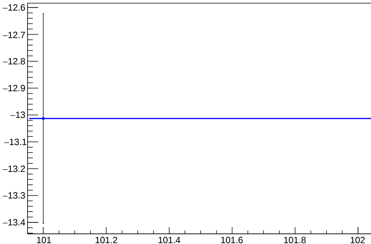
reg_asym_sam6_diff_bpm4eY_slope vs Slug
