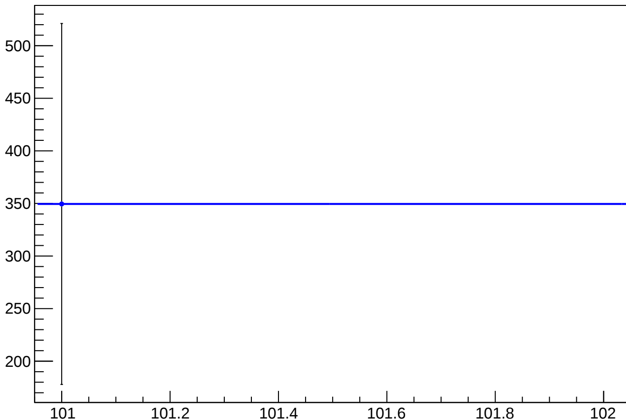
dit_asym_sam_1526_avg_mean vs Slug
