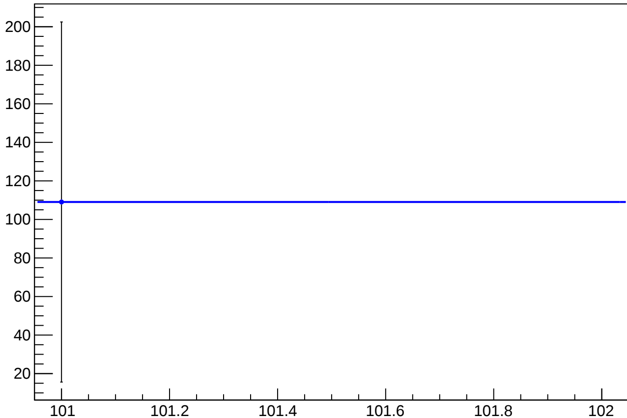
asym_sam_15_avg_correction_mean vs Slug
