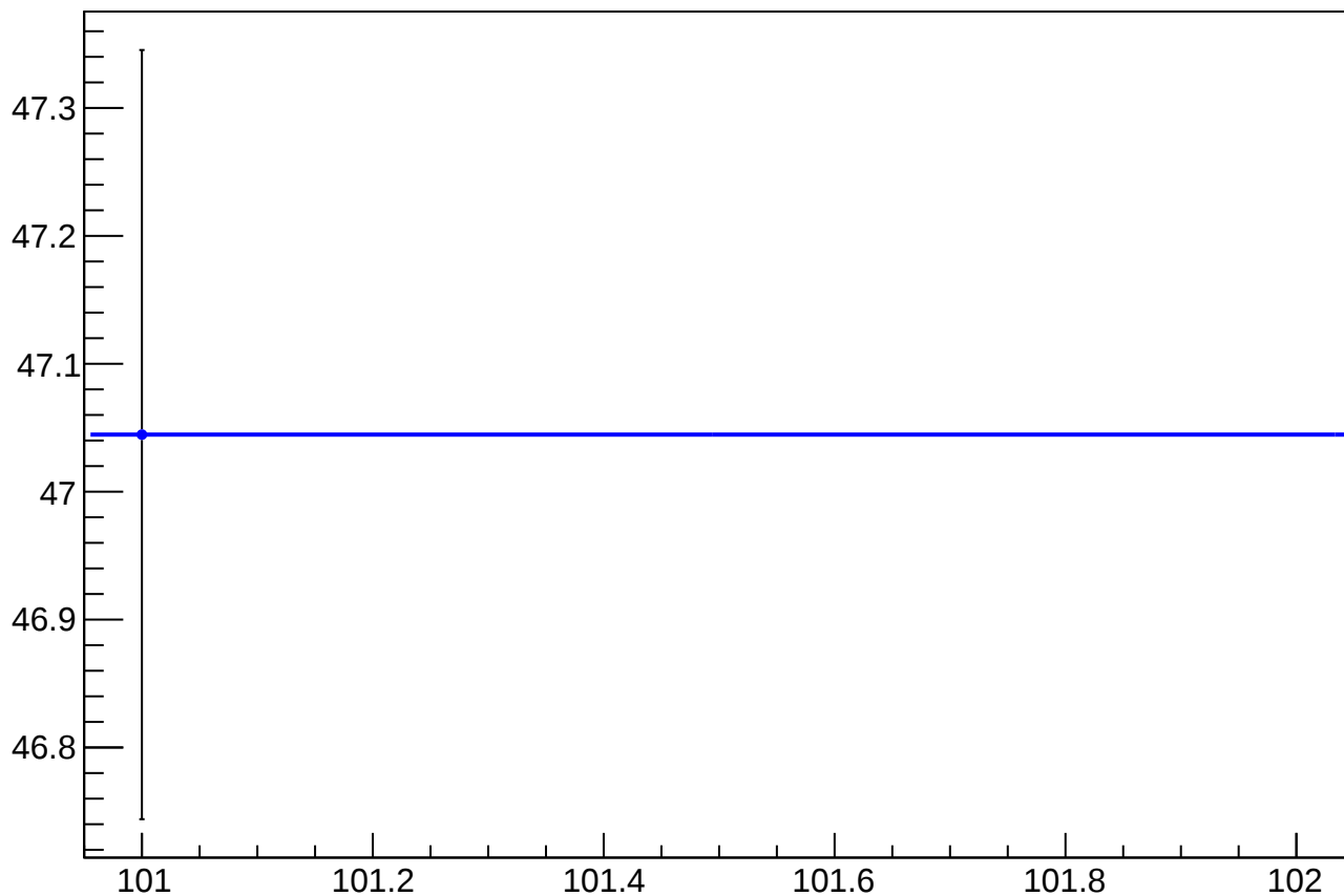
dit_sam8_4eY_slope vs Slug
