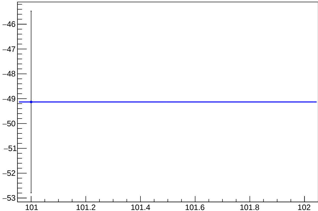
reg_asym_sam2_diff_bpm4aY_slope vs Slug
