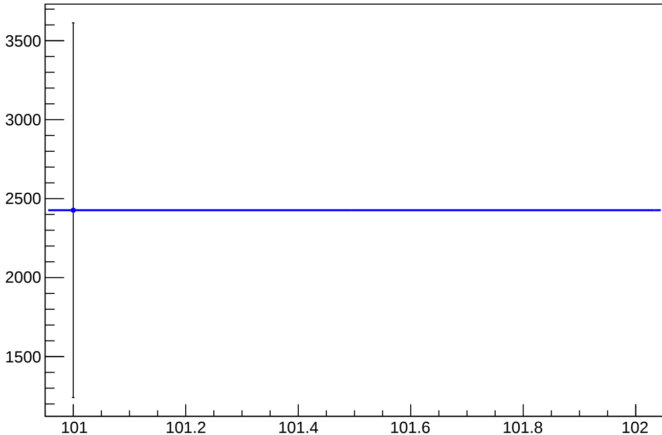
asym_sam_48_dd_mean vs Slug
