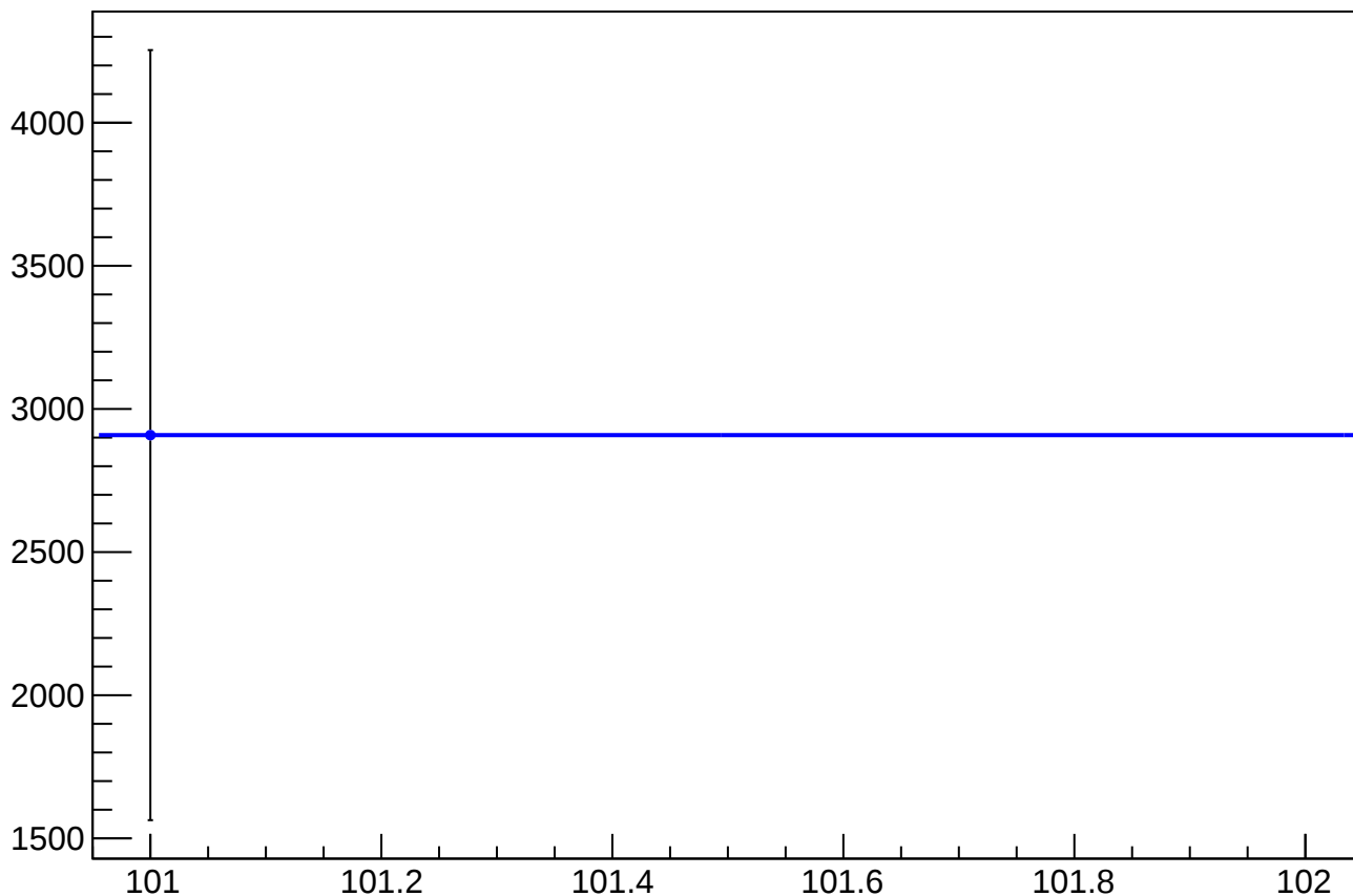
asym_atl_dd_atr_dd_dd_correction_mean vs Slug
