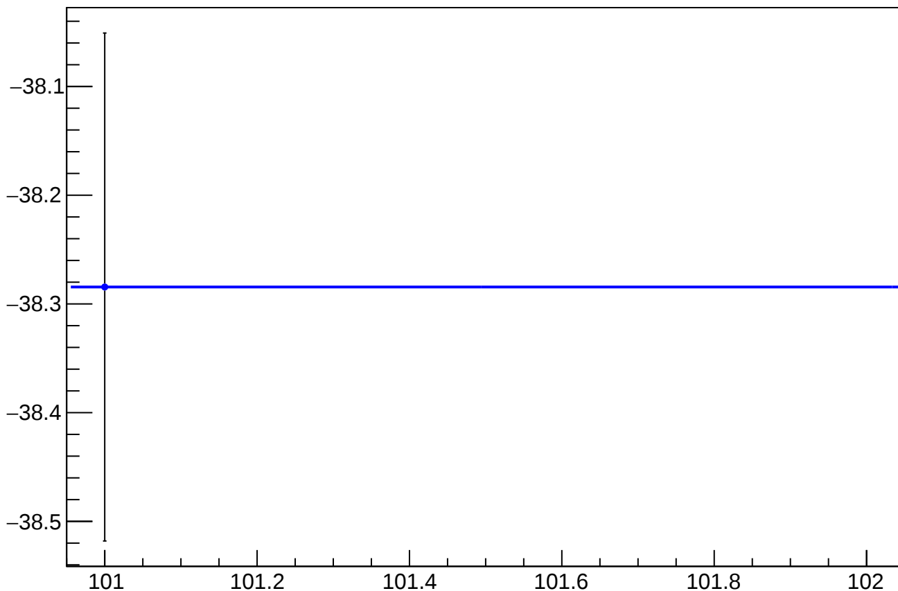
reg_asym_sam8_diff_bpm4aY_slope vs Slug
