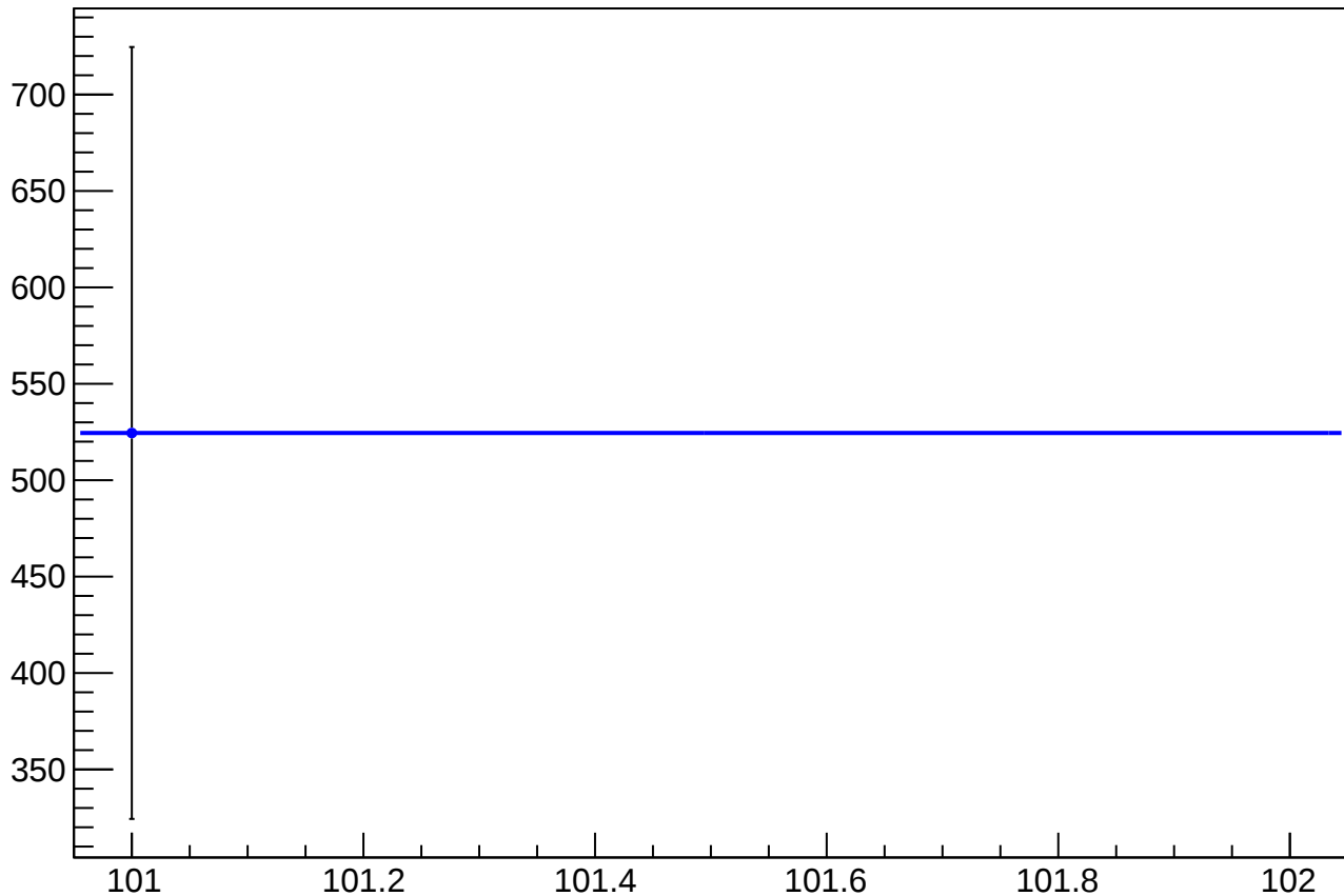
dit_asym_sam_26_48_dd_mean vs Slug
