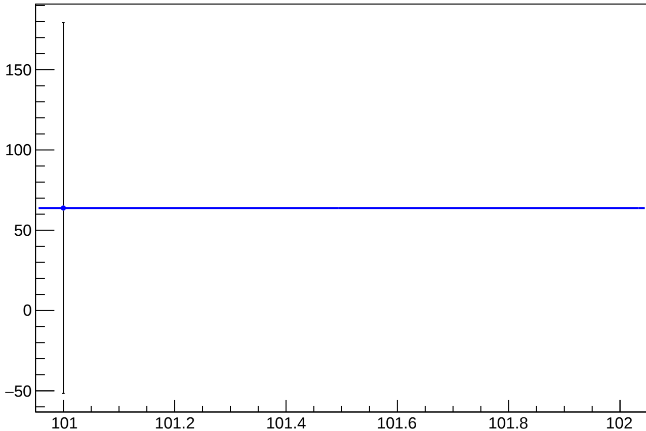
dit_asym_sam_12345678_avg_mean vs Slug
