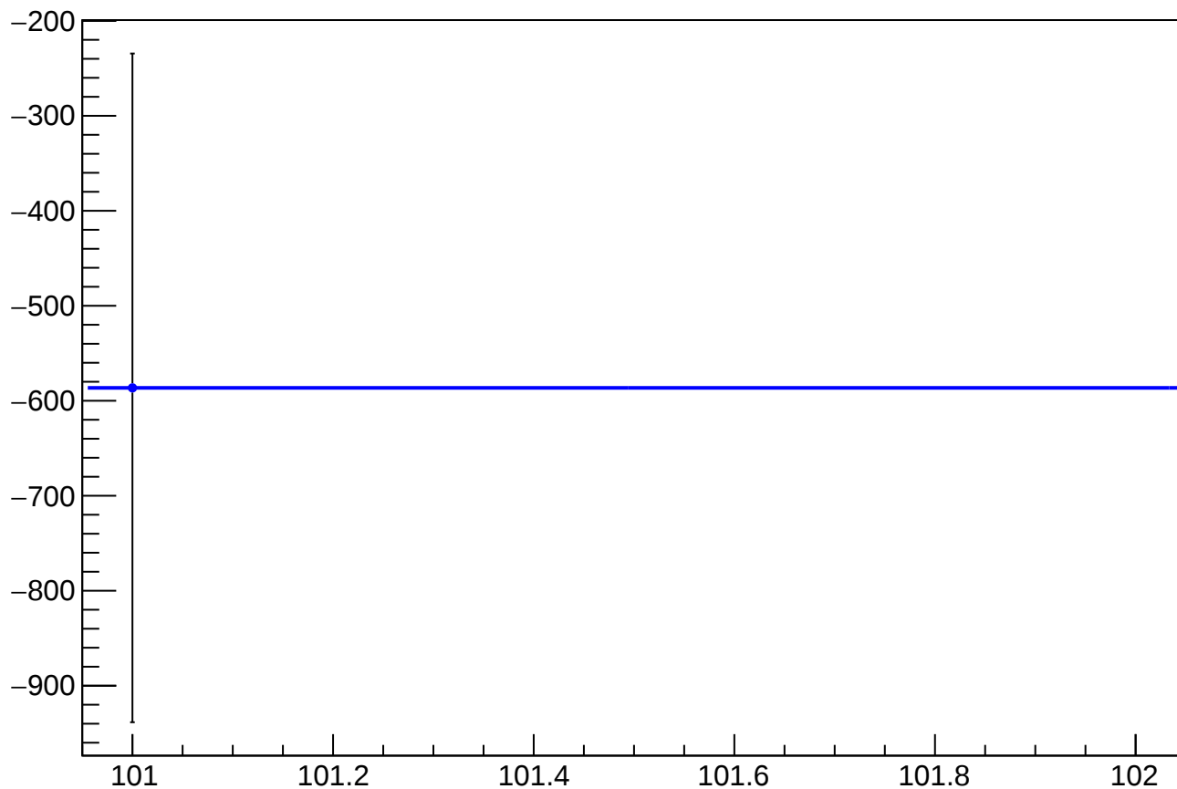
dit_asym_sam4_mean vs Slug
