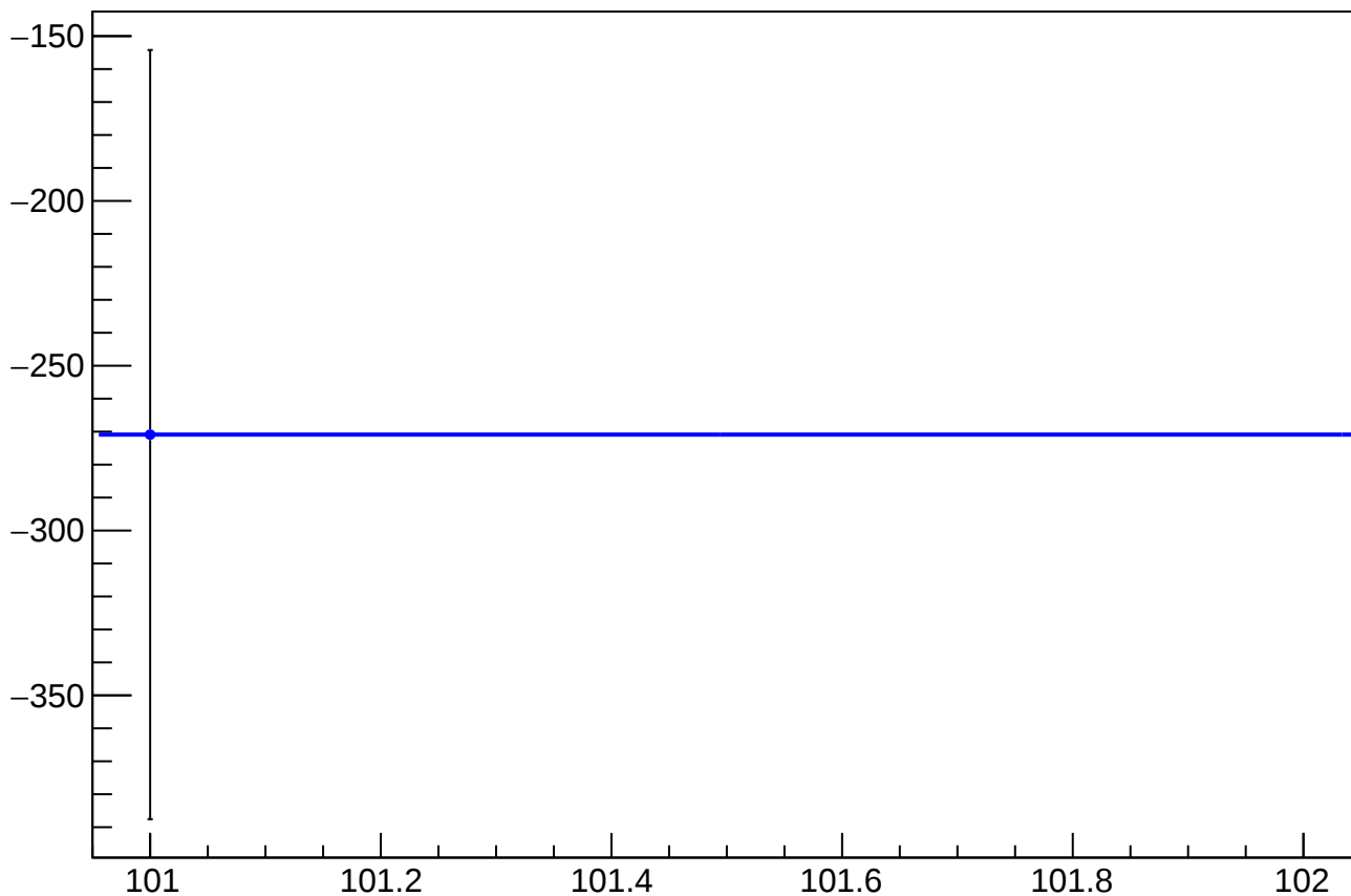
dit_asym_sam6_mean vs Slug
