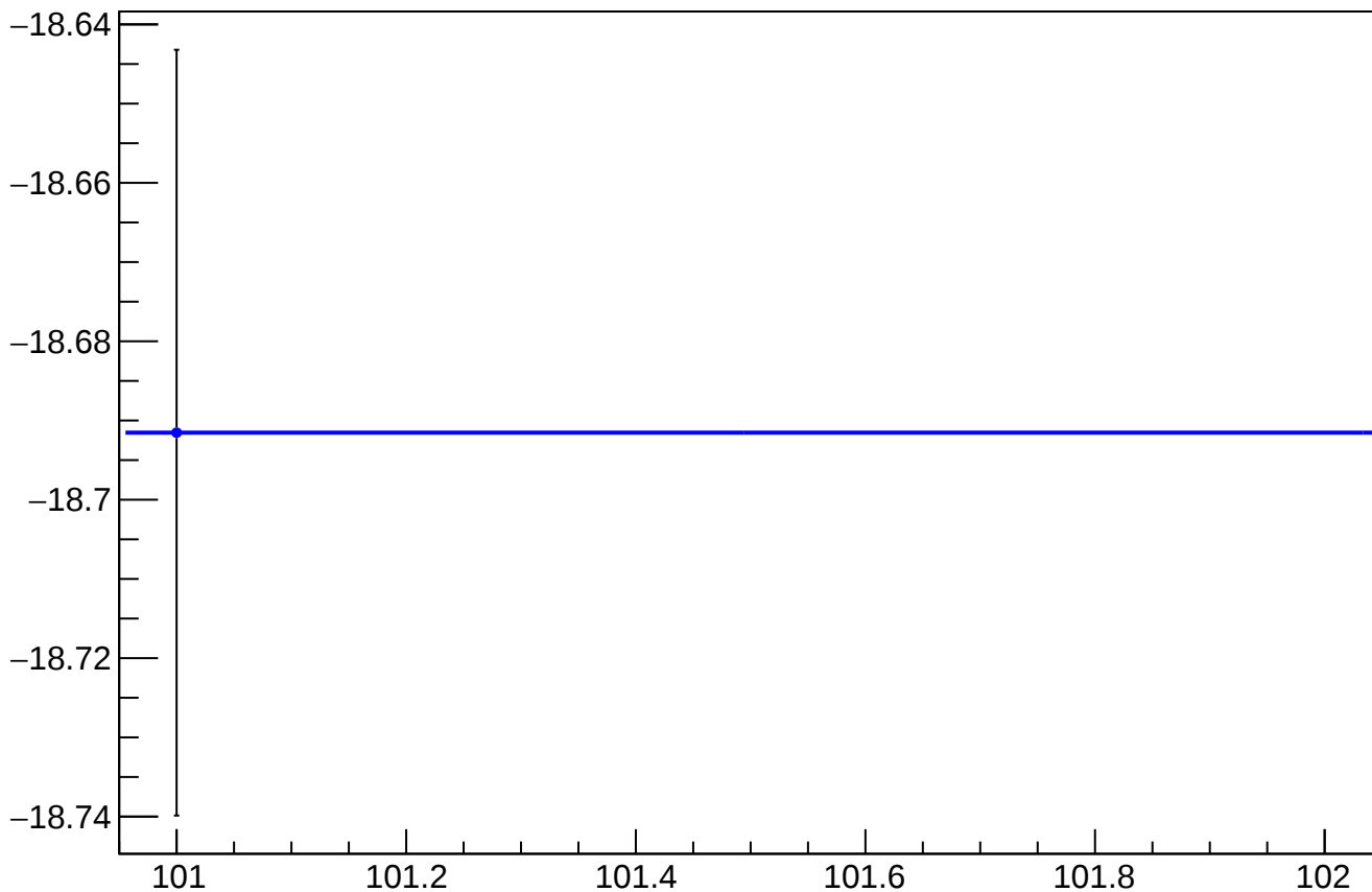
reg_asym_right_avg_diff_bpm12X_slope vs Slug
