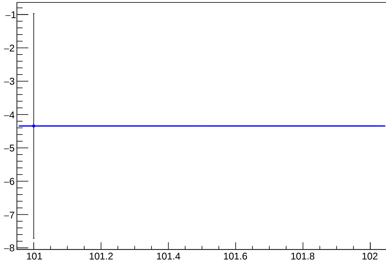
reg_asym_sam4_diff_bpm4eX_slope vs Slug
