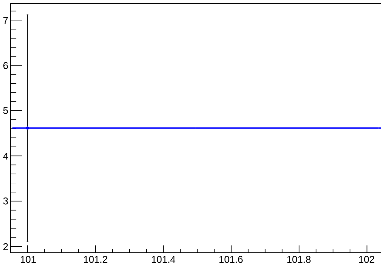
reg_asym_usl_diff_bpm4eX_slope vs Slug, Sign Corrected
