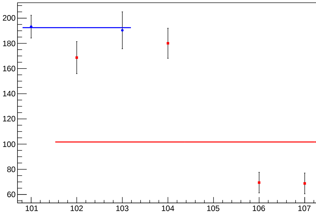
reg_asym_atl_dd_diff_bpm4aX_slope vs Slug, Sign Corrected
