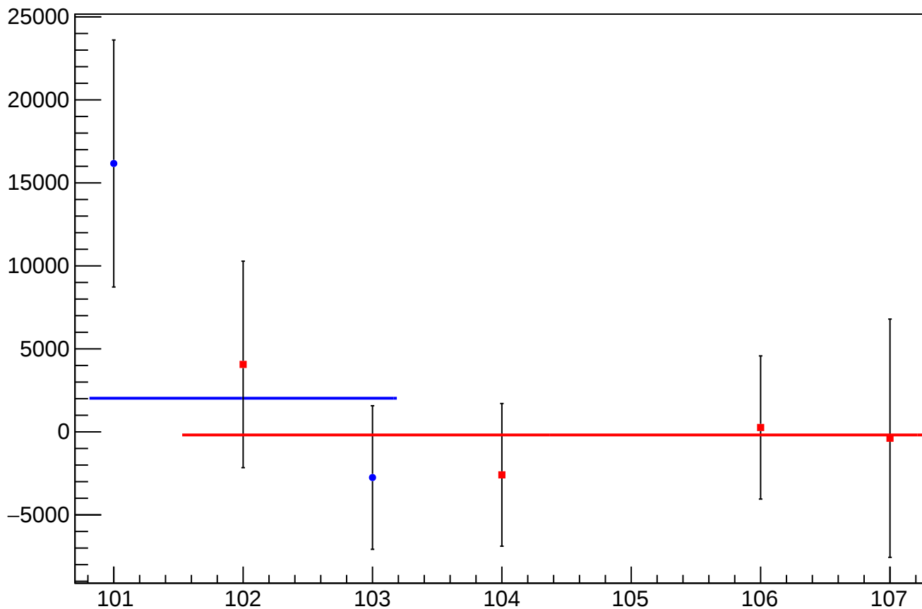
asym_at1_avg_mean vs Slug, Sign Corrected
