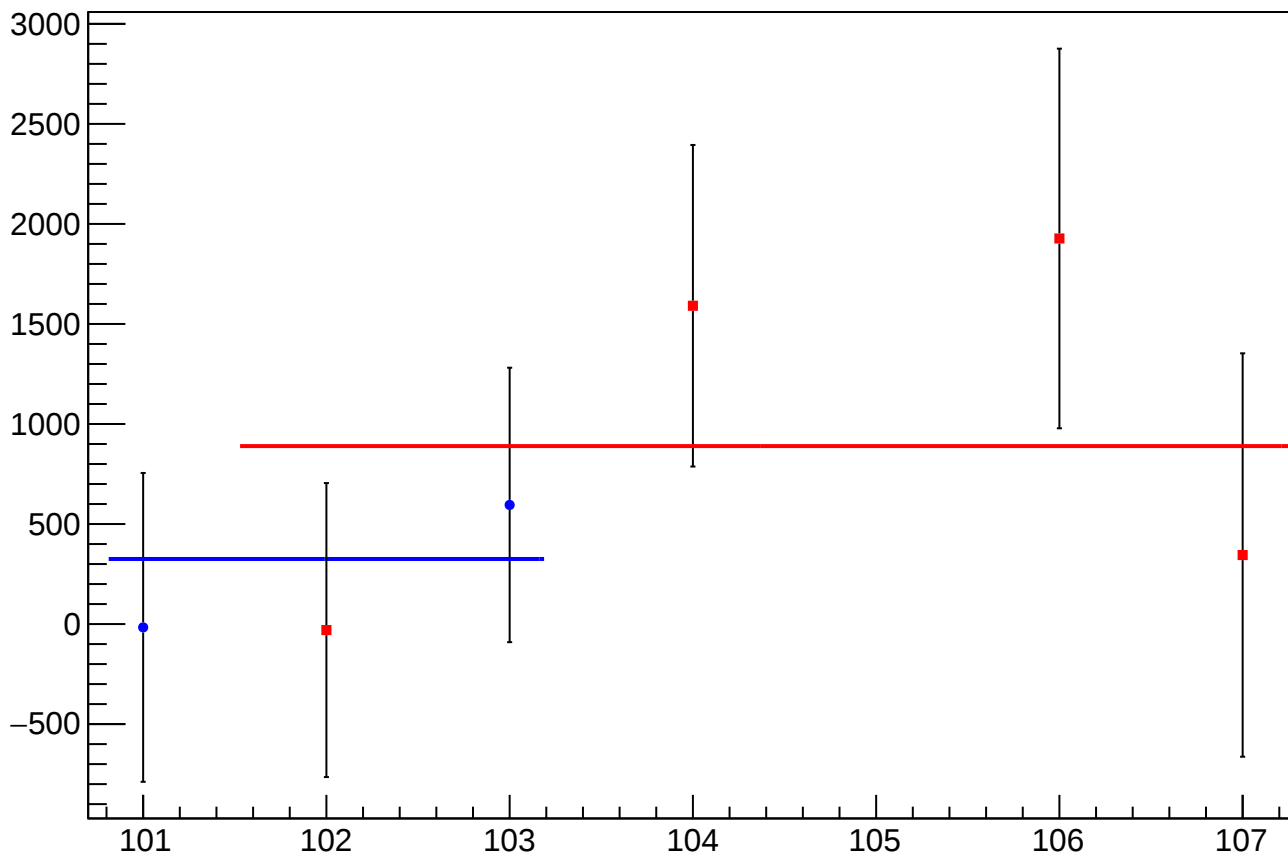
asym_sam5_correction_mean vs Slug, Sign Corrected
