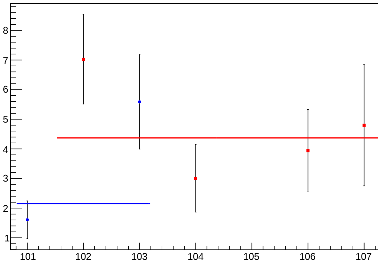
reg_asym_left_avg_diff_bpm4aY_slope vs Slug, Sign Corrected
