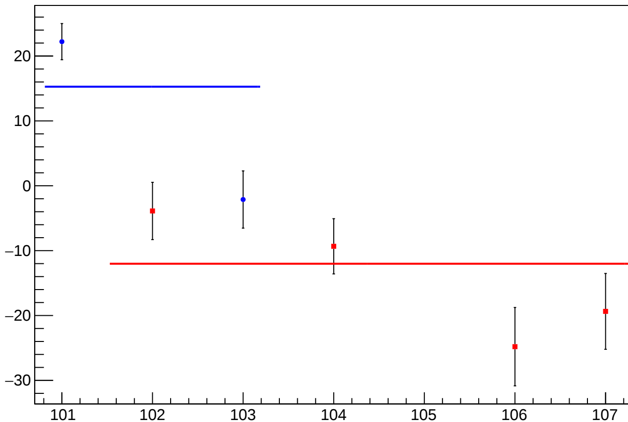
reg_asym_usr_diff_bpm4aX_slope vs Slug, Sign Corrected
