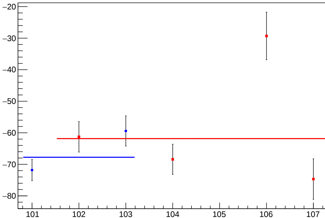
reg_asym_sam_26_avg_diff_bpm4eX_slope vs Slug, Sign Corrected
