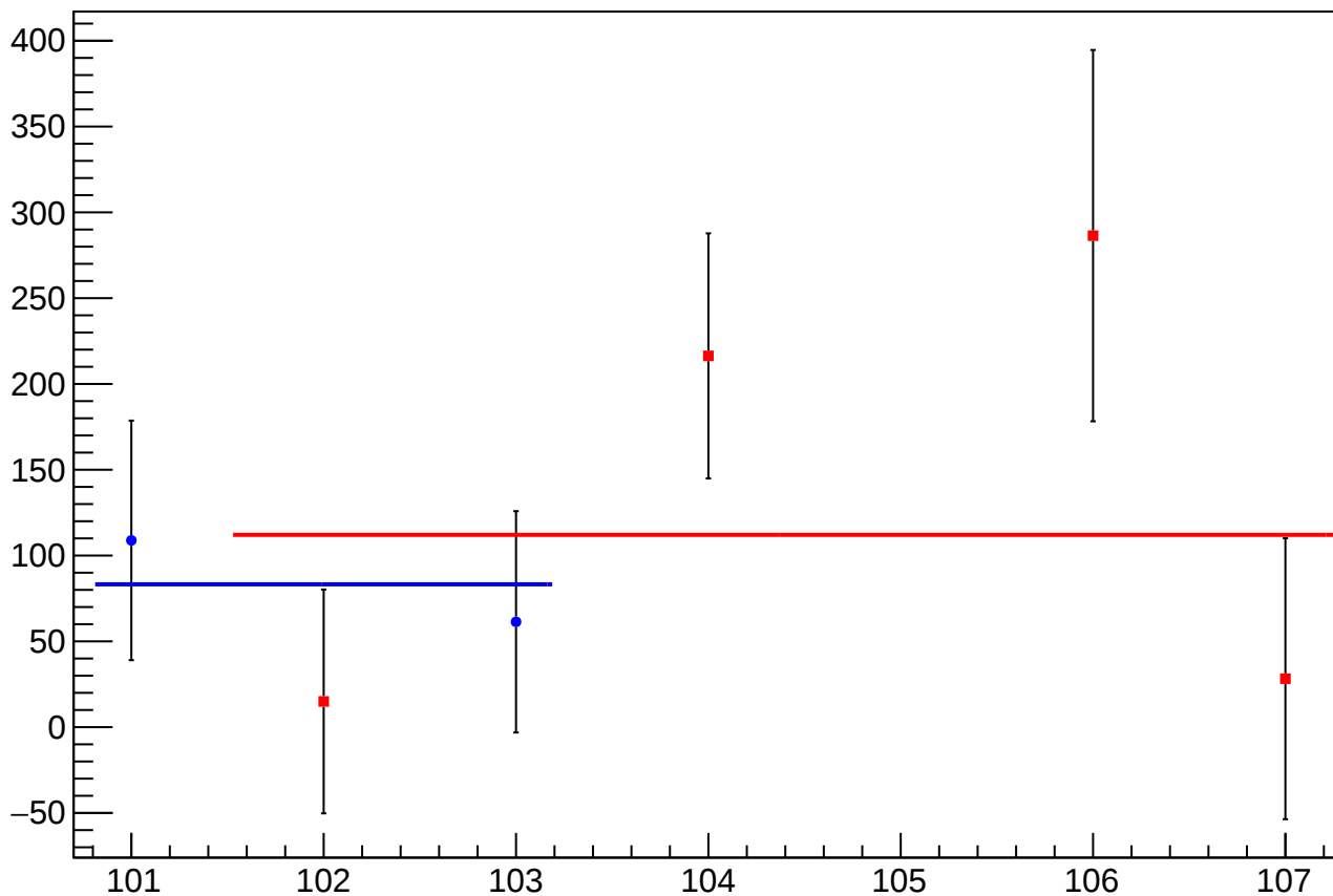
dit_asym_sam_15_avg_mean vs Slug, Sign Corrected
