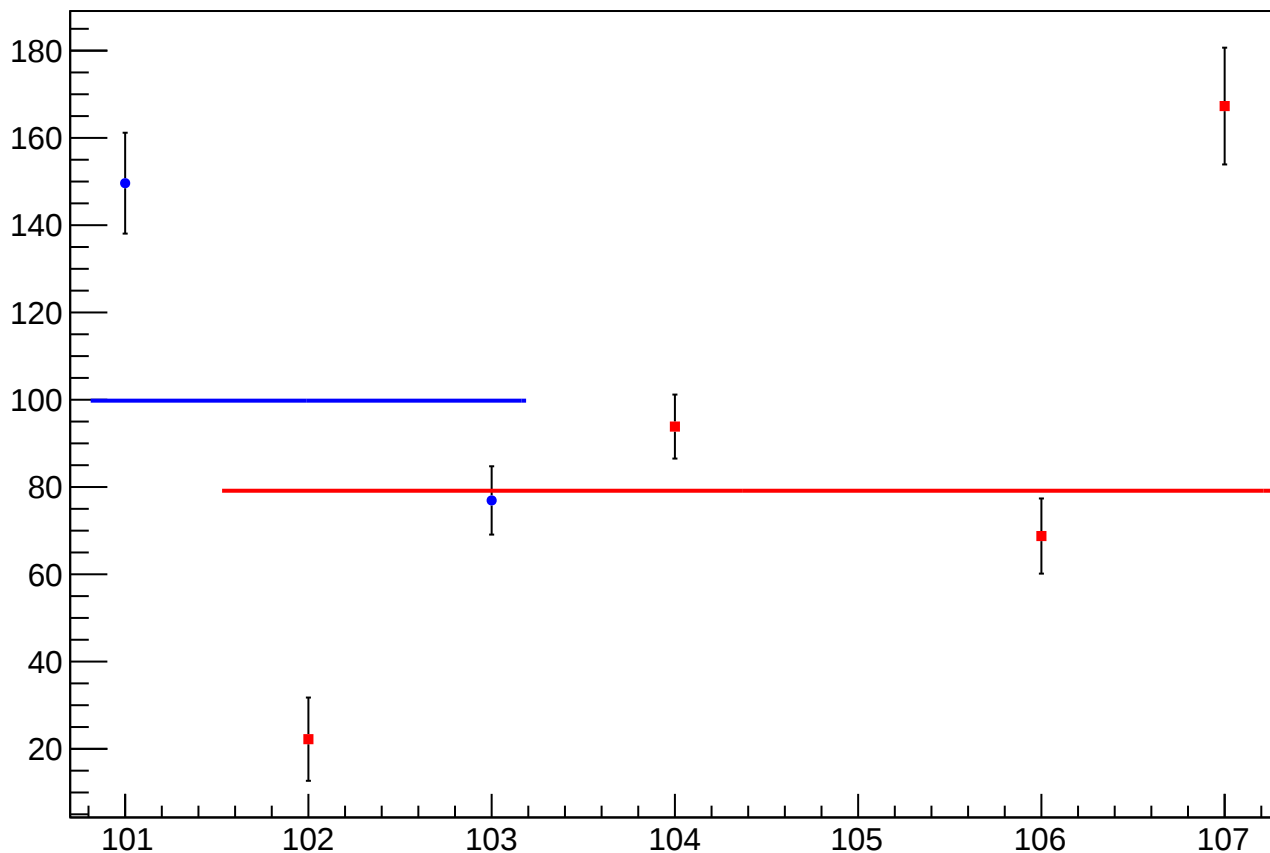
reg_asym_atr1l2_dd_diff_bpm4aX_slope vs Slug, Sign Corrected
