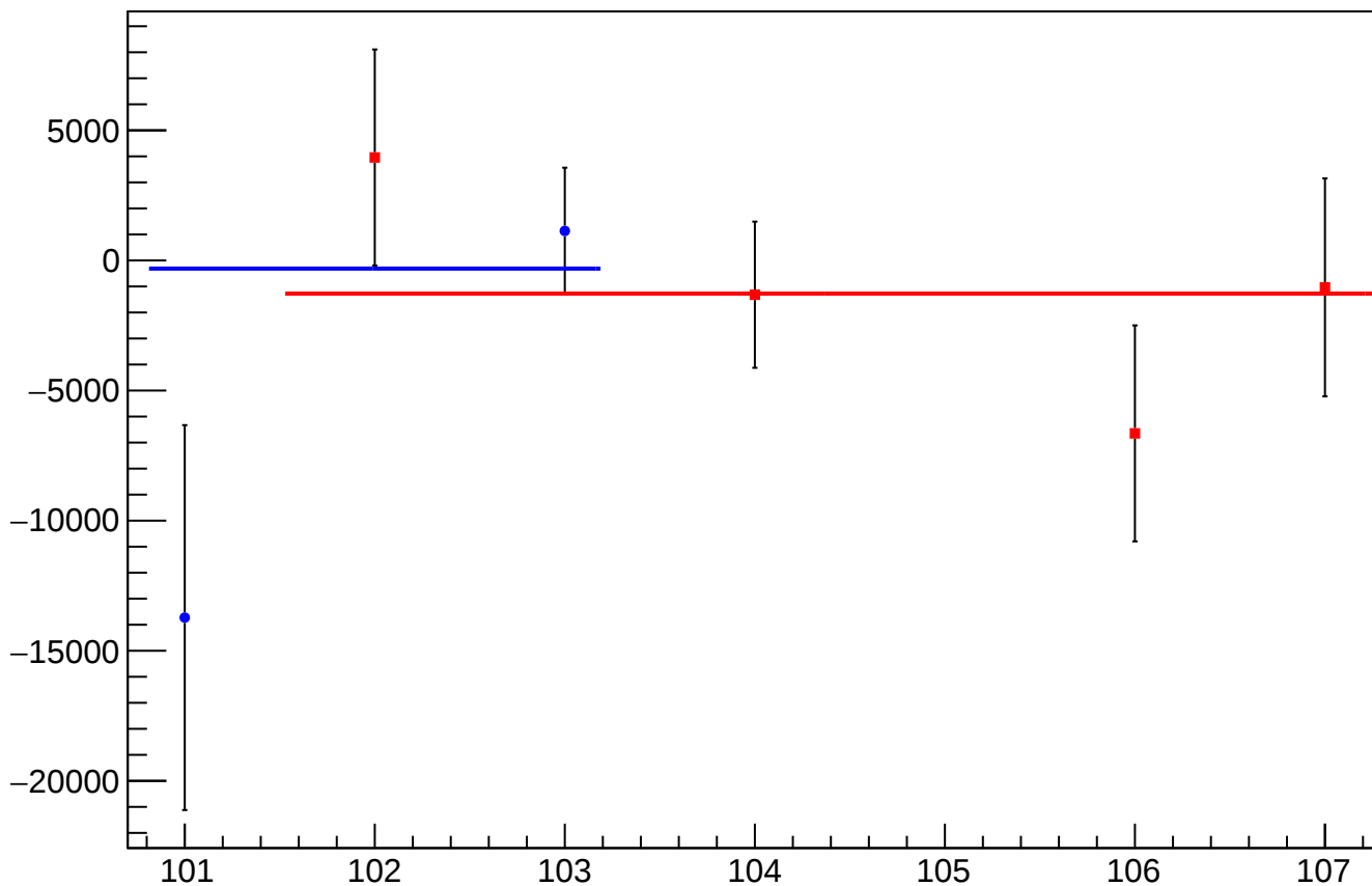
dit_asym_at1_dd_mean vs Slug, Sign Corrected
