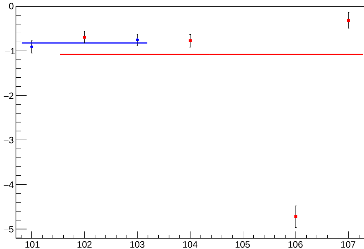
reg_asym_sam_26_dd_diff_bpm12X_slope vs Slug, Sign Corrected
