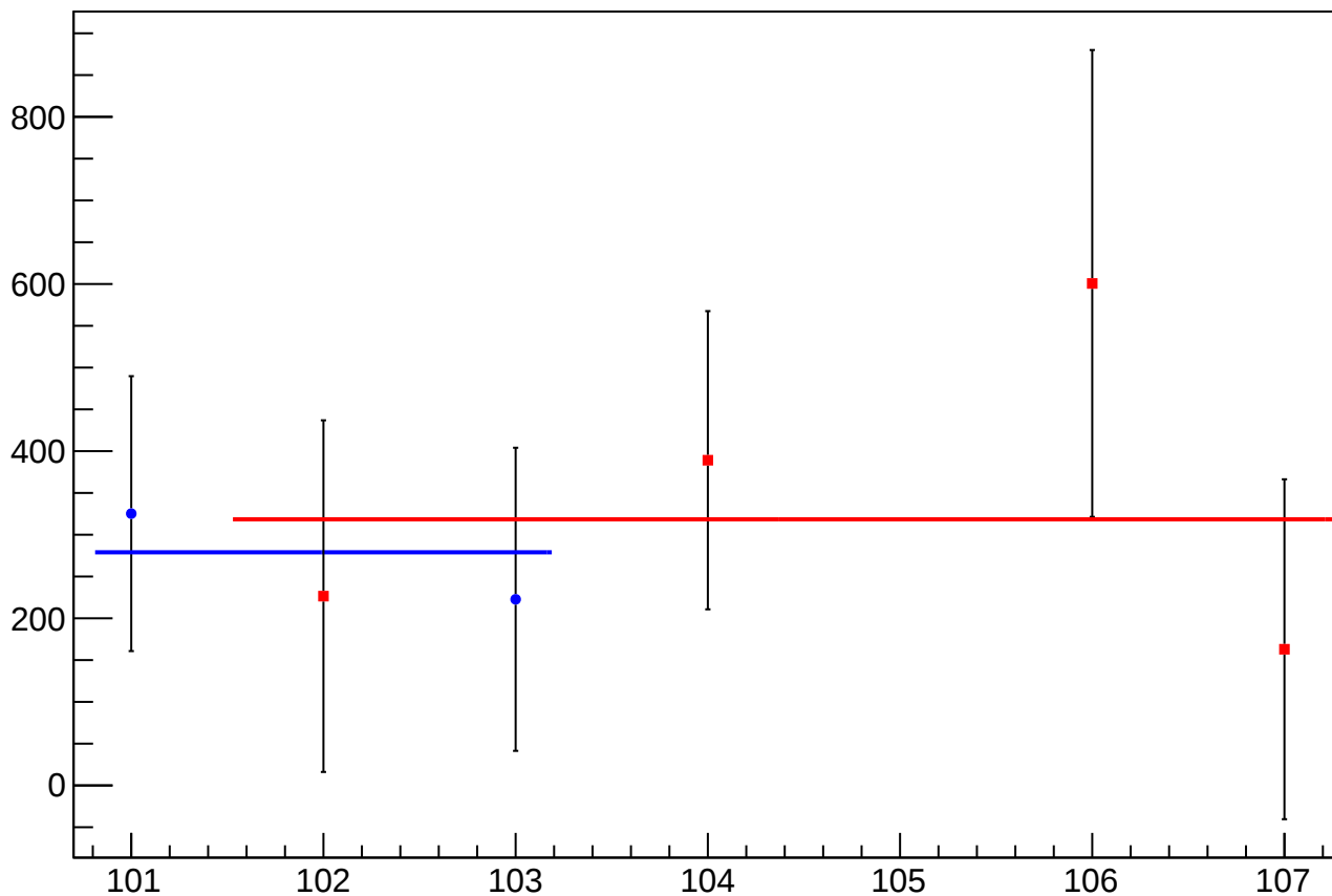
dit_asym_sam_24_68_dd_mean vs Slug, Sign Corrected
