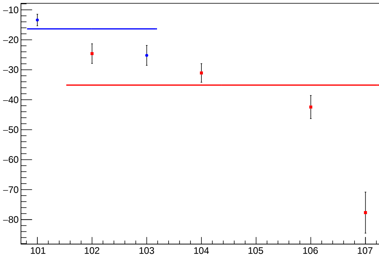
reg_asym_us_avg_diff_bpm4aX_slope vs Slug, Sign Corrected
