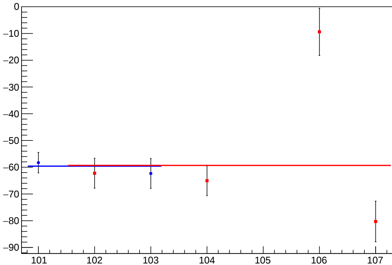
reg_asym_sam_26_dd_diff_bpm4eX_slope vs Slug, Sign Corrected
