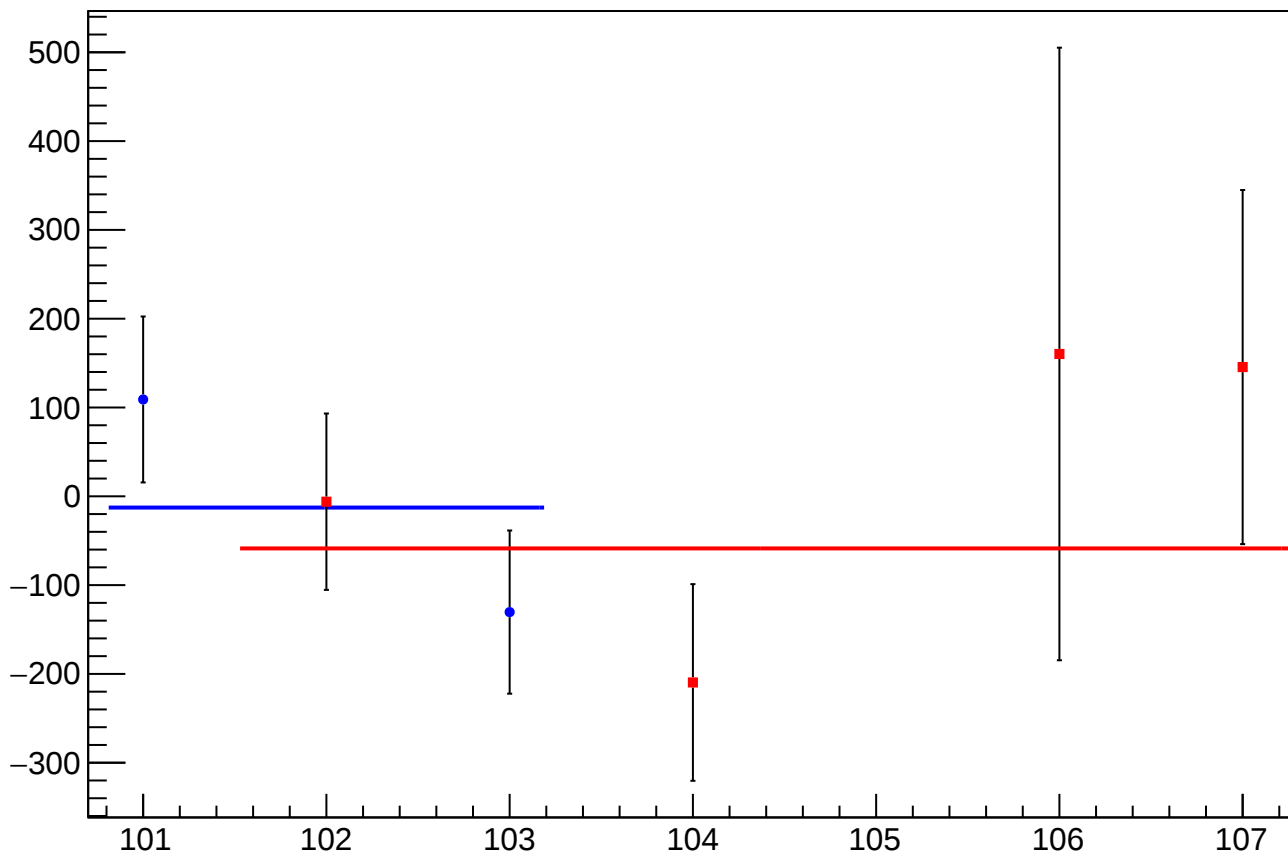
asym_sam_15_avg_correction_mean vs Slug, Sign Corrected
