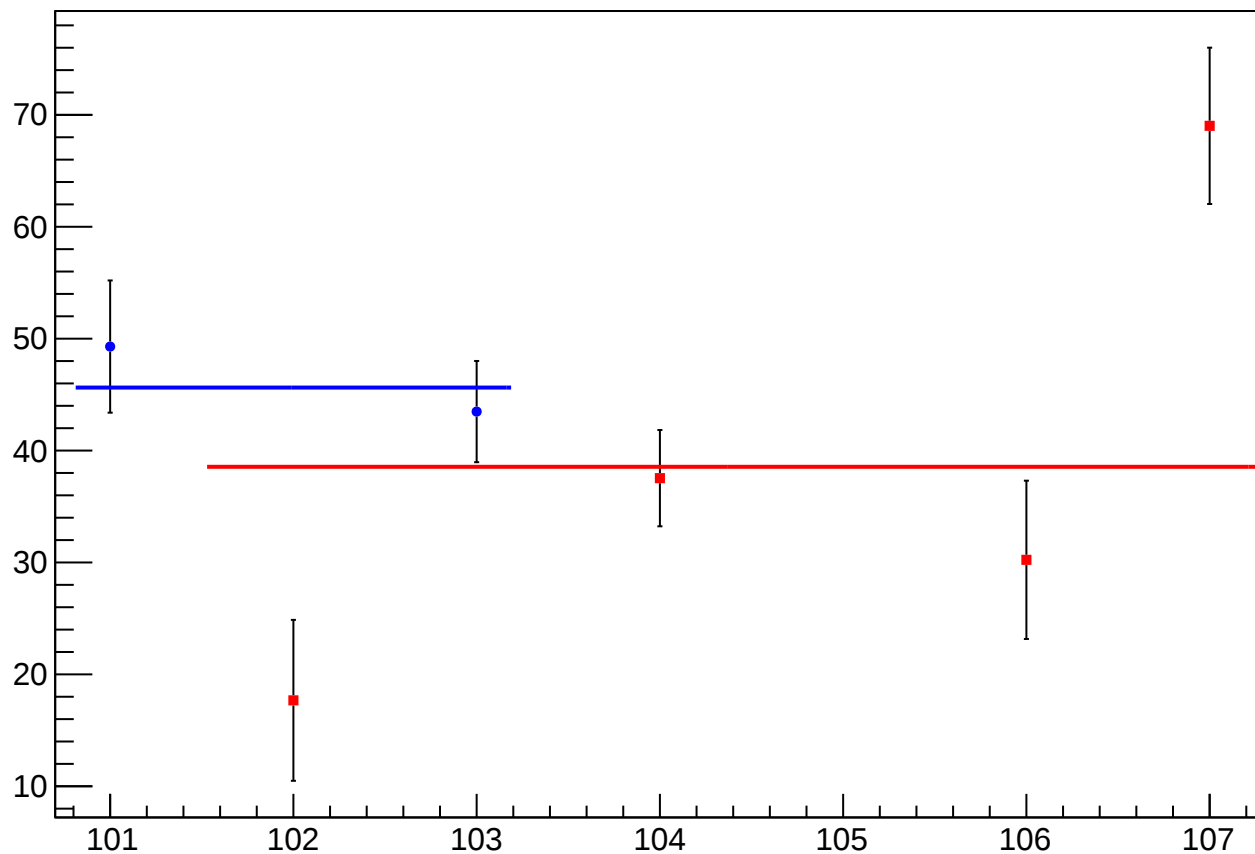
reg_asym_at2_dd_diff_bpm4aX_slope vs Slug, Sign Corrected
