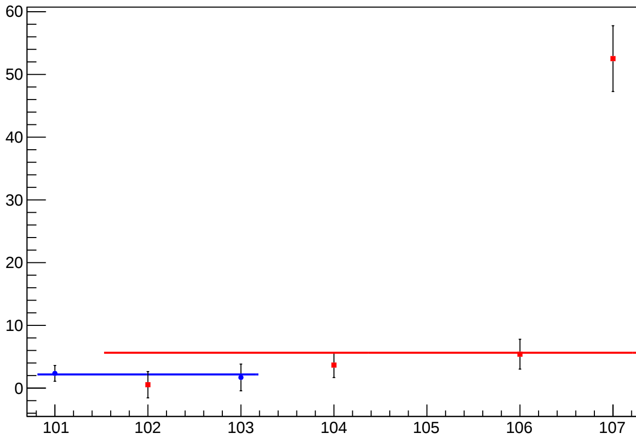
reg_asym_left_avg_diff_bpm4eX_slope vs Slug, Sign Corrected
