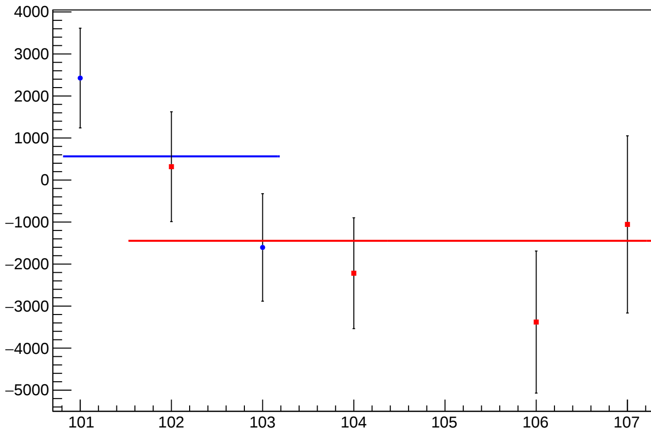
asym_sam_48_dd_mean vs Slug, Sign Corrected
